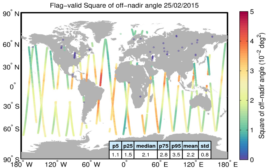
Figure 37. Geographical distribution of flag-valid mispointing data over oceans and lakes for 25/02/2015. The statistical values shown in the table refer to the mispointing in 10^{-2} \text{ deg}^2 and are calculated over all measurements shown in the figure.
