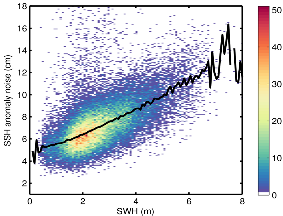
Figure 9. 2D histogram showing flag-valid SSH anomaly noise as a function of SWH for 25/02/2015. The black line denotes the median SSH anomaly as a function of SWH.
