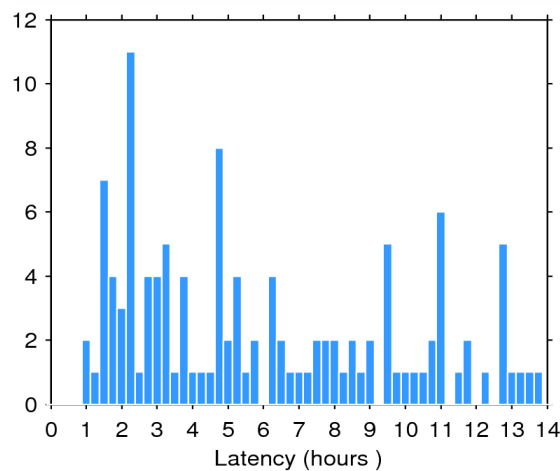
Figure 2. Histogram of the data latency for 25/02/2015. The y-axis denotes the number of files that are made available with a delay of x-hours with respect to the mean time of the records stored in the file.
