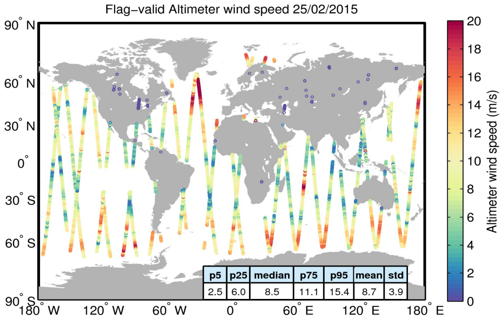
Figure 31. Geographical distribution of flag-valid wind data over oceans and lakes for 25/02/2015. The statistical values shown in the table refer to the wind in m/s and are calculated over all measurements shown in the figure.
