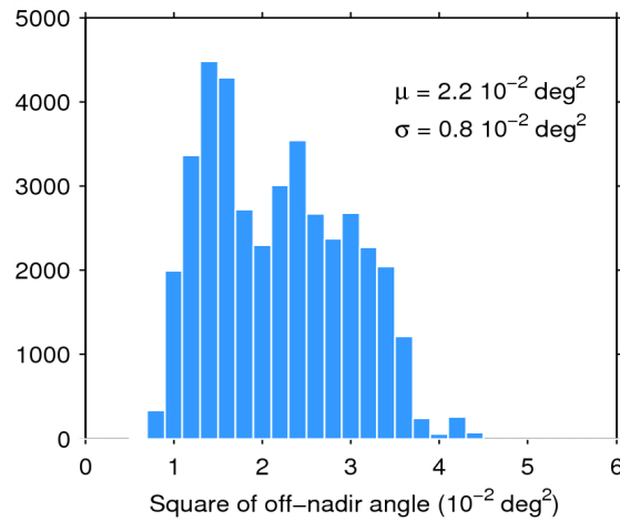
Figure 39. Histogram of flag-valid mispointing over oceans and lakes for 25/02/2015. The mean ( \mu ) and standard deviation ( \sigma ) are also shown. Note that values than 6 \cdot 10^{-2} \text{ deg}^2 are excluded from the histogram for the sake of readability but not from the computation of \mu and \sigma .
