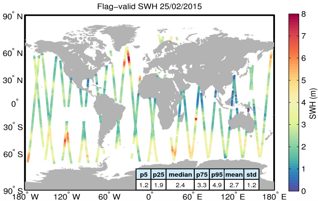
Figure 15. Geographical distribution of flag-valid SWH data over oceans and lakes for 25/02/2015. The statistical values shown in the table refer to the SWH in m and are calculated over all measurements shown in the figure.
