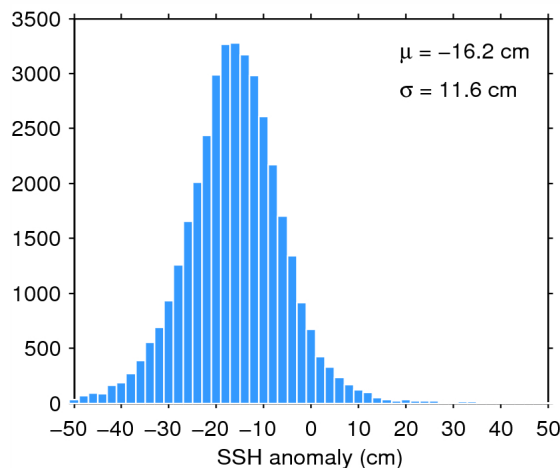
Figure 11. Histogram of science-valid SSH anomaly over oceans and lakes for 25/02/2015. The mean ( \mu ) and standard deviation ( \sigma ) are also shown. Note that values outside [-50 50] cm are excluded from the histogram for the sake of readability but not from the computation of \mu and \sigma .
