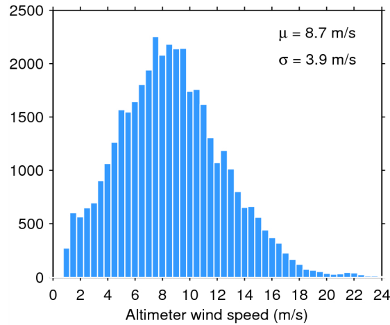
Figure 33. Histogram of flag-valid wind over oceans and lakes for 25/02/2015. The mean ( \mu ) and standard deviation ( \sigma ) are also shown. Note that values larger than 24 m/s are excluded from the histogram for the sake of readability but not from the computation of \mu and \sigma .
