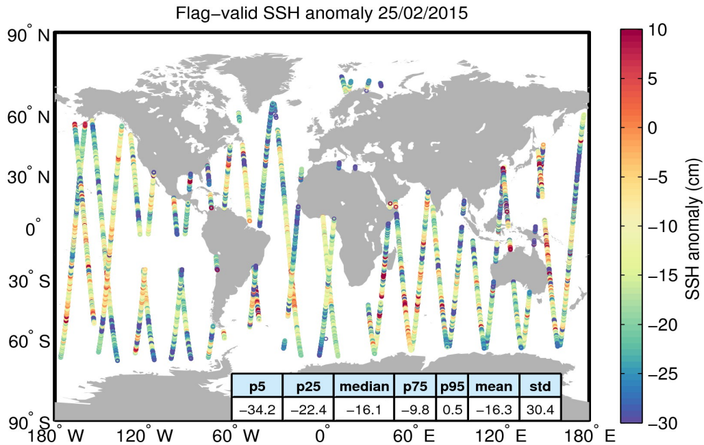
Figure 5. Geographical distribution of flag-valid 1-Hz SSH anomaly data over oceans and lakes for 25/02/2015. The statistical values shown in the table refer to the SSH anomaly in cm and are calculated over all measurements shown in the figure.
