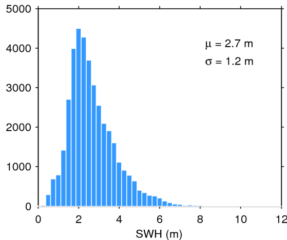
Figure 20. Histogram of science-valid SWH over oceans and lakes for 25/02/2015. The mean ( \mu ) and standard deviation ( \sigma ) are also shown. Note that values larger than 12 m are excluded from the histogram for the sake of readability but not from the computation of \mu and \sigma .
