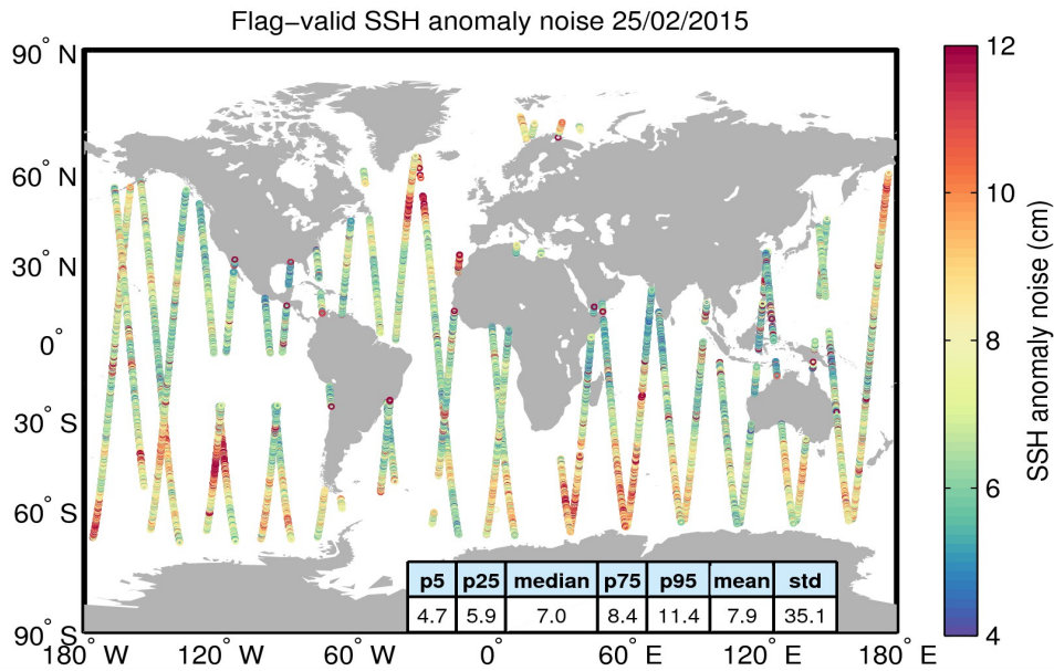
Figure 8. Geographical distribution of flag-valid 20-Hz SSH anomaly measurement noise over oceans and lakes for 25/02/2015. The statistical values shown in the table refer to the SSH anomaly noise and are calculated over all measurements shown in the figure.
