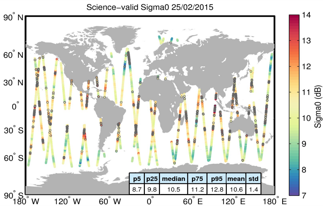
Figure 27. Geographical distribution of science-valid sigma0 data over oceans and lakes for 25/02/2015. The statistical values shown in the table refer to the sigma0 in dB and are calculated over all measurements shown in the figure. Gray circles denote records that have been rejected based on the editing criteria described in Table 4.
