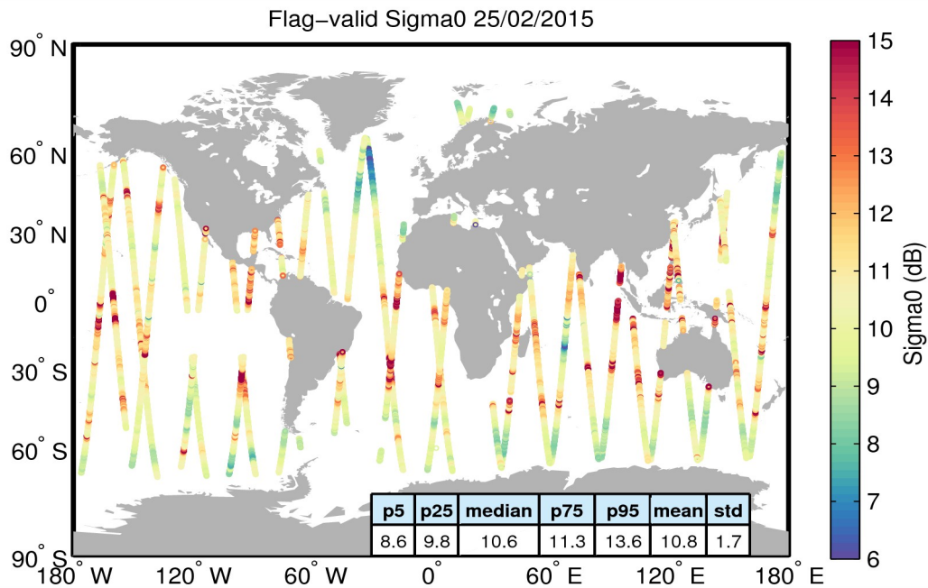
Figure 23. Geographical distribution of flag-valid sigma0 data over oceans and lakes for 25/02/2015. The statistical values shown in the table refer to the sigma0 in dB and are calculated over all measurements shown in the figure.
