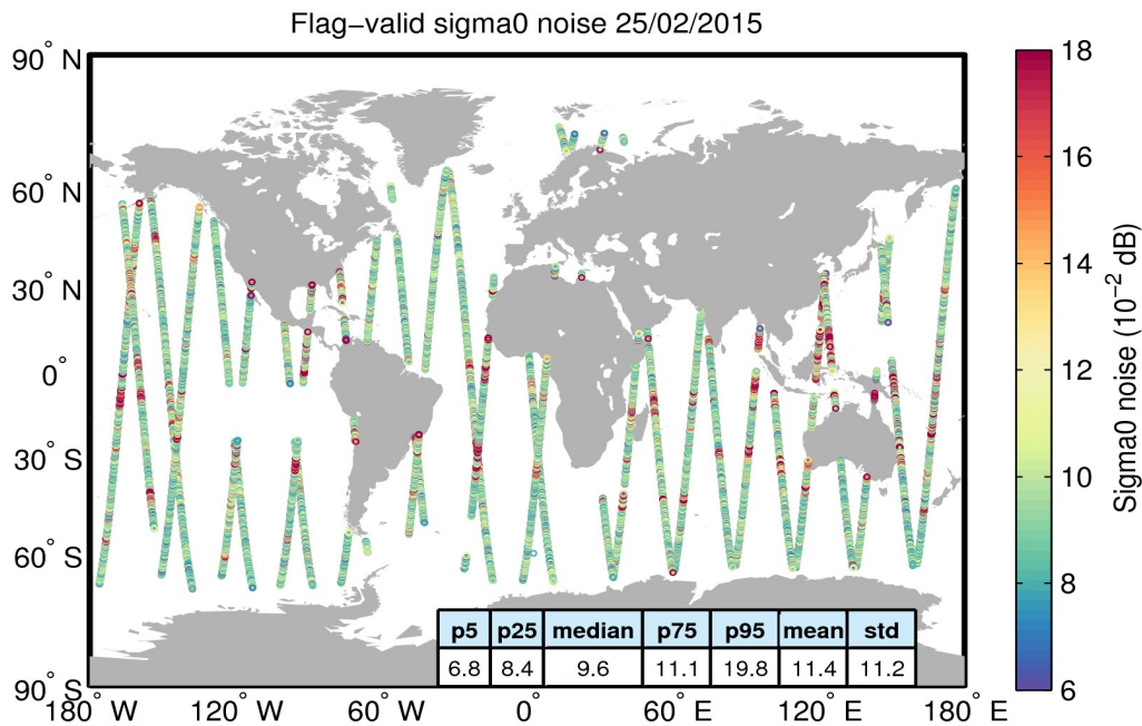
Figure 26. Geographical distribution of flag-valid 20-Hz sigma0 measurement noise over oceans and lakes for 25/02/2015. The statistical values shown in the table refer to the sigma0 noise and are calculated over all measurements shown in the figure.
