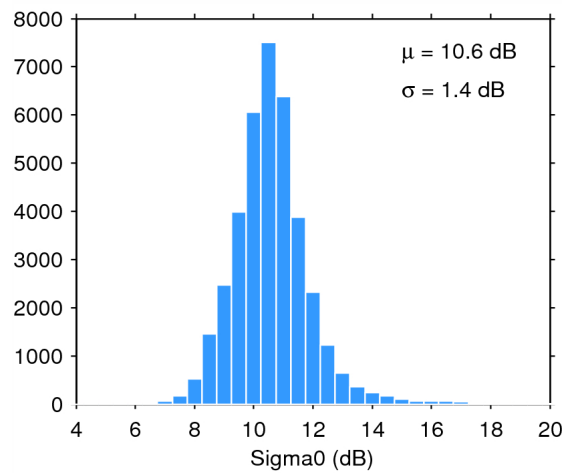
Figure 28. Histogram of science-valid sigma0 over oceans and lakes for 25/02/2015. The mean ( \mu ) and standard deviation ( \sigma ) are also shown. Note that values outside [4 20] dB are excluded from the histogram for the sake of readability but not from the computation of \mu and \sigma .
