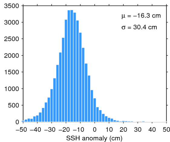
Figure 7. Histogram of flag-valid SSH anomaly over oceans and lakes for 25/02/2015. The mean ( \mu ) and standard deviation ( \sigma ) are also shown. Note that values outside [-50 50] cm are excluded from the histogram for the sake of readability but not from the computation of \mu and \sigma .
