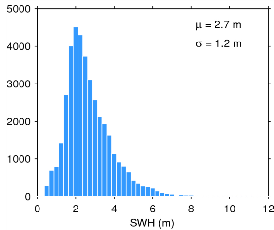
Figure 17. Histogram of flag-valid SWH over oceans and lakes for 25/02/2015. The mean ( \mu ) and standard deviation ( \sigma ) are also shown. Note that values larger than 12 m are excluded from the histogram for the sake of readability but not from the computation of \mu and \sigma .
