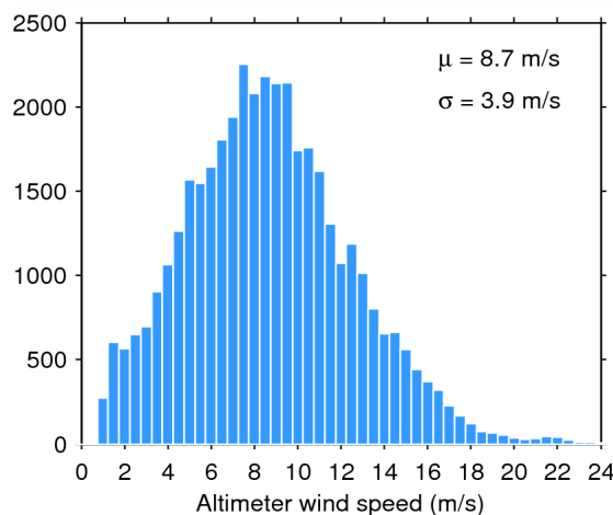
Figure 35. Histogram of science-valid wind over oceans and lakes for 25/02/2015. The mean ( \mu ) and standard deviation ( \sigma ) are also shown. Note that values larger than 24 m/s are excluded from the histogram for the sake of readability but not from the computation of \mu and \sigma .
