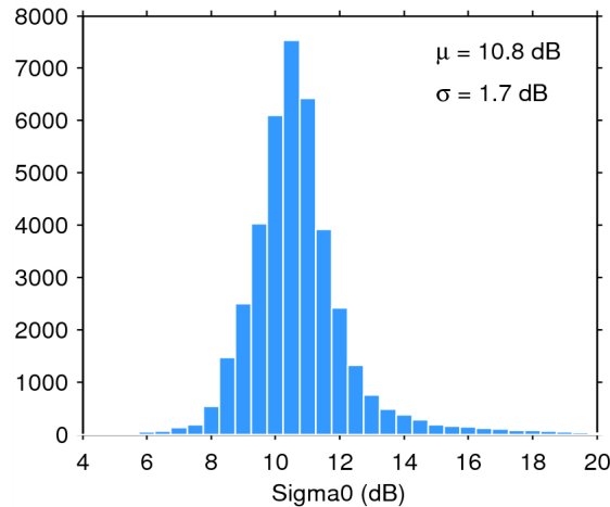
Figure 25. Histogram of flag-valid sigma0 over oceans and lakes for 25/02/2015. The mean ( \mu ) and standard deviation ( \sigma ) are also shown. Note that values outside [4 20] dB are excluded from the histogram for the sake of readability but not from the computation of \mu and \sigma .
