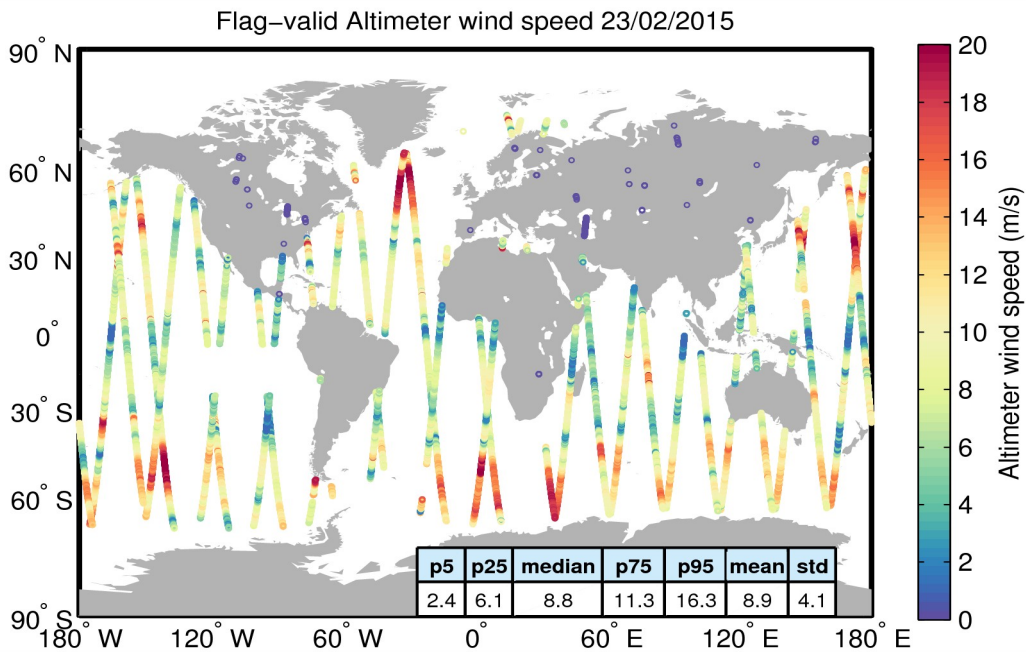
Figure 31. Geographical distribution of flag-valid wind data over oceans and lakes for 23/02/2015. The statistical values shown in the table refer to the wind in m/s and are calculated over all measurements shown in the figure.
