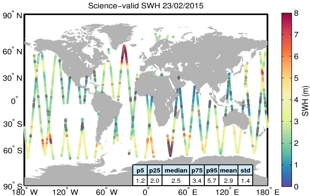
Figure 19. Geographical distribution of science-valid SWH data over oceans and lakes for 23/02/2015. The statistical values shown in the table refer to the SWH in m and are calculated over all measurements shown in the figure. Gray circles denote records that have been rejected based on the editing criteria described in Table 3.
