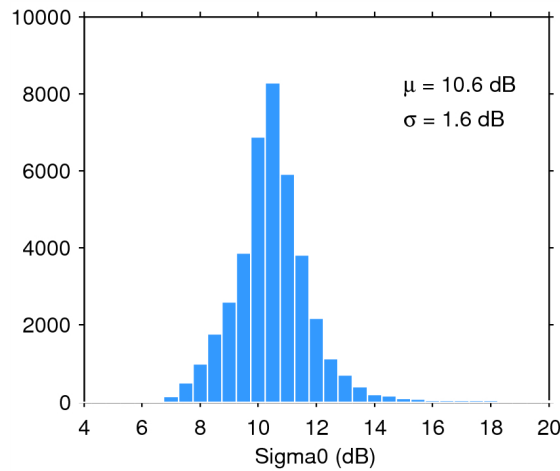
Figure 28. Histogram of science-valid sigma0 over oceans and lakes for 23/02/2015. The mean ( \mu ) and standard deviation ( \sigma ) are also shown. Note that values outside [4 20] dB are excluded from the histogram for the sake of readability but not from the computation of \mu and \sigma .
