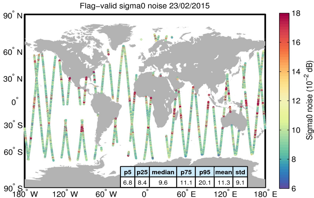
Figure 26. Geographical distribution of flag-valid 20-Hz sigma0 measurement noise over oceans and lakes for 23/02/2015. The statistical values shown in the table refer to the sigma0 noise and are calculated over all measurements shown in the figure.
