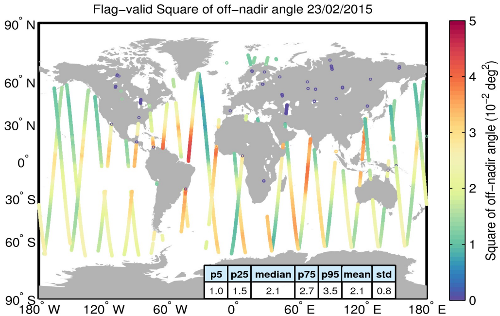
Figure 37. Geographical distribution of flag-valid mispointing data over oceans and lakes for 23/02/2015. The statistical values shown in the table refer to the mispointing in 10^{-2} \text{deg}^2 and are calculated over all measurements shown in the figure.
