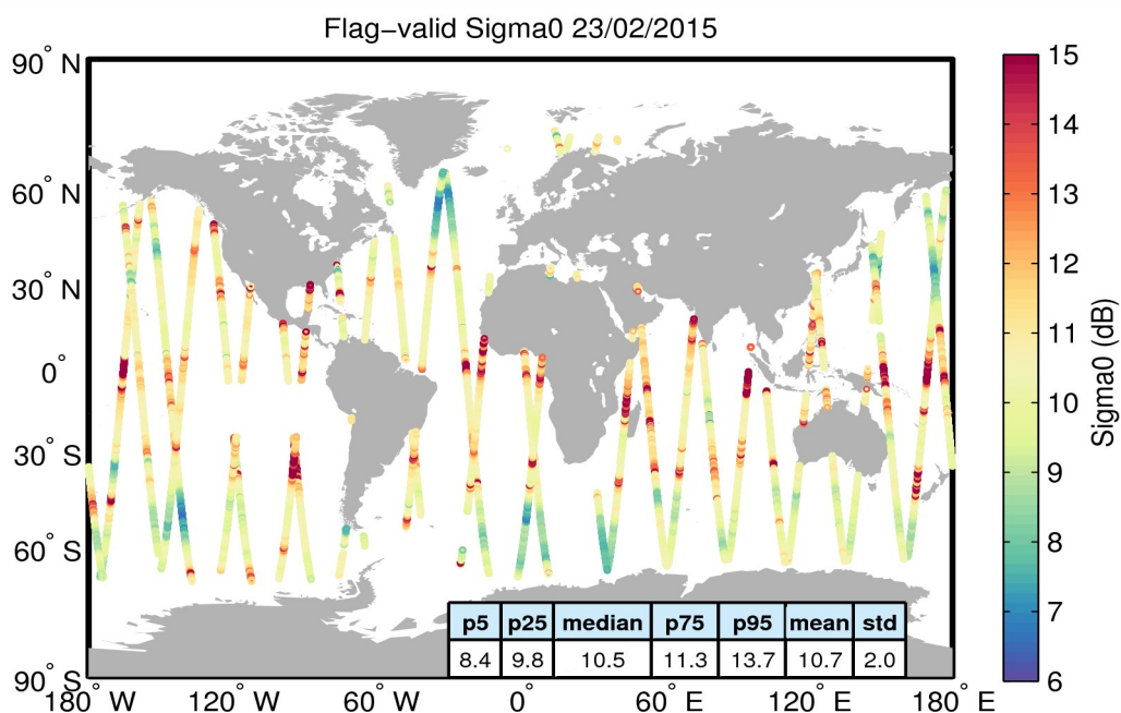
Figure 23. Geographical distribution of flag-valid sigma0 data over oceans and lakes for 23/02/2015. The statistical values shown in the table refer to the sigma0 in dB and are calculated over all measurements shown in the figure.
