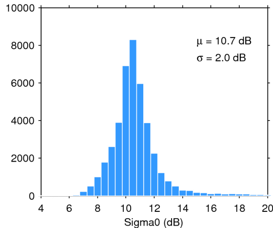
Figure 25. Histogram of flag-valid sigma0 over oceans and lakes for 23/02/2015. The mean ( \mu ) and standard deviation ( \sigma ) are also shown. Note that values outside [4 20] dB are excluded from the histogram for the sake of readability but not from the computation of \mu and \sigma .
