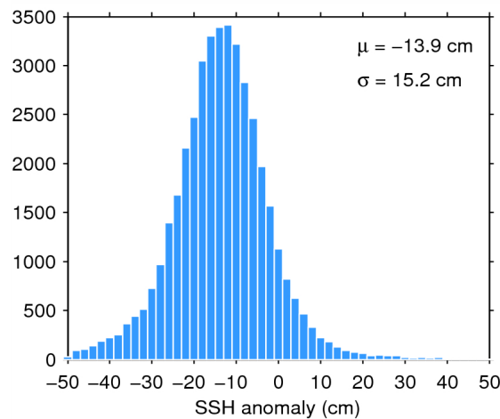
Figure 7. Histogram of flag-valid SSH anomaly over oceans and lakes for 23/02/2015. The mean ( \mu ) and standard deviation ( \sigma ) are also shown. Note that values outside [-50\ 50] cm are excluded from the histogram for the sake of readability but not from the computation of \mu and \sigma .
