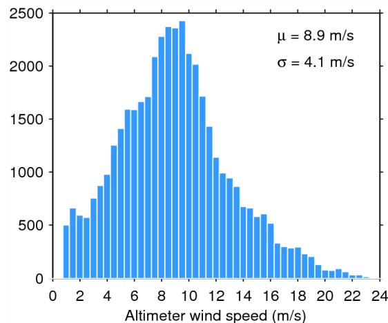
Figure 35. Histogram of science-valid wind over oceans and lakes for 23/02/2015. The mean ( \mu ) and standard deviation ( \sigma ) are also shown. Note that values larger than 24 m/s are excluded from the histogram for the sake of readability but not from the computation of \mu and \sigma .
