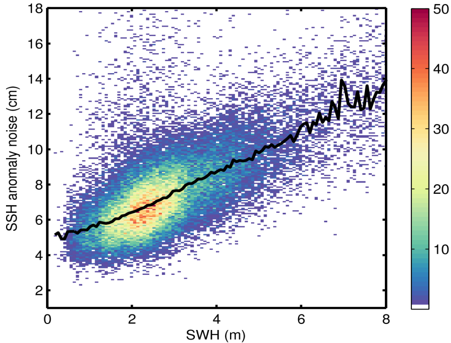
Figure 9. 2D histogram showing flag-valid SSH anomaly noise as a function of SWH for 23/02/2015. The black line denotes the median SSH anomaly as a function of SWH.
