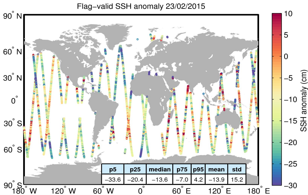
Figure 5. Geographical distribution of flag-valid 1-Hz SSH anomaly data over oceans and lakes for 23/02/2015. The statistical values shown in the table refer to the SSH anomaly in cm and are calculated over all measurements shown in the figure.
