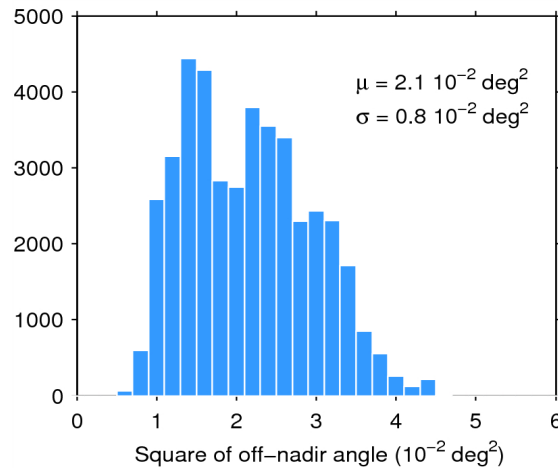
Figure 39. Histogram of flag-valid mispointing over oceans and lakes for 23/02/2015. The mean ( \mu ) and standard deviation ( \sigma ) are also shown. Note that values than 6 \cdot 10^{-2} \text{ deg}^2 are excluded from the histogram for the sake of readability but not from the computation of \mu and \sigma .
