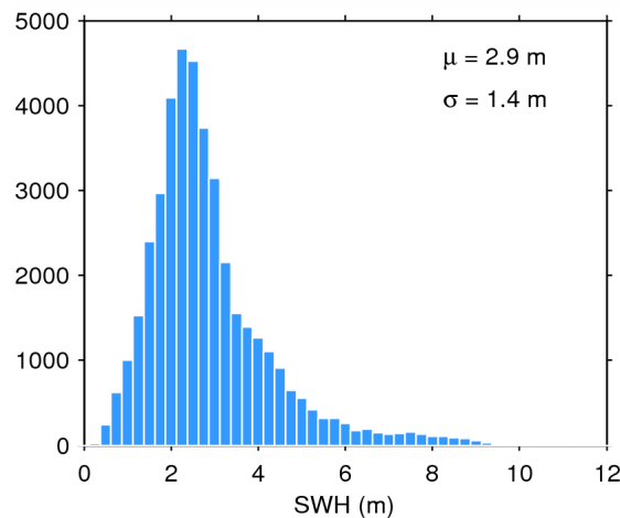
Figure 20. Histogram of science-valid SWH over oceans and lakes for 23/02/2015. The mean ( \mu ) and standard deviation ( \sigma ) are also shown. Note that values larger than 12 m are excluded from the histogram for the sake of readability but not from the computation of \mu and \sigma .
