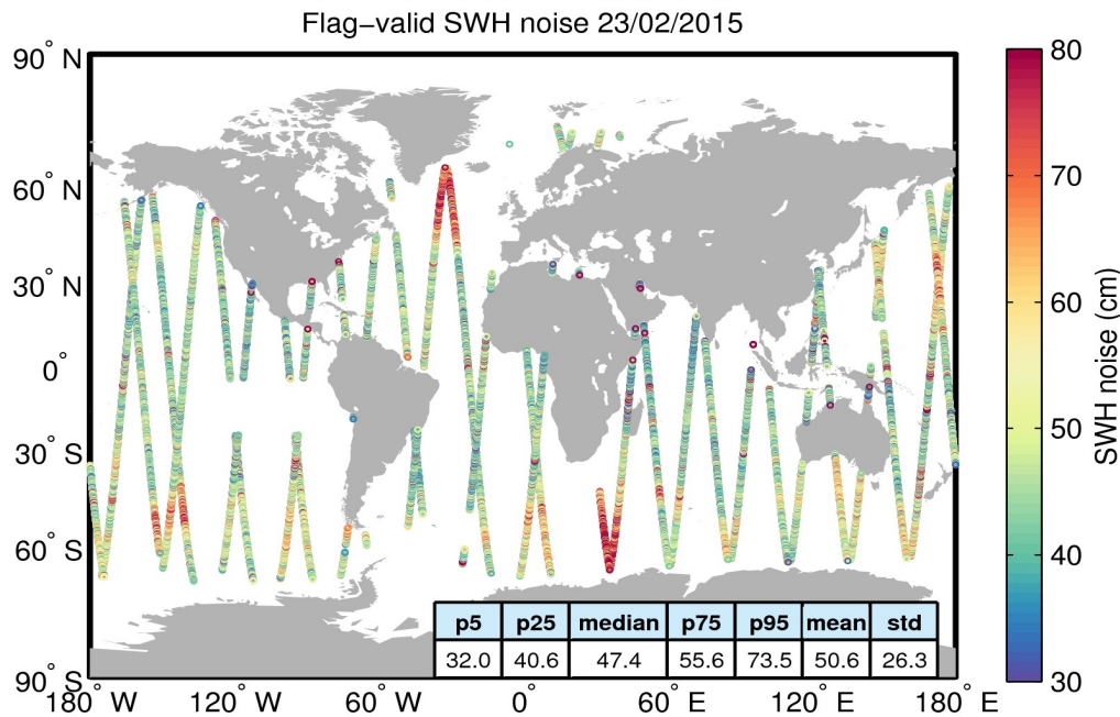
Figure 18. Geographical distribution of flag-valid 20-Hz SWH measurement noise over oceans and lakes for 23/02/2015. The statistical values shown in the figure refer to the SWH noise and are calculated over all measurements shown in the figure.
