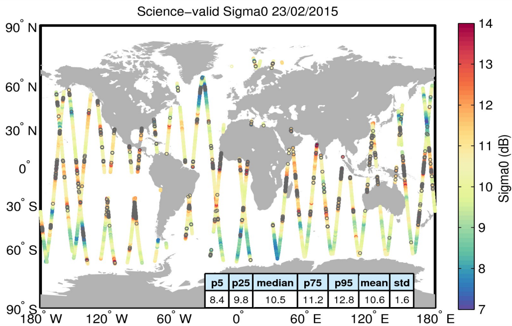
Figure 27. Geographical distribution of science-valid sigma0 data over oceans and lakes for 23/02/2015. The statistical values shown in the table refer to the sigma0 in dB and are calculated over all measurements shown in the figure. Gray circles denote records that have been rejected based on the editing criteria described in Table 4.
