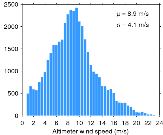
Figure 33. Histogram of flag-valid wind over oceans and lakes for 23/02/2015. The mean ( \mu ) and standard deviation ( \sigma ) are also shown. Note that values larger than 24 m/s are excluded from the histogram for the sake of readability but not from the computation of \mu and \sigma .
