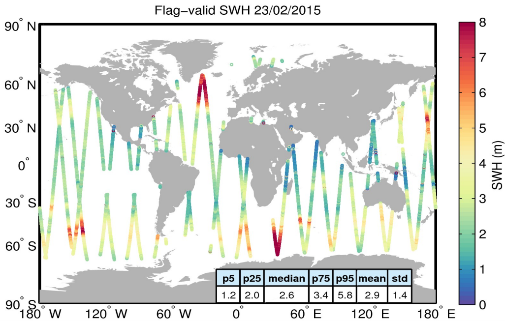
Figure 15. Geographical distribution of flag-valid SWH data over oceans and lakes for 23/02/2015. The statistical values shown in the table refer to the SWH in m and are calculated over all measurements shown in the figure.
