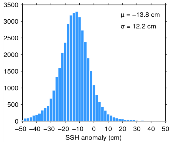
Figure 11. Histogram of science-valid SSH anomaly over oceans and lakes for 23/02/2015. The mean ( \mu ) and standard deviation ( \sigma ) are also shown. Note that values outside [-50 50] cm are excluded from the histogram for the sake of readability but not from the computation of \mu and \sigma .
