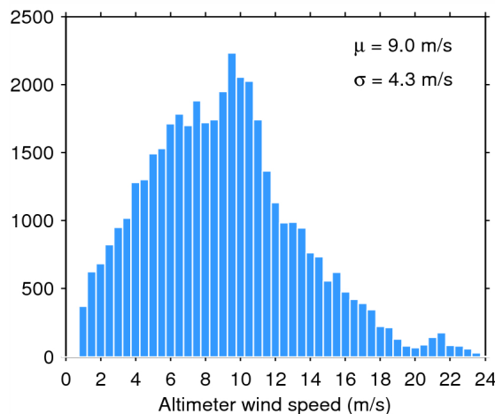
Figure 35. Histogram of science-valid wind over oceans and lakes for 22/02/2015. The mean ( \mu ) and standard deviation ( \sigma ) are also shown. Note that values larger than 24 m/s are excluded from the histogram for the sake of readability but not from the computation of \mu and \sigma .
