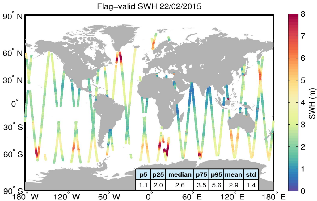
Figure 15. Geographical distribution of flag-valid SWH data over oceans and lakes for 22/02/2015. The statistical values shown in the table refer to the SWH in m and are calculated over all measurements shown in the figure.
