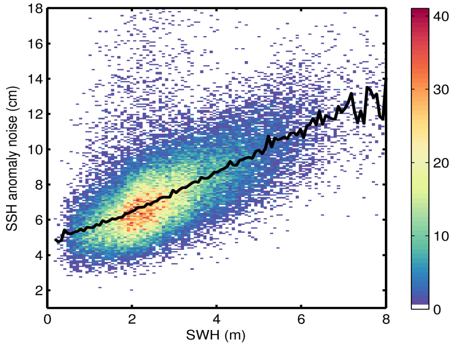
Figure 9. 2D histogram showing flag-valid SSH anomaly noise as a function of SWH for 22/02/2015. The black line denotes the median SSH anomaly as a function of SWH.
