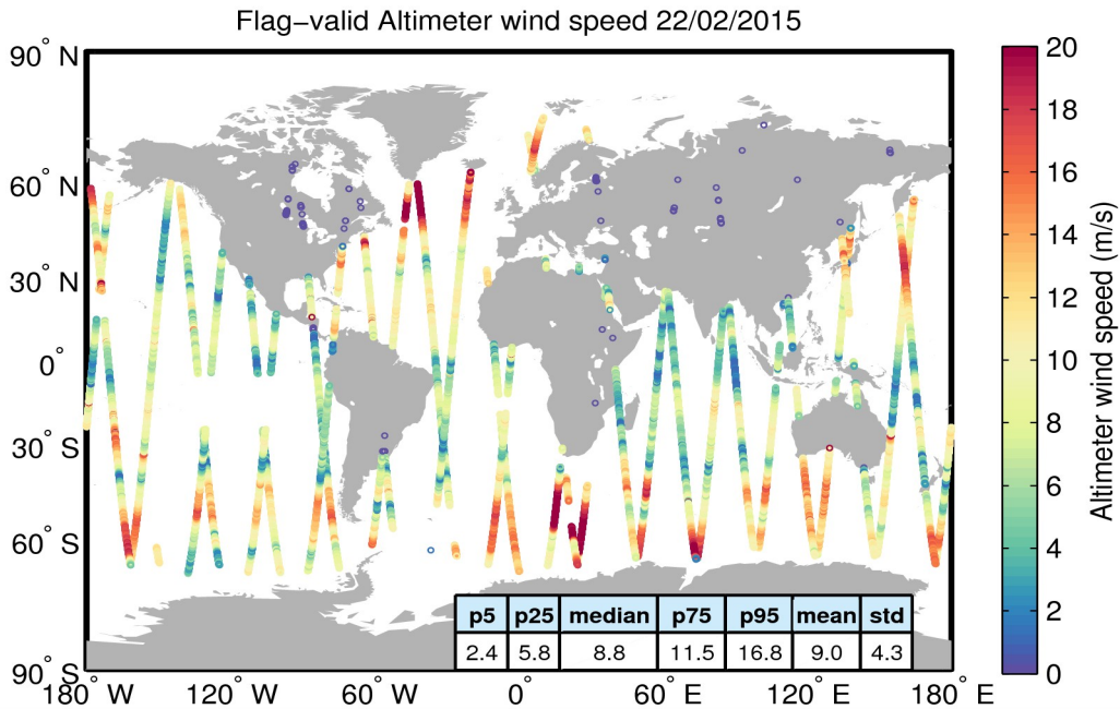
Figure 31. Geographical distribution of flag-valid wind data over oceans and lakes for 22/02/2015. The statistical values shown in the table refer to the wind in m/s and are calculated over all measurements shown in the figure.
