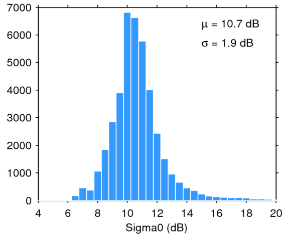
Figure 25. Histogram of flag-valid sigma0 over oceans and lakes for 22/02/2015. The mean ( \mu ) and standard deviation ( \sigma ) are also shown. Note that values outside [4 20] dB are excluded from the histogram for the sake of readability but not from the computation of \mu and \sigma .
