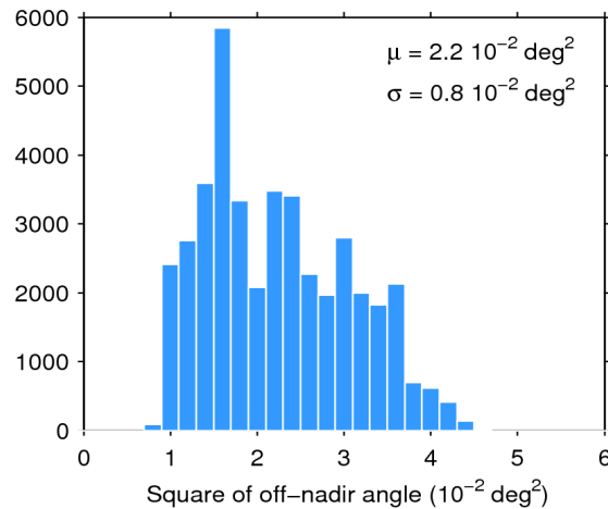
Figure 39. Histogram of flag-valid mispointing over oceans and lakes for 22/02/2015. The mean ( \mu ) and standard deviation ( \sigma ) are also shown. Note that values than 6 \cdot 10^{-2} \text{ deg}^2 are excluded from the histogram for the sake of readability but not from the computation of \mu and \sigma .
