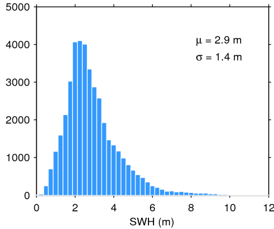
Figure 20. Histogram of science-valid SWH over oceans and lakes for 22/02/2015. The mean ( \mu ) and standard deviation ( \sigma ) are also shown. Note that values larger than 12 m are excluded from the histogram for the sake of readability but not from the computation of \mu and \sigma .
