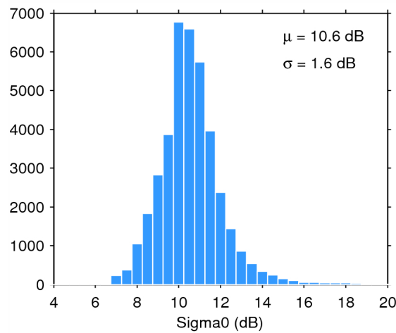
Figure 28. Histogram of science-valid sigma0 over oceans and lakes for 22/02/2015. The mean ( \mu ) and standard deviation ( \sigma ) are also shown. Note that values outside [4 20] dB are excluded from the histogram for the sake of readability but not from the computation of \mu and \sigma .
