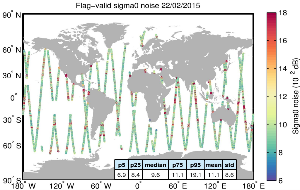
Figure 26. Geographical distribution of flag-valid 20-Hz sigma0 measurement noise over oceans and lakes for 22/02/2015. The statistical values shown in the table refer to the sigma0 noise and are calculated over all measurements shown in the figure.
