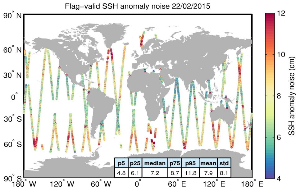
Figure 8. Geographical distribution of flag-valid 20-Hz SSH anomaly measurement noise over oceans and lakes for 22/02/2015. The statistical values shown in the table refer to the SSH anomaly noise and are calculated over all measurements shown in the figure.
