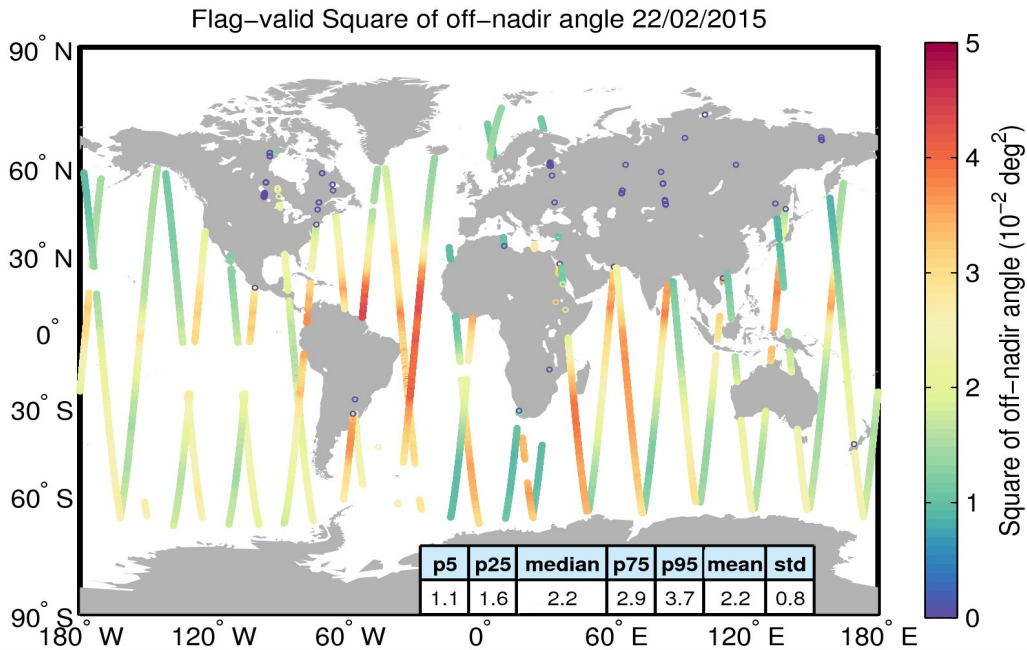
Figure 37. Geographical distribution of flag-valid mispointing data over oceans and lakes for 22/02/2015. The statistical values shown in the table refer to the mispointing in 10^{-2} \text{ deg}^2 and are calculated over all measurements shown in the figure.
