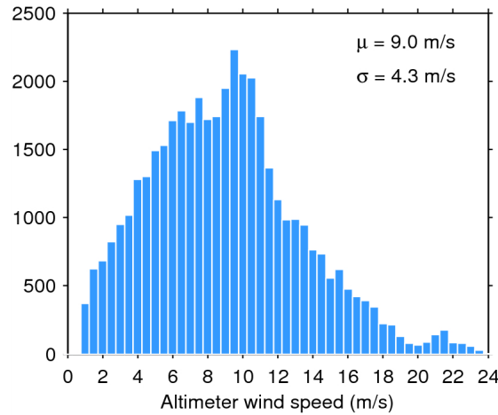
Figure 33. Histogram of flag-valid wind over oceans and lakes for 22/02/2015. The mean ( \mu ) and standard deviation ( \sigma ) are also shown. Note that values larger than 24 m/s are excluded from the histogram for the sake of readability but not from the computation of \mu and \sigma .
