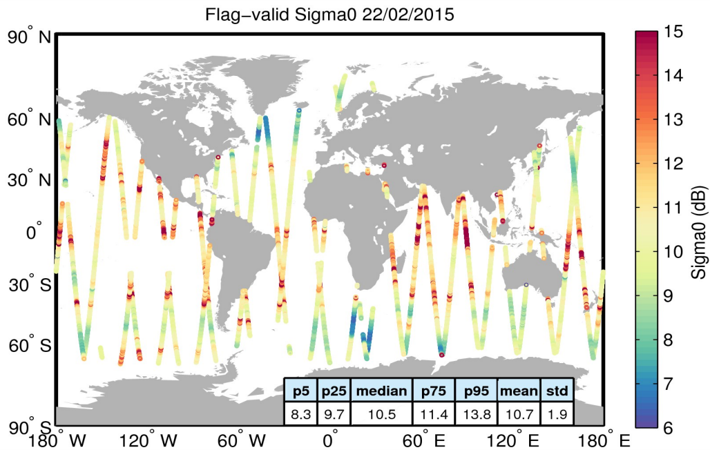
Figure 23. Geographical distribution of flag-valid sigma0 data over oceans and lakes for 22/02/2015. The statistical values shown in the table refer to the sigma0 in dB and are calculated over all measurements shown in the figure.
