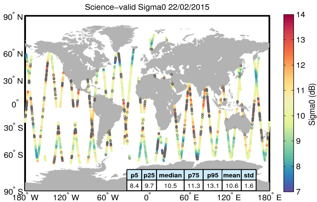
Figure 27. Geographical distribution of science-valid sigma0 data over oceans and lakes for 22/02/2015. The statistical values shown in the table refer to the sigma0 in dB and are calculated over all measurements shown in the figure. Gray circles denote records that have been rejected based on the editing criteria described in Table 4.
