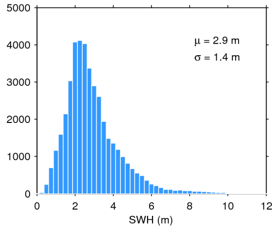
Figure 17. Histogram of flag-valid SWH over oceans and lakes for 22/02/2015. The mean ( \mu ) and standard deviation ( \sigma ) are also shown. Note that values larger than 12 m are excluded from the histogram for the sake of readability but not from the computation of \mu and \sigma .
