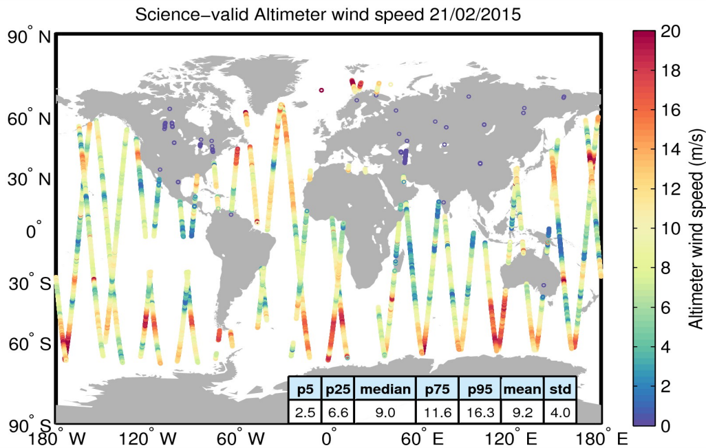
Figure 34. Geographical distribution of science-valid wind data over oceans and lakes for 21/02/2015. The statistical values shown in the table refer to the wind in m/s and are calculated over all measurements shown in the figure. Gray circles denote records that have been rejected based on the editing criteria described in Table 5.
