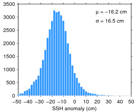
Figure 7. Histogram of flag-valid SSH anomaly over oceans and lakes for 21/02/2015. The mean ( \mu ) and standard deviation ( \sigma ) are also shown. Note that values outside [-50\ 50] cm are excluded from the histogram for the sake of readability but not from the computation of \mu and \sigma .
