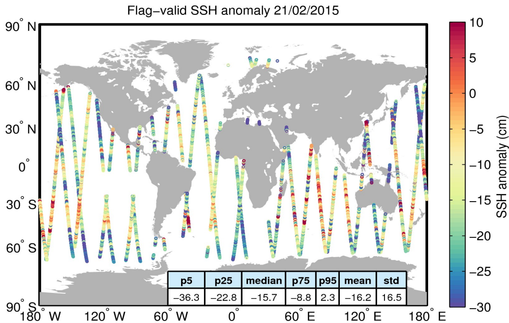
Figure 5. Geographical distribution of flag-valid 1-Hz SSH anomaly data over oceans and lakes for 21/02/2015. The statistical values shown in the table refer to the SSH anomaly in cm and are calculated over all measurements shown in the figure.
