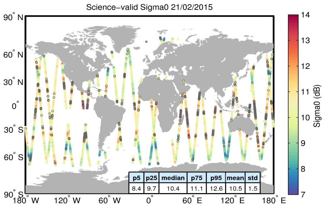
Figure 27. Geographical distribution of science-valid sigma0 data over oceans and lakes for 21/02/2015. The statistical values shown in the table refer to the sigma0 in dB and are calculated over all measurements shown in the figure. Gray circles denote records that have been rejected based on the editing criteria described in Table 4.
