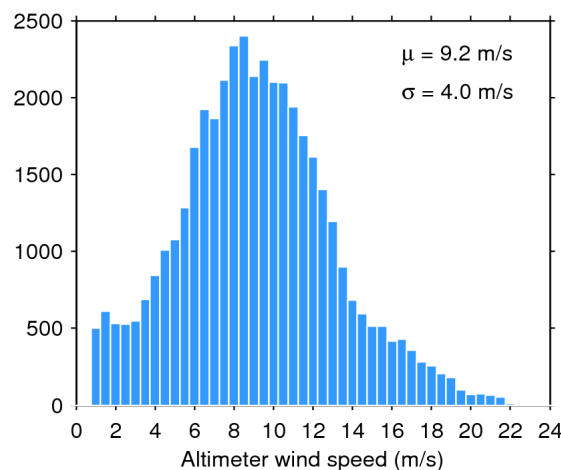
Figure 35. Histogram of science-valid wind over oceans and lakes for 21/02/2015. The mean ( \mu ) and standard deviation ( \sigma ) are also shown. Note that values larger than 24 m/s are excluded from the histogram for the sake of readability but not from the computation of \mu and \sigma .
