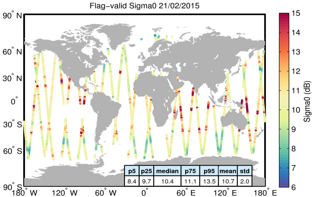
Figure 23. Geographical distribution of flag-valid sigma0 data over oceans and lakes for 21/02/2015. The statistical values shown in the table refer to the sigma0 in dB and are calculated over all measurements shown in the figure.
