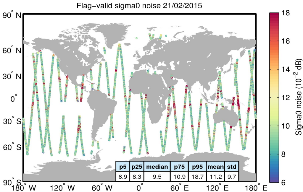
Figure 26. Geographical distribution of flag-valid 20-Hz sigma0 measurement noise over oceans and lakes for 21/02/2015. The statistical values shown in the table refer to the sigma0 noise and are calculated over all measurements shown in the figure.
