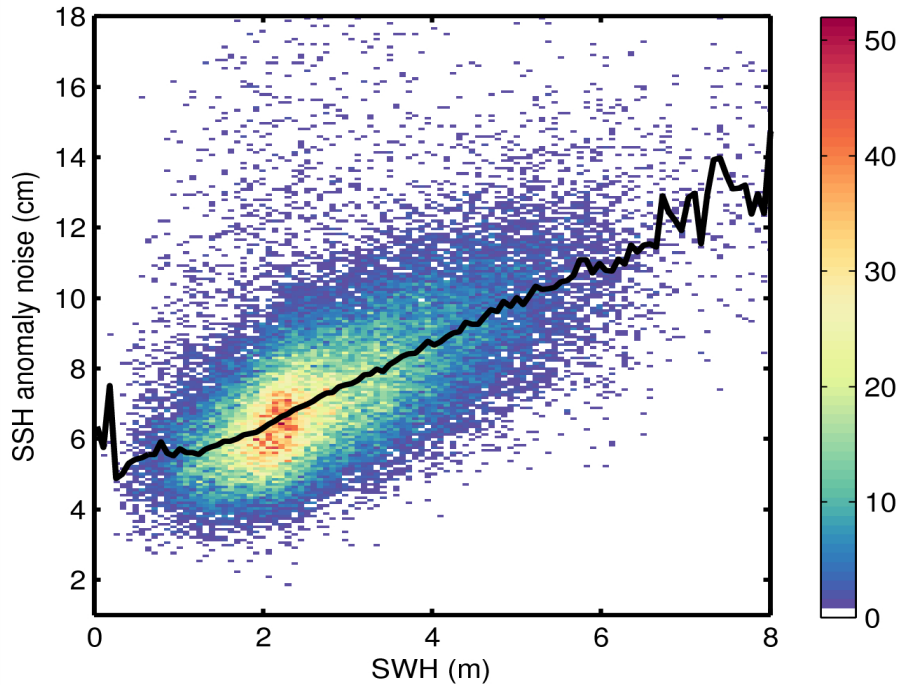
Figure 9. 2D histogram showing flag-valid SSH anomaly noise as a function of SWH for 21/02/2015. The black line denotes the median SSH anomaly as a function of SWH.
