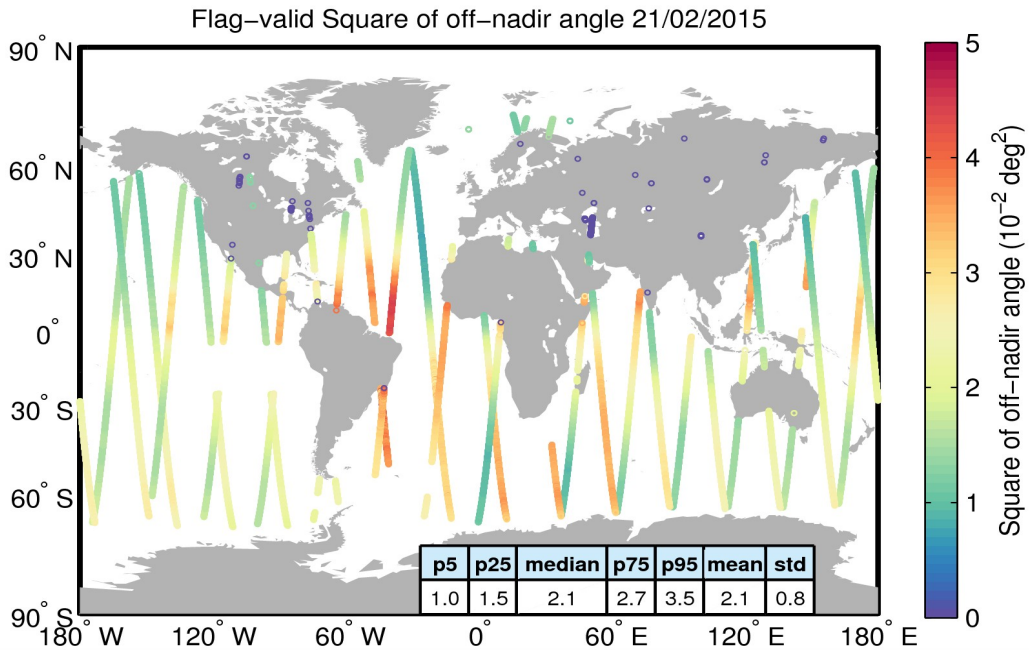
Figure 37. Geographical distribution of flag-valid mispointing data over oceans and lakes for 21/02/2015. The statistical values shown in the table refer to the mispointing in 10^{-2} \text{deg}^2 and are calculated over all measurements shown in the figure.
