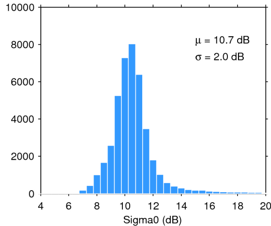
Figure 25. Histogram of flag-valid sigma0 over oceans and lakes for 21/02/2015. The mean ( \mu ) and standard deviation ( \sigma ) are also shown. Note that values outside [4 20] dB are excluded from the histogram for the sake of readability but not from the computation of \mu and \sigma .
