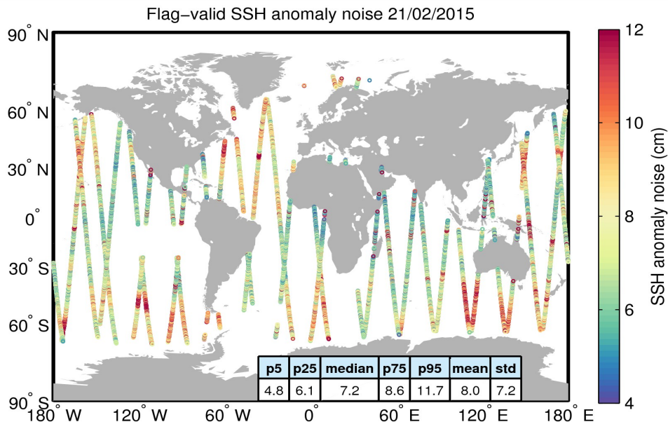
Figure 8. Geographical distribution of flag-valid 20-Hz SSH anomaly measurement noise over oceans and lakes for 21/02/2015. The statistical values shown in the table refer to the SSH anomaly noise and are calculated over all measurements shown in the figure.
