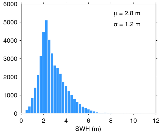
Figure 20. Histogram of science-valid SWH over oceans and lakes for 21/02/2015. The mean ( \mu ) and standard deviation ( \sigma ) are also shown. Note that values larger than 12 m are excluded from the histogram for the sake of readability but not from the computation of \mu and \sigma .
