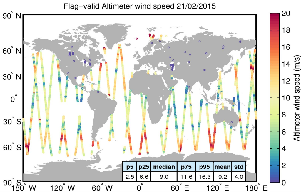
Figure 31. Geographical distribution of flag-valid wind data over oceans and lakes for 21/02/2015. The statistical values shown in the table refer to the wind in m/s and are calculated over all measurements shown in the figure.
