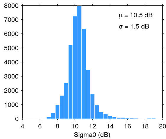
Figure 28. Histogram of science-valid sigma0 over oceans and lakes for 21/02/2015. The mean ( \mu ) and standard deviation ( \sigma ) are also shown. Note that values outside [4 20] dB are excluded from the histogram for the sake of readability but not from the computation of \mu and \sigma .
