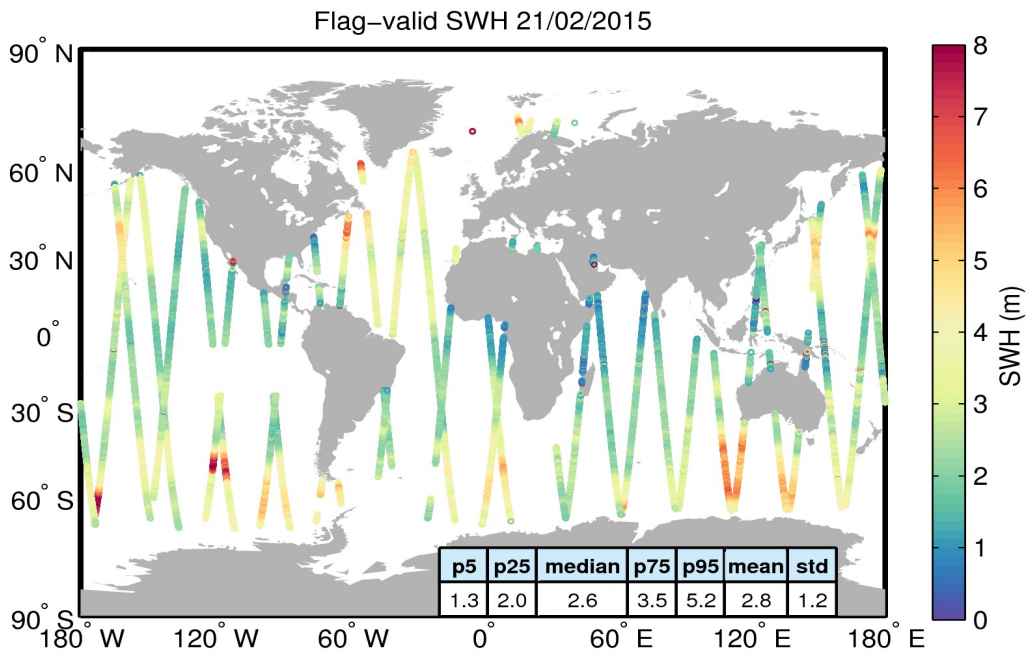
Figure 15. Geographical distribution of flag-valid SWH data over oceans and lakes for 21/02/2015. The statistical values shown in the table refer to the SWH in m and are calculated over all measurements shown in the figure.
