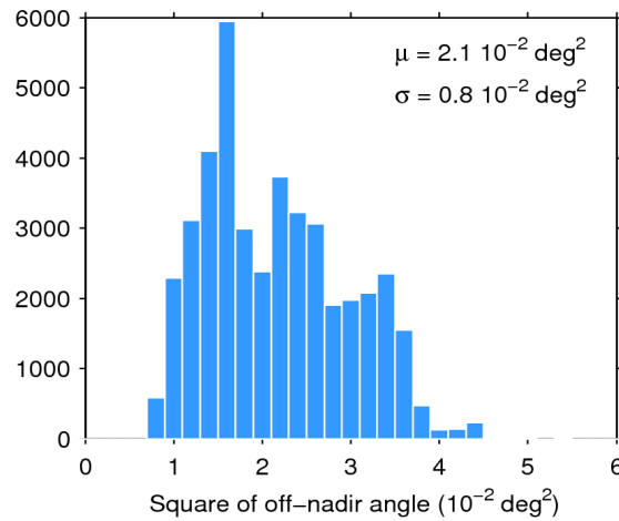
Figure 39. Histogram of flag-valid mispointing over oceans and lakes for 21/02/2015. The mean ( \mu ) and standard deviation ( \sigma ) are also shown. Note that values than 6 \cdot 10^{-2} \text{ deg}^2 are excluded from the histogram for the sake of readability but not from the computation of \mu and \sigma .
