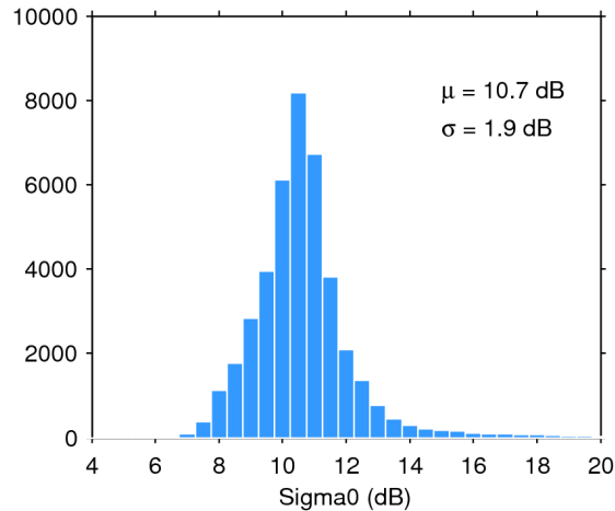
Figure 25. Histogram of flag-valid sigma0 over oceans and lakes for 20/02/2015. The mean ( \mu ) and standard deviation ( \sigma ) are also shown. Note that values outside [4 20] dB are excluded from the histogram for the sake of readability but not from the computation of \mu and \sigma .
