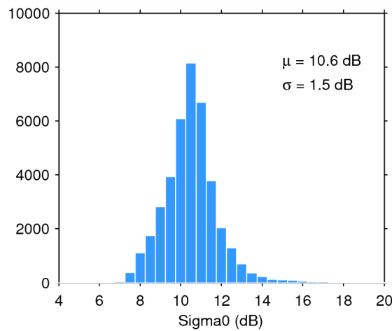
Figure 28. Histogram of science-valid sigma0 over oceans and lakes for 20/02/2015. The mean ( \mu ) and standard deviation ( \sigma ) are also shown. Note that values outside [4 20] dB are excluded from the histogram for the sake of readability but not from the computation of \mu and \sigma .
