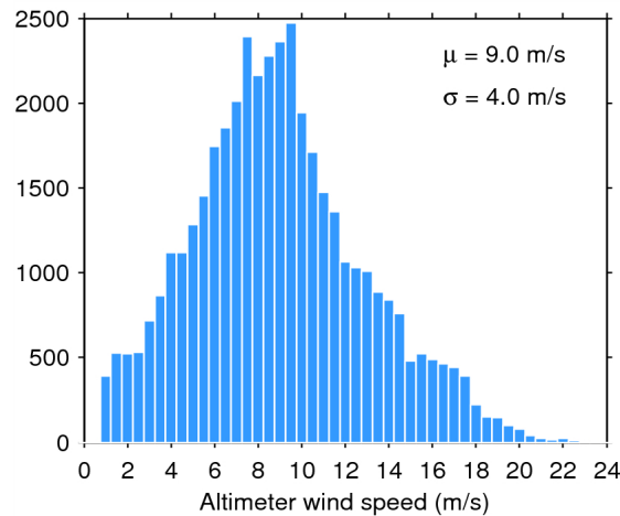
Figure 33. Histogram of flag-valid wind over oceans and lakes for 20/02/2015. The mean ( \mu ) and standard deviation ( \sigma ) are also shown. Note that values larger than 24 m/s are excluded from the histogram for the sake of readability but not from the computation of \mu and \sigma .
