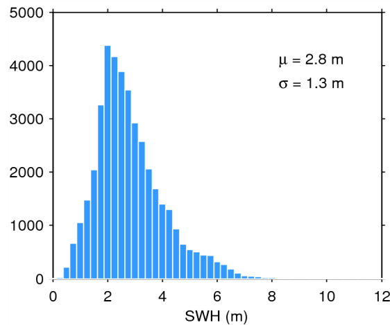
Figure 17. Histogram of flag-valid SWH over oceans and lakes for 20/02/2015. The mean ( \mu ) and standard deviation ( \sigma ) are also shown. Note that values larger than 12 m are excluded from the histogram for the sake of readability but not from the computation of \mu and \sigma .
