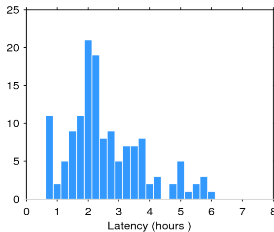
Figure 2. Histogram of the data latency for 20/02/2015. The y-axis denotes the number of files that are made available with a delay of x-hours with respect to the mean time of the records stored in the file.
