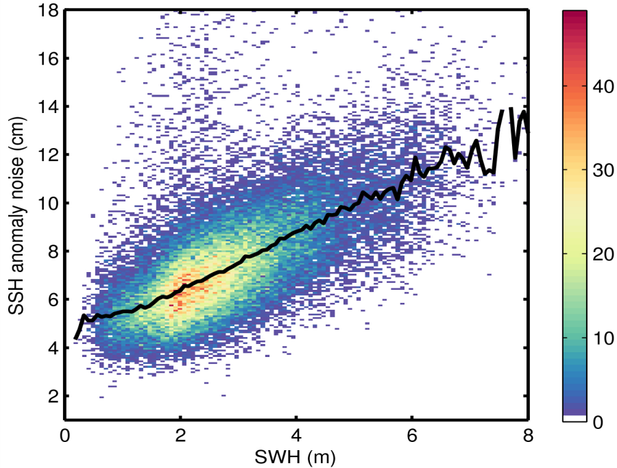
Figure 9. 2D histogram showing flag-valid SSH anomaly noise as a function of SWH for 20/02/2015. The black line denotes the median SSH anomaly as a function of SWH.
