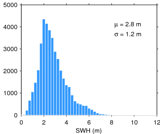
Figure 20. Histogram of science-valid SWH over oceans and lakes for 20/02/2015. The mean ( \mu ) and standard deviation ( \sigma ) are also shown. Note that values larger than 12 m are excluded from the histogram for the sake of readability but not from the computation of \mu and \sigma .
