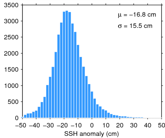
Figure 7. Histogram of flag-valid SSH anomaly over oceans and lakes for 20/02/2015. The mean ( \mu ) and standard deviation ( \sigma ) are also shown. Note that values outside [-50\ 50] cm are excluded from the histogram for the sake of readability but not from the computation of \mu and \sigma .
