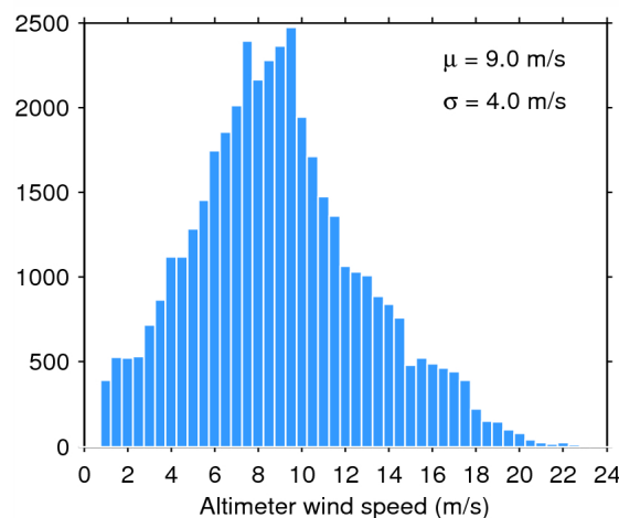
Figure 35. Histogram of science-valid wind over oceans and lakes for 20/02/2015. The mean ( \mu ) and standard deviation ( \sigma ) are also shown. Note that values larger than 24 m/s are excluded from the histogram for the sake of readability but not from the computation of \mu and \sigma .
