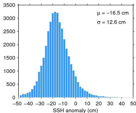
Figure 11. Histogram of science-valid SSH anomaly over oceans and lakes for 20/02/2015. The mean ( \mu ) and standard deviation ( \sigma ) are also shown. Note that values outside [-50 50] cm are excluded from the histogram for the sake of readability but not from the computation of \mu and \sigma .
