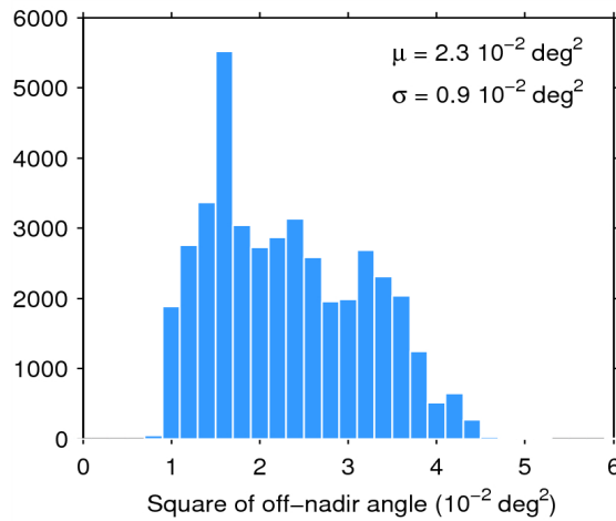
Figure 39. Histogram of flag-valid mispointing over oceans and lakes for 20/02/2015. The mean ( \mu ) and standard deviation ( \sigma ) are also shown. Note that values than 6 \cdot 10^{-2} \text{ deg}^2 are excluded from the histogram for the sake of readability but not from the computation of \mu and \sigma .
