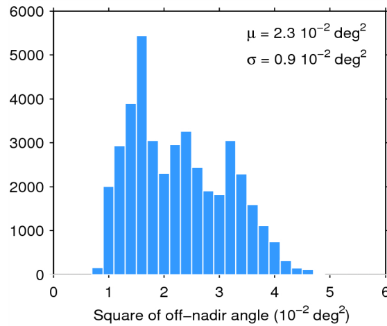
Figure 39. Histogram of flag-valid mispointing over oceans and lakes for 18/02/2015. The mean ( \mu ) and standard deviation ( \sigma ) are also shown. Note that values than 6 \cdot 10^{-2} \text{ deg}^2 are excluded from the histogram for the sake of readability but not from the computation of \mu and \sigma .
