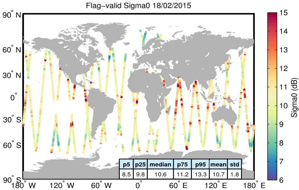
Figure 23. Geographical distribution of flag-valid sigma0 data over oceans and lakes for 18/02/2015. The statistical values shown in the table refer to the sigma0 in dB and are calculated over all measurements shown in the figure.
