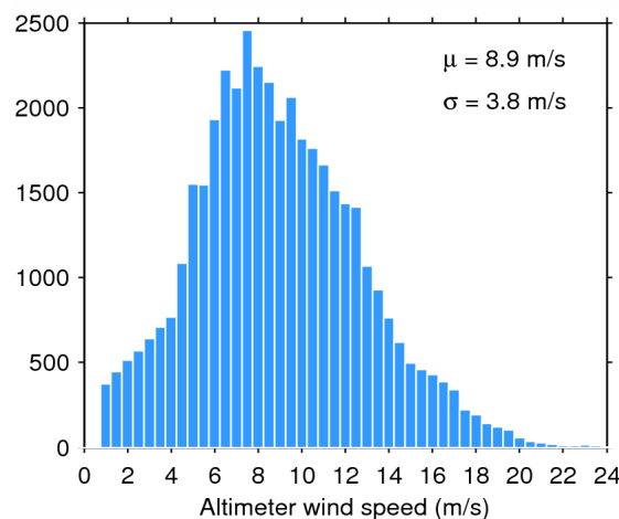
Figure 35. Histogram of science-valid wind over oceans and lakes for 18/02/2015. The mean ( \mu ) and standard deviation ( \sigma ) are also shown. Note that values larger than 24 m/s are excluded from the histogram for the sake of readability but not from the computation of \mu and \sigma .
