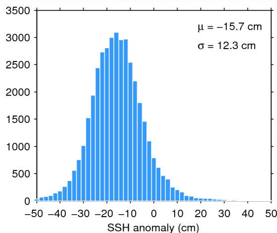
Figure 11. Histogram of science-valid SSH anomaly over oceans and lakes for 18/02/2015. The mean ( \mu ) and standard deviation ( \sigma ) are also shown. Note that values outside [-50 50] cm are excluded from the histogram for the sake of readability but not from the computation of \mu and \sigma .
