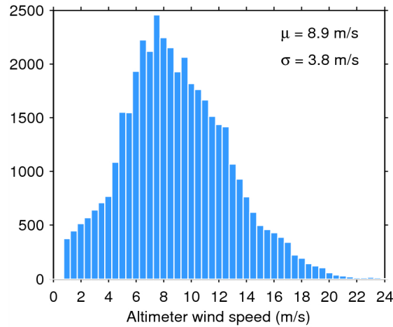
Figure 33. Histogram of flag-valid wind over oceans and lakes for 18/02/2015. The mean ( \mu ) and standard deviation ( \sigma ) are also shown. Note that values larger than 24 m/s are excluded from the histogram for the sake of readability but not from the computation of \mu and \sigma .
