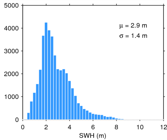
Figure 17. Histogram of flag-valid SWH over oceans and lakes for 18/02/2015. The mean ( \mu ) and standard deviation ( \sigma ) are also shown. Note that values larger than 12 m are excluded from the histogram for the sake of readability but not from the computation of \mu and \sigma .
