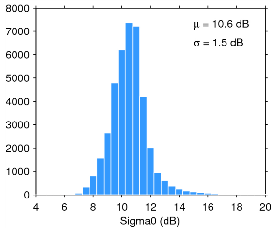
Figure 28. Histogram of science-valid sigma0 over oceans and lakes for 18/02/2015. The mean ( \mu ) and standard deviation ( \sigma ) are also shown. Note that values outside [4 20] dB are excluded from the histogram for the sake of readability but not from the computation of \mu and \sigma .
