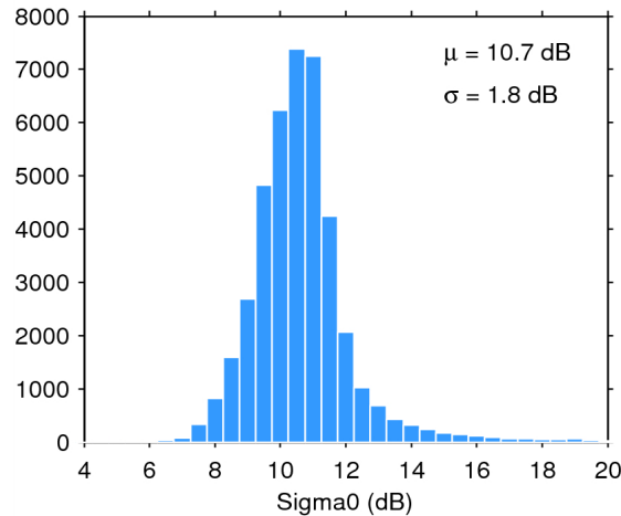
Figure 25. Histogram of flag-valid sigma0 over oceans and lakes for 18/02/2015. The mean ( \mu ) and standard deviation ( \sigma ) are also shown. Note that values outside [4 20] dB are excluded from the histogram for the sake of readability but not from the computation of \mu and \sigma .
