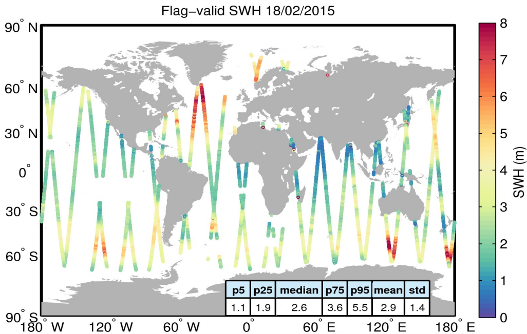
Figure 15. Geographical distribution of flag-valid SWH data over oceans and lakes for 18/02/2015. The statistical values shown in the table refer to the SWH in m and are calculated over all measurements shown in the figure.
