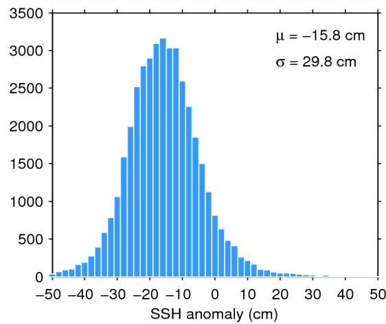
Figure 7. Histogram of flag-valid SSH anomaly over oceans and lakes for 18/02/2015. The mean ( \mu ) and standard deviation ( \sigma ) are also shown. Note that values outside [-50\ 50] cm are excluded from the histogram for the sake of readability but not from the computation of \mu and \sigma .
