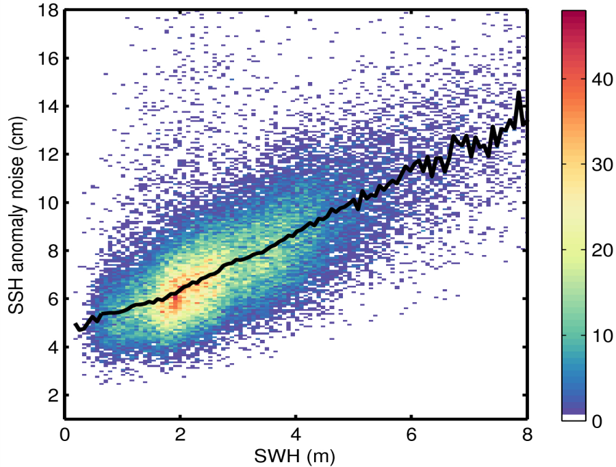
Figure 9. 2D histogram showing flag-valid SSH anomaly noise as a function of SWH for 18/02/2015. The black line denotes the median SSH anomaly as a function of SWH.
