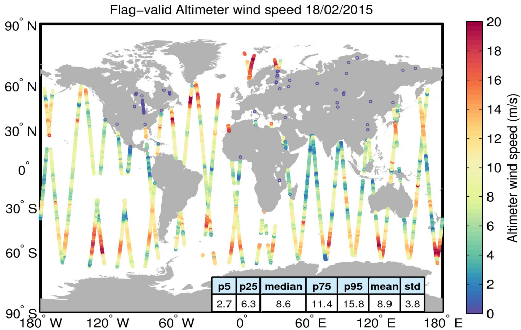
Figure 31. Geographical distribution of flag-valid wind data over oceans and lakes for 18/02/2015. The statistical values shown in the table refer to the wind in m/s and are calculated over all measurements shown in the figure.
