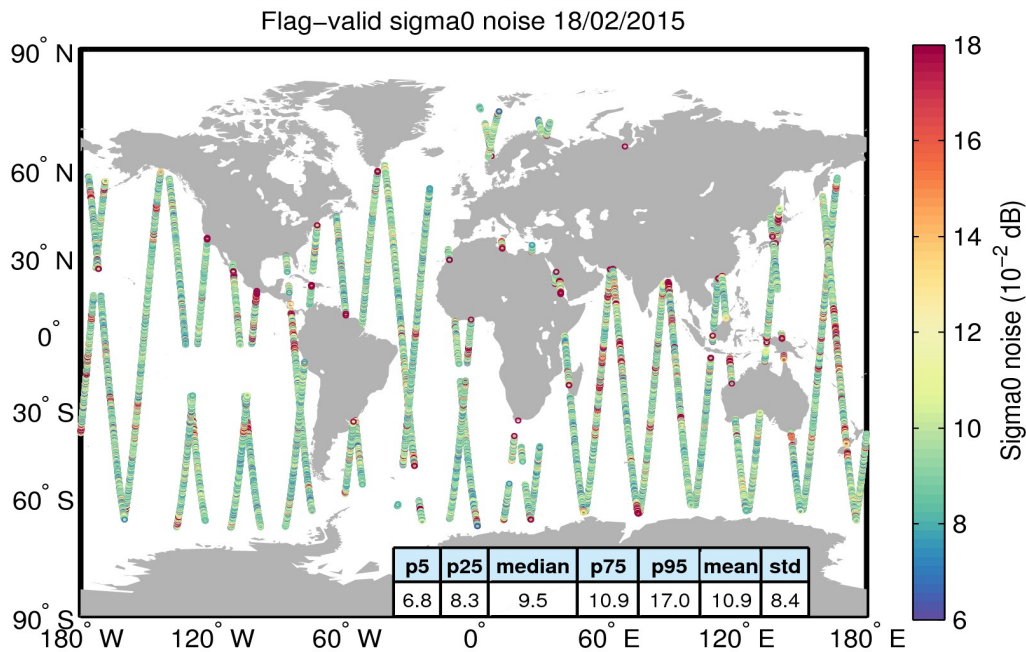
Figure 26. Geographical distribution of flag-valid 20-Hz sigma0 measurement noise over oceans and lakes for 18/02/2015. The statistical values shown in the table refer to the sigma0 noise and are calculated over all measurements shown in the figure.
