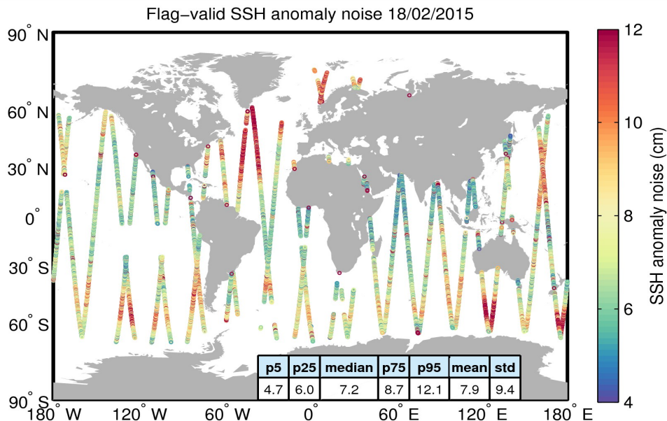
Figure 8. Geographical distribution of flag-valid 20-Hz SSH anomaly measurement noise over oceans and lakes for 18/02/2015. The statistical values shown in the table refer to the SSH anomaly noise and are calculated over all measurements shown in the figure.
