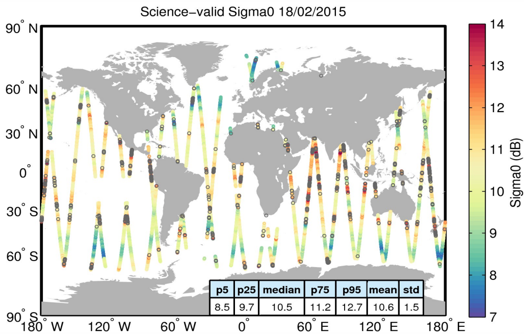
Figure 27. Geographical distribution of science-valid sigma0 data over oceans and lakes for 18/02/2015. The statistical values shown in the table refer to the sigma0 in dB and are calculated over all measurements shown in the figure. Gray circles denote records that have been rejected based on the editing criteria described in Table 4.
