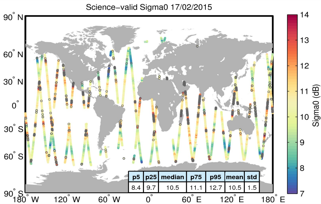
Figure 27. Geographical distribution of science-valid sigma0 data over oceans and lakes for 17/02/2015. The statistical values shown in the table refer to the sigma0 in dB and are calculated over all measurements shown in the figure. Gray circles denote records that have been rejected based on the editing criteria described in Table 4.
