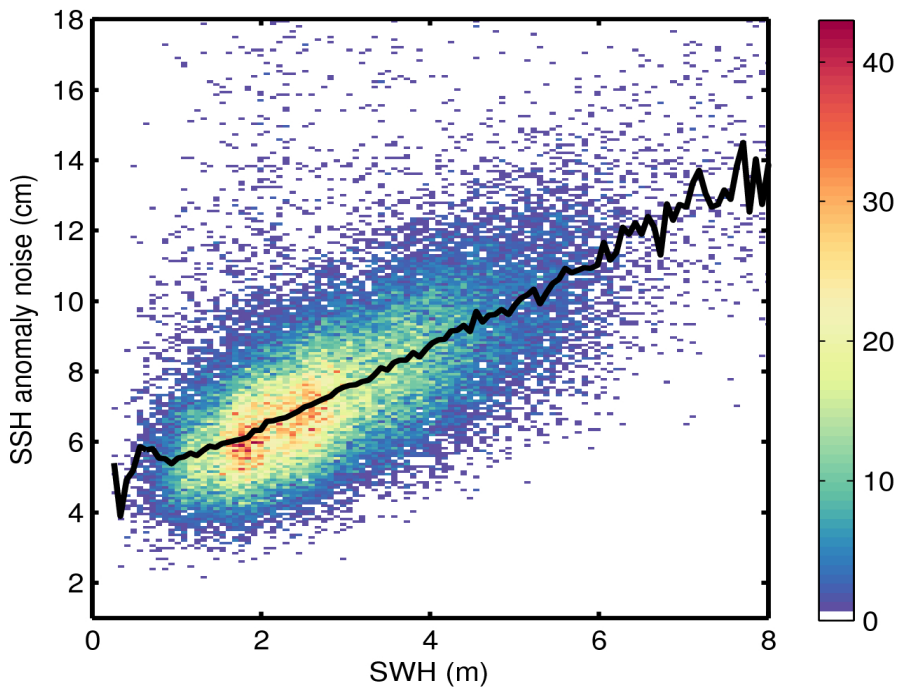
Figure 9. 2D histogram showing flag-valid SSH anomaly noise as a function of SWH for 17/02/2015. The black line denotes the median SSH anomaly as a function of SWH.
