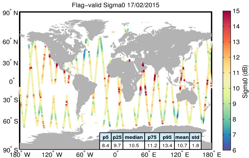
Figure 23. Geographical distribution of flag-valid sigma0 data over oceans and lakes for 17/02/2015. The statistical values shown in the table refer to the sigma0 in dB and are calculated over all measurements shown in the figure.
