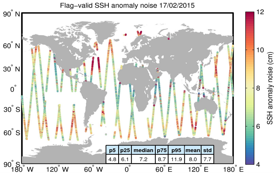
Figure 8. Geographical distribution of flag-valid 20-Hz SSH anomaly measurement noise over oceans and lakes for 17/02/2015. The statistical values shown in the table refer to the SSH anomaly noise and are calculated over all measurements shown in the figure.
