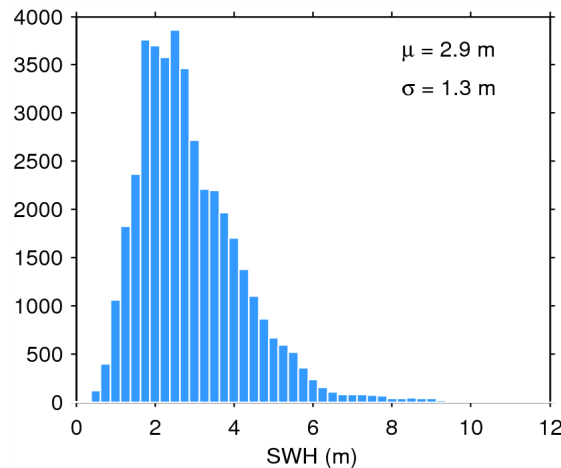
Figure 20. Histogram of science-valid SWH over oceans and lakes for 17/02/2015. The mean ( \mu ) and standard deviation ( \sigma ) are also shown. Note that values larger than 12 m are excluded from the histogram for the sake of readability but not from the computation of \mu and \sigma .
