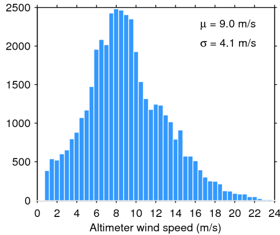
Figure 33. Histogram of flag-valid wind over oceans and lakes for 17/02/2015. The mean ( \mu ) and standard deviation ( \sigma ) are also shown. Note that values larger than 24 m/s are excluded from the histogram for the sake of readability but not from the computation of \mu and \sigma .
