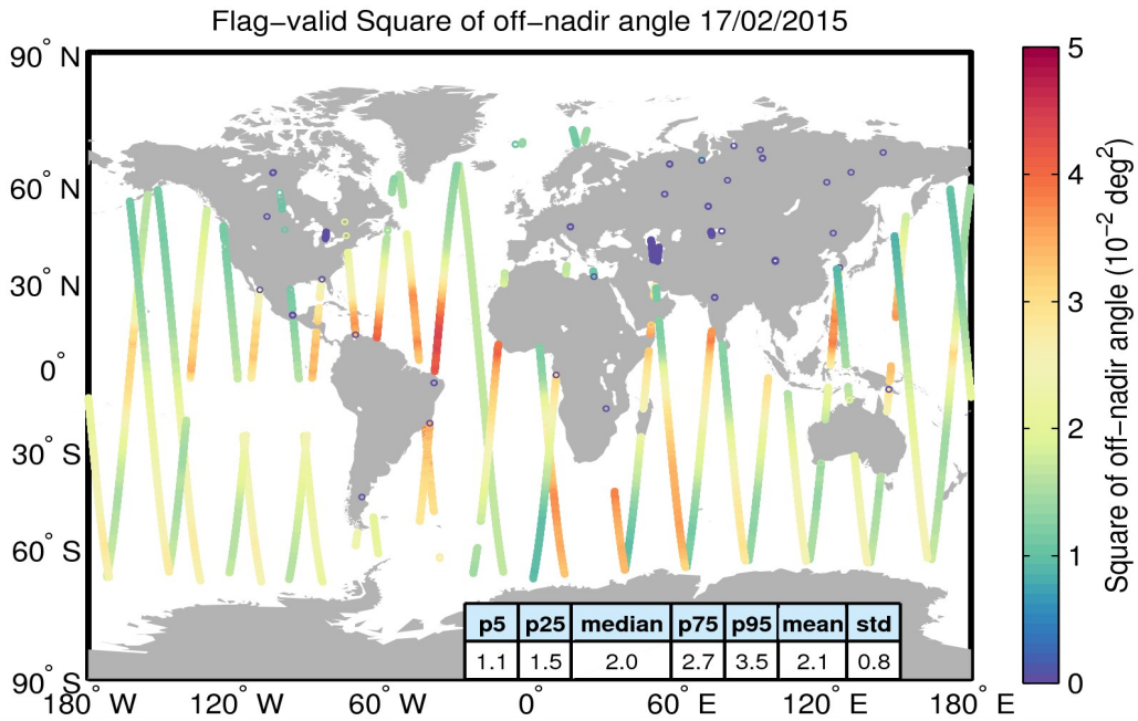
Figure 37. Geographical distribution of flag-valid mispointing data over oceans and lakes for 17/02/2015. The statistical values shown in the table refer to the mispointing in 10^{-2} \text{ deg}^2 and are calculated over all measurements shown in the figure.
