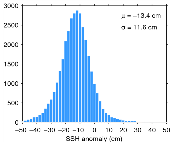
Figure 11. Histogram of science-valid SSH anomaly over oceans and lakes for 17/02/2015. The mean ( \mu ) and standard deviation ( \sigma ) are also shown. Note that values outside [-50 50] cm are excluded from the histogram for the sake of readability but not from the computation of \mu and \sigma .
