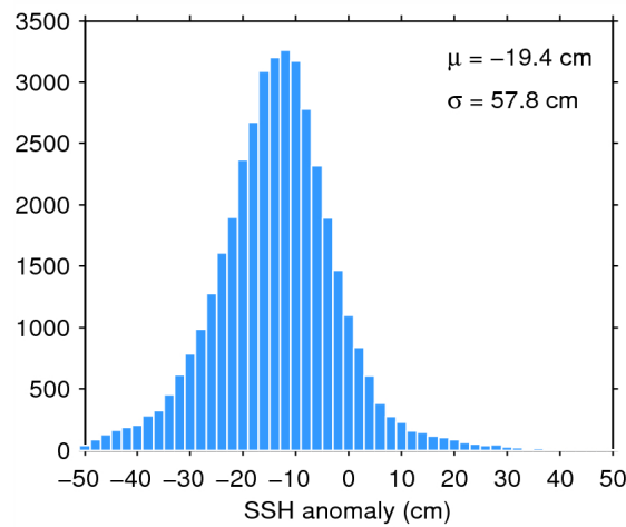
Figure 7. Histogram of flag-valid SSH anomaly over oceans and lakes for 17/02/2015. The mean ( \mu ) and standard deviation ( \sigma ) are also shown. Note that values outside [-50 50] cm are excluded from the histogram for the sake of readability but not from the computation of \mu and \sigma .
