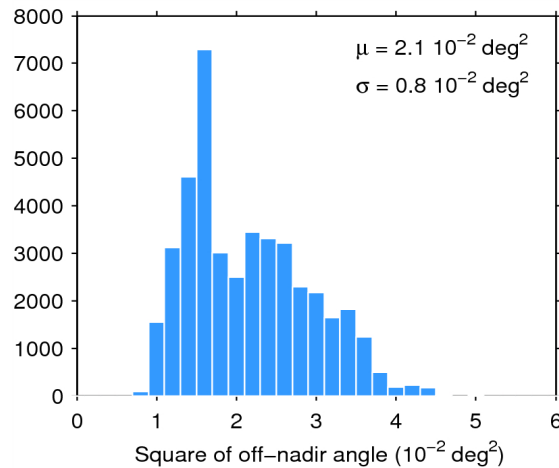
Figure 39. Histogram of flag-valid mispointing over oceans and lakes for 17/02/2015. The mean ( \mu ) and standard deviation ( \sigma ) are also shown. Note that values than 6 \cdot 10^{-2} \text{ deg}^2 are excluded from the histogram for the sake of readability but not from the computation of \mu and \sigma .
