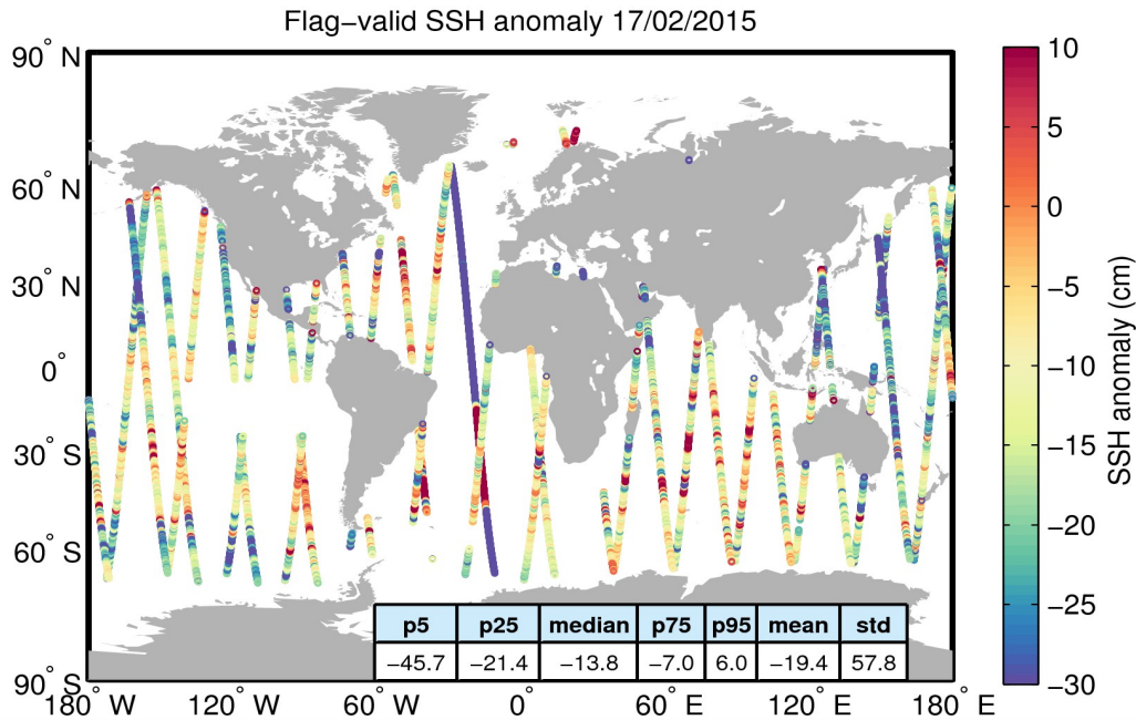
Figure 5. Geographical distribution of flag-valid 1-Hz SSH anomaly data over oceans and lakes for 17/02/2015. The statistical values shown in the table refer to the SSH anomaly in cm and are calculated over all measurements shown in the figure.
