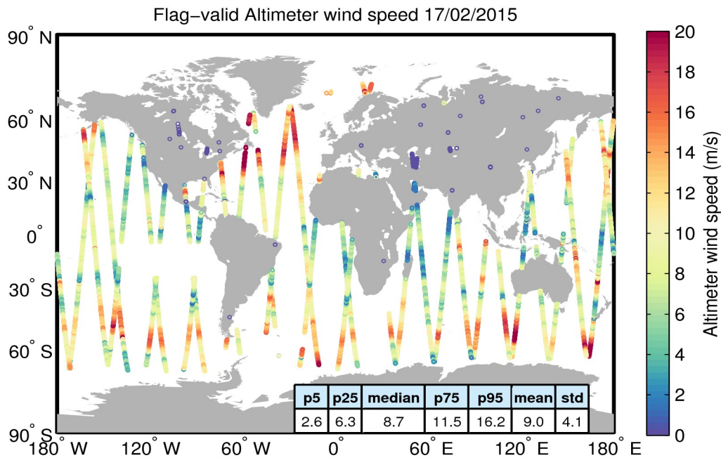
Figure 31. Geographical distribution of flag-valid wind data over oceans and lakes for 17/02/2015. The statistical values shown in the table refer to the wind in m/s and are calculated over all measurements shown in the figure.
