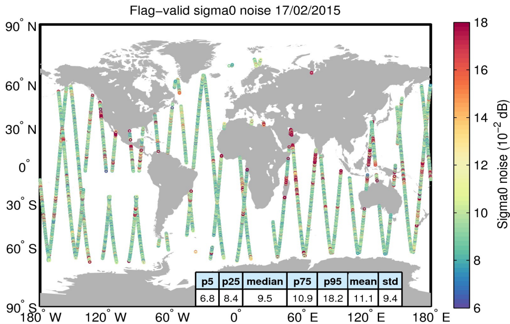
Figure 26. Geographical distribution of flag-valid 20-Hz sigma0 measurement noise over oceans and lakes for 17/02/2015. The statistical values shown in the table refer to the sigma0 noise and are calculated over all measurements shown in the figure.
