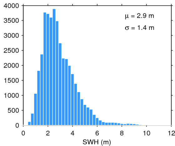
Figure 17. Histogram of flag-valid SWH over oceans and lakes for 17/02/2015. The mean ( \mu ) and standard deviation ( \sigma ) are also shown. Note that values larger than 12 m are excluded from the histogram for the sake of readability but not from the computation of \mu and \sigma .
