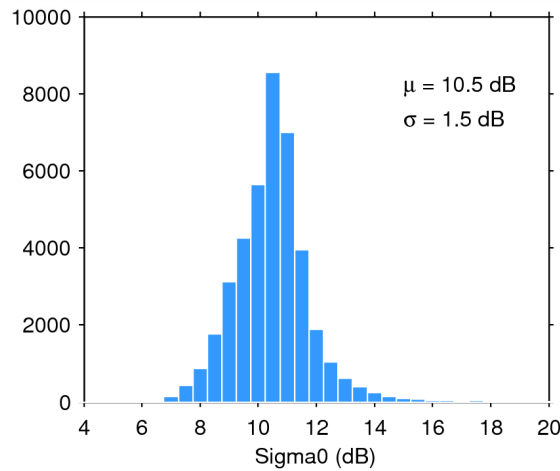
Figure 28. Histogram of science-valid sigma0 over oceans and lakes for 17/02/2015. The mean ( \mu ) and standard deviation ( \sigma ) are also shown. Note that values outside [4 20] dB are excluded from the histogram for the sake of readability but not from the computation of \mu and \sigma .
