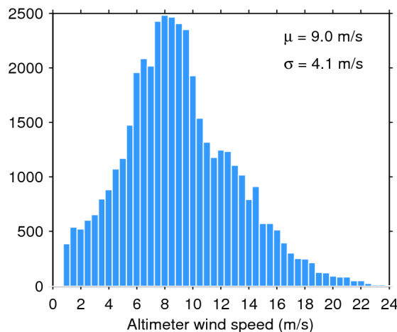
Figure 35. Histogram of science-valid wind over oceans and lakes for 17/02/2015. The mean ( \mu ) and standard deviation ( \sigma ) are also shown. Note that values larger than 24 m/s are excluded from the histogram for the sake of readability but not from the computation of \mu and \sigma .
