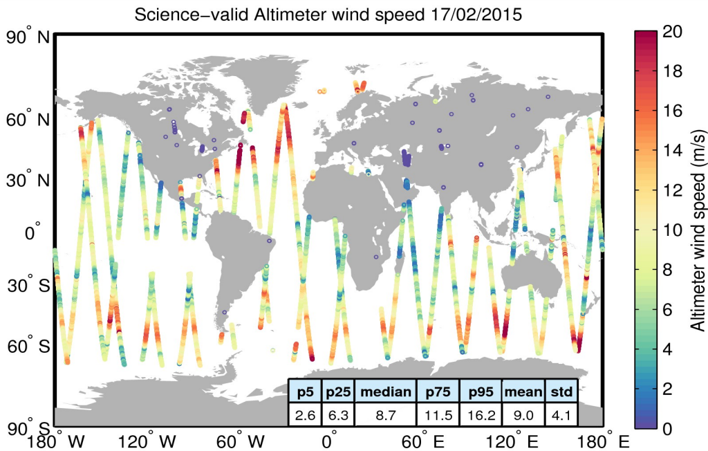
Figure 34. Geographical distribution of science-valid wind data over oceans and lakes for 17/02/2015. The statistical values shown in the table refer to the wind in m/s and are calculated over all measurements shown in the figure. Gray circles denote records that have been rejected based on the editing criteria described in Table 5.
