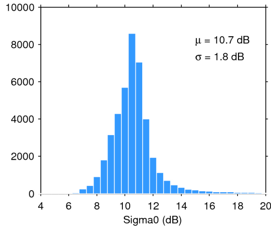
Figure 25. Histogram of flag-valid sigma0 over oceans and lakes for 17/02/2015. The mean ( \mu ) and standard deviation ( \sigma ) are also shown. Note that values outside [4 20] dB are excluded from the histogram for the sake of readability but not from the computation of \mu and \sigma .
