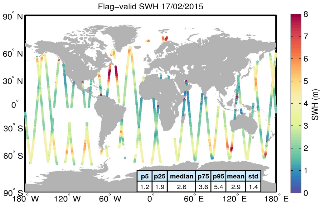
Figure 15. Geographical distribution of flag-valid SWH data over oceans and lakes for 17/02/2015. The statistical values shown in the table refer to the SWH in m and are calculated over all measurements shown in the figure.
