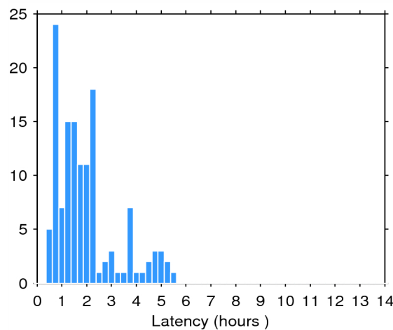
Figure 2. Histogram of the data latency for 17/02/2015. The y-axis denotes the number of files that are made available with a delay of x-hours with respect to the mean time of the records stored in the file.
