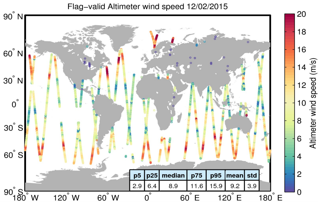
Figure 31. Geographical distribution of flag-valid wind data over oceans and lakes for 12/02/2015. The statistical values shown in the table refer to the wind in m/s and are calculated over all measurements shown in the figure.
