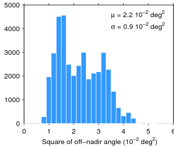
Figure 39. Histogram of flag-valid mispointing over oceans and lakes for 12/02/2015. The mean ( \mu ) and standard deviation ( \sigma ) are also shown. Note that values than 6 \cdot 10^{-2} \text{ deg}^2 are excluded from the histogram for the sake of readability but not from the computation of \mu and \sigma .
