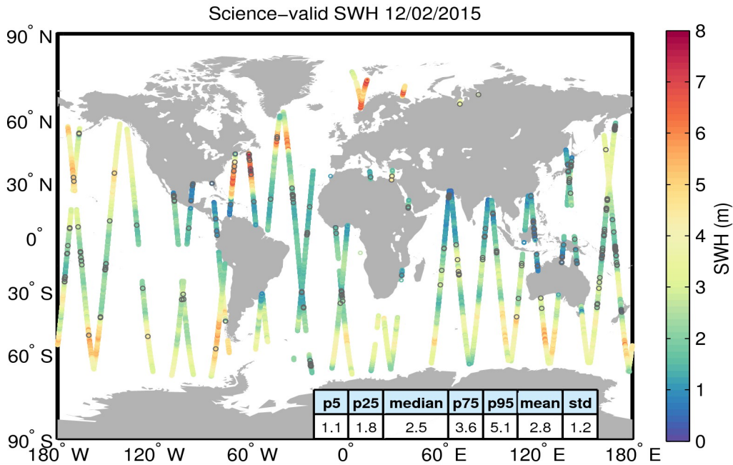
Figure 19. Geographical distribution of science-valid SWH data over oceans and lakes for 12/02/2015. The statistical values shown in the table refer to the SWH in m and are calculated over all measurements shown in the figure. Gray circles denote records that have been rejected based on the editing criteria described in Table 3.
