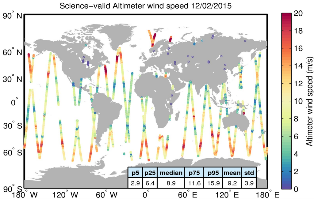
Figure 34. Geographical distribution of science-valid wind data over oceans and lakes for 12/02/2015. The statistical values shown in the table refer to the wind in m/s and are calculated over all measurements shown in the figure. Gray circles denote records that have been rejected based on the editing criteria described in Table 5.
