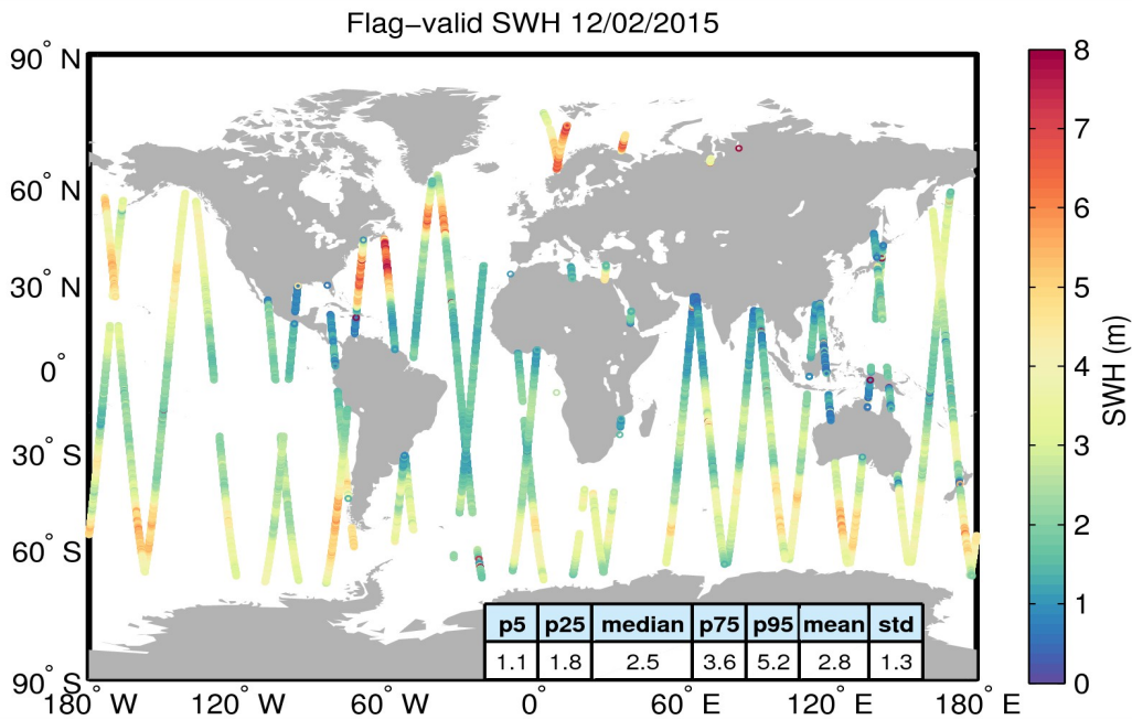
Figure 15. Geographical distribution of flag-valid SWH data over oceans and lakes for 12/02/2015. The statistical values shown in the table refer to the SWH in m and are calculated over all measurements shown in the figure.
