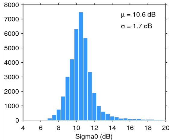
Figure 25. Histogram of flag-valid sigma0 over oceans and lakes for 12/02/2015. The mean ( \mu ) and standard deviation ( \sigma ) are also shown. Note that values outside [4 20] dB are excluded from the histogram for the sake of readability but not from the computation of \mu and \sigma .
