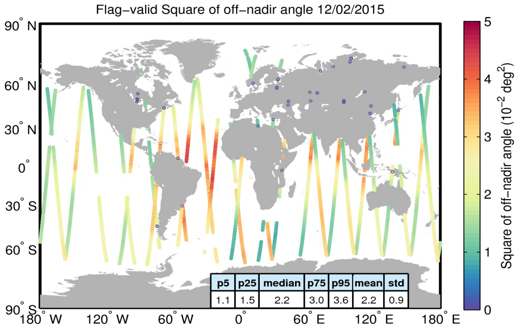
Figure 37. Geographical distribution of flag-valid mispointing data over oceans and lakes for 12/02/2015. The statistical values shown in the table refer to the mispointing in 10^{-2} \text{ deg}^2 and are calculated over all measurements shown in the figure.
