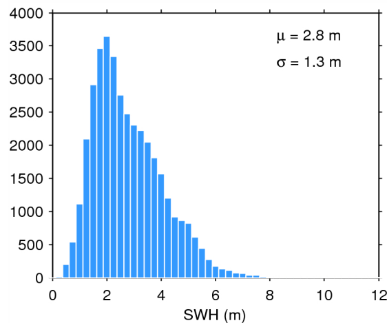
Figure 17. Histogram of flag-valid SWH over oceans and lakes for 12/02/2015. The mean ( \mu ) and standard deviation ( \sigma ) are also shown. Note that values larger than 12 m are excluded from the histogram for the sake of readability but not from the computation of \mu and \sigma .
