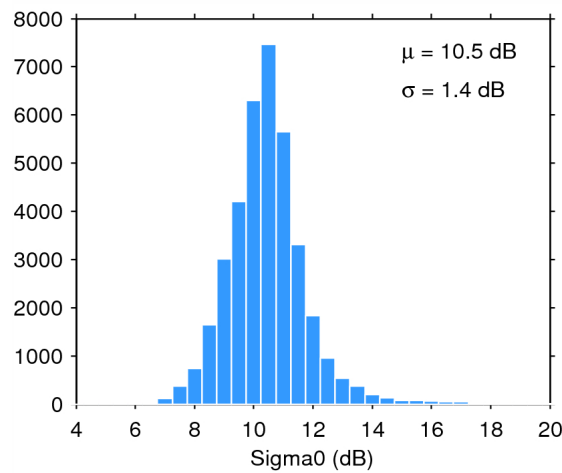
Figure 28. Histogram of science-valid sigma0 over oceans and lakes for 12/02/2015. The mean ( \mu ) and standard deviation ( \sigma ) are also shown. Note that values outside [4 20] dB are excluded from the histogram for the sake of readability but not from the computation of \mu and \sigma .
