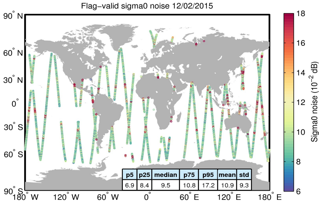
Figure 26. Geographical distribution of flag-valid 20-Hz sigma0 measurement noise over oceans and lakes for 12/02/2015. The statistical values shown in the table refer to the sigma0 noise and are calculated over all measurements shown in the figure.
