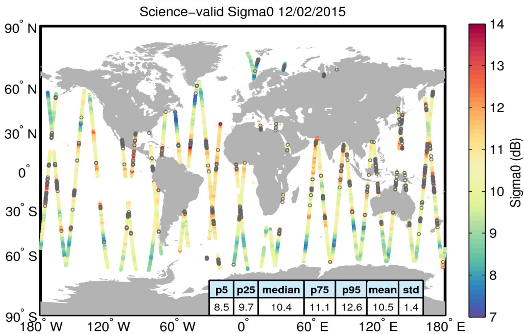
Figure 27. Geographical distribution of science-valid sigma0 data over oceans and lakes for 12/02/2015. The statistical values shown in the table refer to the sigma0 in dB and are calculated over all measurements shown in the figure. Gray circles denote records that have been rejected based on the editing criteria described in Table 4.
