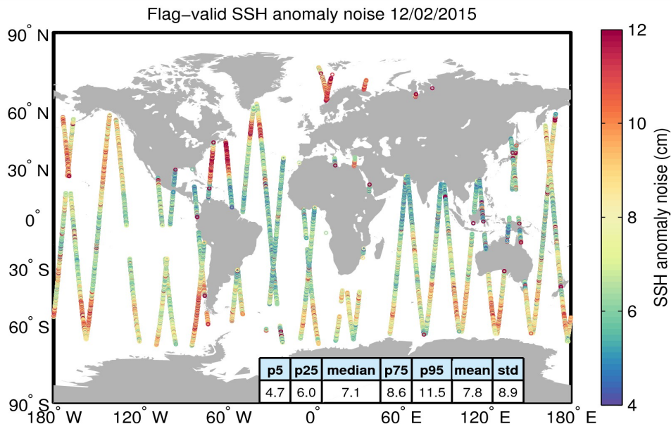
Figure 8. Geographical distribution of flag-valid 20-Hz SSH anomaly measurement noise over oceans and lakes for 12/02/2015. The statistical values shown in the table refer to the SSH anomaly noise and are calculated over all measurements shown in the figure.
