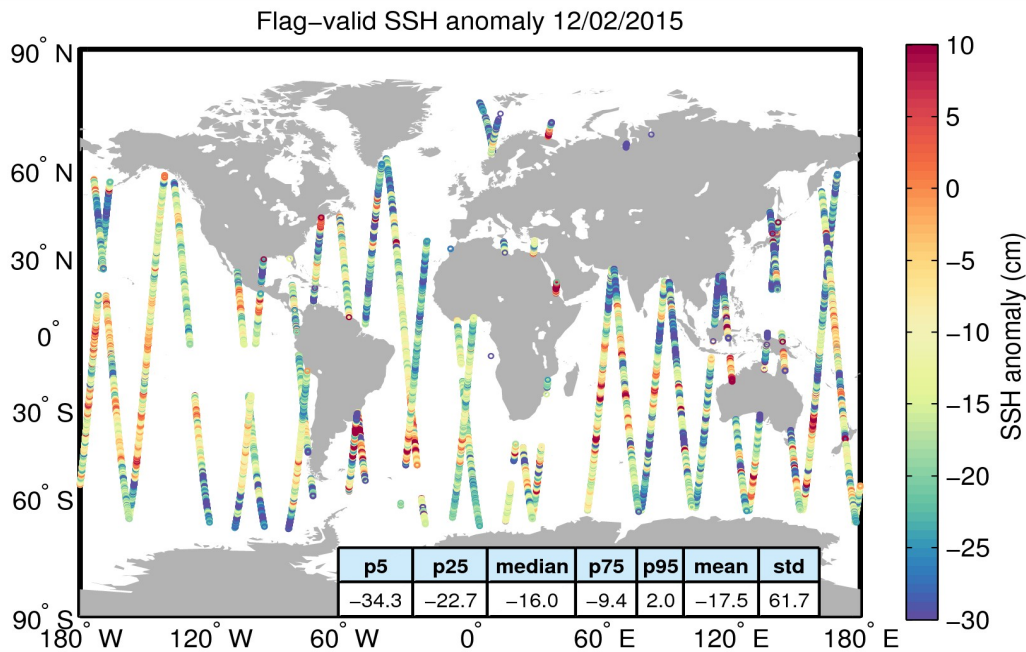
Figure 5. Geographical distribution of flag-valid 1-Hz SSH anomaly data over oceans and lakes for 12/02/2015. The statistical values shown in the table refer to the SSH anomaly in cm and are calculated over all measurements shown in the figure.
