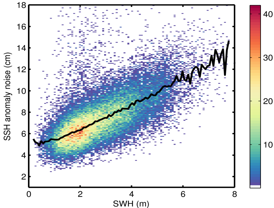
Figure 9. 2D histogram showing flag-valid SSH anomaly noise as a function of SWH for 12/02/2015. The black line denotes the median SSH anomaly as a function of SWH.
