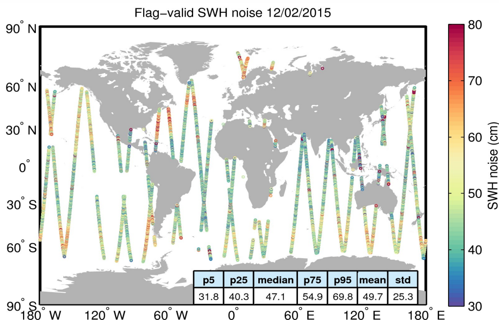
Figure 18. Geographical distribution of flag-valid 20-Hz SWH measurement noise over oceans and lakes for 12/02/2015. The statistical values shown in the figure refer to the SWH noise and are calculated over all measurements shown in the figure.
