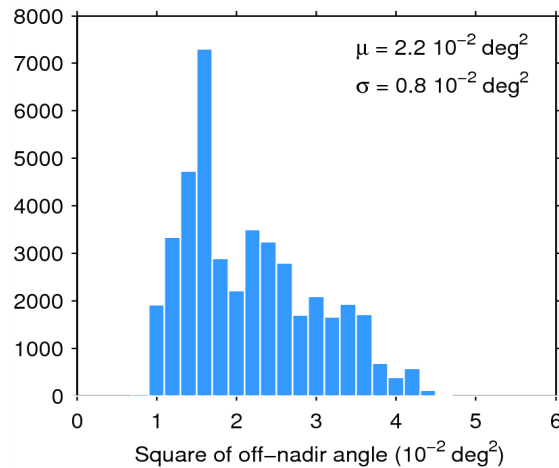
Figure 39. Histogram of flag-valid mispointing over oceans and lakes for 11/02/2015. The mean ( \mu ) and standard deviation ( \sigma ) are also shown. Note that values than 6 \cdot 10^{-2} \text{ deg}^2 are excluded from the histogram for the sake of readability but not from the computation of \mu and \sigma .
