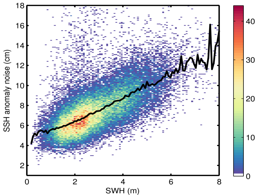
Figure 9. 2D histogram showing flag-valid SSH anomaly noise as a function of SWH for 11/02/2015. The black line denotes the median SSH anomaly as a function of SWH.
