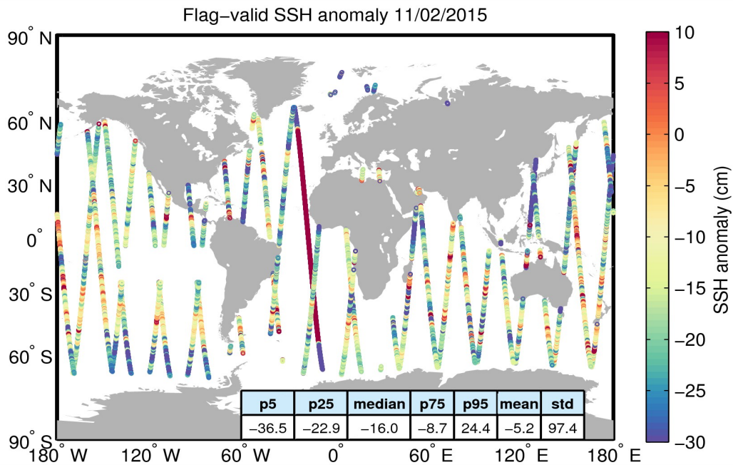
Figure 5. Geographical distribution of flag-valid 1-Hz SSH anomaly data over oceans and lakes for 11/02/2015. The statistical values shown in the table refer to the SSH anomaly in cm and are calculated over all measurements shown in the figure.
