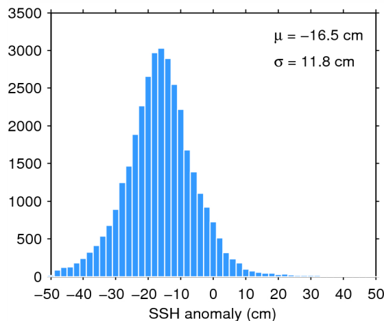
Figure 11. Histogram of science-valid SSH anomaly over oceans and lakes for 11/02/2015. The mean ( \mu ) and standard deviation ( \sigma ) are also shown. Note that values outside [-50 50] cm are excluded from the histogram for the sake of readability but not from the computation of \mu and \sigma .
