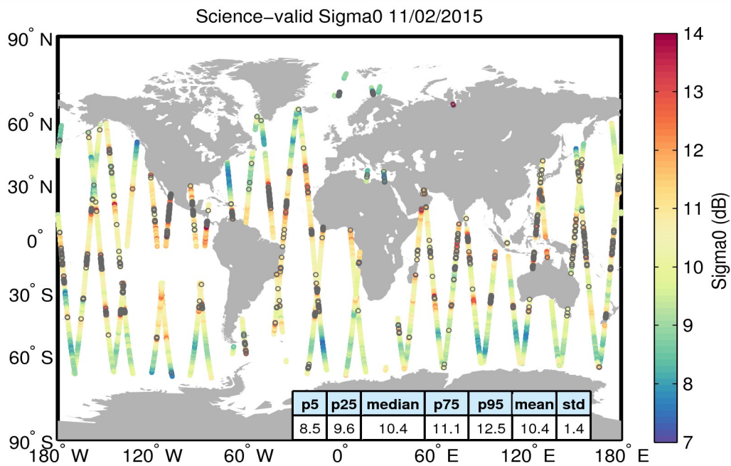
Figure 27. Geographical distribution of science-valid sigma0 data over oceans and lakes for 11/02/2015. The statistical values shown in the table refer to the sigma0 in dB and are calculated over all measurements shown in the figure. Gray circles denote records that have been rejected based on the editing criteria described in Table 4.
