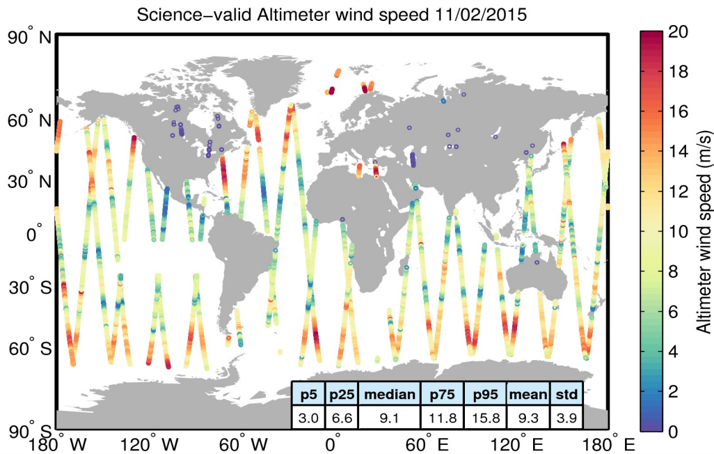
Figure 34. Geographical distribution of science-valid wind data over oceans and lakes for 11/02/2015. The statistical values shown in the table refer to the wind in m/s and are calculated over all measurements shown in the figure. Gray circles denote records that have been rejected based on the editing criteria described in Table 5.
