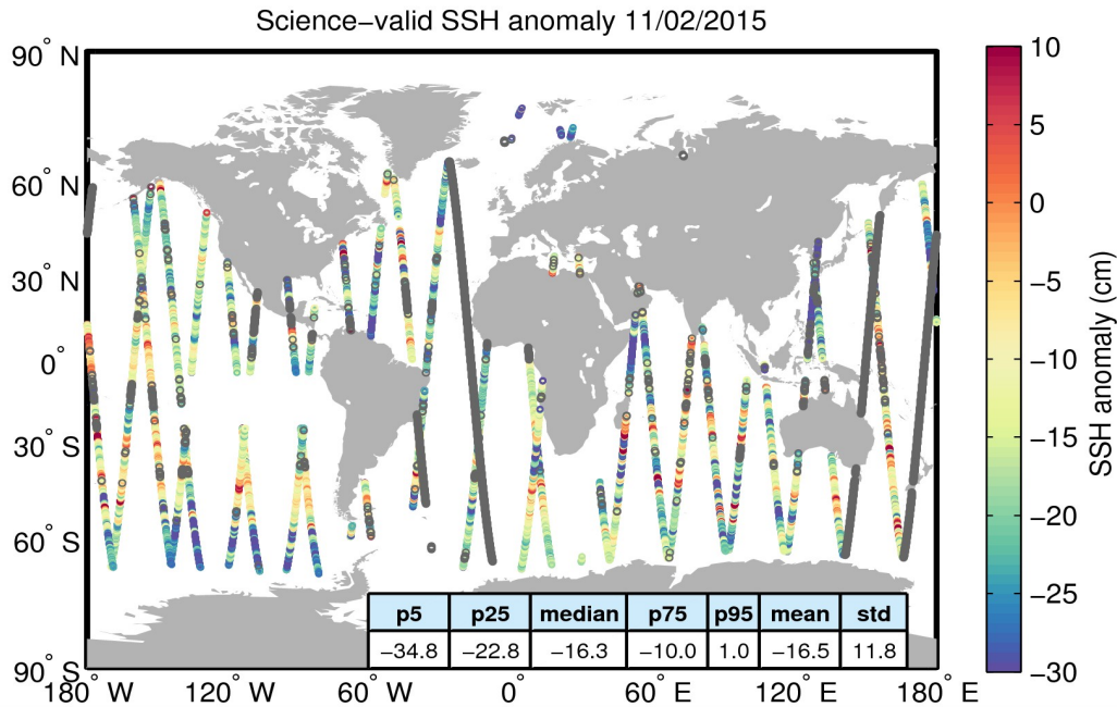
Figure 10. Geographical distribution of science-valid SSH anomaly data over oceans and lakes for 11/02/2015. The statistical values shown in the table refer to the SSH anomaly in cm and are calculated over all measurements shown in the figure. Gray circles denote records that have been rejected based on the editing criteria described in Table 2.
