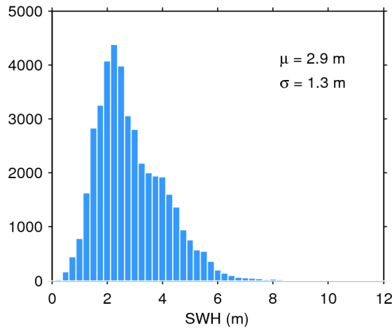
Figure 17. Histogram of flag-valid SWH over oceans and lakes for 11/02/2015. The mean ( \mu ) and standard deviation ( \sigma ) are also shown. Note that values larger than 12 m are excluded from the histogram for the sake of readability but not from the computation of \mu and \sigma .
