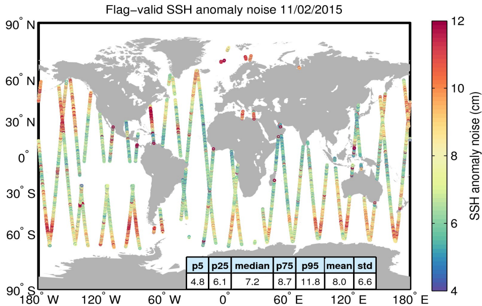
Figure 8. Geographical distribution of flag-valid 20-Hz SSH anomaly measurement noise over oceans and lakes for 11/02/2015. The statistical values shown in the table refer to the SSH anomaly noise and are calculated over all measurements shown in the figure.
