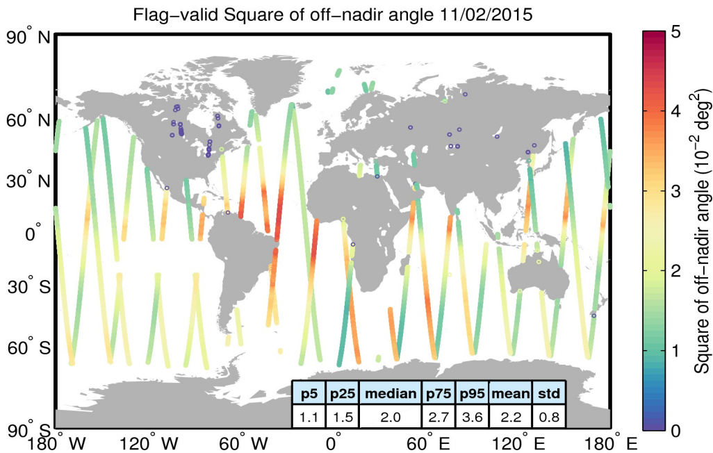
Figure 37. Geographical distribution of flag-valid mispointing data over oceans and lakes for 11/02/2015. The statistical values shown in the table refer to the mispointing in 10^{-2} deg 2 and are calculated over all measurements shown in the figure.
