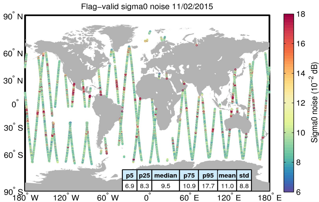
Figure 26. Geographical distribution of flag-valid 20-Hz sigma0 measurement noise over oceans and lakes for 11/02/2015. The statistical values shown in the table refer to the sigma0 noise and are calculated over all measurements shown in the figure.
