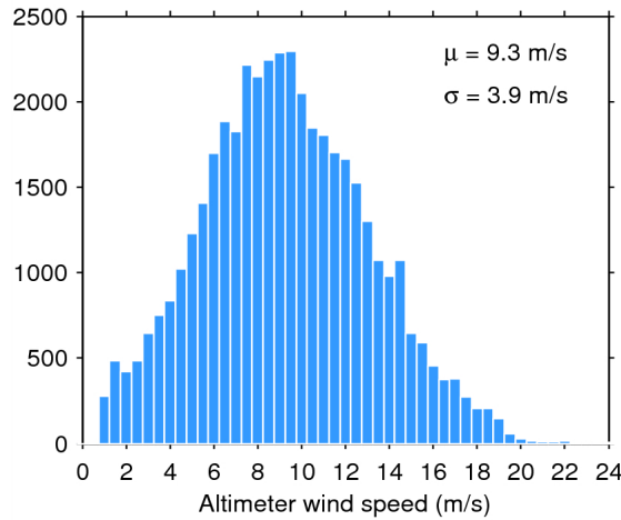
Figure 33. Histogram of flag-valid wind over oceans and lakes for 11/02/2015. The mean ( \mu ) and standard deviation ( \sigma ) are also shown. Note that values larger than 24 m/s are excluded from the histogram for the sake of readability but not from the computation of \mu and \sigma .
