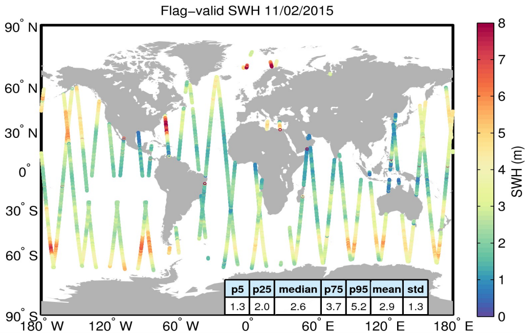
Figure 15. Geographical distribution of flag-valid SWH data over oceans and lakes for 11/02/2015. The statistical values shown in the table refer to the SWH in m and are calculated over all measurements shown in the figure.
