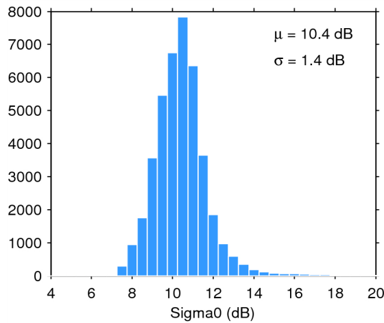
Figure 28. Histogram of science-valid sigma0 over oceans and lakes for 11/02/2015. The mean ( \mu ) and standard deviation ( \sigma ) are also shown. Note that values outside [4 20] dB are excluded from the histogram for the sake of readability but not from the computation of \mu and \sigma .
