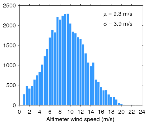
Figure 35. Histogram of science-valid wind over oceans and lakes for 11/02/2015. The mean ( \mu ) and standard deviation ( \sigma ) are also shown. Note that values larger than 24 m/s are excluded from the histogram for the sake of readability but not from the computation of \mu and \sigma .
