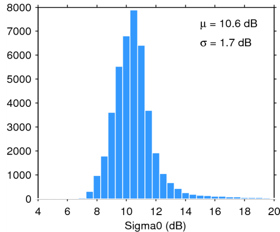
Figure 25. Histogram of flag-valid sigma0 over oceans and lakes for 11/02/2015. The mean ( \mu ) and standard deviation ( \sigma ) are also shown. Note that values outside [4 20] dB are excluded from the histogram for the sake of readability but not from the computation of \mu and \sigma .
