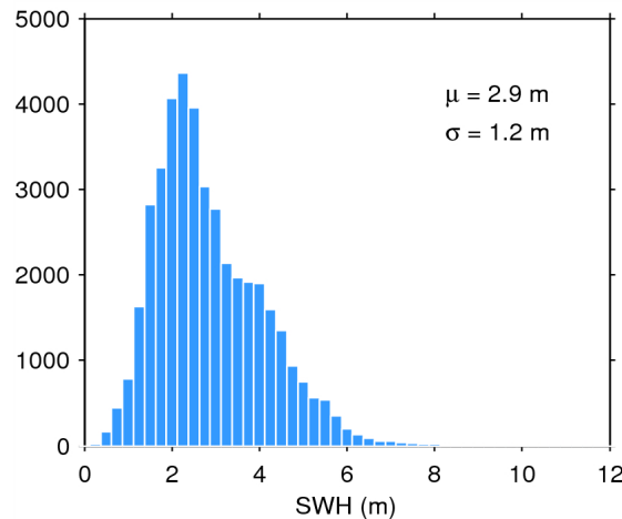
Figure 20. Histogram of science-valid SWH over oceans and lakes for 11/02/2015. The mean ( \mu ) and standard deviation ( \sigma ) are also shown. Note that values larger than 12 m are excluded from the histogram for the sake of readability but not from the computation of \mu and \sigma .
