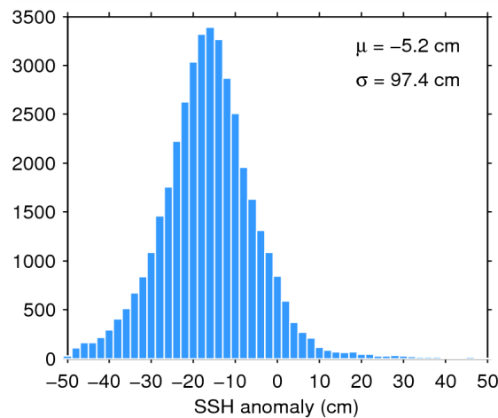
Figure 7. Histogram of flag-valid SSH anomaly over oceans and lakes for 11/02/2015. The mean ( \mu ) and standard deviation ( \sigma ) are also shown. Note that values outside [-50 50] cm are excluded from the histogram for the sake of readability but not from the computation of \mu and \sigma .
