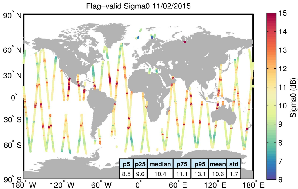
Figure 23. Geographical distribution of flag-valid sigma0 data over oceans and lakes for 11/02/2015. The statistical values shown in the table refer to the sigma0 in dB and are calculated over all measurements shown in the figure.
