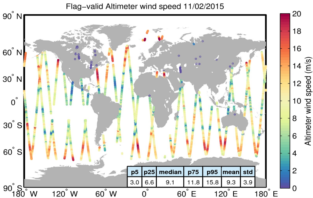
Figure 31. Geographical distribution of flag-valid wind data over oceans and lakes for 11/02/2015. The statistical values shown in the table refer to the wind in m/s and are calculated over all measurements shown in the figure.
