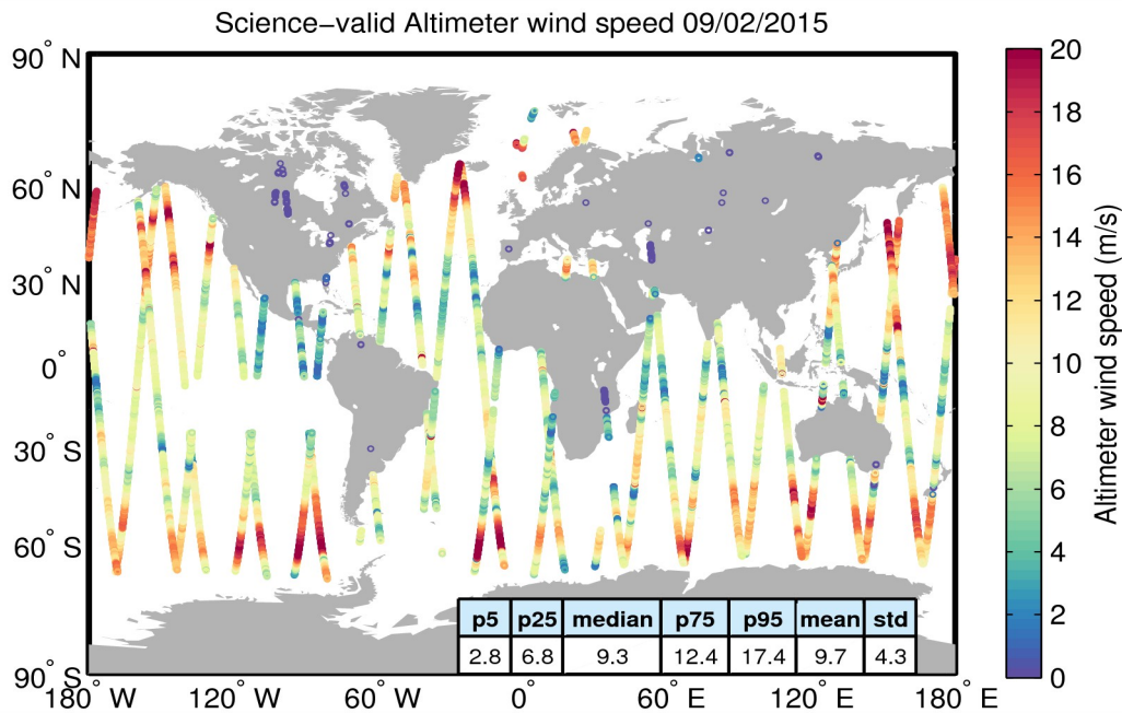
Figure 34. Geographical distribution of science-valid wind data over oceans and lakes for 09/02/2015. The statistical values shown in the table refer to the wind in m/s and are calculated over all measurements shown in the figure. Gray circles denote records that have been rejected based on the editing criteria described in Table 5.
