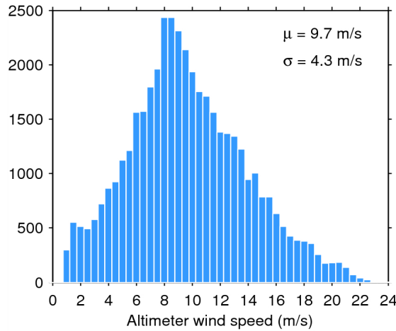
Figure 33. Histogram of flag-valid wind over oceans and lakes for 09/02/2015. The mean ( \mu ) and standard deviation ( \sigma ) are also shown. Note that values larger than 24 m/s are excluded from the histogram for the sake of readability but not from the computation of \mu and \sigma .
