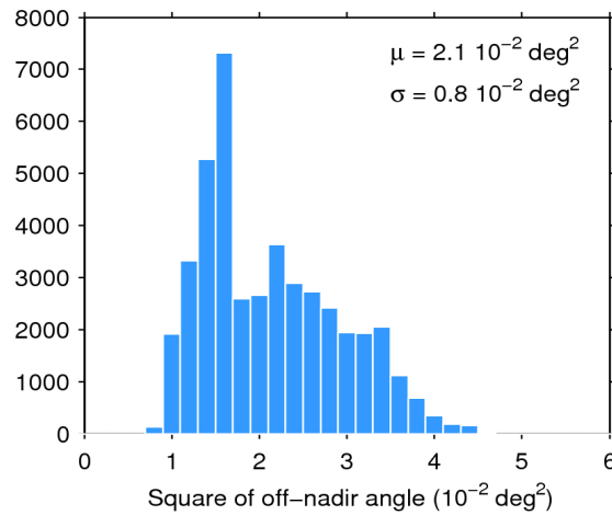
Figure 39. Histogram of flag-valid mispointing over oceans and lakes for 09/02/2015. The mean ( \mu ) and standard deviation ( \sigma ) are also shown. Note that values than 6 \cdot 10^{-2} \text{ deg}^2 are excluded from the histogram for the sake of readability but not from the computation of \mu and \sigma .
