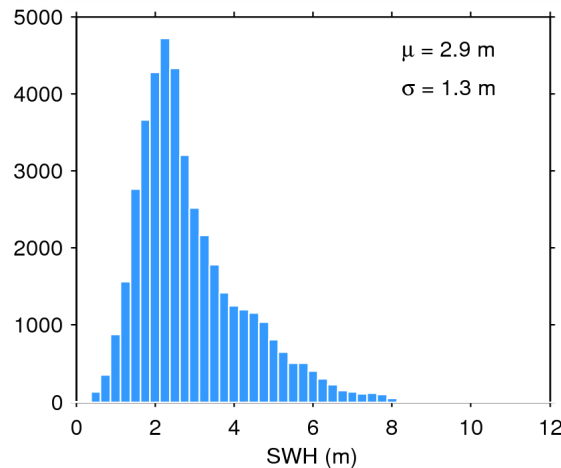
Figure 20. Histogram of science-valid SWH over oceans and lakes for 09/02/2015. The mean ( \mu ) and standard deviation ( \sigma ) are also shown. Note that values larger than 12 m are excluded from the histogram for the sake of readability but not from the computation of \mu and \sigma .
