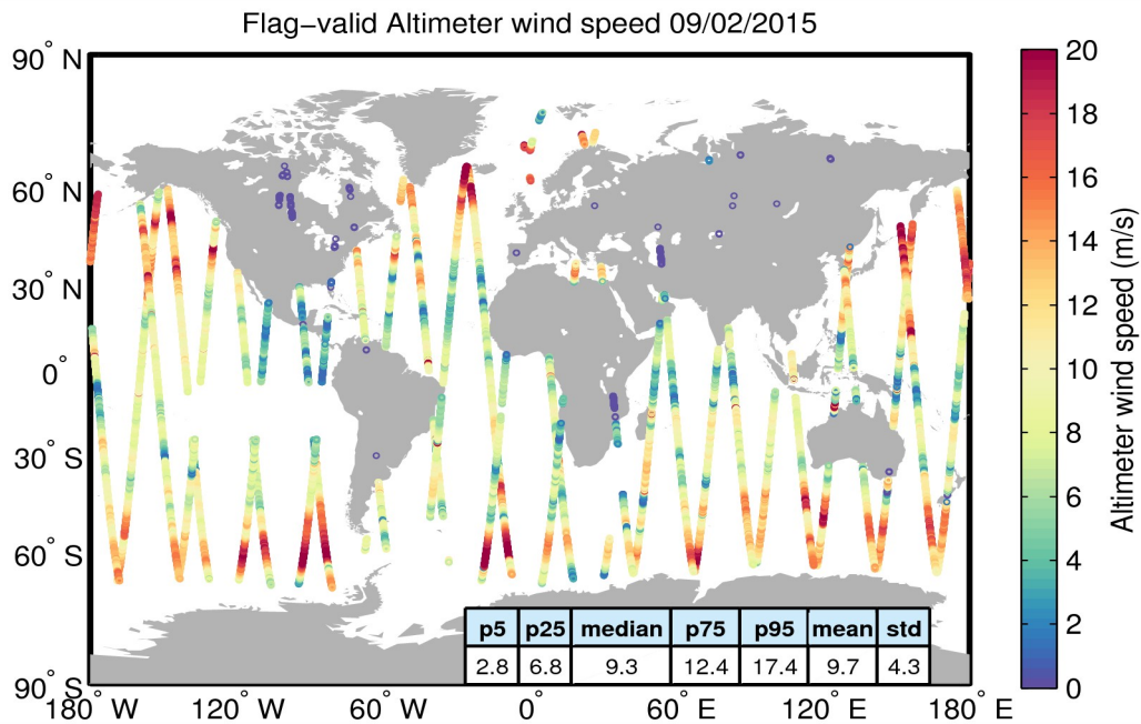
Figure 31. Geographical distribution of flag-valid wind data over oceans and lakes for 09/02/2015. The statistical values shown in the table refer to the wind in m/s and are calculated over all measurements shown in the figure.
