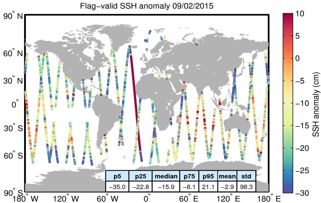
Figure 5. Geographical distribution of flag-valid 1-Hz SSH anomaly data over oceans and lakes for 09/02/2015. The statistical values shown in the table refer to the SSH anomaly in cm and are calculated over all measurements shown in the figure.
