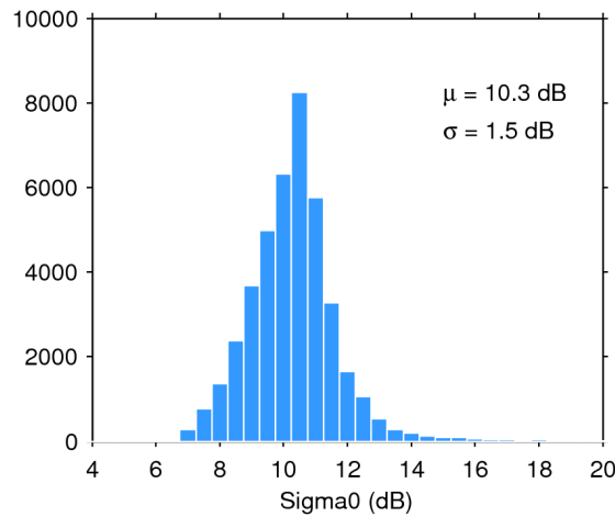
Figure 28. Histogram of science-valid sigma0 over oceans and lakes for 09/02/2015. The mean ( \mu ) and standard deviation ( \sigma ) are also shown. Note that values outside [4 20] dB are excluded from the histogram for the sake of readability but not from the computation of \mu and \sigma .
