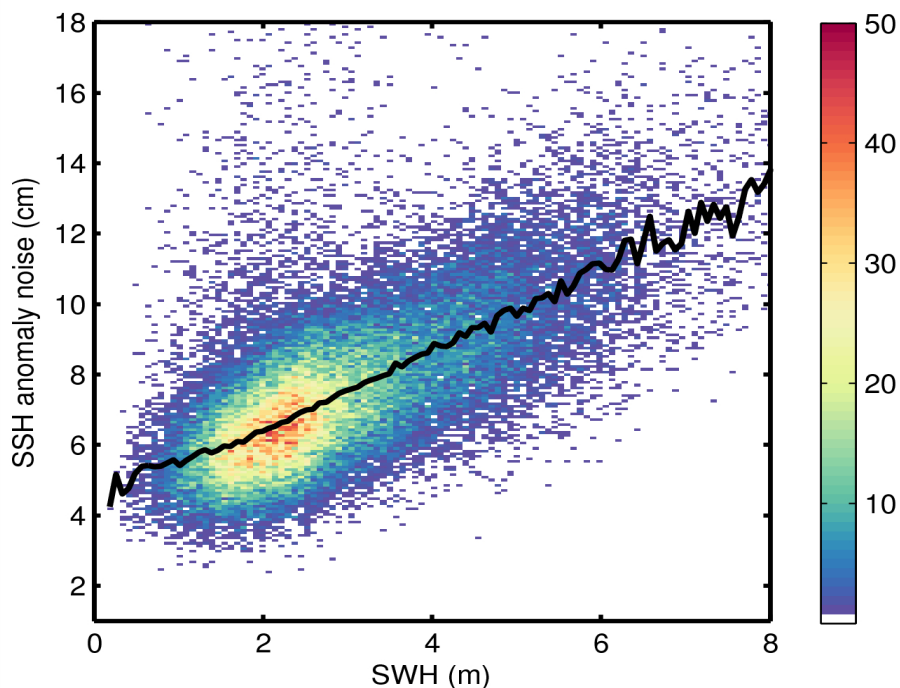
Figure 9. 2D histogram showing flag-valid SSH anomaly noise as a function of SWH for 09/02/2015. The black line denotes the median SSH anomaly as a function of SWH.
