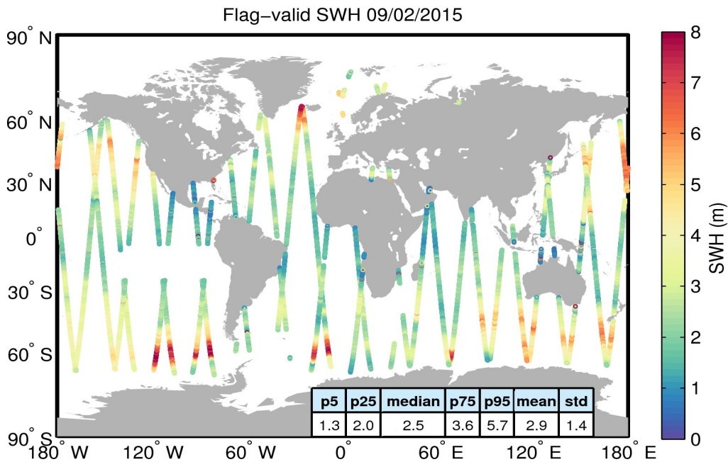
Figure 15. Geographical distribution of flag-valid SWH data over oceans and lakes for 09/02/2015. The statistical values shown in the figure refer to the SWH in m and are calculated over all measurements shown in the figure.
