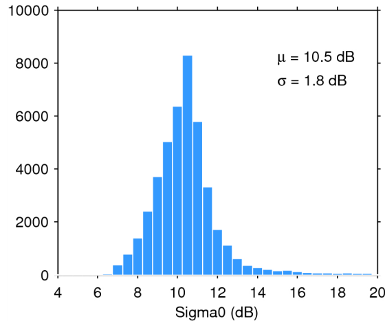
Figure 25. Histogram of flag-valid sigma0 over oceans and lakes for 09/02/2015. The mean ( \mu ) and standard deviation ( \sigma ) are also shown. Note that values outside [4 20] dB are excluded from the histogram for the sake of readability but not from the computation of \mu and \sigma .
