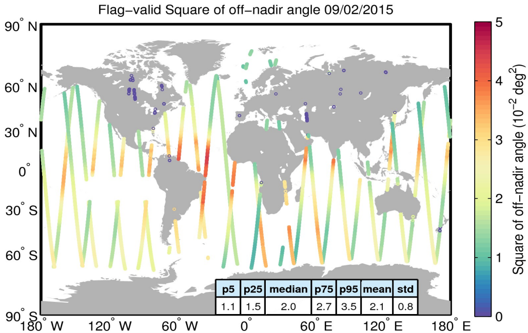
Figure 37. Geographical distribution of flag-valid mispointing data over oceans and lakes for 09/02/2015. The statistical values shown in the table refer to the mispointing in 10^{-2} \text{deg}^2 and are calculated over all measurements shown in the figure.
