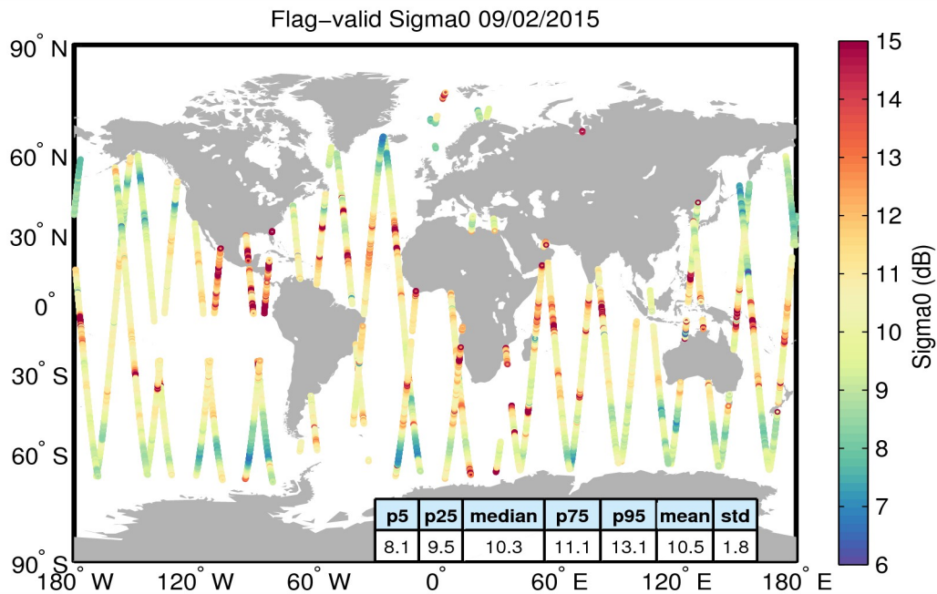
Figure 23. Geographical distribution of flag-valid sigma0 data over oceans and lakes for 09/02/2015. The statistical values shown in the table refer to the sigma0 in dB and are calculated over all measurements shown in the figure.
