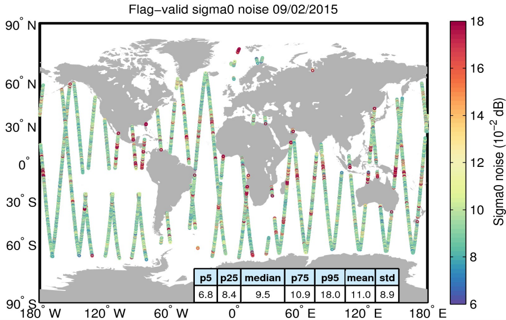
Figure 26. Geographical distribution of flag-valid 20-Hz sigma0 measurement noise over oceans and lakes for 09/02/2015. The statistical values shown in the table refer to the sigma0 noise and are calculated over all measurements shown in the figure.
