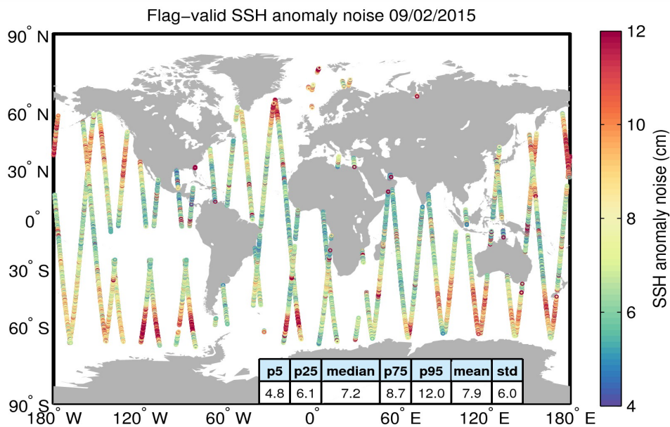
Figure 8. Geographical distribution of flag-valid 20-Hz SSH anomaly measurement noise over oceans and lakes for 09/02/2015. The statistical values shown in the table refer to the SSH anomaly noise and are calculated over all measurements shown in the figure.
