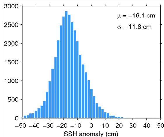
Figure 11. Histogram of science-valid SSH anomaly over oceans and lakes for 09/02/2015. The mean ( \mu ) and standard deviation ( \sigma ) are also shown. Note that values outside [-50 50] cm are excluded from the histogram for the sake of readability but not from the computation of \mu and \sigma .
