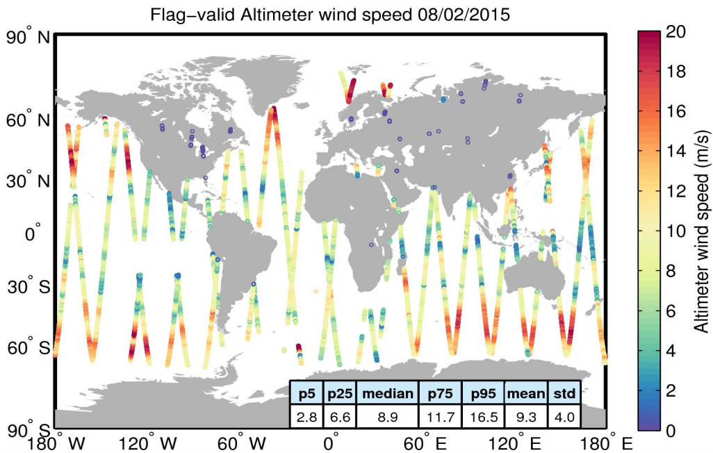
Figure 31. Geographical distribution of flag-valid wind data over oceans and lakes for 08/02/2015. The statistical values shown in the table refer to the wind in m/s and are calculated over all measurements shown in the figure.
