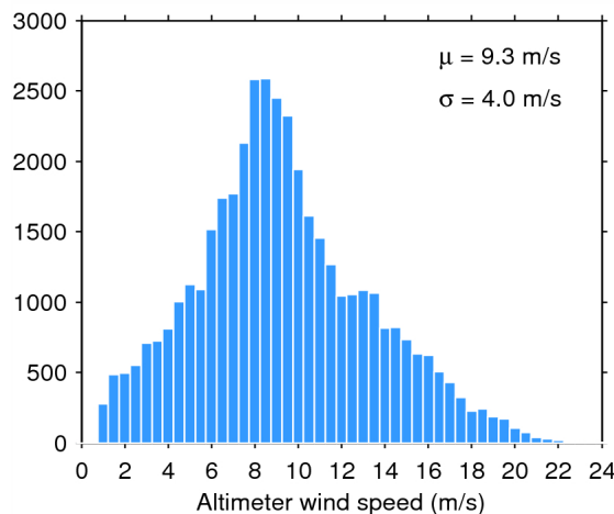
Figure 35. Histogram of science-valid wind over oceans and lakes for 08/02/2015. The mean ( \mu ) and standard deviation ( \sigma ) are also shown. Note that values larger than 24 m/s are excluded from the histogram for the sake of readability but not from the computation of \mu and \sigma .
