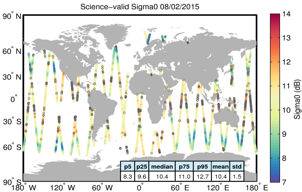
Figure 27. Geographical distribution of science-valid sigma0 data over oceans and lakes for 08/02/2015. The statistical values shown in the table refer to the sigma0 in dB and are calculated over all measurements shown in the figure. Gray circles denote records that have been rejected based on the editing criteria described in Table 4.
