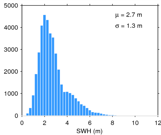
Figure 17. Histogram of flag-valid SWH over oceans and lakes for 08/02/2015. The mean ( \mu ) and standard deviation ( \sigma ) are also shown. Note that values larger than 12 m are excluded from the histogram for the sake of readability but not from the computation of \mu and \sigma .
