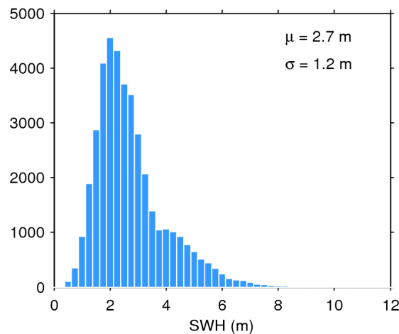
Figure 20. Histogram of science-valid SWH over oceans and lakes for 08/02/2015. The mean ( \mu ) and standard deviation ( \sigma ) are also shown. Note that values larger than 12 m are excluded from the histogram for the sake of readability but not from the computation of \mu and \sigma .
