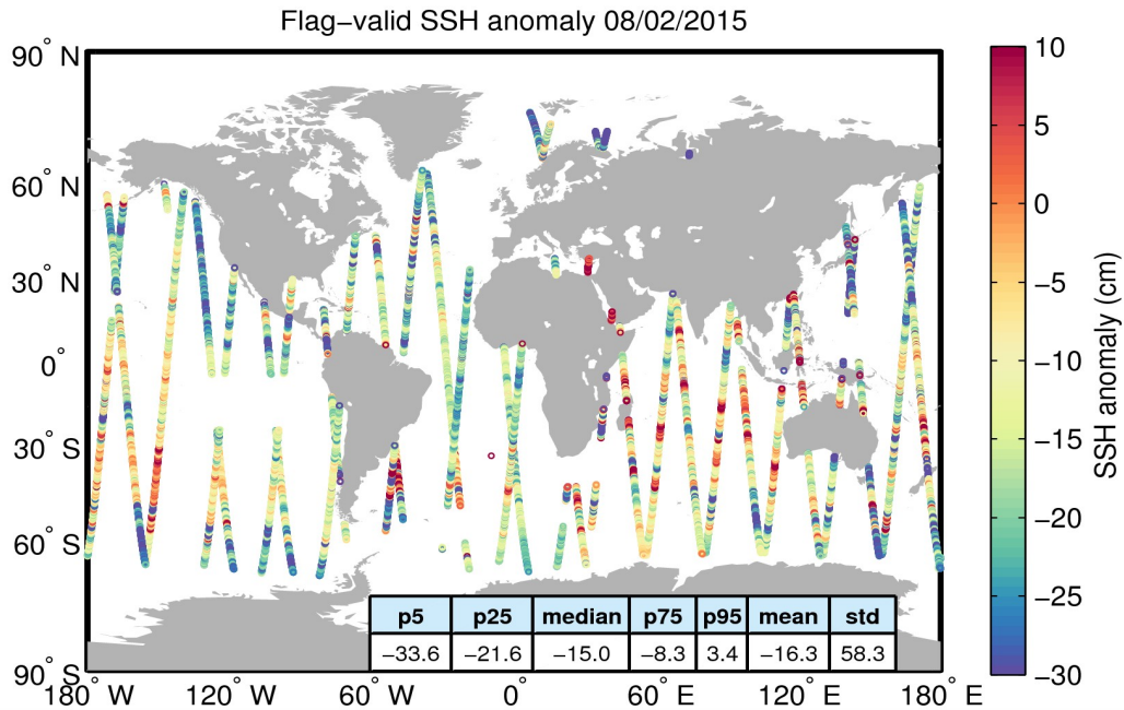
Figure 5. Geographical distribution of flag-valid 1-Hz SSH anomaly data over oceans and lakes for 08/02/2015. The statistical values shown in the table refer to the SSH anomaly in cm and are calculated over all measurements shown in the figure.
