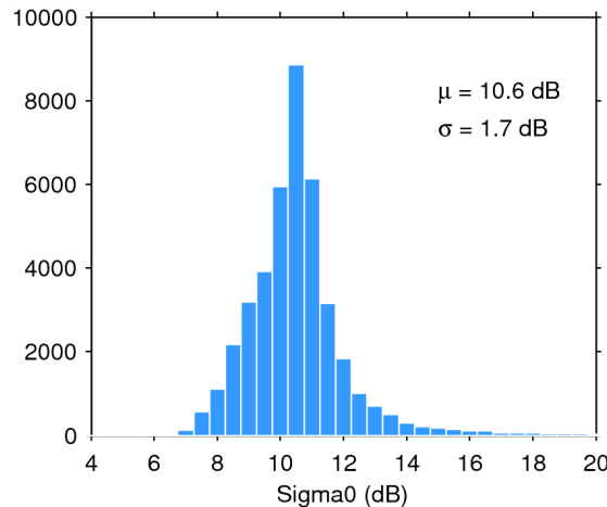
Figure 25. Histogram of flag-valid sigma0 over oceans and lakes for 08/02/2015. The mean ( \mu ) and standard deviation ( \sigma ) are also shown. Note that values outside [4 20] dB are excluded from the histogram for the sake of readability but not from the computation of \mu and \sigma .
