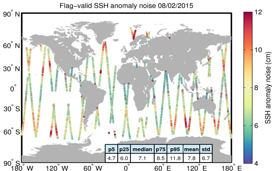
Figure 8. Geographical distribution of flag-valid 20-Hz SSH anomaly measurement noise over oceans and lakes for 08/02/2015. The statistical values shown in the table refer to the SSH anomaly noise and are calculated over all measurements shown in the figure.
