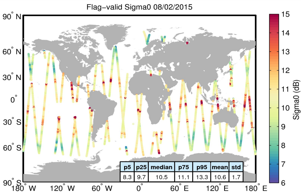
Figure 23. Geographical distribution of flag-valid sigma0 data over oceans and lakes for 08/02/2015. The statistical values shown in the table refer to the sigma0 in dB and are calculated over all measurements shown in the figure.
