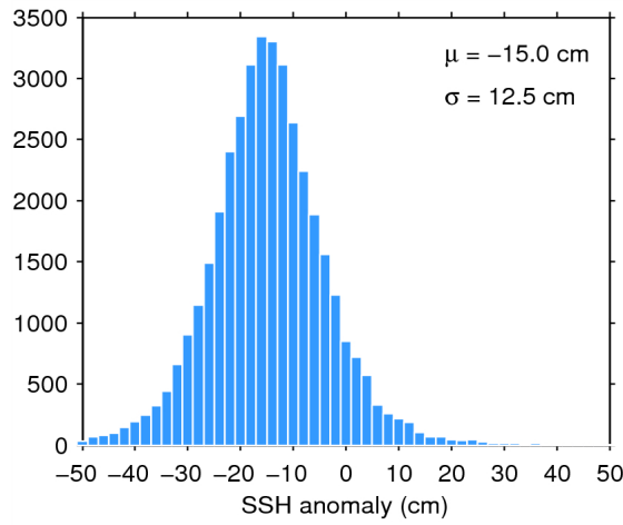
Figure 11. Histogram of science-valid SSH anomaly over oceans and lakes for 08/02/2015. The mean ( \mu ) and standard deviation ( \sigma ) are also shown. Note that values outside [-50 50] cm are excluded from the histogram for the sake of readability but not from the computation of \mu and \sigma .
