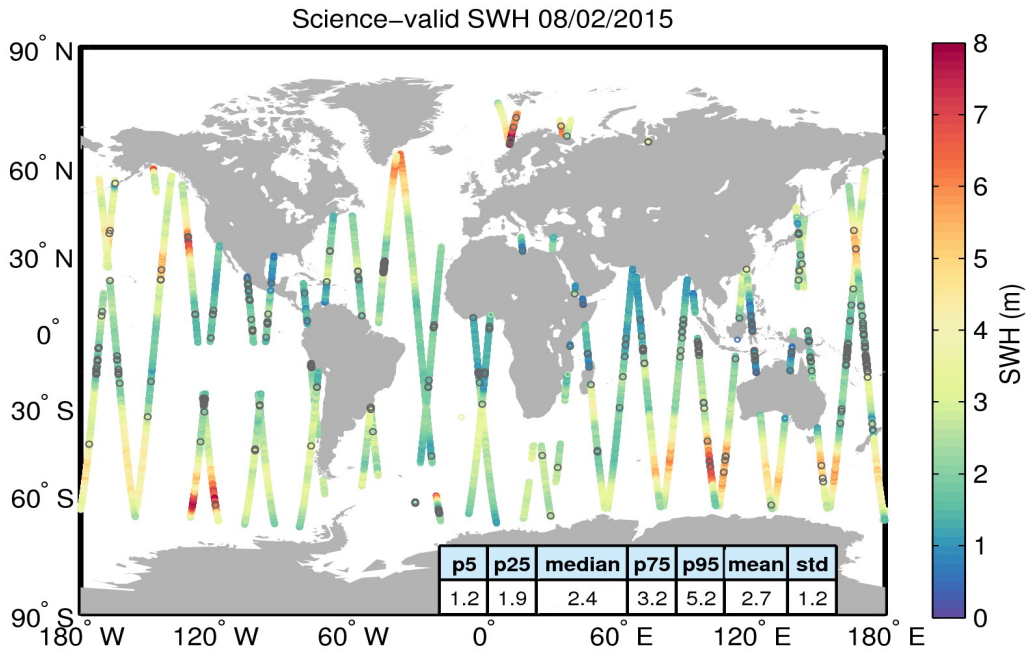
Figure 19. Geographical distribution of science-valid SWH data over oceans and lakes for 08/02/2015. The statistical values shown in the table refer to the SWH in m and are calculated over all measurements shown in the figure. Gray circles denote records that have been rejected based on the editing criteria described in Table 3.
