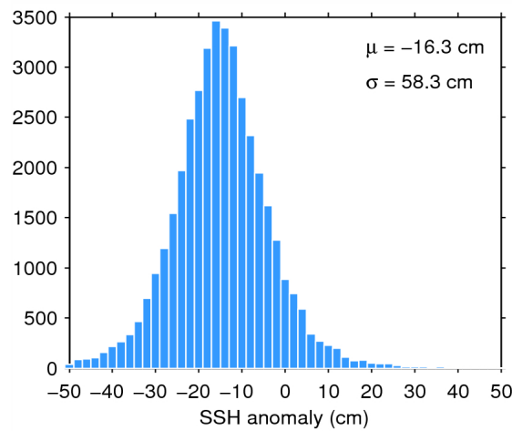
Figure 7. Histogram of flag-valid SSH anomaly over oceans and lakes for 08/02/2015. The mean ( \mu ) and standard deviation ( \sigma ) are also shown. Note that values outside [-50\ 50] cm are excluded from the histogram for the sake of readability but not from the computation of \mu and \sigma .
