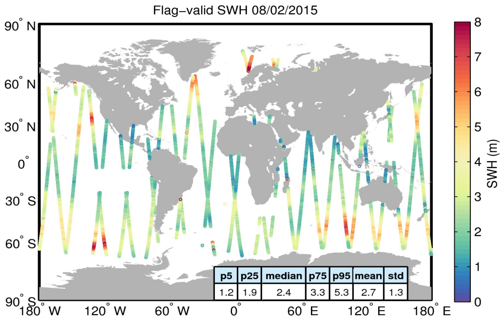
Figure 15. Geographical distribution of flag-valid SWH data over oceans and lakes for 08/02/2015. The statistical values shown in the table refer to the SWH in m and are calculated over all measurements shown in the figure.
