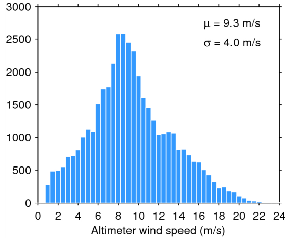
Figure 33. Histogram of flag-valid wind over oceans and lakes for 08/02/2015. The mean ( \mu ) and standard deviation ( \sigma ) are also shown. Note that values larger than 24 m/s are excluded from the histogram for the sake of readability but not from the computation of \mu and \sigma .
