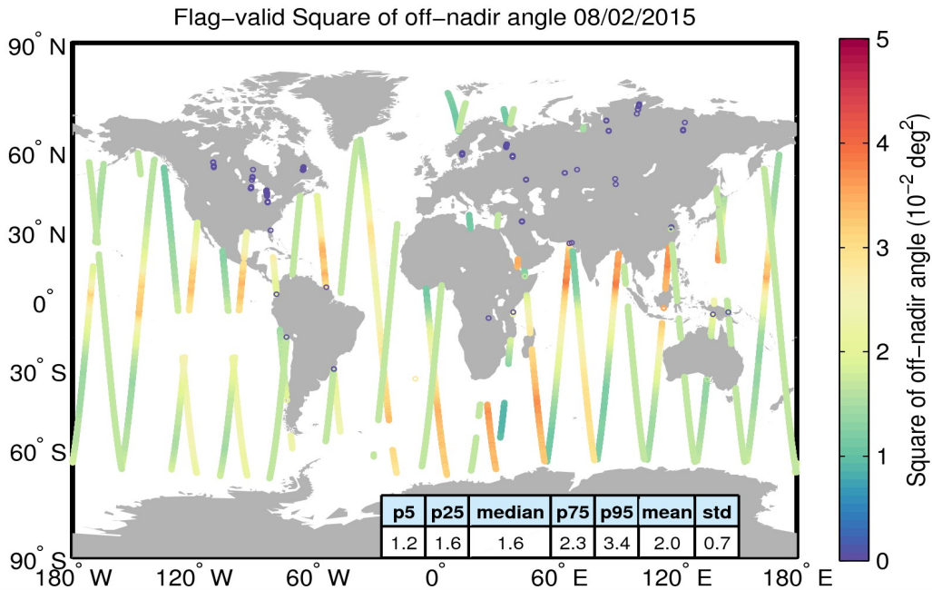
Figure 37. Geographical distribution of flag-valid mispointing data over oceans and lakes for 08/02/2015. The statistical values shown in the table refer to the mispointing in 10^{-2} \text{ deg}^2 and are calculated over all measurements shown in the figure.
