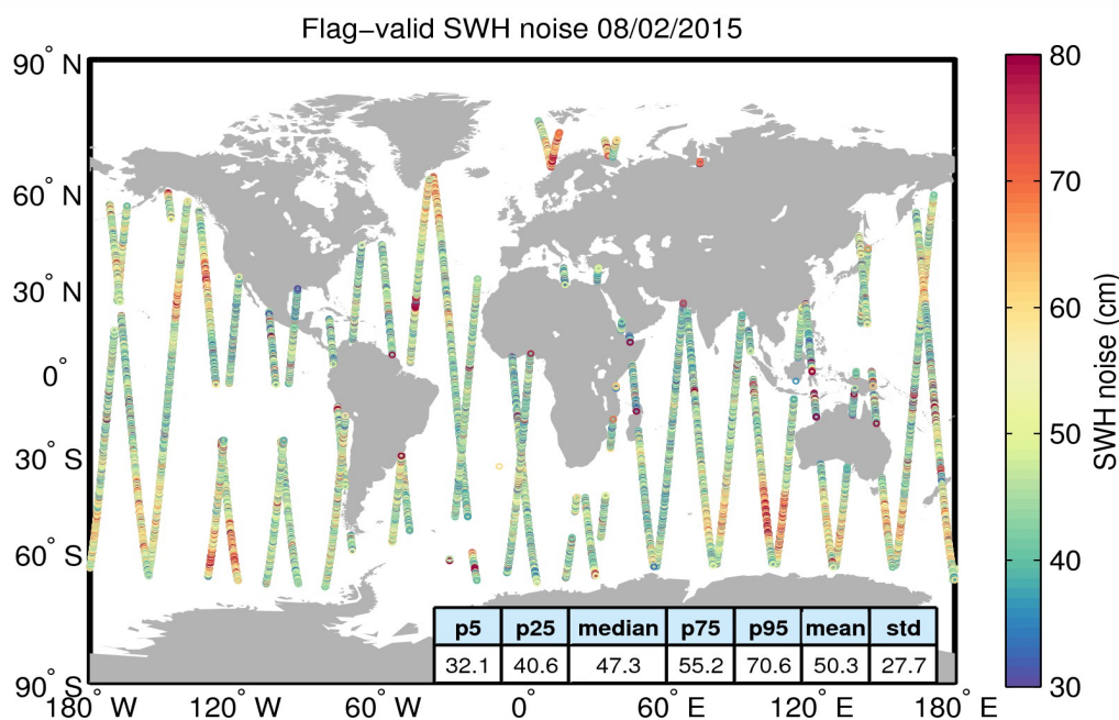
Figure 18. Geographical distribution of flag-valid 20-Hz SWH measurement noise over oceans and lakes for 08/02/2015. The statistical values shown in the figure refer to the SWH noise and are calculated over all measurements shown in the figure.
