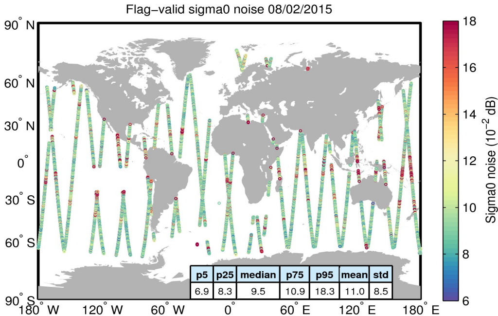
Figure 26. Geographical distribution of flag-valid 20-Hz sigma0 measurement noise over oceans and lakes for 08/02/2015. The statistical values shown in the table refer to the sigma0 noise and are calculated over all measurements shown in the figure.
