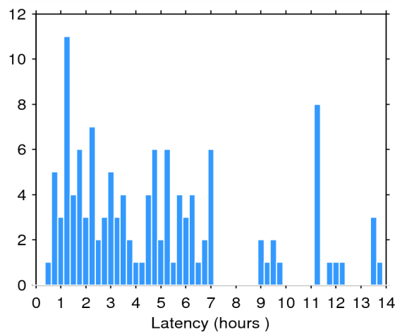
Figure 2. Histogram of the data latency for 08/02/2015. The y-axis denotes the number of files that are made available with a delay of x-hours with respect to the mean time of the records stored in the file.
