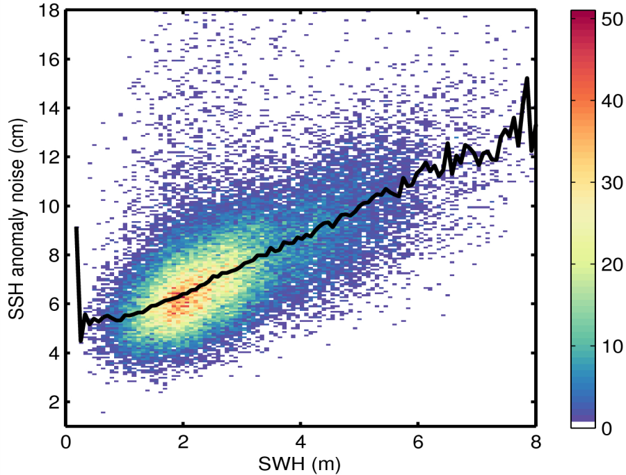
Figure 9. 2D histogram showing flag-valid SSH anomaly noise as a function of SWH for 08/02/2015. The black line denotes the median SSH anomaly as a function of SWH.
