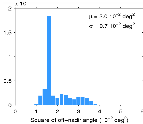
Figure 39. Histogram of flag-valid mispointing over oceans and lakes for 08/02/2015. The mean ( \mu ) and standard deviation ( \sigma ) are also shown. Note that values than 6 \cdot 10^{-2} \text{ deg}^2 are excluded from the histogram for the sake of readability but not from the computation of \mu and \sigma .
