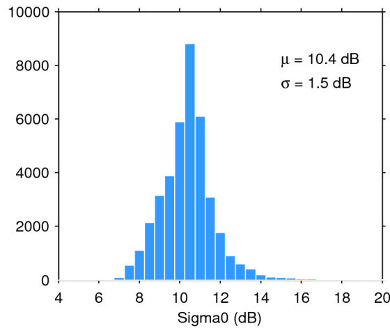
Figure 28. Histogram of science-valid sigma0 over oceans and lakes for 08/02/2015. The mean ( \mu ) and standard deviation ( \sigma ) are also shown. Note that values outside [4 20] dB are excluded from the histogram for the sake of readability but not from the computation of \mu and \sigma .
