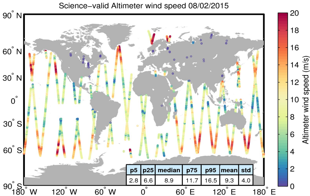
Figure 34. Geographical distribution of science-valid wind data over oceans and lakes for 08/02/2015. The statistical values shown in the table refer to the wind in m/s and are calculated over all measurements shown in the figure. Gray circles denote records that have been rejected based on the editing criteria described in Table 5.
