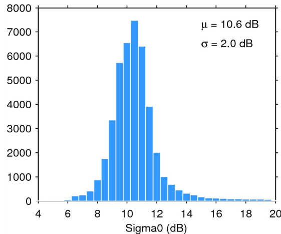
Figure 25. Histogram of flag-valid sigma0 over oceans and lakes for 07/02/2015. The mean ( \mu ) and standard deviation ( \sigma ) are also shown. Note that values outside [4 20] dB are excluded from the histogram for the sake of readability but not from the computation of \mu and \sigma .
