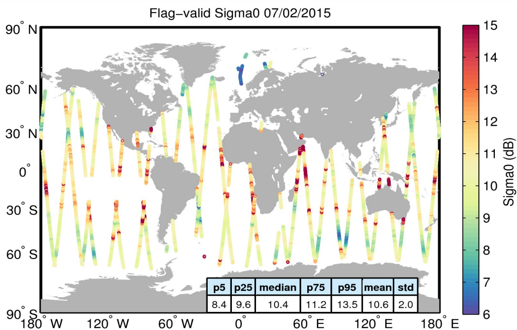
Figure 23. Geographical distribution of flag-valid sigma0 data over oceans and lakes for 07/02/2015. The statistical values shown in the table refer to the sigma0 in dB and are calculated over all measurements shown in the figure.
