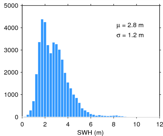
Figure 20. Histogram of science-valid SWH over oceans and lakes for 07/02/2015. The mean ( \mu ) and standard deviation ( \sigma ) are also shown. Note that values larger than 12 m are excluded from the histogram for the sake of readability but not from the computation of \mu and \sigma .
