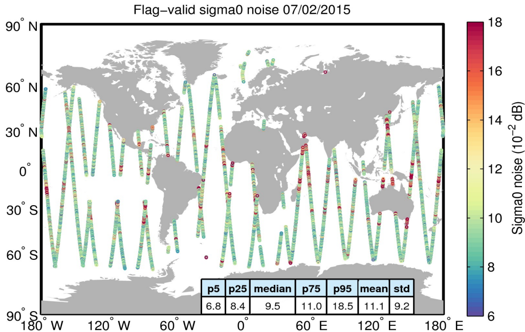
Figure 26. Geographical distribution of flag-valid 20-Hz sigma0 measurement noise over oceans and lakes for 07/02/2015. The statistical values shown in the table refer to the sigma0 noise and are calculated over all measurements shown in the figure.
