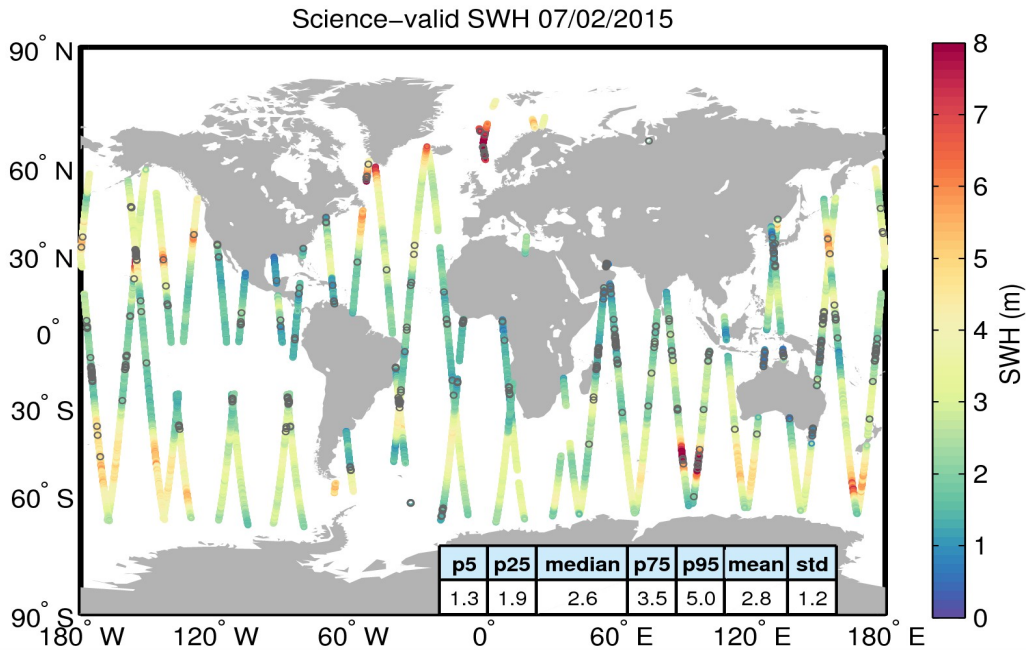
Figure 19. Geographical distribution of science-valid SWH data over oceans and lakes for 07/02/2015. The statistical values shown in the table refer to the SWH in m and are calculated over all measurements shown in the figure. Gray circles denote records that have been rejected based on the editing criteria described in Table 3.
