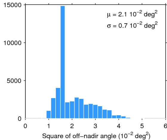
Figure 39. Histogram of flag-valid mispointing over oceans and lakes for 07/02/2015. The mean ( \mu ) and standard deviation ( \sigma ) are also shown. Note that values than 6 \cdot 10^{-2} \text{ deg}^2 are excluded from the histogram for the sake of readability but not from the computation of \mu and \sigma .
