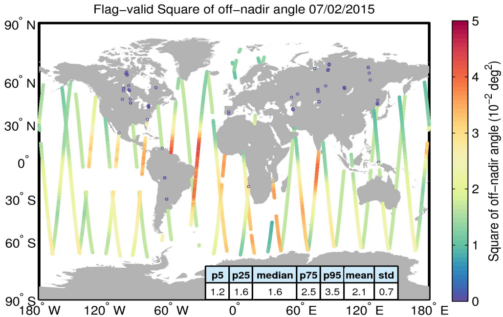
Figure 37. Geographical distribution of flag-valid mispointing data over oceans and lakes for 07/02/2015. The statistical values shown in the table refer to the mispointing in 10^{-2} \text{ deg}^2 and are calculated over all measurements shown in the figure.
