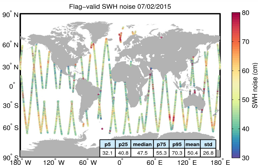
Figure 18. Geographical distribution of flag-valid 20-Hz SWH measurement noise over oceans and lakes for 07/02/2015. The statistical values shown in the figure refer to the SWH noise and are calculated over all measurements shown in the figure.
