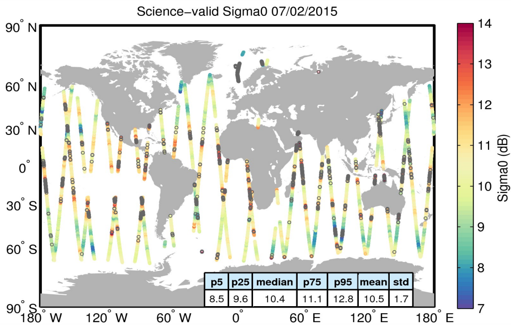
Figure 27. Geographical distribution of science-valid sigma0 data over oceans and lakes for 07/02/2015. The statistical values shown in the table refer to the sigma0 in dB and are calculated over all measurements shown in the figure. Gray circles denote records that have been rejected based on the editing criteria described in Table 4.
