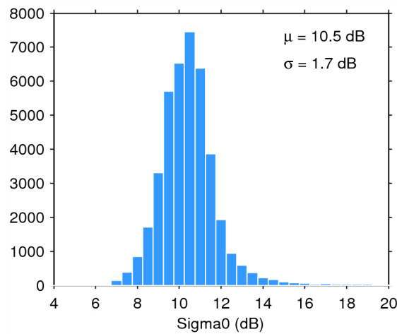
Figure 28. Histogram of science-valid sigma0 over oceans and lakes for 07/02/2015. The mean ( \mu ) and standard deviation ( \sigma ) are also shown. Note that values outside [4 20] dB are excluded from the histogram for the sake of readability but not from the computation of \mu and \sigma .
