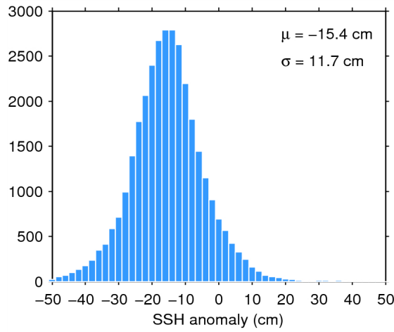
Figure 11. Histogram of science-valid SSH anomaly over oceans and lakes for 07/02/2015. The mean ( \mu ) and standard deviation ( \sigma ) are also shown. Note that values outside [-50 50] cm are excluded from the histogram for the sake of readability but not from the computation of \mu and \sigma .
