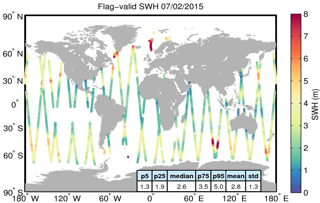
Figure 15. Geographical distribution of flag-valid SWH data over oceans and lakes for 07/02/2015. The statistical values shown in the table refer to the SWH in m and are calculated over all measurements shown in the figure.
