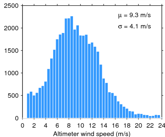
Figure 35. Histogram of science-valid wind over oceans and lakes for 07/02/2015. The mean ( \mu ) and standard deviation ( \sigma ) are also shown. Note that values larger than 24 m/s are excluded from the histogram for the sake of readability but not from the computation of \mu and \sigma .
