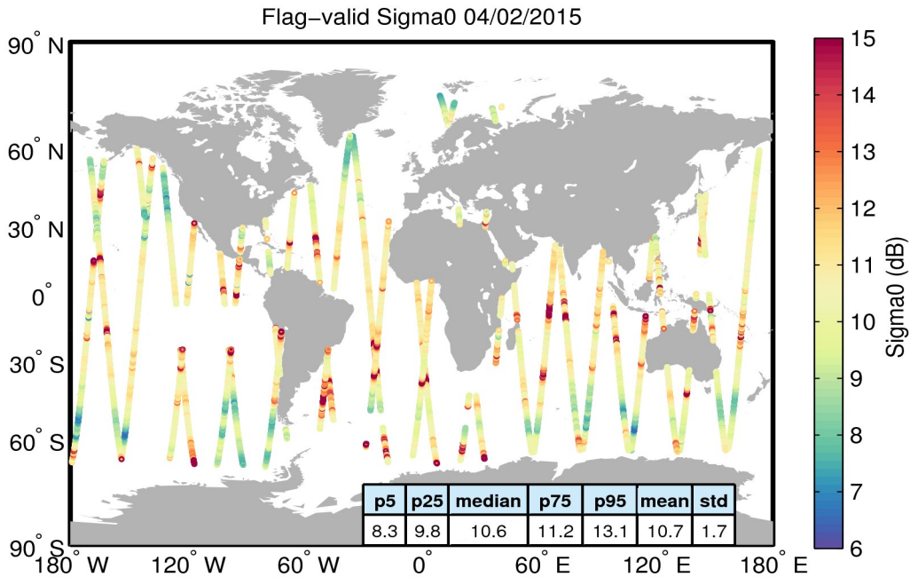
Figure 23. Geographical distribution of flag-valid sigma0 data over oceans and lakes for 04/02/2015. The statistical values shown in the table refer to the sigma0 in dB and are calculated over all measurements shown in the figure.
