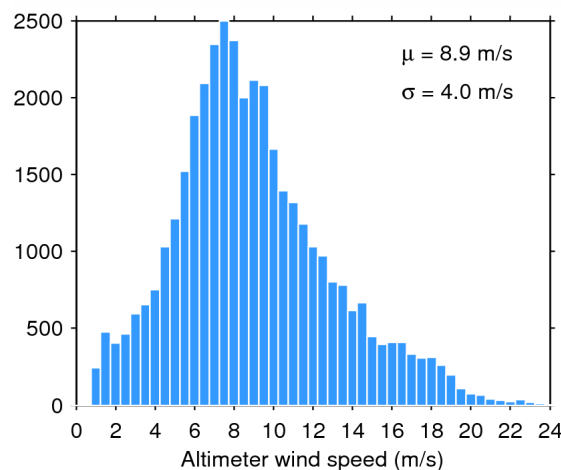
Figure 35. Histogram of science-valid wind over oceans and lakes for 04/02/2015. The mean ( \mu ) and standard deviation ( \sigma ) are also shown. Note that values larger than 24 m/s are excluded from the histogram for the sake of readability but not from the computation of \mu and \sigma .
