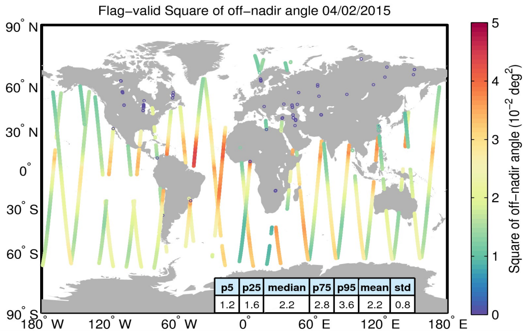
Figure 37. Geographical distribution of flag-valid mispointing data over oceans and lakes for 04/02/2015. The statistical values shown in the table refer to the mispointing in 10^{-2} \text{ deg}^2 and are calculated over all measurements shown in the figure.
