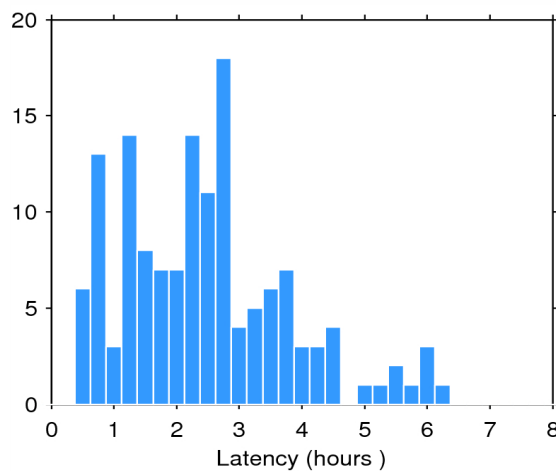
Figure 2. Histogram of the data latency for 04/02/2015. The y-axis denotes the number of files that are made available with a delay of x-hours with respect to the mean time of the records stored in the file.
