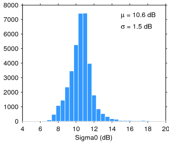
Figure 28. Histogram of science-valid sigma0 over oceans and lakes for 04/02/2015. The mean ( \mu ) and standard deviation ( \sigma ) are also shown. Note that values outside [4 20] dB are excluded from the histogram for the sake of readability but not from the computation of \mu and \sigma .
