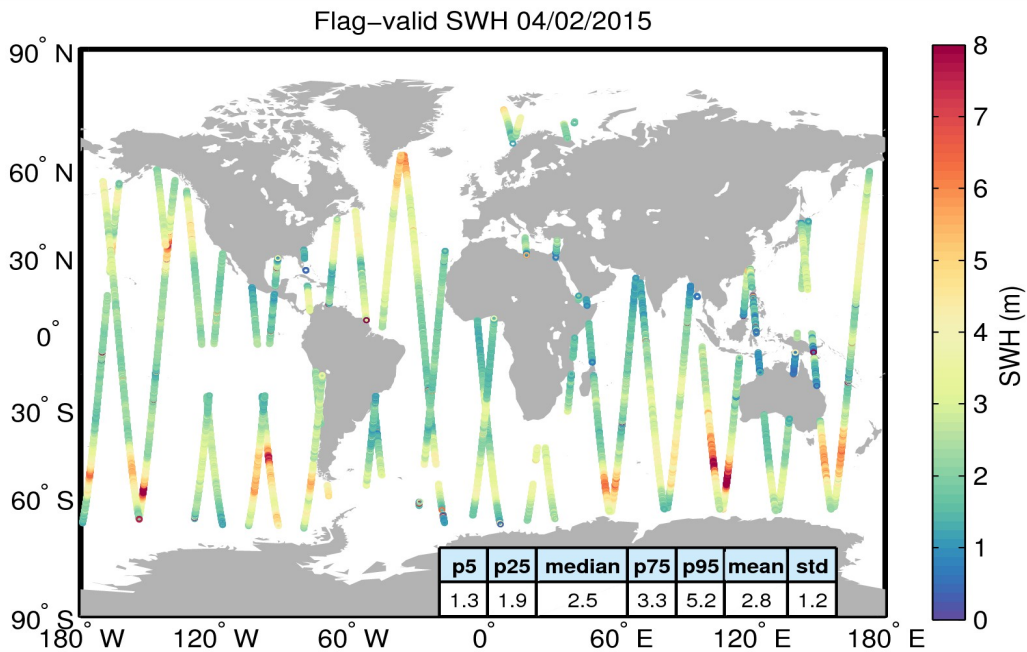
Figure 15. Geographical distribution of flag-valid SWH data over oceans and lakes for 04/02/2015. The statistical values shown in the figure refer to the SWH in m and are calculated over all measurements shown in the figure.
