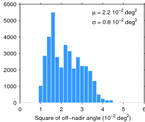
Figure 39. Histogram of flag-valid mispointing over oceans and lakes for 04/02/2015. The mean ( \mu ) and standard deviation ( \sigma ) are also shown. Note that values than 6 \cdot 10^{-2} \text{ deg}^2 are excluded from the histogram for the sake of readability but not from the computation of \mu and \sigma .
