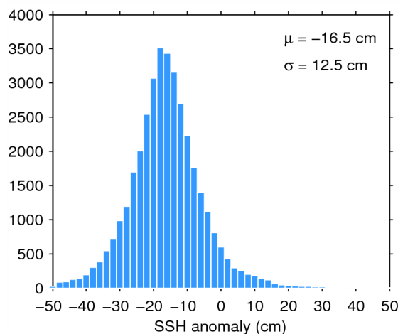
Figure 11. Histogram of science-valid SSH anomaly over oceans and lakes for 04/02/2015. The mean ( \mu ) and standard deviation ( \sigma ) are also shown. Note that values outside [-50 50] cm are excluded from the histogram for the sake of readability but not from the computation of \mu and \sigma .
