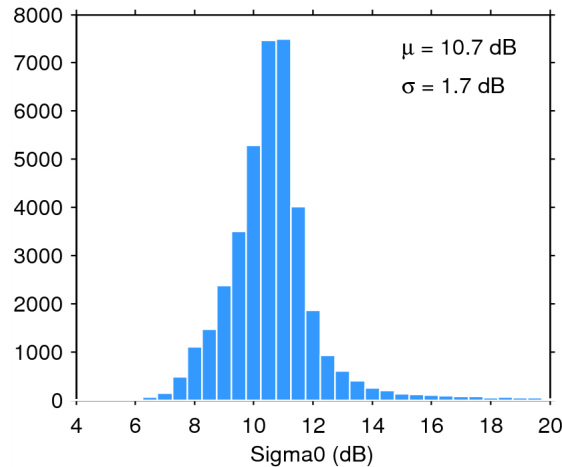
Figure 25. Histogram of flag-valid sigma0 over oceans and lakes for 04/02/2015. The mean ( \mu ) and standard deviation ( \sigma ) are also shown. Note that values outside [4 20] dB are excluded from the histogram for the sake of readability but not from the computation of \mu and \sigma .
