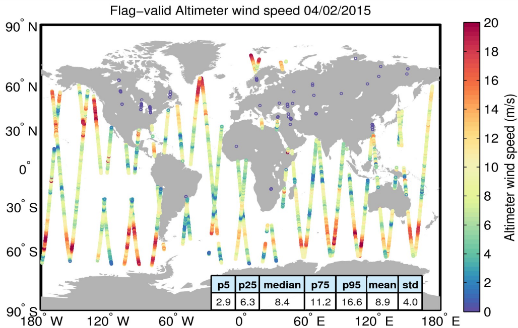
Figure 31. Geographical distribution of flag-valid wind data over oceans and lakes for 04/02/2015. The statistical values shown in the table refer to the wind in m/s and are calculated over all measurements shown in the figure.
