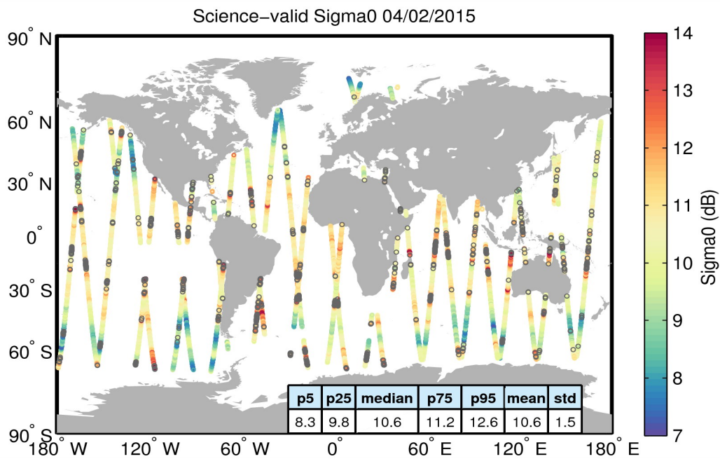
Figure 27. Geographical distribution of science-valid sigma0 data over oceans and lakes for 04/02/2015. The statistical values shown in the table refer to the sigma0 in dB and are calculated over all measurements shown in the figure. Gray circles denote records that have been rejected based on the editing criteria described in Table 4.
