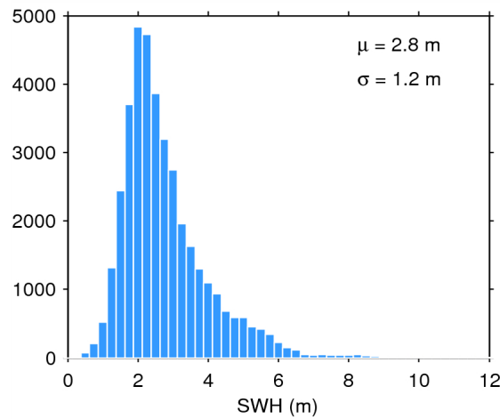
Figure 17. Histogram of flag-valid SWH over oceans and lakes for 04/02/2015. The mean ( \mu ) and standard deviation ( \sigma ) are also shown. Note that values larger than 12 m are excluded from the histogram for the sake of readability but not from the computation of \mu and \sigma .
