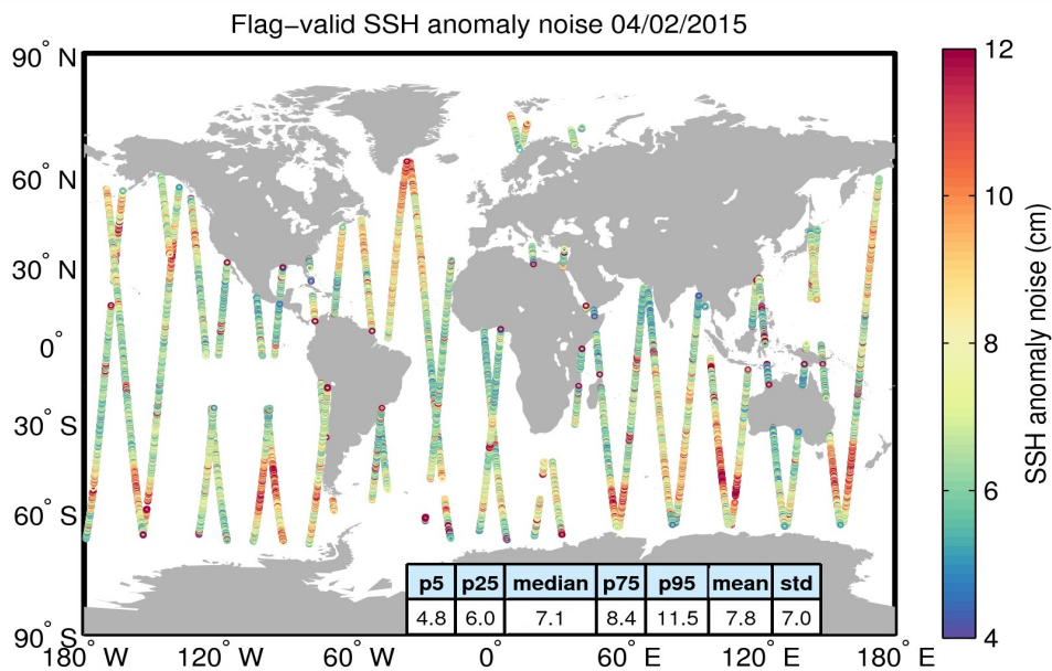
Figure 8. Geographical distribution of flag-valid 20-Hz SSH anomaly measurement noise over oceans and lakes for 04/02/2015. The statistical values shown in the table refer to the SSH anomaly noise and are calculated over all measurements shown in the figure.
