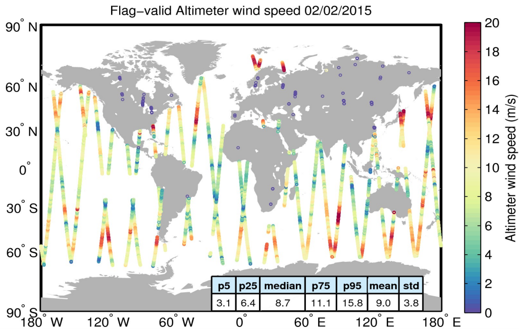
Figure 31. Geographical distribution of flag-valid wind data over oceans and lakes for 02/02/2015. The statistical values shown in the table refer to the wind in m/s and are calculated over all measurements shown in the figure.
