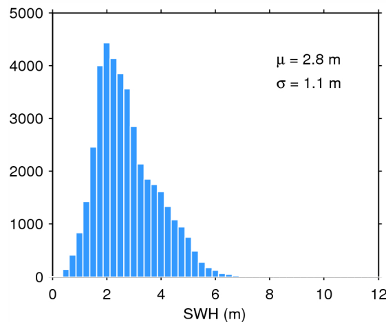
Figure 17. Histogram of flag-valid SWH over oceans and lakes for 02/02/2015. The mean ( \mu ) and standard deviation ( \sigma ) are also shown. Note that values larger than 12 m are excluded from the histogram for the sake of readability but not from the computation of \mu and \sigma .
