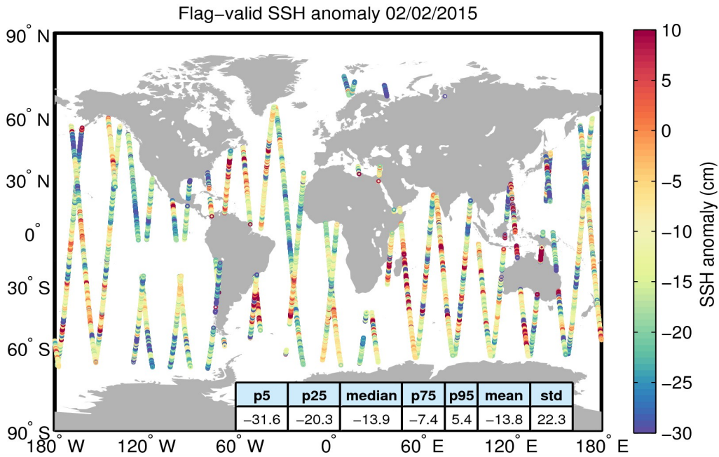
Figure 5. Geographical distribution of flag-valid 1-Hz SSH anomaly data over oceans and lakes for 02/02/2015. The statistical values shown in the table refer to the SSH anomaly in cm and are calculated over all measurements shown in the figure.
