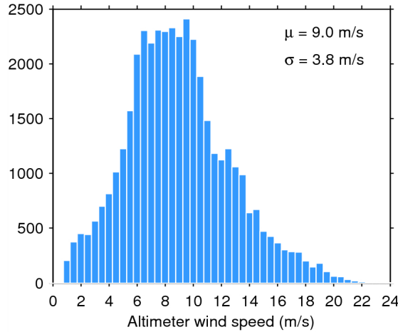
Figure 33. Histogram of flag-valid wind over oceans and lakes for 02/02/2015. The mean ( \mu ) and standard deviation ( \sigma ) are also shown. Note that values larger than 24 m/s are excluded from the histogram for the sake of readability but not from the computation of \mu and \sigma .
