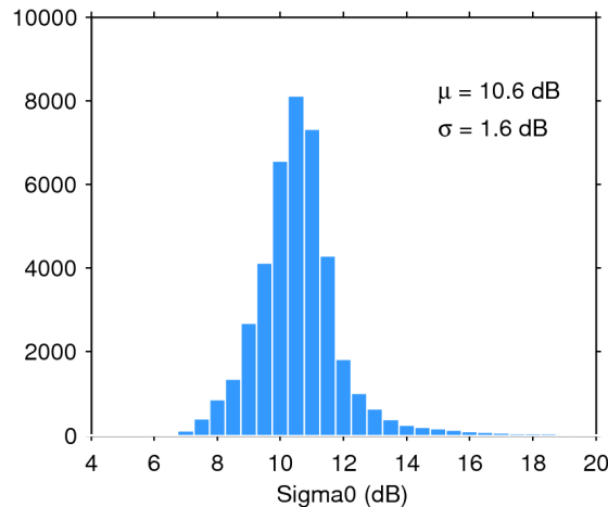
Figure 25. Histogram of flag-valid sigma0 over oceans and lakes for 02/02/2015. The mean ( \mu ) and standard deviation ( \sigma ) are also shown. Note that values outside [4 20] dB are excluded from the histogram for the sake of readability but not from the computation of \mu and \sigma .
