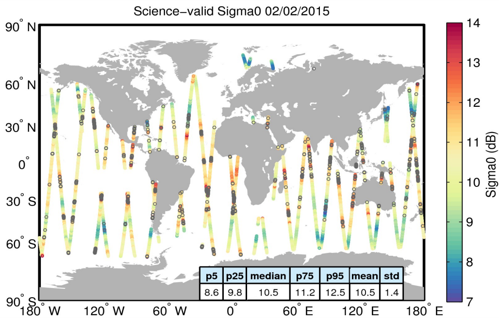
Figure 27. Geographical distribution of science-valid sigma0 data over oceans and lakes for 02/02/2015. The statistical values shown in the table refer to the sigma0 in dB and are calculated over all measurements shown in the figure. Gray circles denote records that have been rejected based on the editing criteria described in Table 4.
