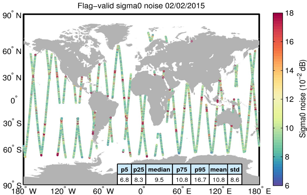
Figure 26. Geographical distribution of flag-valid 20-Hz sigma0 measurement noise over oceans and lakes for 02/02/2015. The statistical values shown in the table refer to the sigma0 noise and are calculated over all measurements shown in the figure.
