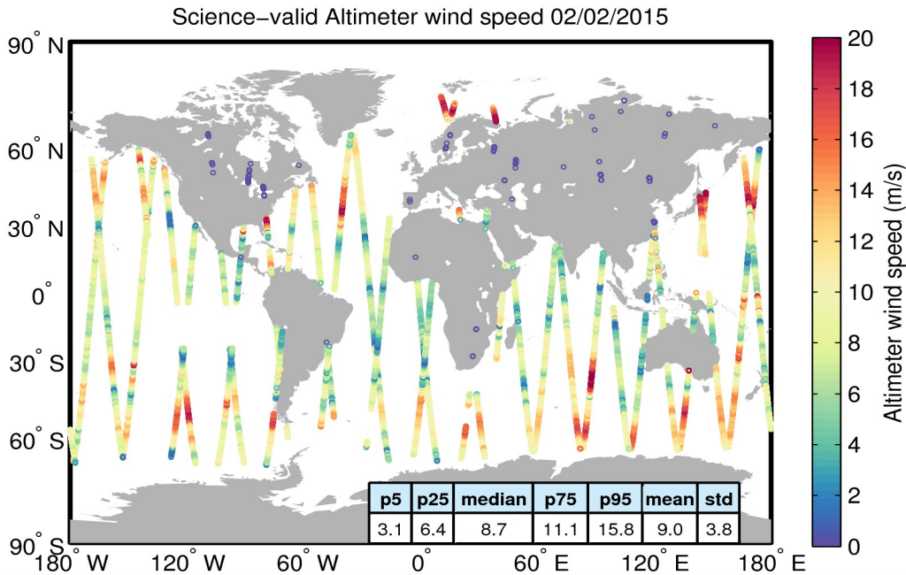
Figure 34. Geographical distribution of science-valid wind data over oceans and lakes for 02/02/2015. The statistical values shown in the table refer to the wind in m/s and are calculated over all measurements shown in the figure. Gray circles denote records that have been rejected based on the editing criteria described in Table 5.
