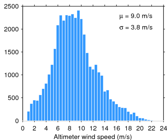
Figure 35. Histogram of science-valid wind over oceans and lakes for 02/02/2015. The mean ( \mu ) and standard deviation ( \sigma ) are also shown. Note that values larger than 24 m/s are excluded from the histogram for the sake of readability but not from the computation of \mu and \sigma .
