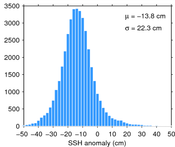
Figure 7. Histogram of flag-valid SSH anomaly over oceans and lakes for 02/02/2015. The mean ( \mu ) and standard deviation ( \sigma ) are also shown. Note that values outside [-50\ 50] cm are excluded from the histogram for the sake of readability but not from the computation of \mu and \sigma .
