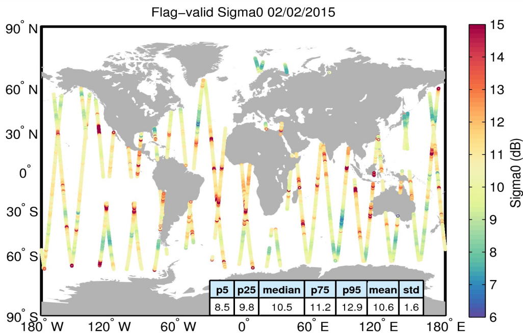
Figure 23. Geographical distribution of flag-valid sigma0 data over oceans and lakes for 02/02/2015. The statistical values shown in the table refer to the sigma0 in dB and are calculated over all measurements shown in the figure.
