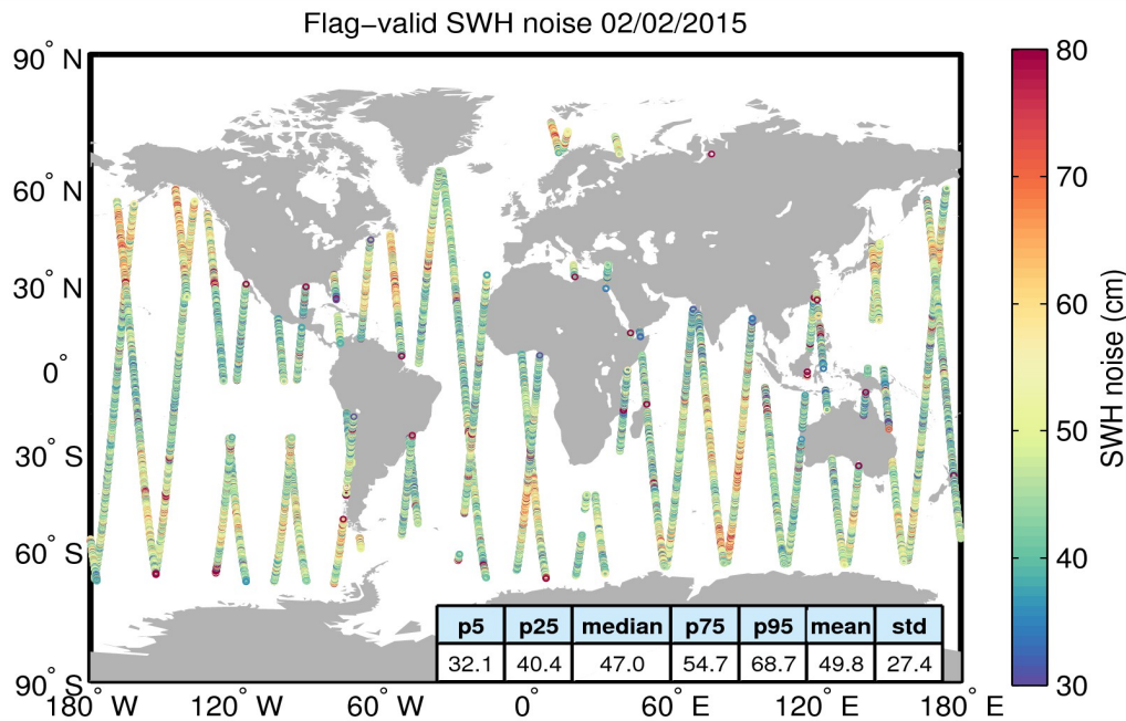
Figure 18. Geographical distribution of flag-valid 20-Hz SWH measurement noise over oceans and lakes for 02/02/2015. The statistical values shown in the figure refer to the SWH noise and are calculated over all measurements shown in the figure.
