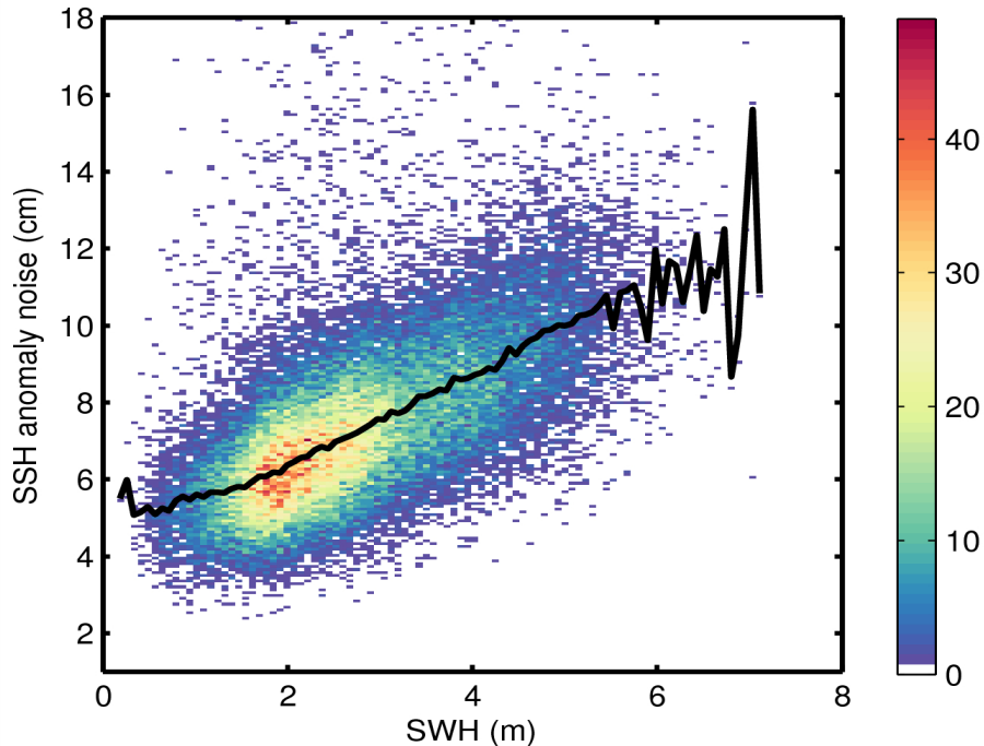
Figure 9. 2D histogram showing flag-valid SSH anomaly noise as a function of SWH for 02/02/2015. The black line denotes the median SSH anomaly as a function of SWH.
