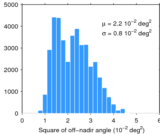
Figure 39. Histogram of flag-valid mispointing over oceans and lakes for 02/02/2015. The mean ( \mu ) and standard deviation ( \sigma ) are also shown. Note that values than 6 \cdot 10^{-2} \text{ deg}^2 are excluded from the histogram for the sake of readability but not from the computation of \mu and \sigma .
