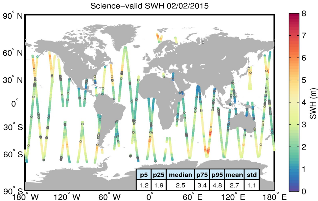
Figure 19. Geographical distribution of science-valid SWH data over oceans and lakes for 02/02/2015. The statistical values shown in the table refer to the SWH in m and are calculated over all measurements shown in the figure. Gray circles denote records that have been rejected based on the editing criteria described in Table 3.
