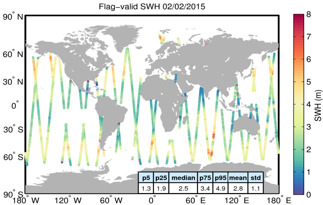
Figure 15. Geographical distribution of flag-valid SWH data over oceans and lakes for 02/02/2015. The statistical values shown in the table refer to the SWH in m and are calculated over all measurements shown in the figure.
