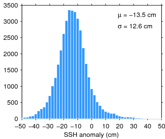
Figure 11. Histogram of science-valid SSH anomaly over oceans and lakes for 02/02/2015. The mean ( \mu ) and standard deviation ( \sigma ) are also shown. Note that values outside [-50 50] cm are excluded from the histogram for the sake of readability but not from the computation of \mu and \sigma .
