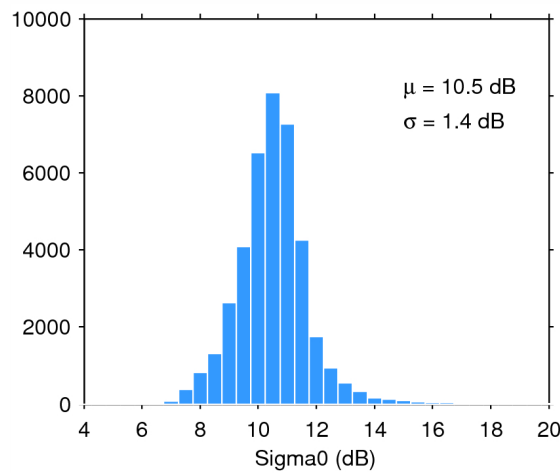
Figure 28. Histogram of science-valid sigma0 over oceans and lakes for 02/02/2015. The mean ( \mu ) and standard deviation ( \sigma ) are also shown. Note that values outside [4 20] dB are excluded from the histogram for the sake of readability but not from the computation of \mu and \sigma .
