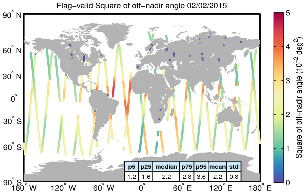
Figure 37. Geographical distribution of flag-valid mispointing data over oceans and lakes for 02/02/2015. The statistical values shown in the table refer to the mispointing in 10^{-2} \text{deg}^2 and are calculated over all measurements shown in the figure.
