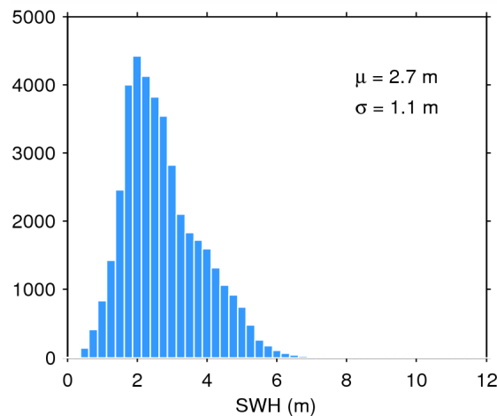
Figure 20. Histogram of science-valid SWH over oceans and lakes for 02/02/2015. The mean ( \mu ) and standard deviation ( \sigma ) are also shown. Note that values larger than 12 m are excluded from the histogram for the sake of readability but not from the computation of \mu and \sigma .
