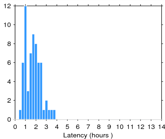
Figure 2. Histogram of the data latency for 02/02/2015. The y-axis denotes the number of files that are made available with a delay of x-hours with respect to the mean time of the records stored in the file.
