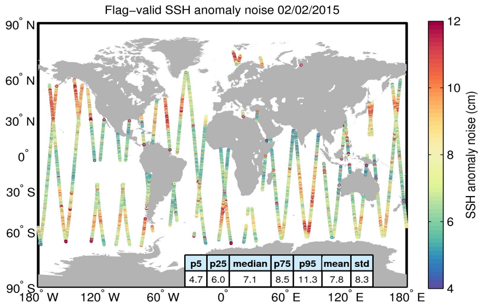
Figure 8. Geographical distribution of flag-valid 20-Hz SSH anomaly measurement noise over oceans and lakes for 02/02/2015. The statistical values shown in the table refer to the SSH anomaly noise and are calculated over all measurements shown in the figure.
