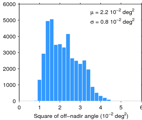
Figure 39. Histogram of flag-valid mispointing over oceans and lakes for 01/02/2015. The mean ( \mu ) and standard deviation ( \sigma ) are also shown. Note that values than 6 \cdot 10^{-2} \text{ deg}^2 are excluded from the histogram for the sake of readability but not from the computation of \mu and \sigma .
