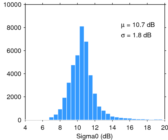
Figure 25. Histogram of flag-valid sigma0 over oceans and lakes for 01/02/2015. The mean ( \mu ) and standard deviation ( \sigma ) are also shown. Note that values outside [4 20] dB are excluded from the histogram for the sake of readability but not from the computation of \mu and \sigma .
