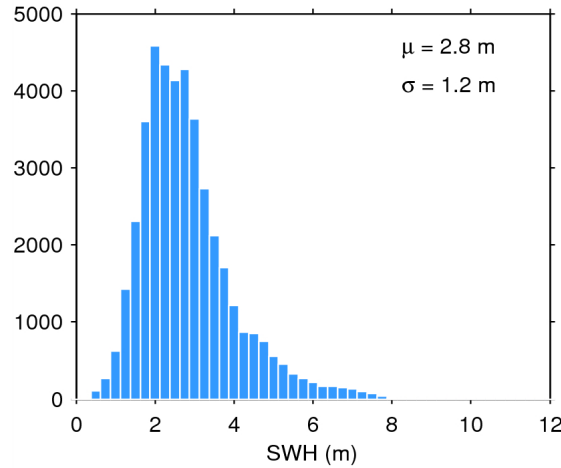
Figure 20. Histogram of science-valid SWH over oceans and lakes for 01/02/2015. The mean ( \mu ) and standard deviation ( \sigma ) are also shown. Note that values larger than 12 m are excluded from the histogram for the sake of readability but not from the computation of \mu and \sigma .
