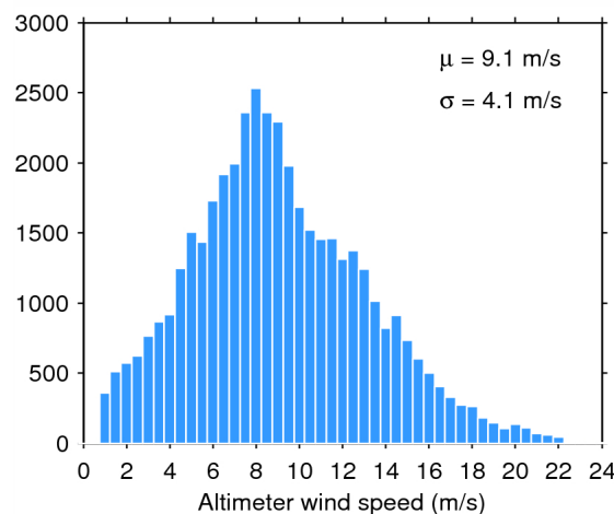
Figure 35. Histogram of science-valid wind over oceans and lakes for 01/02/2015. The mean ( \mu ) and standard deviation ( \sigma ) are also shown. Note that values larger than 24 m/s are excluded from the histogram for the sake of readability but not from the computation of \mu and \sigma .
