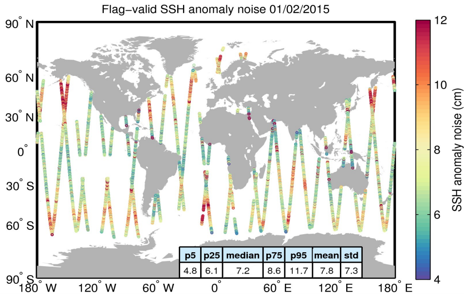
Figure 8. Geographical distribution of flag-valid 20-Hz SSH anomaly measurement noise over oceans and lakes for 01/02/2015. The statistical values shown in the table refer to the SSH anomaly noise and are calculated over all measurements shown in the figure.
