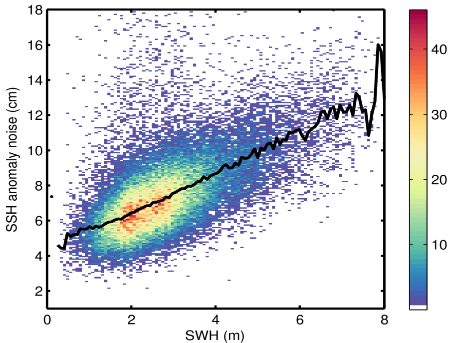
Figure 9. 2D histogram showing flag-valid SSH anomaly noise as a function of SWH for 01/02/2015. The black line denotes the median SSH anomaly as a function of SWH.
