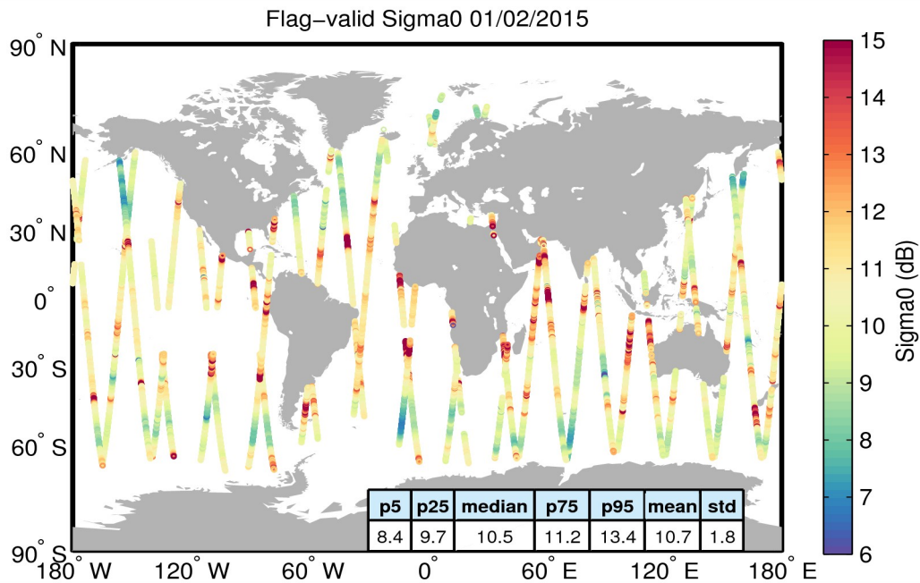
Figure 23. Geographical distribution of flag-valid sigma0 data over oceans and lakes for 01/02/2015. The statistical values shown in the table refer to the sigma0 in dB and are calculated over all measurements shown in the figure.
