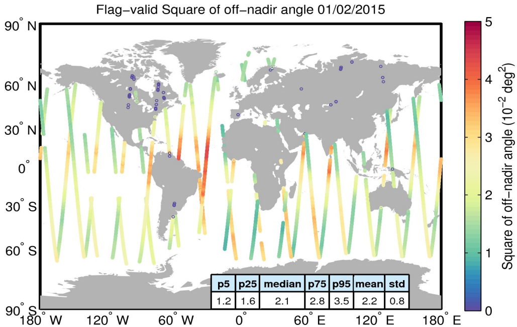
Figure 37. Geographical distribution of flag-valid mispointing data over oceans and lakes for 01/02/2015. The statistical values shown in the table refer to the mispointing in 10^{-2} \text{ deg}^2 and are calculated over all measurements shown in the figure.
