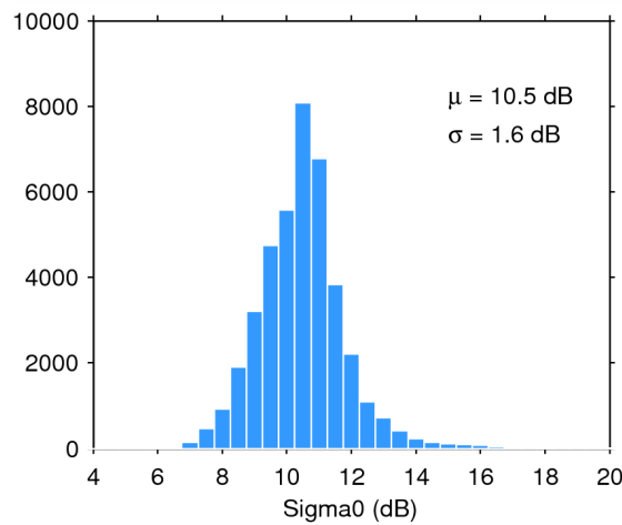
Figure 28. Histogram of science-valid sigma0 over oceans and lakes for 01/02/2015. The mean ( \mu ) and standard deviation ( \sigma ) are also shown. Note that values outside [4 20] dB are excluded from the histogram for the sake of readability but not from the computation of \mu and \sigma .
