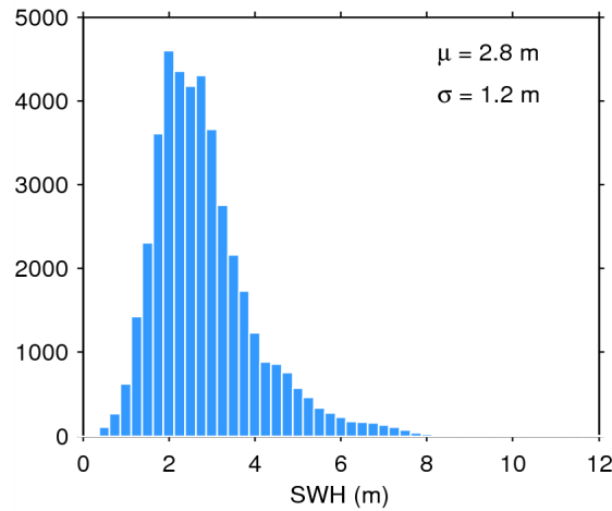
Figure 17. Histogram of flag-valid SWH over oceans and lakes for 01/02/2015. The mean ( \mu ) and standard deviation ( \sigma ) are also shown. Note that values larger than 12 m are excluded from the histogram for the sake of readability but not from the computation of \mu and \sigma .
