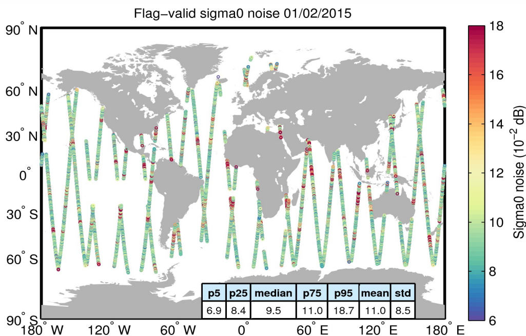
Figure 26. Geographical distribution of flag-valid 20-Hz sigma0 measurement noise over oceans and lakes for 01/02/2015. The statistical values shown in the table refer to the sigma0 noise and are calculated over all measurements shown in the figure.
