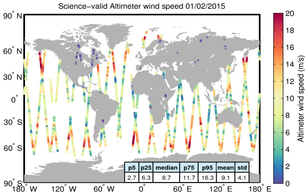
Figure 34. Geographical distribution of science-valid wind data over oceans and lakes for 01/02/2015. The statistical values shown in the table refer to the wind in m/s and are calculated over all measurements shown in the figure. Gray circles denote records that have been rejected based on the editing criteria described in Table 5.
