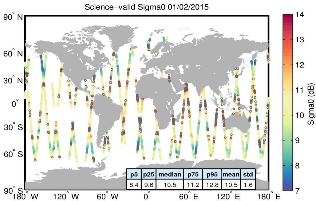
Figure 27. Geographical distribution of science-valid sigma0 data over oceans and lakes for 01/02/2015. The statistical values shown in the table refer to the sigma0 in dB and are calculated over all measurements shown in the figure. Gray circles denote records that have been rejected based on the editing criteria described in Table 4.
