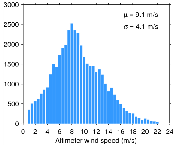
Figure 33. Histogram of flag-valid wind over oceans and lakes for 01/02/2015. The mean ( \mu ) and standard deviation ( \sigma ) are also shown. Note that values larger than 24 m/s are excluded from the histogram for the sake of readability but not from the computation of \mu and \sigma .
