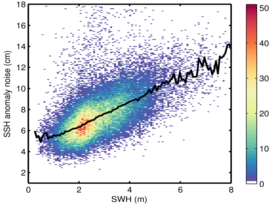
Figure 9. 2D histogram showing flag-valid SSH anomaly noise as a function of SWH for 31/01/2015. The black line denotes the median SSH anomaly as a function of SWH.
