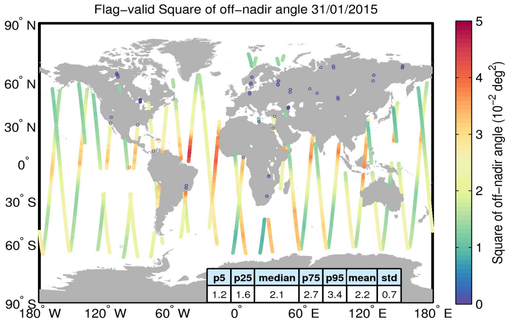
Figure 37. Geographical distribution of flag-valid mispointing data over oceans and lakes for 31/01/2015. The statistical values shown in the table refer to the mispointing in 10^{-2} \text{ deg}^2 and are calculated over all measurements shown in the figure.
