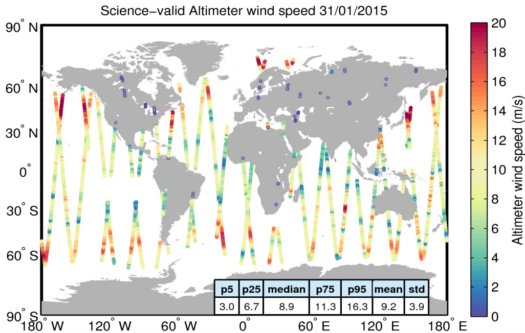
Figure 34. Geographical distribution of science-valid wind data over oceans and lakes for 31/01/2015. The statistical values shown in the table refer to the wind in m/s and are calculated over all measurements shown in the figure. Gray circles denote records that have been rejected based on the editing criteria described in Table 5.
