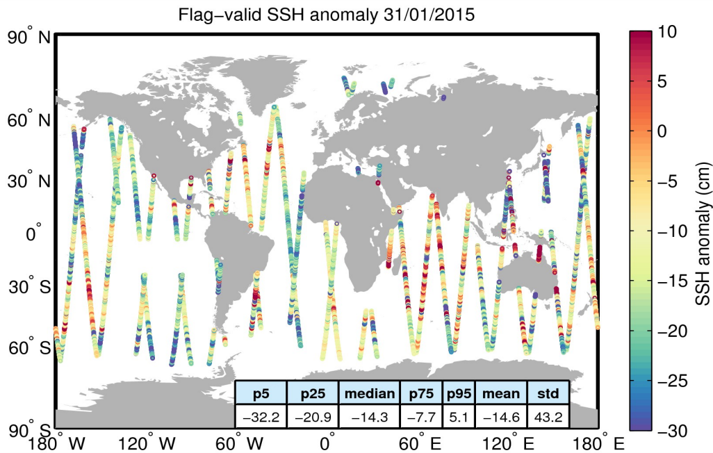
Figure 5. Geographical distribution of flag-valid 1-Hz SSH anomaly data over oceans and lakes for 31/01/2015. The statistical values shown in the table refer to the SSH anomaly in cm and are calculated over all measurements shown in the figure.
