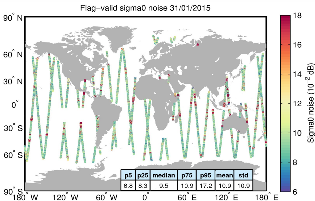
Figure 26. Geographical distribution of flag-valid 20-Hz sigma0 measurement noise over oceans and lakes for 31/01/2015. The statistical values shown in the table refer to the sigma0 noise and are calculated over all measurements shown in the figure.
