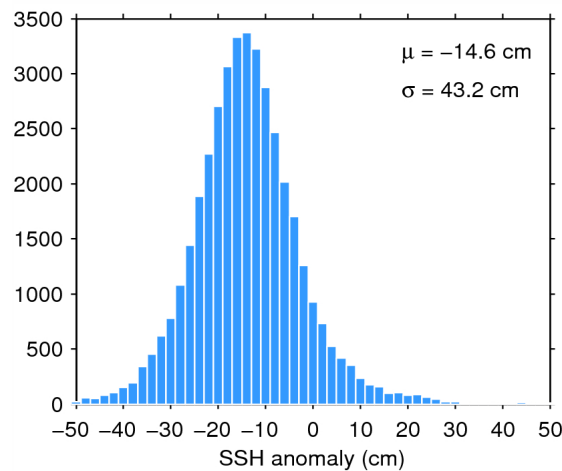
Figure 7. Histogram of flag-valid SSH anomaly over oceans and lakes for 31/01/2015. The mean ( \mu ) and standard deviation ( \sigma ) are also shown. Note that values outside [-50\ 50] cm are excluded from the histogram for the sake of readability but not from the computation of \mu and \sigma .
