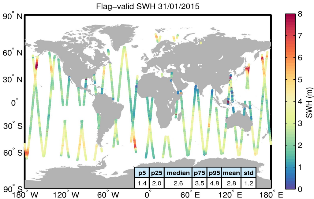
Figure 15. Geographical distribution of flag-valid SWH data over oceans and lakes for 31/01/2015. The statistical values shown in the table refer to the SWH in m and are calculated over all measurements shown in the figure.
