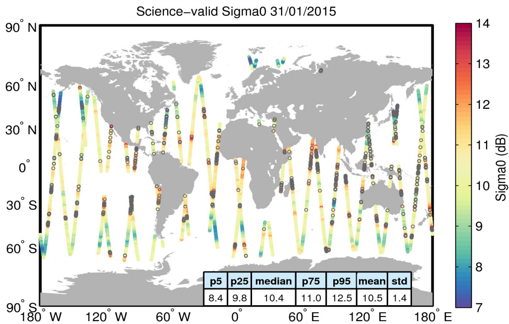
Figure 27. Geographical distribution of science-valid sigma0 data over oceans and lakes for 31/01/2015. The statistical values shown in the table refer to the sigma0 in dB and are calculated over all measurements shown in the figure. Gray circles denote records that have been rejected based on the editing criteria described in Table 4.
