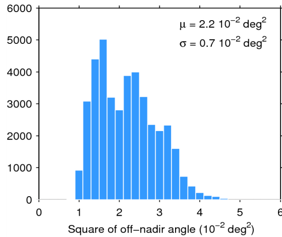
Figure 39. Histogram of flag-valid mispointing over oceans and lakes for 31/01/2015. The mean ( \mu ) and standard deviation ( \sigma ) are also shown. Note that values than 6 \cdot 10^{-2} \text{ deg}^2 are excluded from the histogram for the sake of readability but not from the computation of \mu and \sigma .
