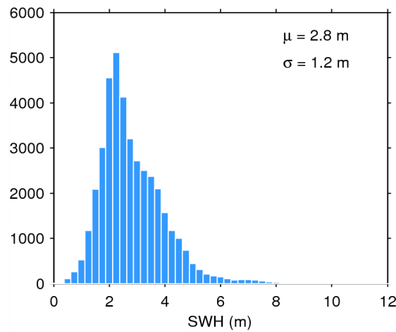
Figure 17. Histogram of flag-valid SWH over oceans and lakes for 31/01/2015. The mean ( \mu ) and standard deviation ( \sigma ) are also shown. Note that values larger than 12 m are excluded from the histogram for the sake of readability but not from the computation of \mu and \sigma .
