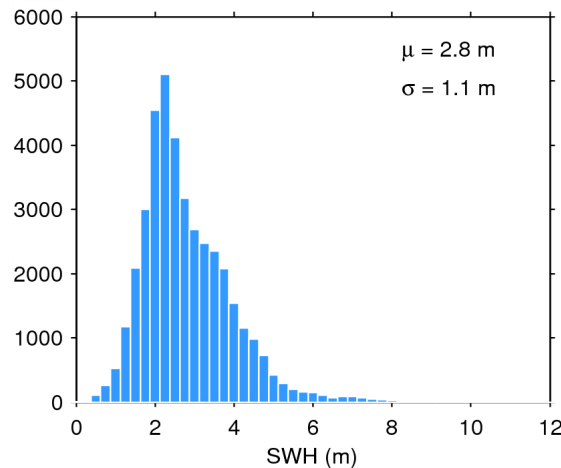
Figure 20. Histogram of science-valid SWH over oceans and lakes for 31/01/2015. The mean ( \mu ) and standard deviation ( \sigma ) are also shown. Note that values larger than 12 m are excluded from the histogram for the sake of readability but not from the computation of \mu and \sigma .
