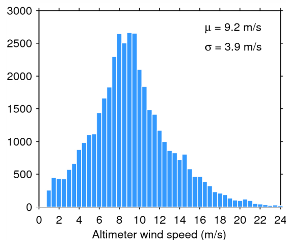
Figure 35. Histogram of science-valid wind over oceans and lakes for 31/01/2015. The mean ( \mu ) and standard deviation ( \sigma ) are also shown. Note that values larger than 24 m/s are excluded from the histogram for the sake of readability but not from the computation of \mu and \sigma .
