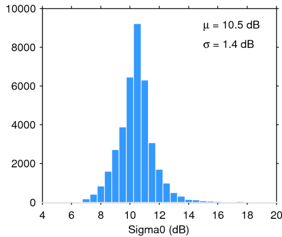
Figure 28. Histogram of science-valid sigma0 over oceans and lakes for 31/01/2015. The mean ( \mu ) and standard deviation ( \sigma ) are also shown. Note that values outside [4 20] dB are excluded from the histogram for the sake of readability but not from the computation of \mu and \sigma .
