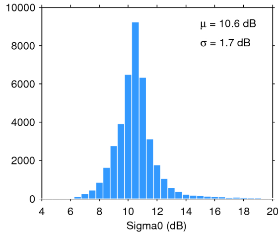
Figure 25. Histogram of flag-valid sigma0 over oceans and lakes for 31/01/2015. The mean ( \mu ) and standard deviation ( \sigma ) are also shown. Note that values outside [4 20] dB are excluded from the histogram for the sake of readability but not from the computation of \mu and \sigma .
