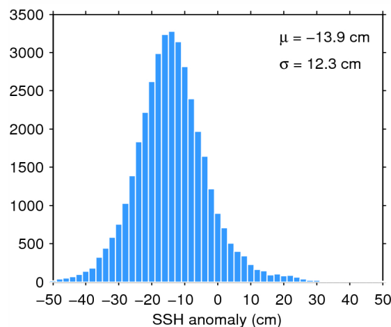
Figure 11. Histogram of science-valid SSH anomaly over oceans and lakes for 31/01/2015. The mean ( \mu ) and standard deviation ( \sigma ) are also shown. Note that values outside [-50 50] cm are excluded from the histogram for the sake of readability but not from the computation of \mu and \sigma .
