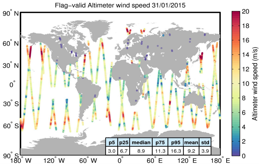
Figure 31. Geographical distribution of flag-valid wind data over oceans and lakes for 31/01/2015. The statistical values shown in the table refer to the wind in m/s and are calculated over all measurements shown in the figure.
