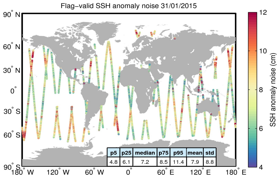
Figure 8. Geographical distribution of flag-valid 20-Hz SSH anomaly measurement noise over oceans and lakes for 31/01/2015. The statistical values shown in the table refer to the SSH anomaly noise and are calculated over all measurements shown in the figure.
