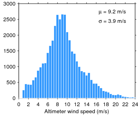
Figure 33. Histogram of flag-valid wind over oceans and lakes for 31/01/2015. The mean ( \mu ) and standard deviation ( \sigma ) are also shown. Note that values larger than 24 m/s are excluded from the histogram for the sake of readability but not from the computation of \mu and \sigma .
