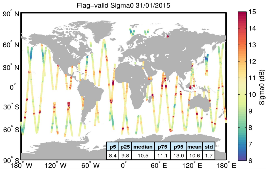
Figure 23. Geographical distribution of flag-valid sigma0 data over oceans and lakes for 31/01/2015. The statistical values shown in the table refer to the sigma0 in dB and are calculated over all measurements shown in the figure.
