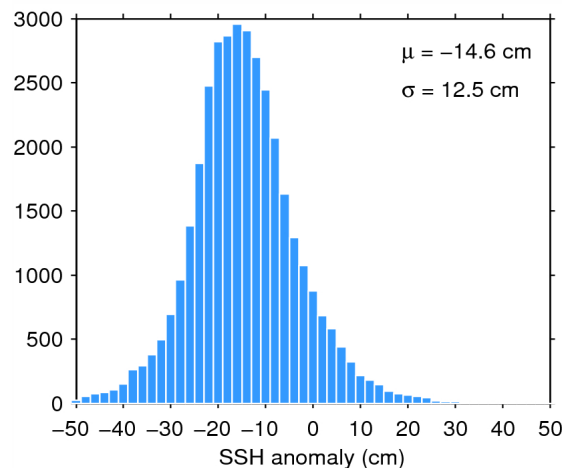
Figure 11. Histogram of science-valid SSH anomaly over oceans and lakes for 29/01/2015. The mean ( \mu ) and standard deviation ( \sigma ) are also shown. Note that values outside [-50 50] cm are excluded from the histogram for the sake of readability but not from the computation of \mu and \sigma .
