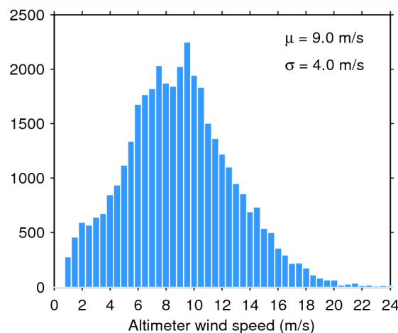
Figure 35. Histogram of science-valid wind over oceans and lakes for 29/01/2015. The mean ( \mu ) and standard deviation ( \sigma ) are also shown. Note that values larger than 24 m/s are excluded from the histogram for the sake of readability but not from the computation of \mu and \sigma .
