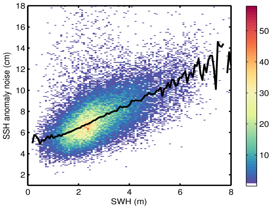
Figure 9. 2D histogram showing flag-valid SSH anomaly noise as a function of SWH for 29/01/2015. The black line denotes the median SSH anomaly as a function of SWH.
