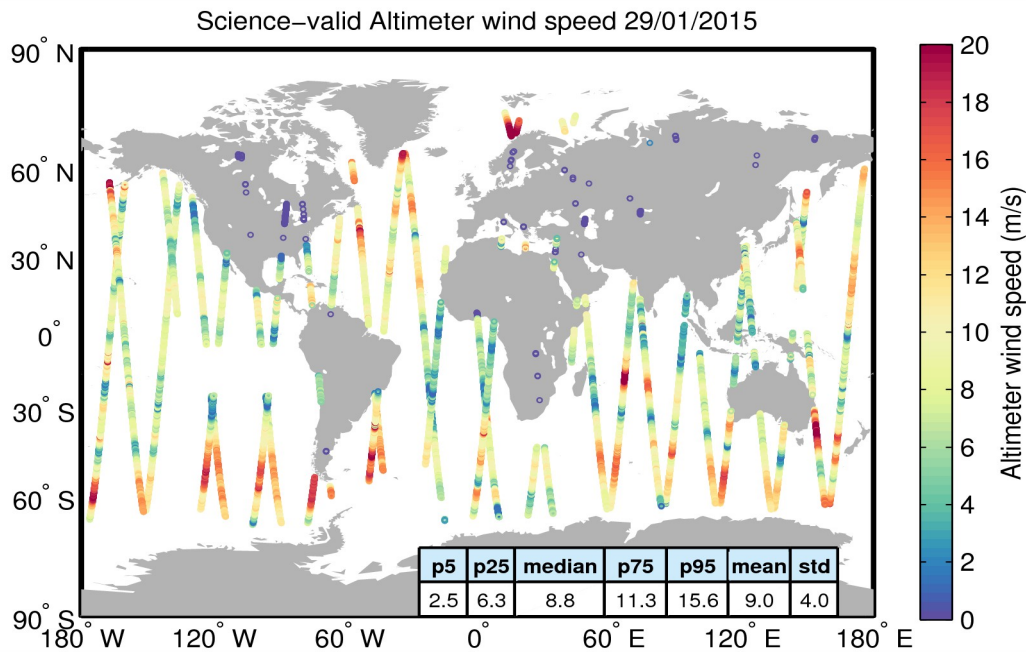
Figure 34. Geographical distribution of science-valid wind data over oceans and lakes for 29/01/2015. The statistical values shown in the table refer to the wind in m/s and are calculated over all measurements shown in the figure. Gray circles denote records that have been rejected based on the editing criteria described in Table 5.
