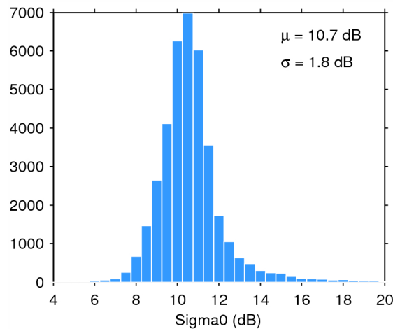
Figure 25. Histogram of flag-valid sigma0 over oceans and lakes for 29/01/2015. The mean ( \mu ) and standard deviation ( \sigma ) are also shown. Note that values outside [4 20] dB are excluded from the histogram for the sake of readability but not from the computation of \mu and \sigma .
