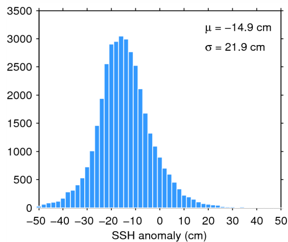
Figure 7. Histogram of flag-valid SSH anomaly over oceans and lakes for 29/01/2015. The mean ( \mu ) and standard deviation ( \sigma ) are also shown. Note that values outside [-50\ 50] cm are excluded from the histogram for the sake of readability but not from the computation of \mu and \sigma .
