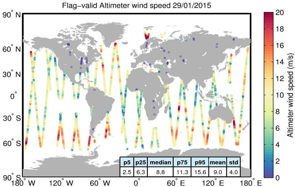
Figure 31. Geographical distribution of flag-valid wind data over oceans and lakes for 29/01/2015. The statistical values shown in the table refer to the wind in m/s and are calculated over all measurements shown in the figure.
