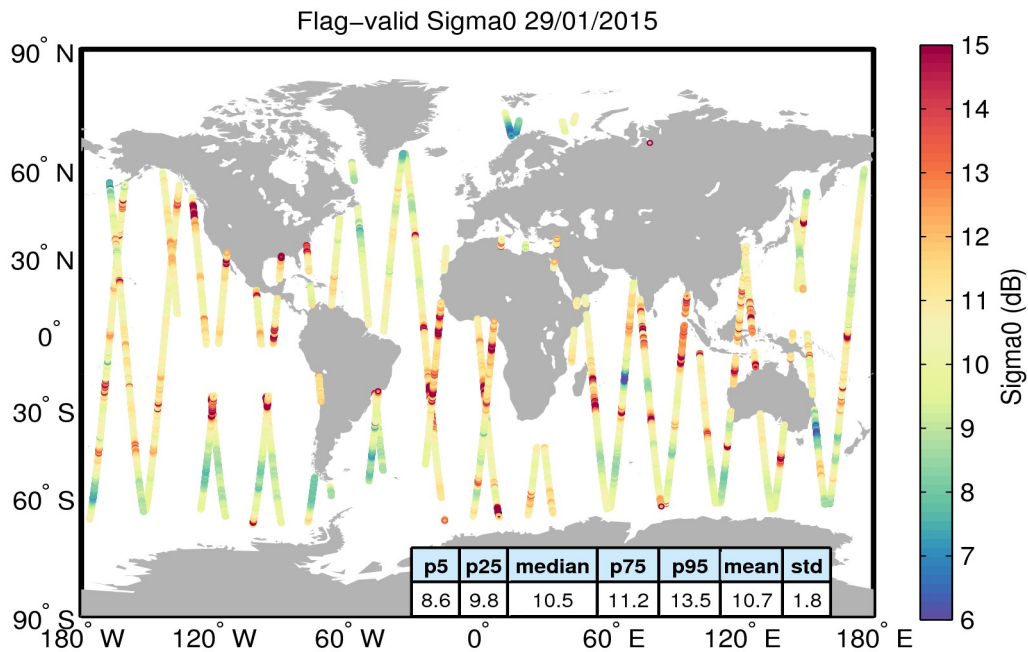
Figure 23. Geographical distribution of flag-valid sigma0 data over oceans and lakes for 29/01/2015. The statistical values shown in the table refer to the sigma0 in dB and are calculated over all measurements shown in the figure.
