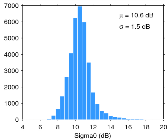
Figure 28. Histogram of science-valid sigma0 over oceans and lakes for 29/01/2015. The mean ( \mu ) and standard deviation ( \sigma ) are also shown. Note that values outside [4 20] dB are excluded from the histogram for the sake of readability but not from the computation of \mu and \sigma .
