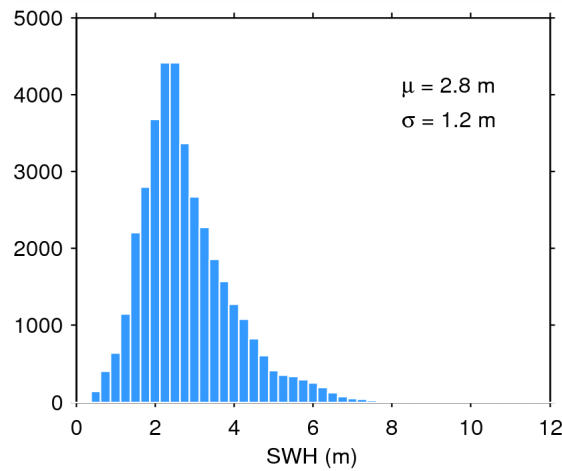
Figure 17. Histogram of flag-valid SWH over oceans and lakes for 29/01/2015. The mean ( \mu ) and standard deviation ( \sigma ) are also shown. Note that values larger than 12 m are excluded from the histogram for the sake of readability but not from the computation of \mu and \sigma .
