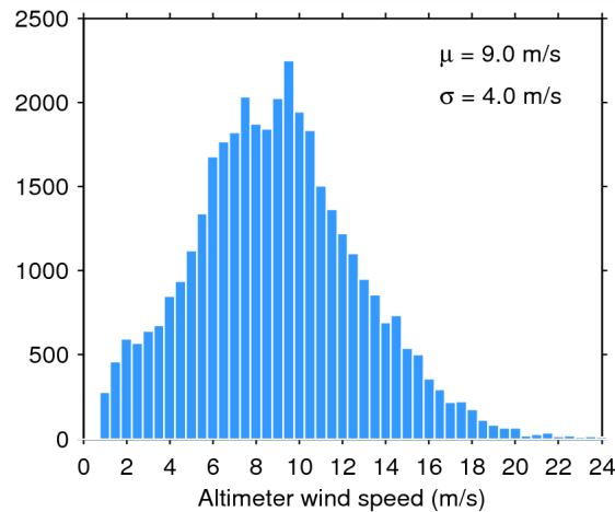
Figure 33. Histogram of flag-valid wind over oceans and lakes for 29/01/2015. The mean ( \mu ) and standard deviation ( \sigma ) are also shown. Note that values larger than 24 m/s are excluded from the histogram for the sake of readability but not from the computation of \mu and \sigma .
