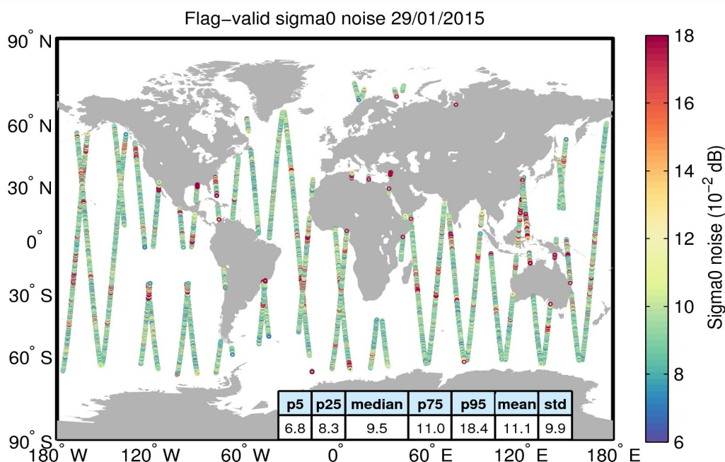
Figure 26. Geographical distribution of flag-valid 20-Hz sigma0 measurement noise over oceans and lakes for 29/01/2015. The statistical values shown in the table refer to the sigma0 noise and are calculated over all measurements shown in the figure.
