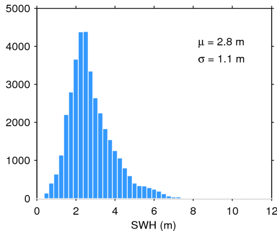
Figure 20. Histogram of science-valid SWH over oceans and lakes for 29/01/2015. The mean ( \mu ) and standard deviation ( \sigma ) are also shown. Note that values larger than 12 m are excluded from the histogram for the sake of readability but not from the computation of \mu and \sigma .
