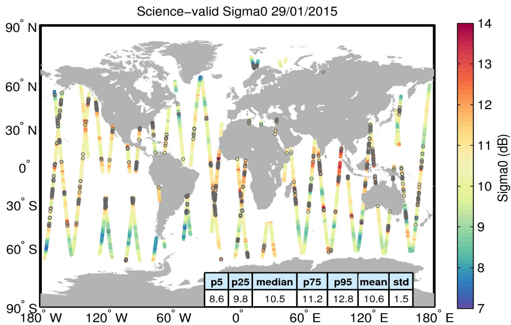
Figure 27. Geographical distribution of science-valid sigma0 data over oceans and lakes for 29/01/2015. The statistical values shown in the table refer to the sigma0 in dB and are calculated over all measurements shown in the figure. Gray circles denote records that have been rejected based on the editing criteria described in Table 4.
