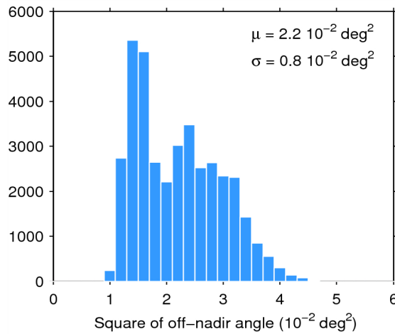
Figure 39. Histogram of flag-valid mispointing over oceans and lakes for 29/01/2015. The mean ( \mu ) and standard deviation ( \sigma ) are also shown. Note that values than 6 \cdot 10^{-2} \text{ deg}^2 are excluded from the histogram for the sake of readability but not from the computation of \mu and \sigma .
