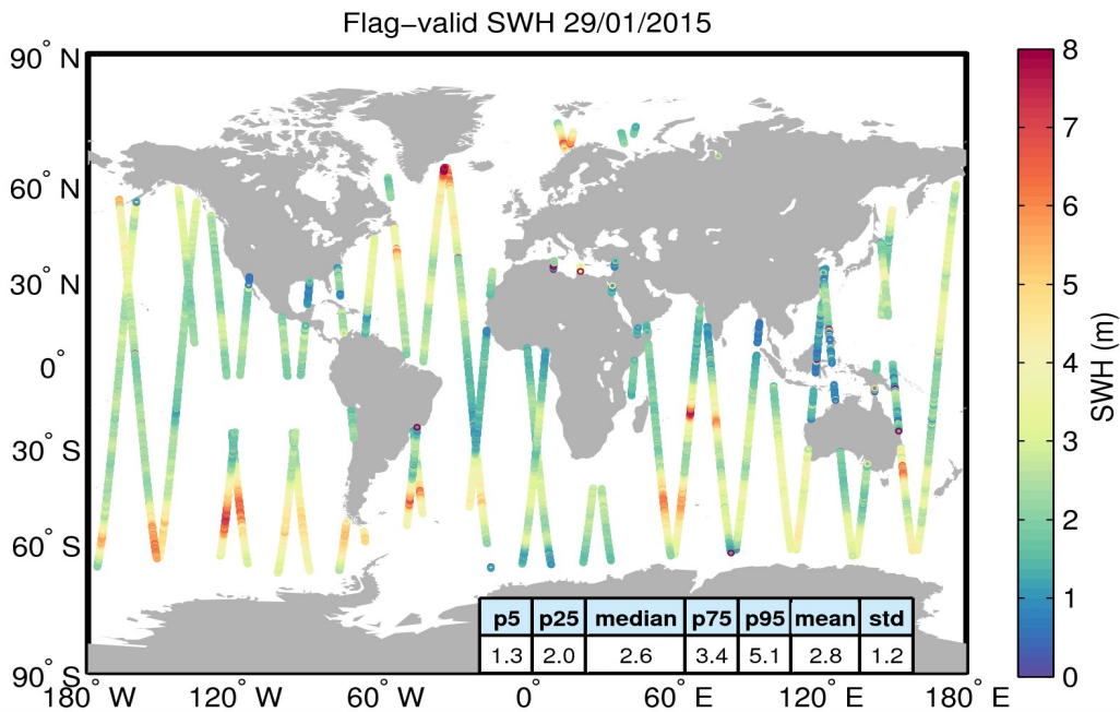
Figure 15. Geographical distribution of flag-valid SWH data over oceans and lakes for 29/01/2015. The statistical values shown in the table refer to the SWH in m and are calculated over all measurements shown in the figure.
