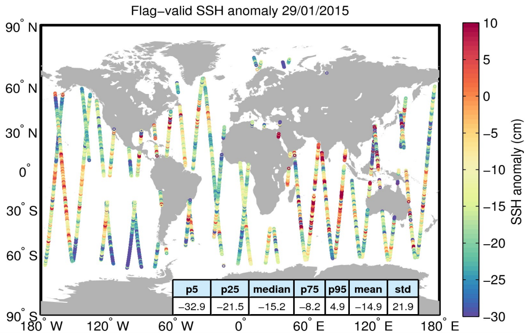
Figure 5. Geographical distribution of flag-valid 1-Hz SSH anomaly data over oceans and lakes for 29/01/2015. The statistical values shown in the table refer to the SSH anomaly in cm and are calculated over all measurements shown in the figure.
