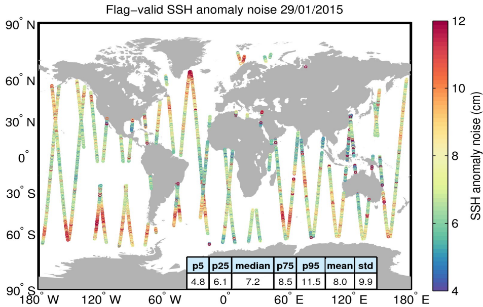
Figure 8. Geographical distribution of flag-valid 20-Hz SSH anomaly measurement noise over oceans and lakes for 29/01/2015. The statistical values shown in the table refer to the SSH anomaly noise and are calculated over all measurements shown in the figure.
