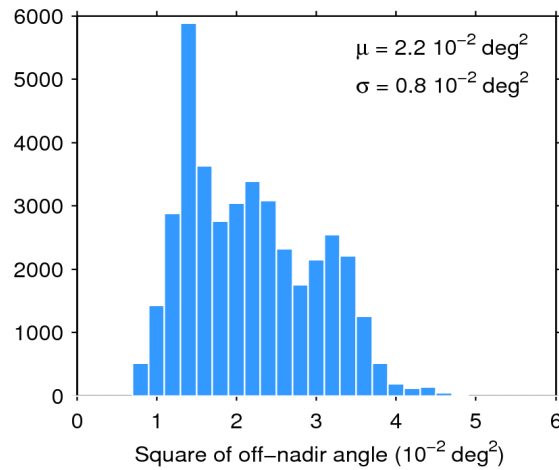
Figure 39. Histogram of flag-valid mispointing over oceans and lakes for 25/01/2015. The mean ( \mu ) and standard deviation ( \sigma ) are also shown. Note that values than 6 \cdot 10^{-2} \text{ deg}^2 are excluded from the histogram for the sake of readability but not from the computation of \mu and \sigma .
