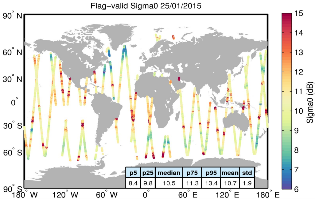
Figure 23. Geographical distribution of flag-valid sigma0 data over oceans and lakes for 25/01/2015. The statistical values shown in the table refer to the sigma0 in dB and are calculated over all measurements shown in the figure.
