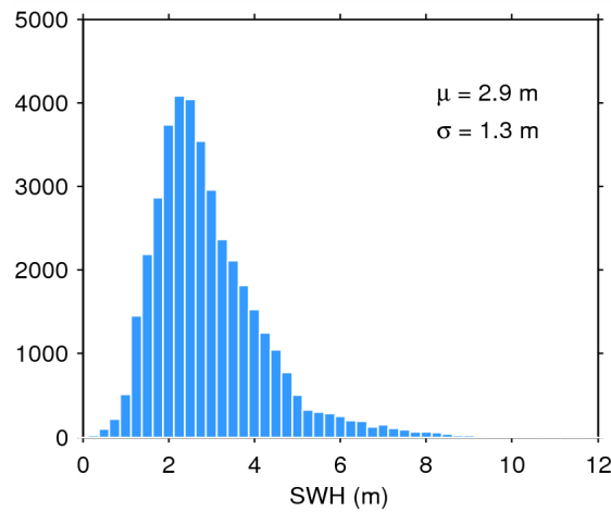
Figure 17. Histogram of flag-valid SWH over oceans and lakes for 25/01/2015. The mean ( \mu ) and standard deviation ( \sigma ) are also shown. Note that values larger than 12 m are excluded from the histogram for the sake of readability but not from the computation of \mu and \sigma .
