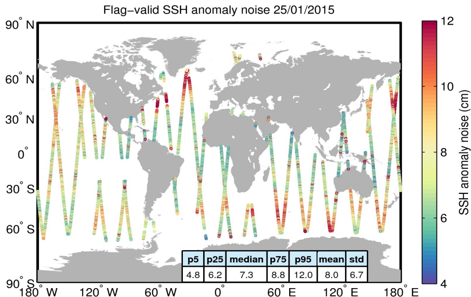
Figure 8. Geographical distribution of flag-valid 20-Hz SSH anomaly measurement noise over oceans and lakes for 25/01/2015. The statistical values shown in the table refer to the SSH anomaly noise and are calculated over all measurements shown in the figure.
