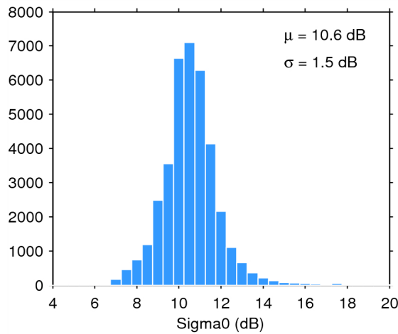
Figure 28. Histogram of science-valid sigma0 over oceans and lakes for 25/01/2015. The mean ( \mu ) and standard deviation ( \sigma ) are also shown. Note that values outside [4 20] dB are excluded from the histogram for the sake of readability but not from the computation of \mu and \sigma .
