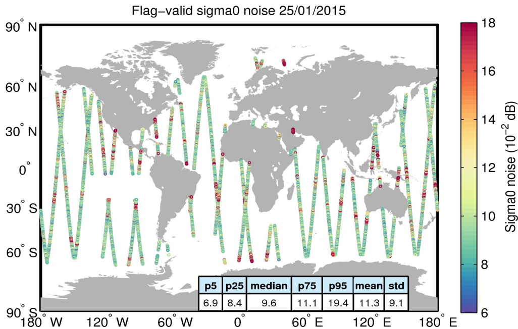
Figure 26. Geographical distribution of flag-valid 20-Hz sigma0 measurement noise over oceans and lakes for 25/01/2015. The statistical values shown in the figure refer to the sigma0 noise and are calculated over all measurements shown in the figure.
