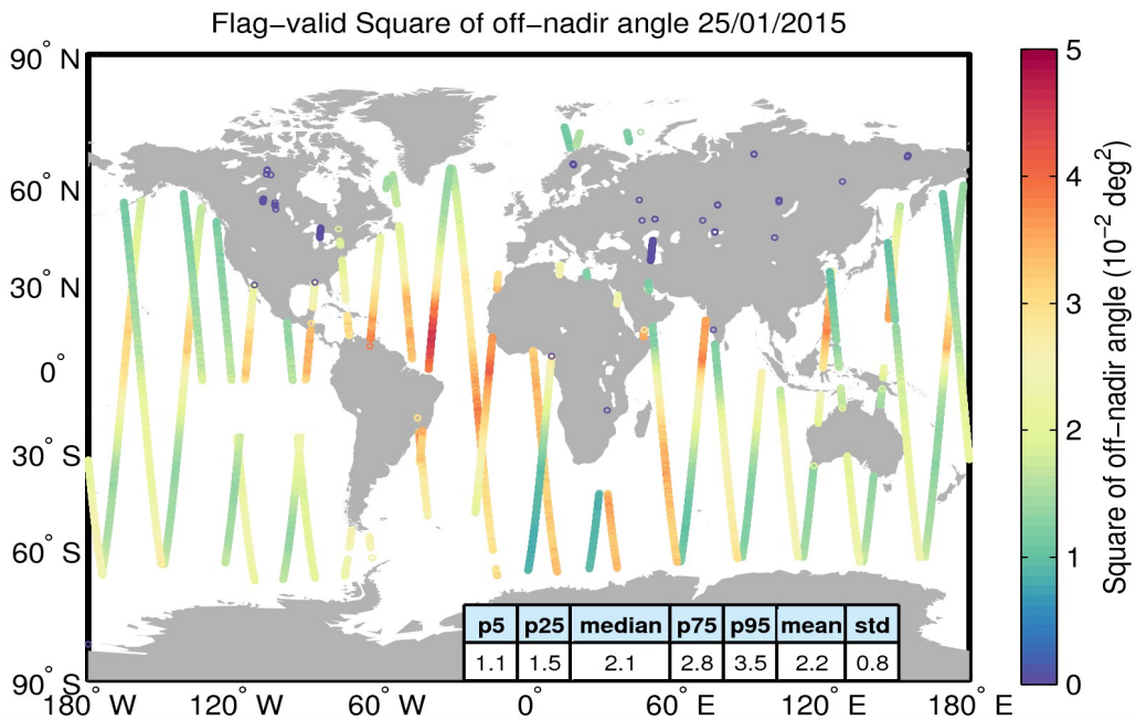
Figure 37. Geographical distribution of flag-valid mispointing data over oceans and lakes for 25/01/2015. The statistical values shown in the table refer to the mispointing in 10^{-2} \text{ deg}^2 and are calculated over all measurements shown in the figure.
