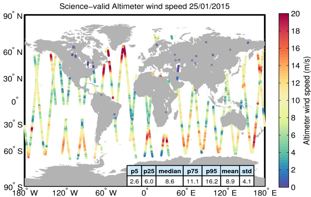
Figure 34. Geographical distribution of science-valid wind data over oceans and lakes for 25/01/2015. The statistical values shown in the table refer to the wind in m/s and are calculated over all measurements shown in the figure. Gray circles denote records that have been rejected based on the editing criteria described in Table 5.
