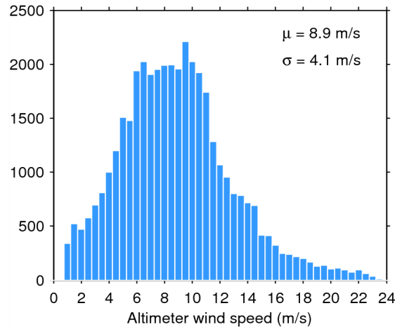
Figure 33. Histogram of flag-valid wind over oceans and lakes for 25/01/2015. The mean ( \mu ) and standard deviation ( \sigma ) are also shown. Note that values larger than 24 m/s are excluded from the histogram for the sake of readability but not from the computation of \mu and \sigma .
