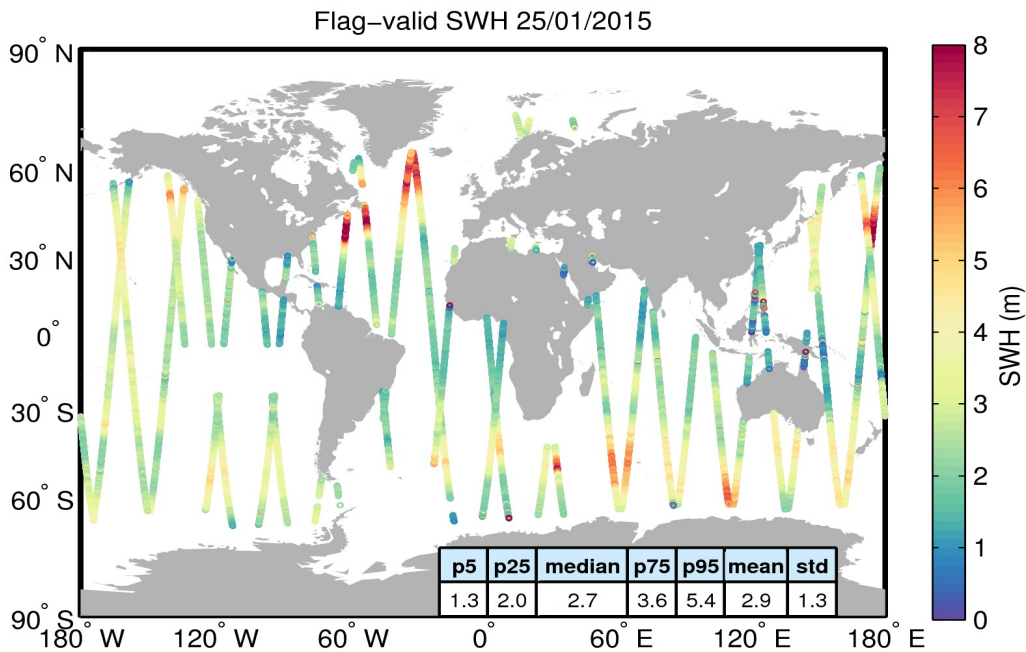
Figure 15. Geographical distribution of flag-valid SWH data over oceans and lakes for 25/01/2015. The statistical values shown in the table refer to the SWH in m and are calculated over all measurements shown in the figure.
