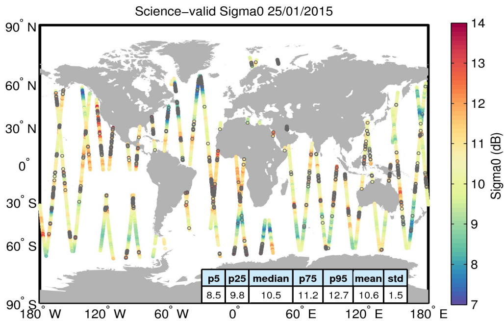
Figure 27. Geographical distribution of science-valid sigma0 data over oceans and lakes for 25/01/2015. The statistical values shown in the table refer to the sigma0 in dB and are calculated over all measurements shown in the figure. Gray circles denote records that have been rejected based on the editing criteria described in Table 4.
