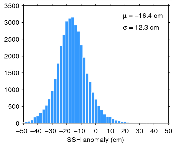
Figure 11. Histogram of science-valid SSH anomaly over oceans and lakes for 25/01/2015. The mean ( \mu ) and standard deviation ( \sigma ) are also shown. Note that values outside [-50 50] cm are excluded from the histogram for the sake of readability but not from the computation of \mu and \sigma .
