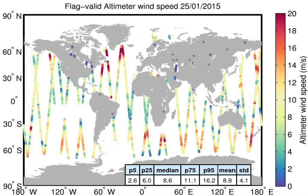
Figure 31. Geographical distribution of flag-valid wind data over oceans and lakes for 25/01/2015. The statistical values shown in the table refer to the wind in m/s and are calculated over all measurements shown in the figure.
