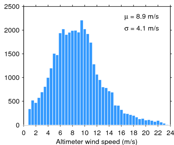
Figure 35. Histogram of science-valid wind over oceans and lakes for 25/01/2015. The mean ( \mu ) and standard deviation ( \sigma ) are also shown. Note that values larger than 24 m/s are excluded from the histogram for the sake of readability but not from the computation of \mu and \sigma .
