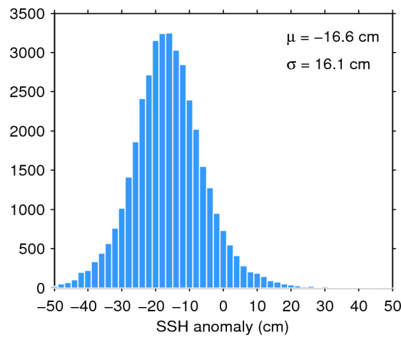
Figure 7. Histogram of flag-valid SSH anomaly over oceans and lakes for 25/01/2015. The mean ( \mu ) and standard deviation ( \sigma ) are also shown. Note that values outside [-50\ 50] cm are excluded from the histogram for the sake of readability but not from the computation of \mu and \sigma .
