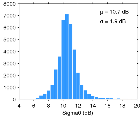
Figure 25. Histogram of flag-valid sigma0 over oceans and lakes for 25/01/2015. The mean ( \mu ) and standard deviation ( \sigma ) are also shown. Note that values outside [4 20] dB are excluded from the histogram for the sake of readability but not from the computation of \mu and \sigma .
