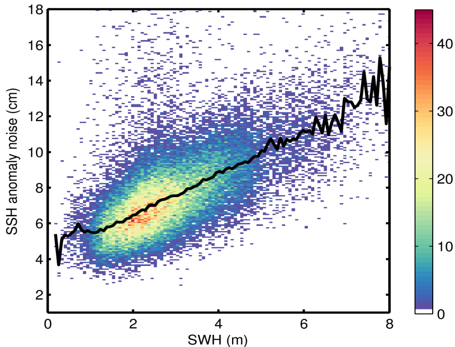
Figure 9. 2D histogram showing flag-valid SSH anomaly noise as a function of SWH for 25/01/2015. The black line denotes the median SSH anomaly as a function of SWH.
