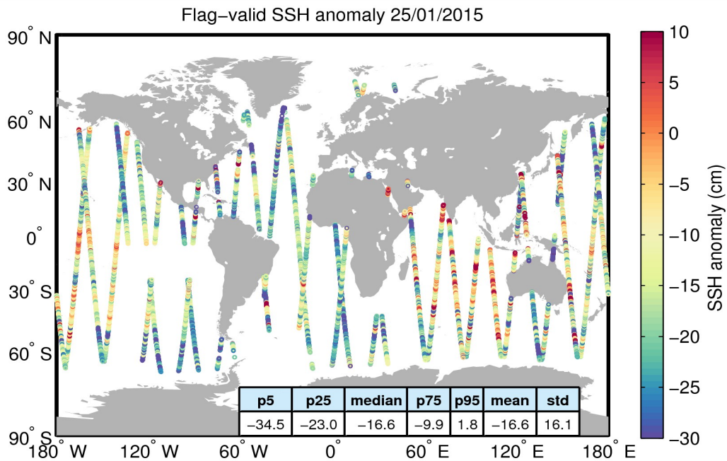
Figure 5. Geographical distribution of flag-valid 1-Hz SSH anomaly data over oceans and lakes for 25/01/2015. The statistical values shown in the table refer to the SSH anomaly in cm and are calculated over all measurements shown in the figure.
