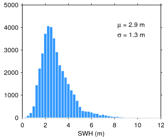
Figure 20. Histogram of science-valid SWH over oceans and lakes for 25/01/2015. The mean ( \mu ) and standard deviation ( \sigma ) are also shown. Note that values larger than 12 m are excluded from the histogram for the sake of readability but not from the computation of \mu and \sigma .
