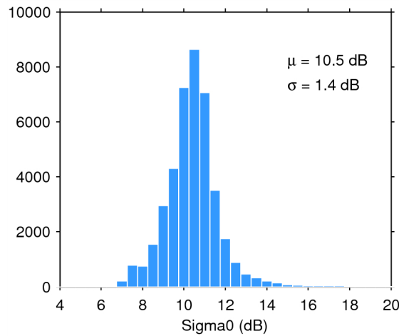
Figure 28. Histogram of science-valid sigma0 over oceans and lakes for 24/01/2015. The mean ( \mu ) and standard deviation ( \sigma ) are also shown. Note that values outside [4 20] dB are excluded from the histogram for the sake of readability but not from the computation of \mu and \sigma .
