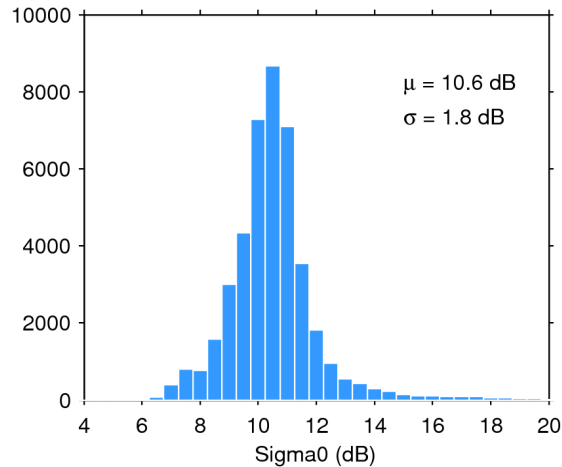
Figure 25. Histogram of flag-valid sigma0 over oceans and lakes for 24/01/2015. The mean ( \mu ) and standard deviation ( \sigma ) are also shown. Note that values outside [4 20] dB are excluded from the histogram for the sake of readability but not from the computation of \mu and \sigma .
