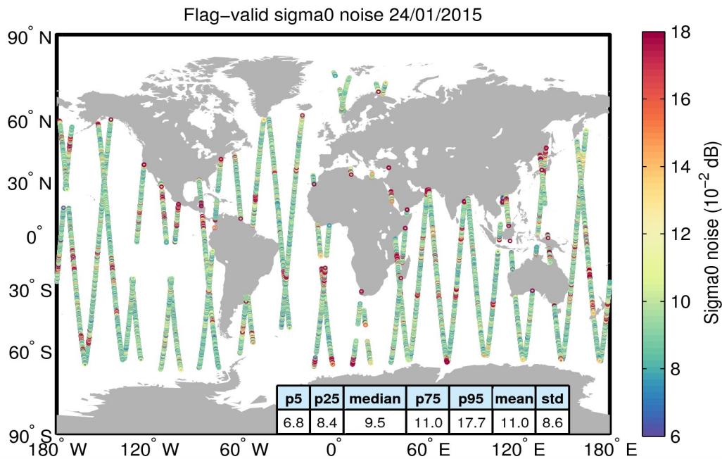
Figure 26. Geographical distribution of flag-valid 20-Hz sigma0 measurement noise over oceans and lakes for 24/01/2015. The statistical values shown in the table refer to the sigma0 noise and are calculated over all measurements shown in the figure.
