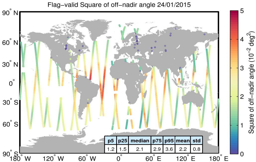
Figure 37. Geographical distribution of flag-valid mispointing data over oceans and lakes for 24/01/2015. The statistical values shown in the table refer to the mispointing in 10^{-2} \text{ deg}^2 and are calculated over all measurements shown in the figure.
