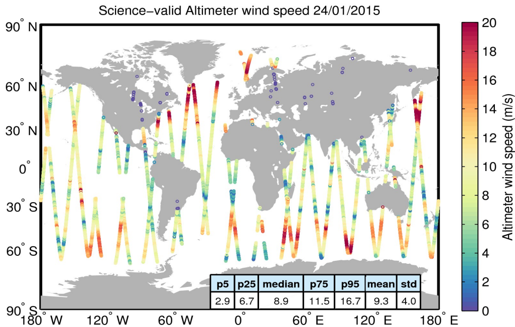
Figure 34. Geographical distribution of science-valid wind data over oceans and lakes for 24/01/2015. The statistical values shown in the table refer to the wind in m/s and are calculated over all measurements shown in the figure. Gray circles denote records that have been rejected based on the editing criteria described in Table 5.
