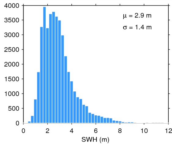
Figure 17. Histogram of flag-valid SWH over oceans and lakes for 24/01/2015. The mean ( \mu ) and standard deviation ( \sigma ) are also shown. Note that values larger than 12 m are excluded from the histogram for the sake of readability but not from the computation of \mu and \sigma .
