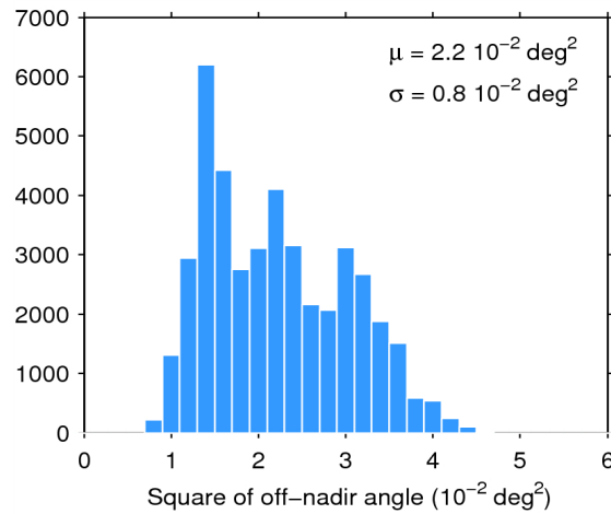
Figure 39. Histogram of flag-valid mispointing over oceans and lakes for 24/01/2015. The mean ( \mu ) and standard deviation ( \sigma ) are also shown. Note that values than 6 \cdot 10^{-2} \text{ deg}^2 are excluded from the histogram for the sake of readability but not from the computation of \mu and \sigma .
