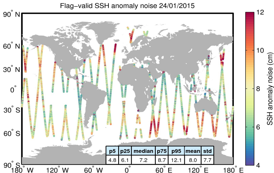
Figure 8. Geographical distribution of flag-valid 20-Hz SSH anomaly measurement noise over oceans and lakes for 24/01/2015. The statistical values shown in the table refer to the SSH anomaly noise and are calculated over all measurements shown in the figure.
