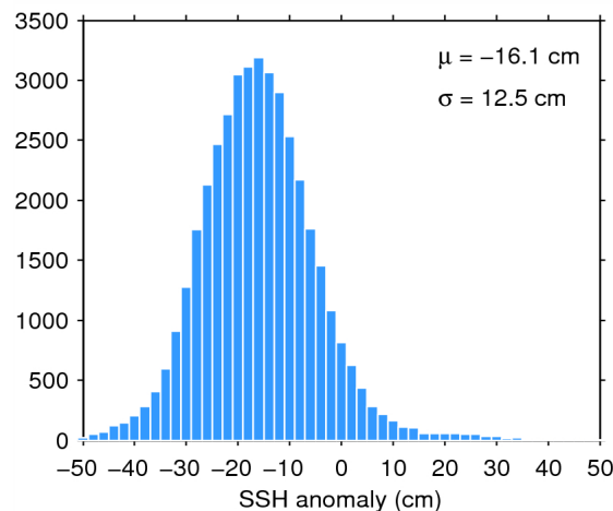
Figure 11. Histogram of science-valid SSH anomaly over oceans and lakes for 24/01/2015. The mean ( \mu ) and standard deviation ( \sigma ) are also shown. Note that values outside [-50 50] cm are excluded from the histogram for the sake of readability but not from the computation of \mu and \sigma .
