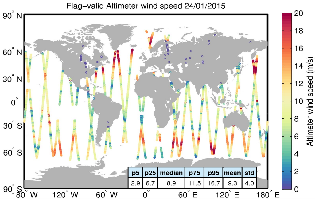
Figure 31. Geographical distribution of flag-valid wind data over oceans and lakes for 24/01/2015. The statistical values shown in the table refer to the wind in m/s and are calculated over all measurements shown in the figure.
