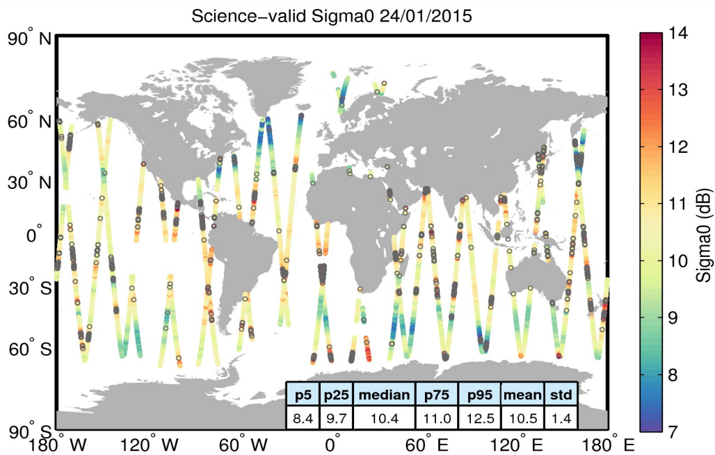
Figure 27. Geographical distribution of science-valid sigma0 data over oceans and lakes for 24/01/2015. The statistical values shown in the table refer to the sigma0 in dB and are calculated over all measurements shown in the figure. Gray circles denote records that have been rejected based on the editing criteria described in Table 4.
