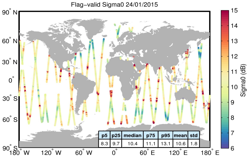
Figure 23. Geographical distribution of flag-valid sigma0 data over oceans and lakes for 24/01/2015. The statistical values shown in the table refer to the sigma0 in dB and are calculated over all measurements shown in the figure.
