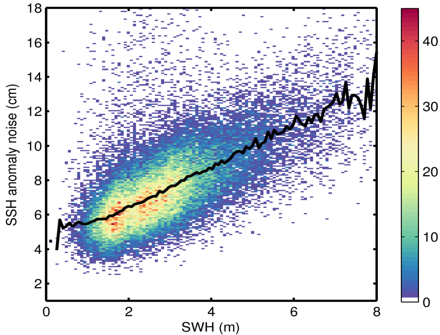
Figure 9. 2D histogram showing flag-valid SSH anomaly noise as a function of SWH for 24/01/2015. The black line denotes the median SSH anomaly as a function of SWH.
