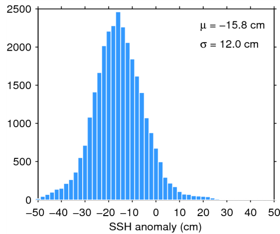
Figure 11. Histogram of science-valid SSH anomaly over oceans and lakes for 19/01/2015. The mean ( \mu ) and standard deviation ( \sigma ) are also shown. Note that values outside [-50 50] cm are excluded from the histogram for the sake of readability but not from the computation of \mu and \sigma .
