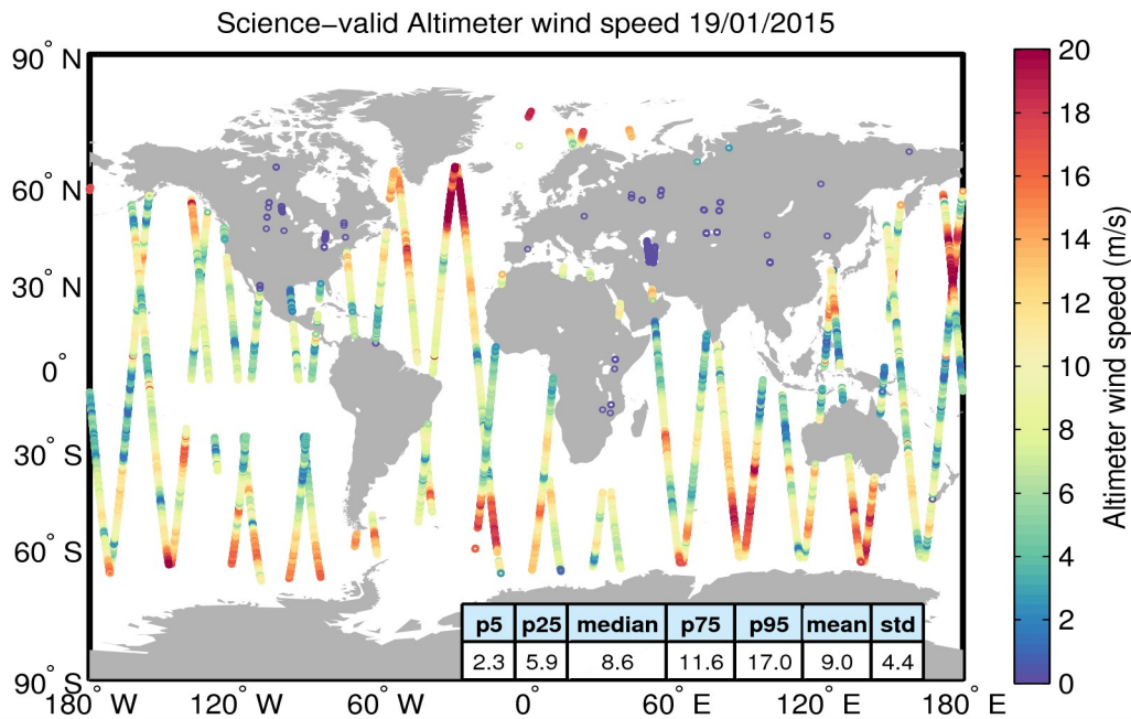
Figure 34. Geographical distribution of science-valid wind data over oceans and lakes for 19/01/2015. The statistical values shown in the table refer to the wind in m/s and are calculated over all measurements shown in the figure. Gray circles denote records that have been rejected based on the editing criteria described in Table 5.
