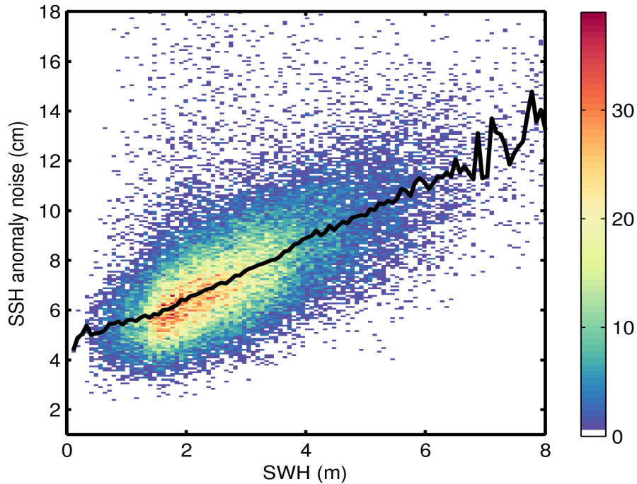
Figure 9. 2D histogram showing flag-valid SSH anomaly noise as a function of SWH for 19/01/2015. The black line denotes the median SSH anomaly as a function of SWH.
