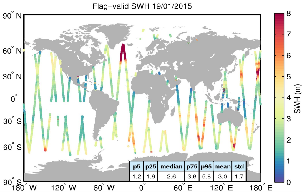
Figure 15. Geographical distribution of flag-valid SWH data over oceans and lakes for 19/01/2015. The statistical values shown in the table refer to the SWH in m and are calculated over all measurements shown in the figure.
