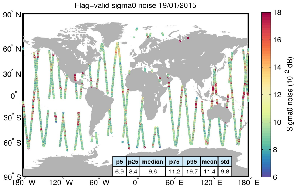
Figure 26. Geographical distribution of flag-valid 20-Hz sigma0 measurement noise over oceans and lakes for 19/01/2015. The statistical values shown in the table refer to the sigma0 noise and are calculated over all measurements shown in the figure.
