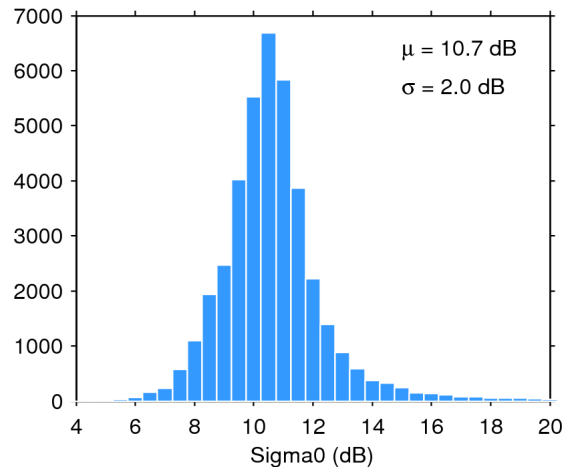
Figure 25. Histogram of flag-valid sigma0 over oceans and lakes for 19/01/2015. The mean ( \mu ) and standard deviation ( \sigma ) are also shown. Note that values outside [4 20] dB are excluded from the histogram for the sake of readability but not from the computation of \mu and \sigma .
