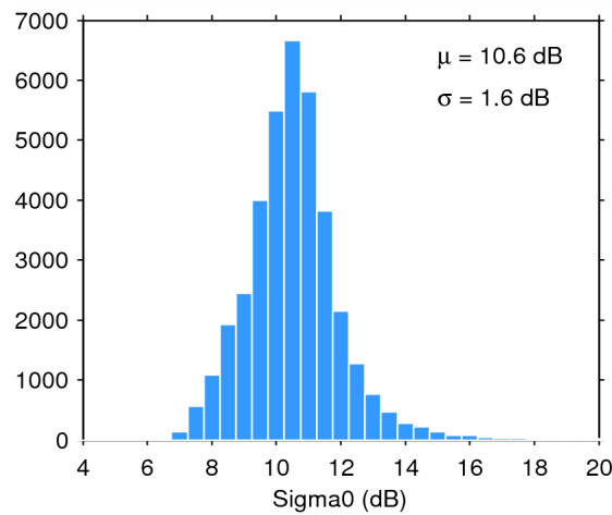
Figure 28. Histogram of science-valid sigma0 over oceans and lakes for 19/01/2015. The mean ( \mu ) and standard deviation ( \sigma ) are also shown. Note that values outside [4 20] dB are excluded from the histogram for the sake of readability but not from the computation of \mu and \sigma .
