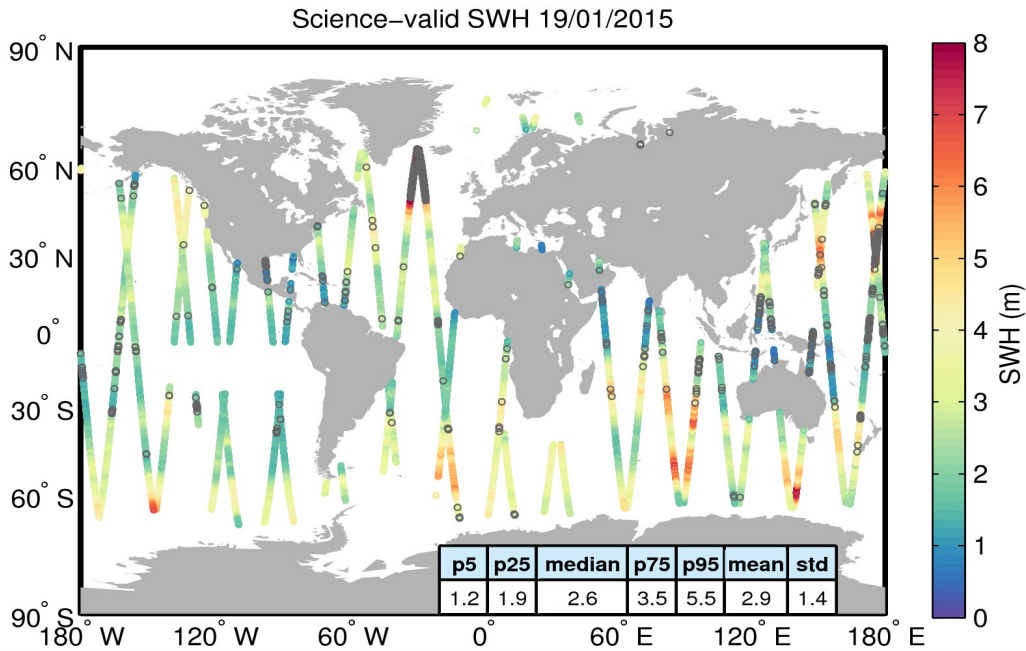
Figure 19. Geographical distribution of science-valid SWH data over oceans and lakes for 19/01/2015. The statistical values shown in the table refer to the SWH in m and are calculated over all measurements shown in the figure. Gray circles denote records that have been rejected based on the editing criteria described in Table 3.
