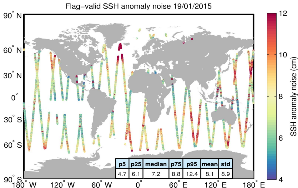
Figure 8. Geographical distribution of flag-valid 20-Hz SSH anomaly measurement noise over oceans and lakes for 19/01/2015. The statistical values shown in the table refer to the SSH anomaly noise and are calculated over all measurements shown in the figure.
