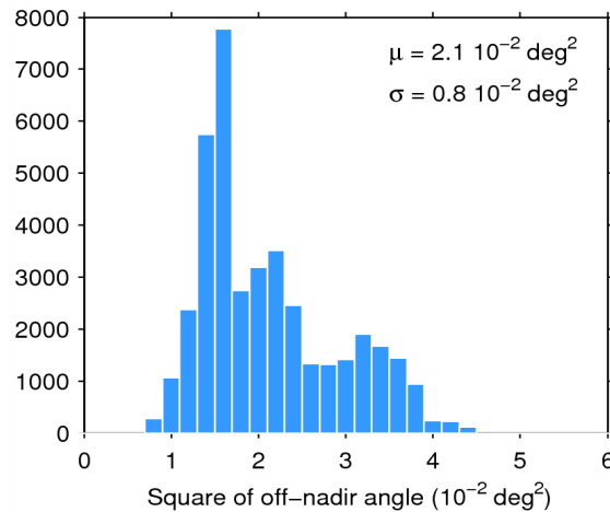
Figure 39. Histogram of flag-valid mispointing over oceans and lakes for 19/01/2015. The mean ( \mu ) and standard deviation ( \sigma ) are also shown. Note that values than 6 \cdot 10^{-2} \text{ deg}^2 are excluded from the histogram for the sake of readability but not from the computation of \mu and \sigma .
