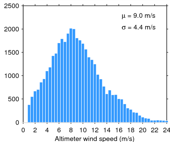
Figure 35. Histogram of science-valid wind over oceans and lakes for 19/01/2015. The mean ( \mu ) and standard deviation ( \sigma ) are also shown. Note that values larger than 24 m/s are excluded from the histogram for the sake of readability but not from the computation of \mu and \sigma .
