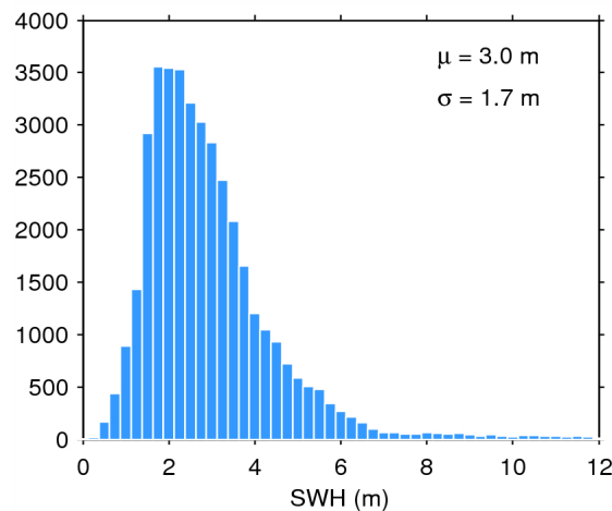
Figure 17. Histogram of flag-valid SWH over oceans and lakes for 19/01/2015. The mean ( \mu ) and standard deviation ( \sigma ) are also shown. Note that values larger than 12 m are excluded from the histogram for the sake of readability but not from the computation of \mu and \sigma .
