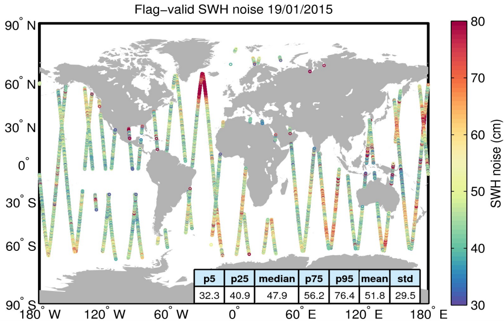
Figure 18. Geographical distribution of flag-valid 20-Hz SWH measurement noise over oceans and lakes for 19/01/2015. The statistical values shown in the figure refer to the SWH noise and are calculated over all measurements shown in the figure.
