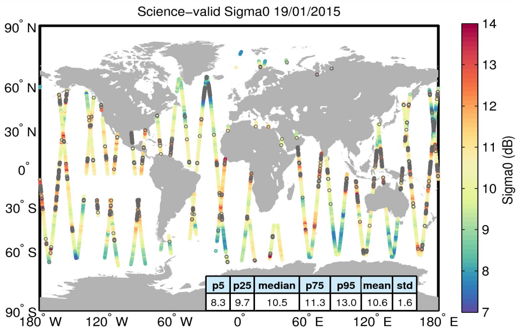
Figure 27. Geographical distribution of science-valid sigma0 data over oceans and lakes for 19/01/2015. The statistical values shown in the table refer to the sigma0 in dB and are calculated over all measurements shown in the figure. Gray circles denote records that have been rejected based on the editing criteria described in Table 4.
