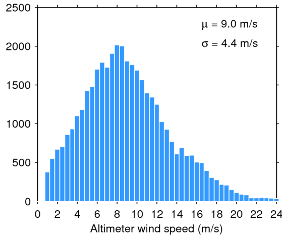
Figure 33. Histogram of flag-valid wind over oceans and lakes for 19/01/2015. The mean ( \mu ) and standard deviation ( \sigma ) are also shown. Note that values larger than 24 m/s are excluded from the histogram for the sake of readability but not from the computation of \mu and \sigma .
