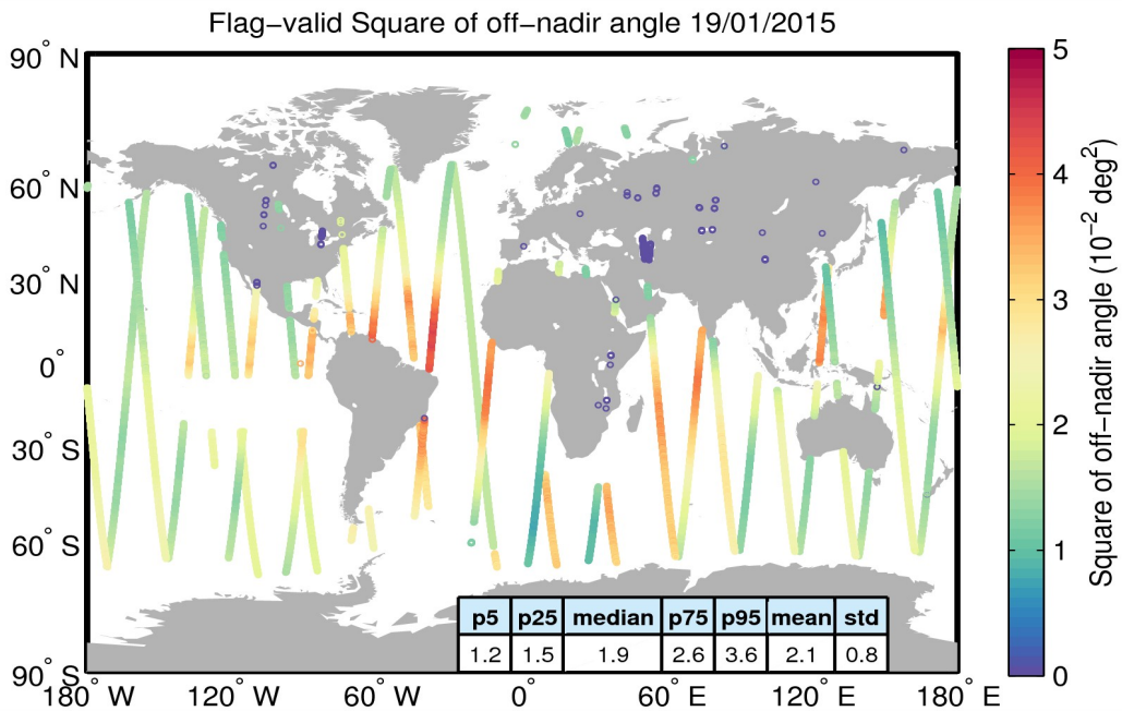
Figure 37. Geographical distribution of flag-valid mispointing data over oceans and lakes for 19/01/2015. The statistical values shown in the table refer to the mispointing in 10^{-2} \text{ deg}^2 and are calculated over all measurements shown in the figure.
