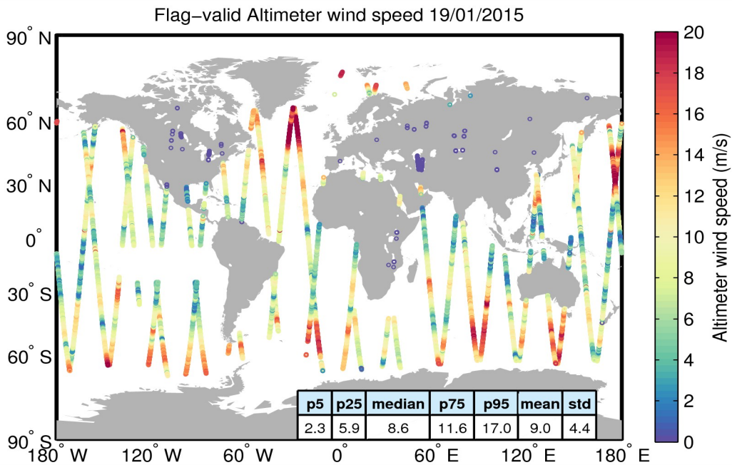
Figure 31. Geographical distribution of flag-valid wind data over oceans and lakes for 19/01/2015. The statistical values shown in the table refer to the wind in m/s and are calculated over all measurements shown in the figure.
