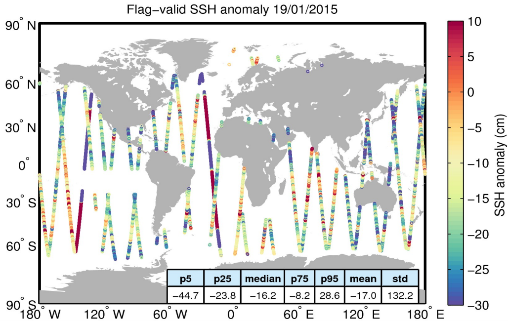
Figure 5. Geographical distribution of flag-valid 1-Hz SSH anomaly data over oceans and lakes for 19/01/2015. The statistical values shown in the table refer to the SSH anomaly in cm and are calculated over all measurements shown in the figure.
