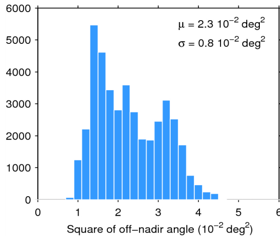
Figure 39. Histogram of flag-valid mispointing over oceans and lakes for 12/01/2015. The mean ( \mu ) and standard deviation ( \sigma ) are also shown. Note that values than 6 \cdot 10^{-2} \text{ deg}^2 are excluded from the histogram for the sake of readability but not from the computation of \mu and \sigma .
