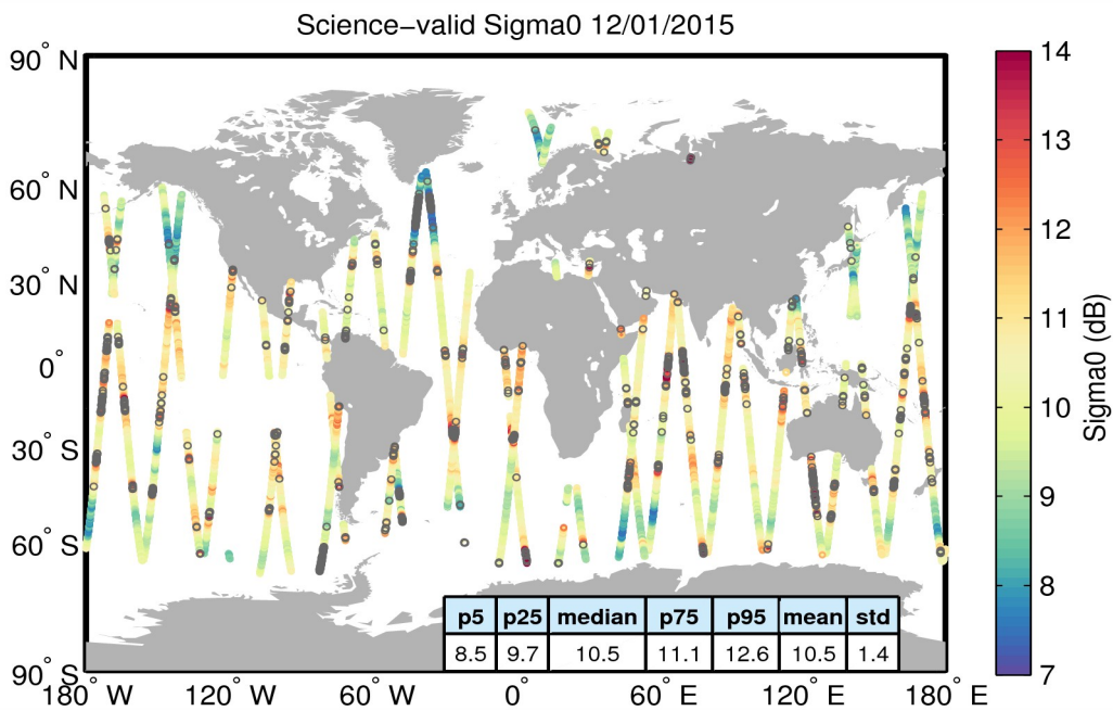
Figure 27. Geographical distribution of science-valid sigma0 data over oceans and lakes for 12/01/2015. The statistical values shown in the table refer to the sigma0 in dB and are calculated over all measurements shown in the figure. Gray circles denote records that have been rejected based on the editing criteria described in Table 4.
