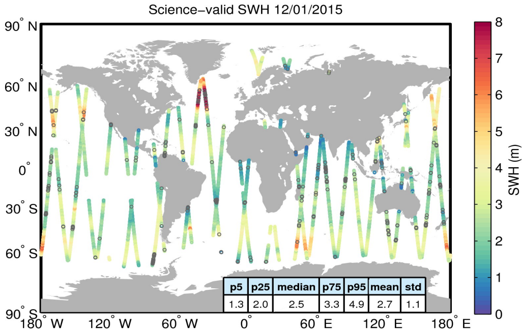
Figure 19. Geographical distribution of science-valid SWH data over oceans and lakes for 12/01/2015. The statistical values shown in the table refer to the SWH in m and are calculated over all measurements shown in the figure. Gray circles denote records that have been rejected based on the editing criteria described in Table 3.
