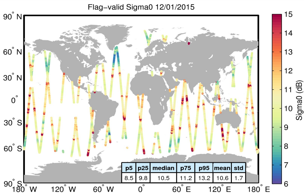
Figure 23. Geographical distribution of flag-valid sigma0 data over oceans and lakes for 12/01/2015. The statistical values shown in the table refer to the sigma0 in dB and are calculated over all measurements shown in the figure.
