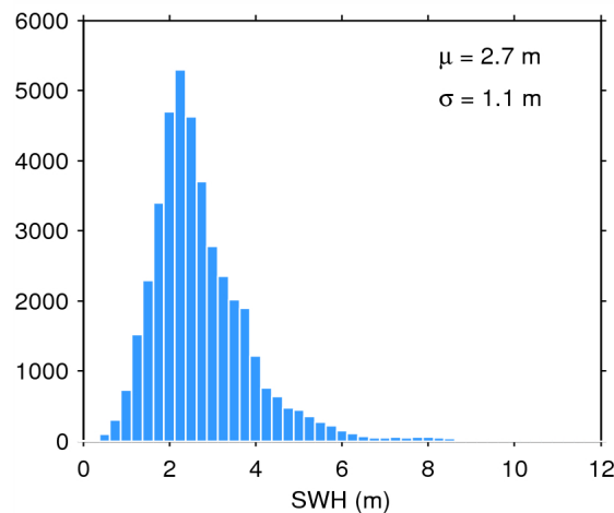
Figure 20. Histogram of science-valid SWH over oceans and lakes for 12/01/2015. The mean ( \mu ) and standard deviation ( \sigma ) are also shown. Note that values larger than 12 m are excluded from the histogram for the sake of readability but not from the computation of \mu and \sigma .
