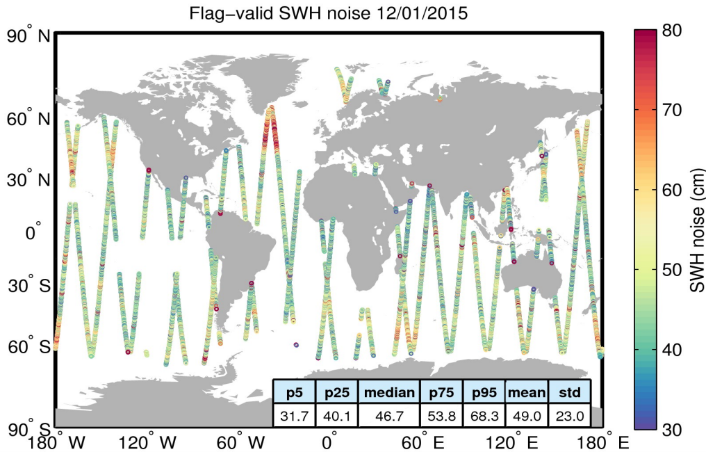
Figure 18. Geographical distribution of flag-valid 20-Hz SWH measurement noise over oceans and lakes for 12/01/2015. The statistical values shown in the figure refer to the SWH noise and are calculated over all measurements shown in the figure.
