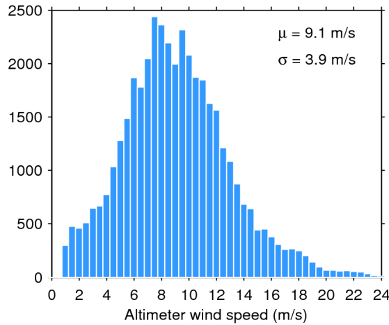
Figure 33. Histogram of flag-valid wind over oceans and lakes for 12/01/2015. The mean ( \mu ) and standard deviation ( \sigma ) are also shown. Note that values larger than 24 m/s are excluded from the histogram for the sake of readability but not from the computation of \mu and \sigma .
