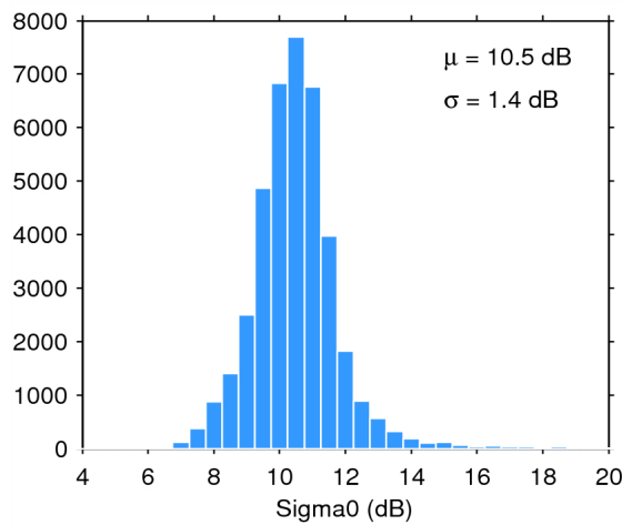
Figure 28. Histogram of science-valid sigma0 over oceans and lakes for 12/01/2015. The mean ( \mu ) and standard deviation ( \sigma ) are also shown. Note that values outside [4 20] dB are excluded from the histogram for the sake of readability but not from the computation of \mu and \sigma .
