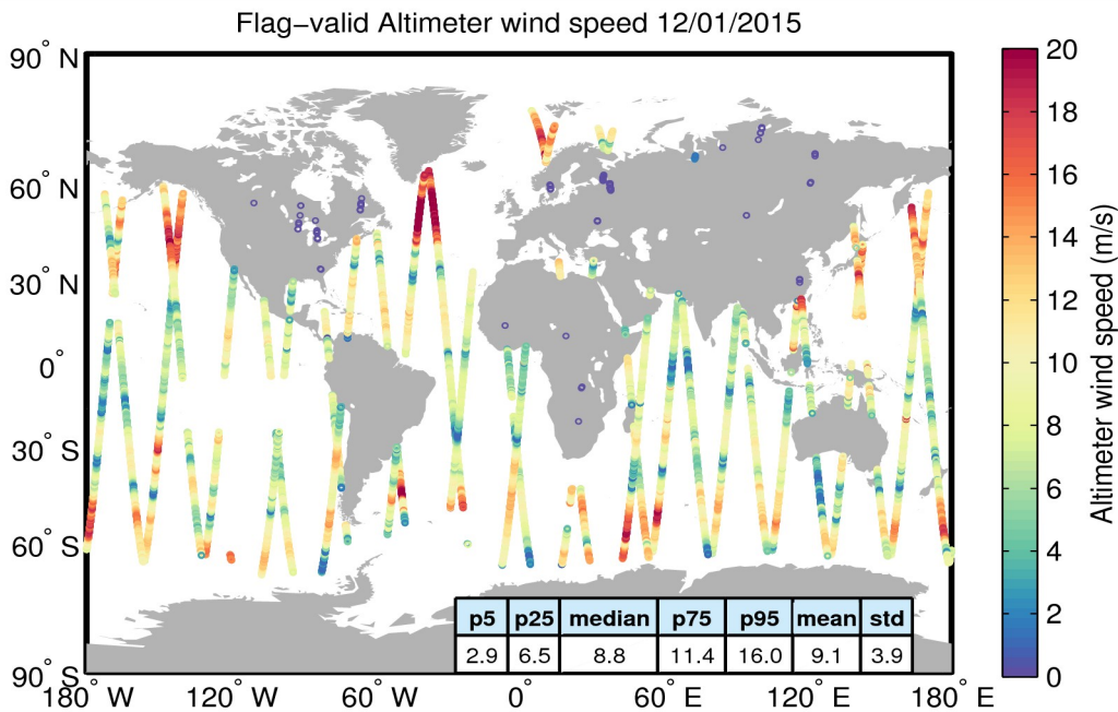
Figure 31. Geographical distribution of flag-valid wind data over oceans and lakes for 12/01/2015. The statistical values shown in the table refer to the wind in m/s and are calculated over all measurements shown in the figure.
