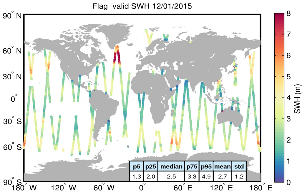
Figure 15. Geographical distribution of flag-valid SWH data over oceans and lakes for 12/01/2015. The statistical values shown in the table refer to the SWH in m and are calculated over all measurements shown in the figure.
