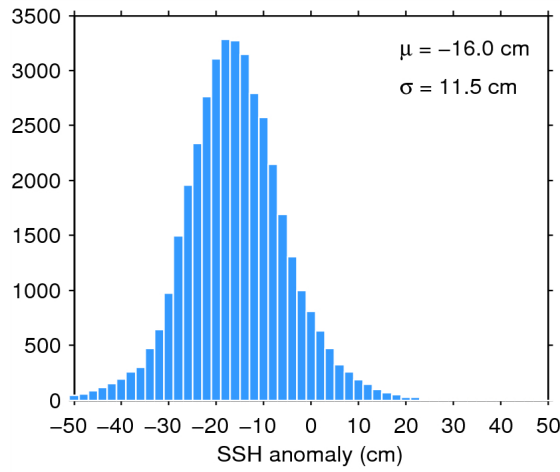
Figure 11. Histogram of science-valid SSH anomaly over oceans and lakes for 12/01/2015. The mean ( \mu ) and standard deviation ( \sigma ) are also shown. Note that values outside [-50 50] cm are excluded from the histogram for the sake of readability but not from the computation of \mu and \sigma .
