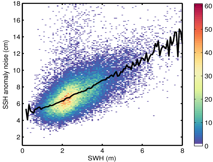
Figure 9. 2D histogram showing flag-valid SSH anomaly noise as a function of SWH for 12/01/2015. The black line denotes the median SSH anomaly as a function of SWH.
