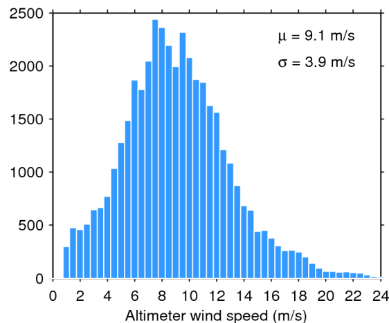
Figure 35. Histogram of science-valid wind over oceans and lakes for 12/01/2015. The mean ( \mu ) and standard deviation ( \sigma ) are also shown. Note that values larger than 24 m/s are excluded from the histogram for the sake of readability but not from the computation of \mu and \sigma .
