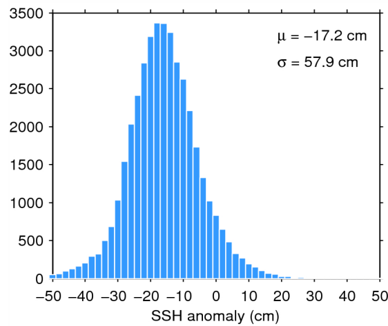
Figure 7. Histogram of flag-valid SSH anomaly over oceans and lakes for 12/01/2015. The mean ( \mu ) and standard deviation ( \sigma ) are also shown. Note that values outside [-50\ 50] cm are excluded from the histogram for the sake of readability but not from the computation of \mu and \sigma .
