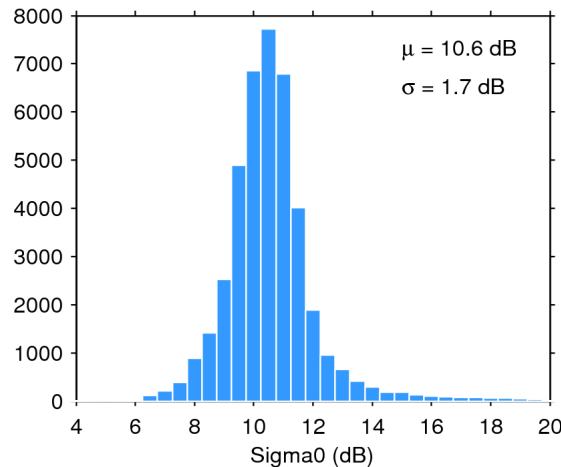
Figure 25. Histogram of flag-valid sigma0 over oceans and lakes for 12/01/2015. The mean ( \mu ) and standard deviation ( \sigma ) are also shown. Note that values outside [4 20] dB are excluded from the histogram for the sake of readability but not from the computation of \mu and \sigma .
