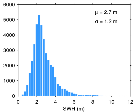
Figure 17. Histogram of flag-valid SWH over oceans and lakes for 12/01/2015. The mean ( \mu ) and standard deviation ( \sigma ) are also shown. Note that values larger than 12 m are excluded from the histogram for the sake of readability but not from the computation of \mu and \sigma .
