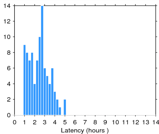
Figure 2. Histogram of the data latency for 12/01/2015. The y-axis denotes the number of files that are made available with a delay of x-hours with respect to the mean time of the records stored in the file.
