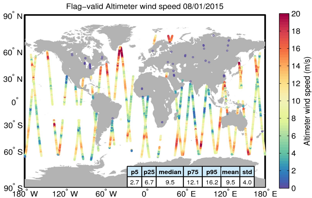
Figure 31. Geographical distribution of flag-valid wind data over oceans and lakes for 08/01/2015. The statistical values shown in the table refer to the wind in m/s and are calculated over all measurements shown in the figure.
