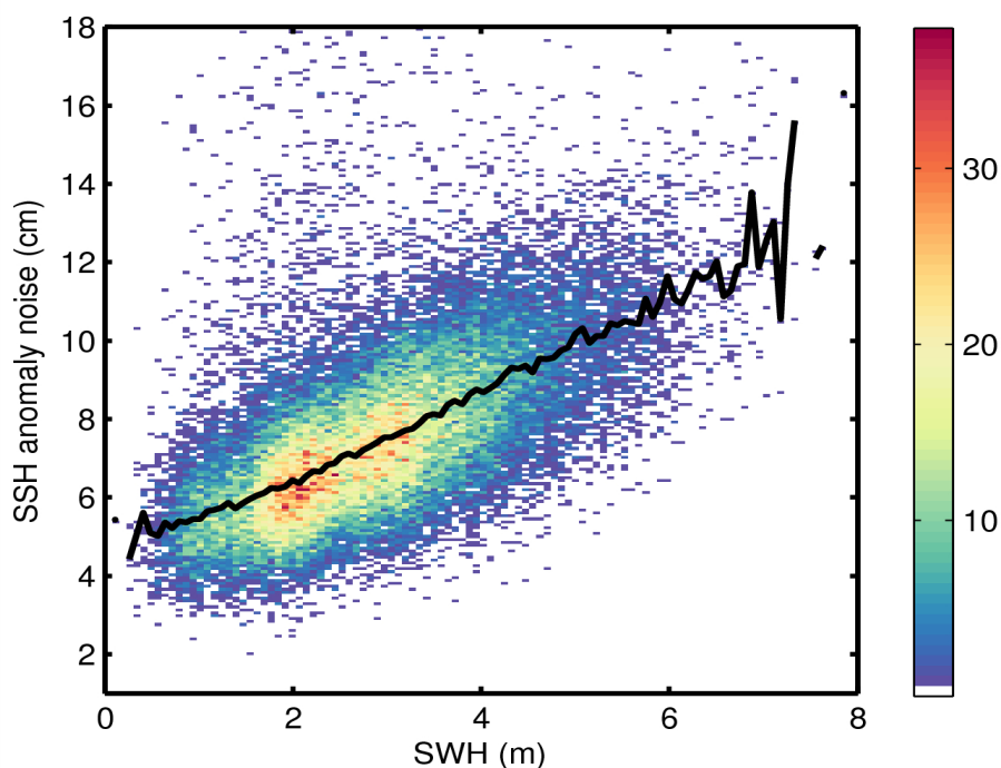
Figure 9. 2D histogram showing flag-valid SSH anomaly noise as a function of SWH for 08/01/2015. The black line denotes the median SSH anomaly as a function of SWH.
