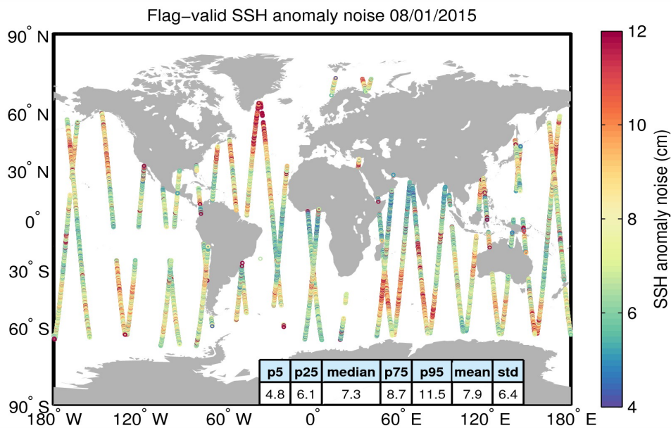
Figure 8. Geographical distribution of flag-valid 20-Hz SSH anomaly measurement noise over oceans and lakes for 08/01/2015. The statistical values shown in the table refer to the SSH anomaly noise and are calculated over all measurements shown in the figure.
