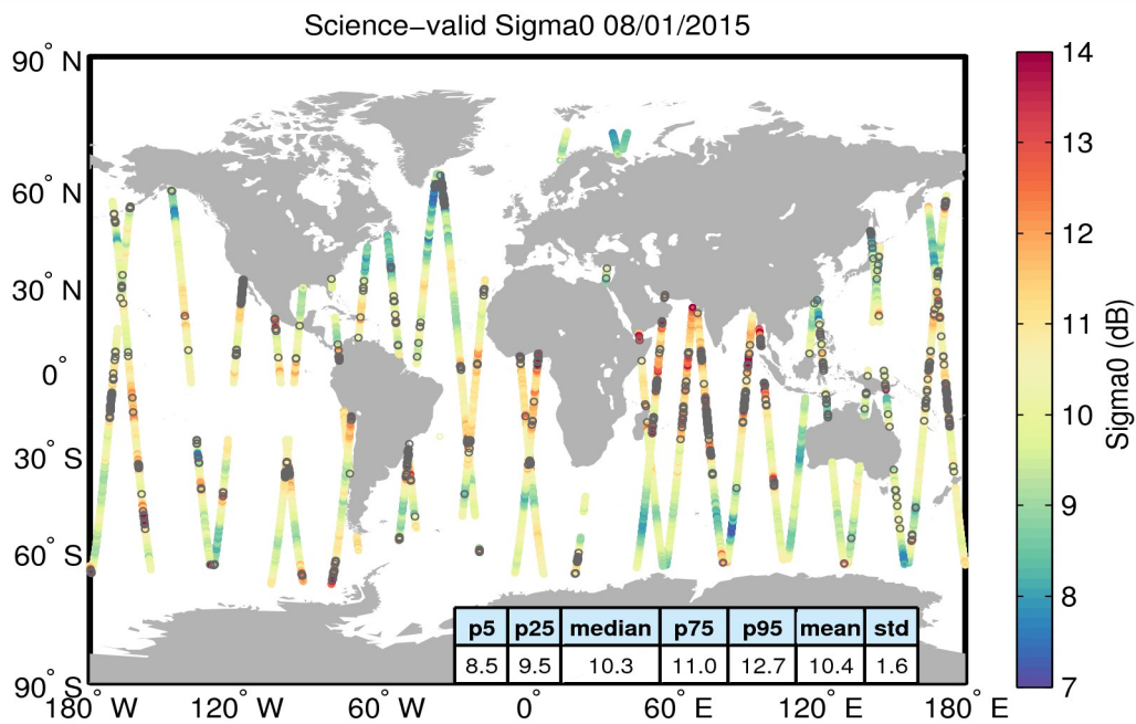
Figure 27. Geographical distribution of science-valid sigma0 data over oceans and lakes for 08/01/2015. The statistical values shown in the table refer to the sigma0 in dB and are calculated over all measurements shown in the figure. Gray circles denote records that have been rejected based on the editing criteria described in Table 4.
