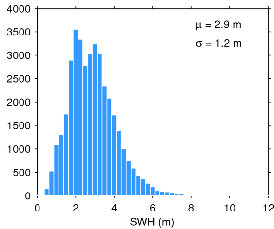
Figure 17. Histogram of flag-valid SWH over oceans and lakes for 08/01/2015. The mean ( \mu ) and standard deviation ( \sigma ) are also shown. Note that values larger than 12 m are excluded from the histogram for the sake of readability but not from the computation of \mu and \sigma .
