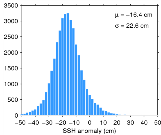
Figure 7. Histogram of flag-valid SSH anomaly over oceans and lakes for 08/01/2015. The mean ( \mu ) and standard deviation ( \sigma ) are also shown. Note that values outside [-50 50] cm are excluded from the histogram for the sake of readability but not from the computation of \mu and \sigma .
