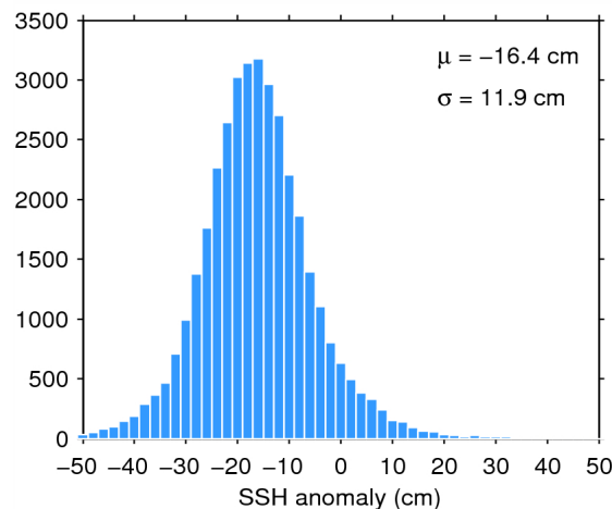
Figure 11. Histogram of science-valid SSH anomaly over oceans and lakes for 08/01/2015. The mean ( \mu ) and standard deviation ( \sigma ) are also shown. Note that values outside [-50 50] cm are excluded from the histogram for the sake of readability but not from the computation of \mu and \sigma .
