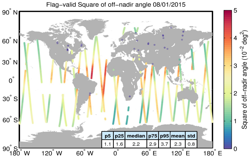
Figure 37. Geographical distribution of flag-valid mispointing data over oceans and lakes for 08/01/2015. The statistical values shown in the table refer to the mispointing in 10^{-2} \text{ deg}^2 and are calculated over all measurements shown in the figure.
