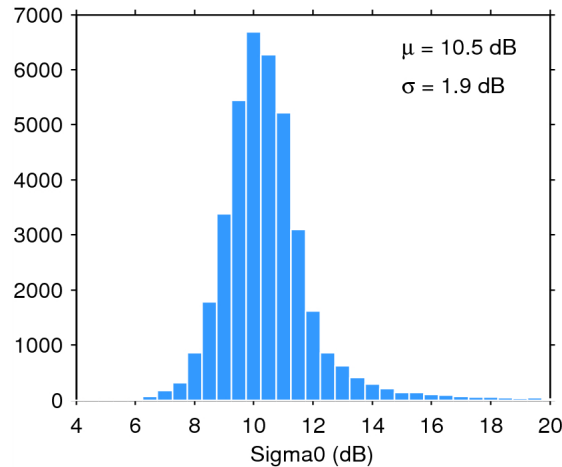
Figure 25. Histogram of flag-valid sigma0 over oceans and lakes for 08/01/2015. The mean ( \mu ) and standard deviation ( \sigma ) are also shown. Note that values outside [4 20] dB are excluded from the histogram for the sake of readability but not from the computation of \mu and \sigma .
