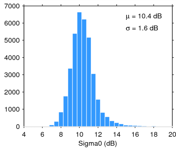
Figure 28. Histogram of science-valid sigma0 over oceans and lakes for 08/01/2015. The mean ( \mu ) and standard deviation ( \sigma ) are also shown. Note that values outside [4 20] dB are excluded from the histogram for the sake of readability but not from the computation of \mu and \sigma .
