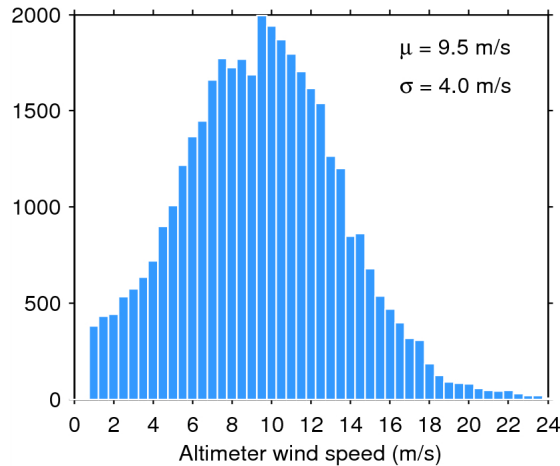
Figure 33. Histogram of flag-valid wind over oceans and lakes for 08/01/2015. The mean ( \mu ) and standard deviation ( \sigma ) are also shown. Note that values larger than 24 m/s are excluded from the histogram for the sake of readability but not from the computation of \mu and \sigma .
