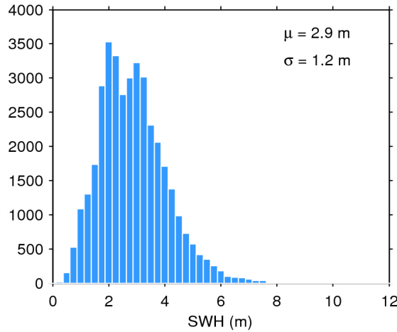
Figure 20. Histogram of science-valid SWH over oceans and lakes for 08/01/2015. The mean ( \mu ) and standard deviation ( \sigma ) are also shown. Note that values larger than 12 m are excluded from the histogram for the sake of readability but not from the computation of \mu and \sigma .
