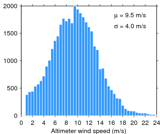
Figure 35. Histogram of science-valid wind over oceans and lakes for 08/01/2015. The mean ( \mu ) and standard deviation ( \sigma ) are also shown. Note that values larger than 24 m/s are excluded from the histogram for the sake of readability but not from the computation of \mu and \sigma .
