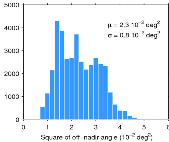
Figure 39. Histogram of flag-valid mispointing over oceans and lakes for 08/01/2015. The mean ( \mu ) and standard deviation ( \sigma ) are also shown. Note that values than 6 \cdot 10^{-2} \text{ deg}^2 are excluded from the histogram for the sake of readability but not from the computation of \mu and \sigma .
