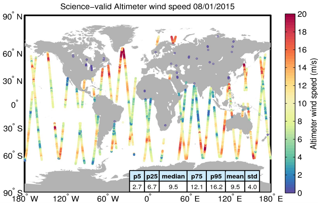
Figure 34. Geographical distribution of science-valid wind data over oceans and lakes for 08/01/2015. The statistical values shown in the table refer to the wind in m/s and are calculated over all measurements shown in the figure. Gray circles denote records that have been rejected based on the editing criteria described in Table 5.
