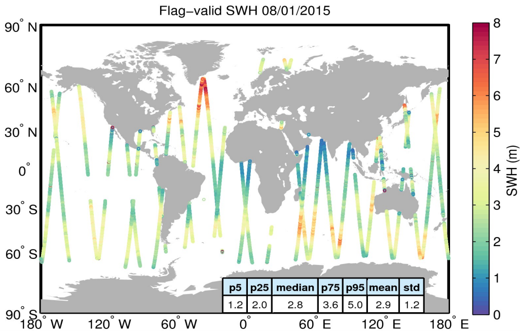
Figure 15. Geographical distribution of flag-valid SWH data over oceans and lakes for 08/01/2015. The statistical values shown in the figure refer to the SWH in m and are calculated over all measurements shown in the figure.
