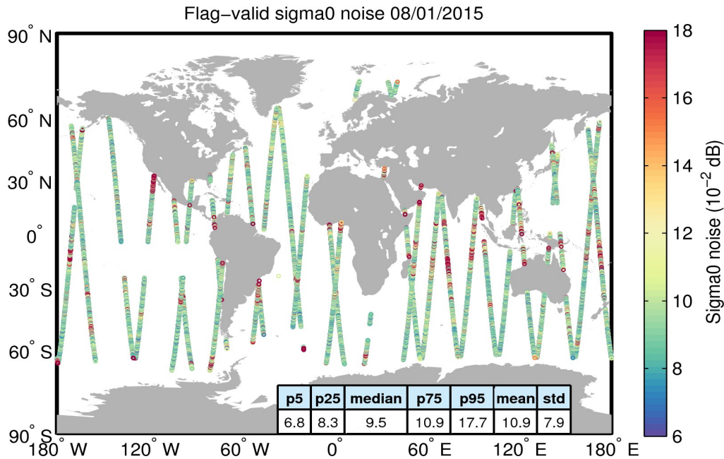
Figure 26. Geographical distribution of flag-valid 20-Hz sigma0 measurement noise over oceans and lakes for 08/01/2015. The statistical values shown in the table refer to the sigma0 noise and are calculated over all measurements shown in the figure.
