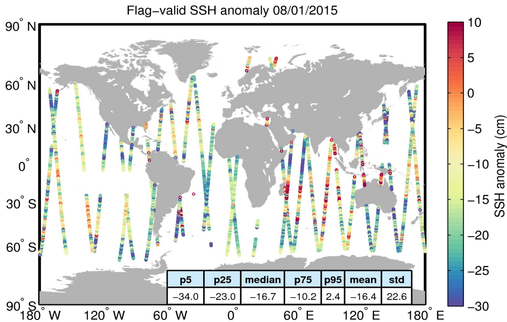
Figure 5. Geographical distribution of flag-valid 1-Hz SSH anomaly data over oceans and lakes for 08/01/2015. The statistical values shown in the table refer to the SSH anomaly in cm and are calculated over all measurements shown in the figure.
