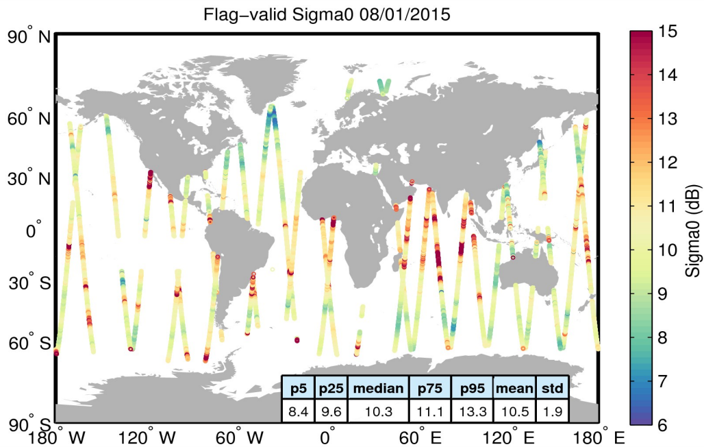
Figure 23. Geographical distribution of flag-valid sigma0 data over oceans and lakes for 08/01/2015. The statistical values shown in the table refer to the sigma0 in dB and are calculated over all measurements shown in the figure.
