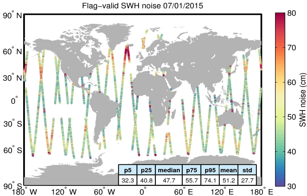
Figure 18. Geographical distribution of flag-valid 20-Hz SWH measurement noise over oceans and lakes for 07/01/2015. The statistical values shown in the figure refer to the SWH noise and are calculated over all measurements shown in the figure.
