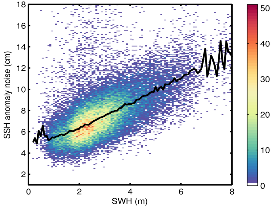
Figure 9. 2D histogram showing flag-valid SSH anomaly noise as a function of SWH for 07/01/2015. The black line denotes the median SSH anomaly as a function of SWH.
