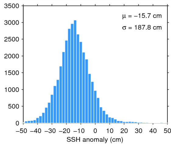
Figure 7. Histogram of flag-valid SSH anomaly over oceans and lakes for 07/01/2015. The mean ( \mu ) and standard deviation ( \sigma ) are also shown. Note that values outside [-50\ 50] cm are excluded from the histogram for the sake of readability but not from the computation of \mu and \sigma .
