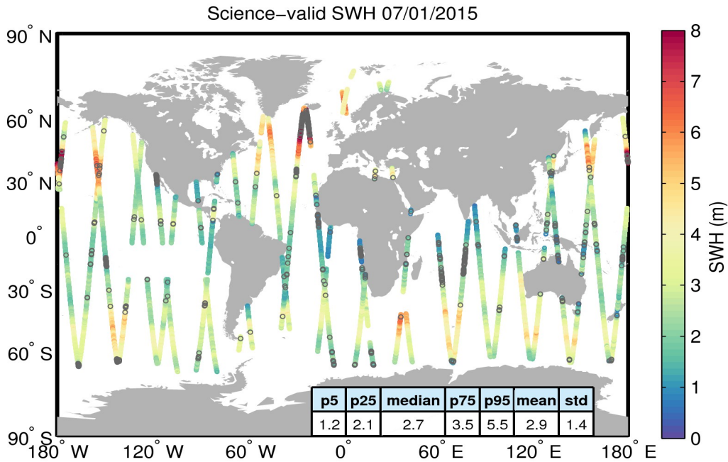
Figure 19. Geographical distribution of science-valid SWH data over oceans and lakes for 07/01/2015. The statistical values shown in the table refer to the SWH in m and are calculated over all measurements shown in the figure. Gray circles denote records that have been rejected based on the editing criteria described in Table 3.
