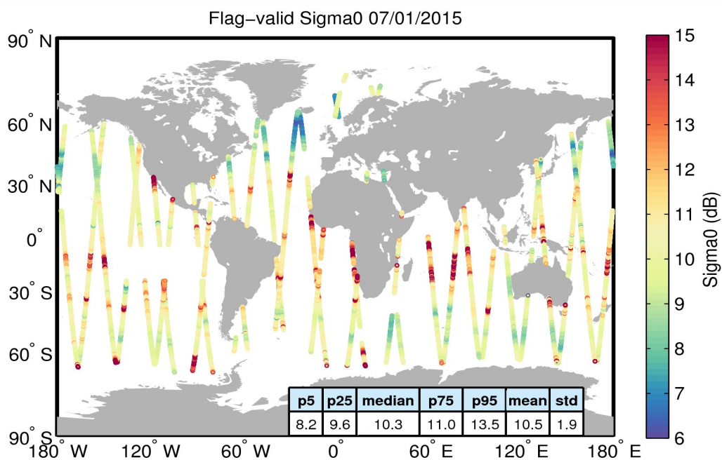
Figure 23. Geographical distribution of flag-valid sigma0 data over oceans and lakes for 07/01/2015. The statistical values shown in the table refer to the sigma0 in dB and are calculated over all measurements shown in the figure.
