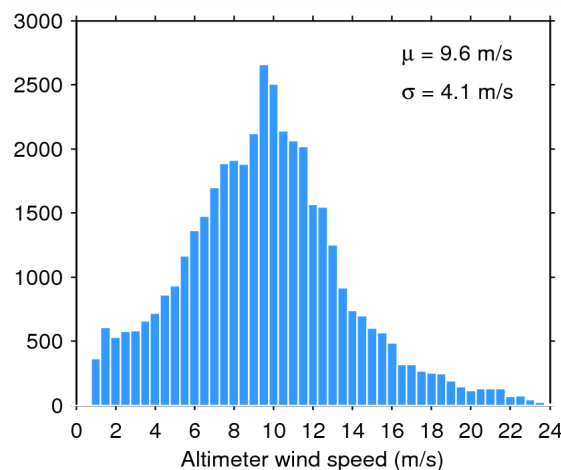
Figure 35. Histogram of science-valid wind over oceans and lakes for 07/01/2015. The mean ( \mu ) and standard deviation ( \sigma ) are also shown. Note that values larger than 24 m/s are excluded from the histogram for the sake of readability but not from the computation of \mu and \sigma .
