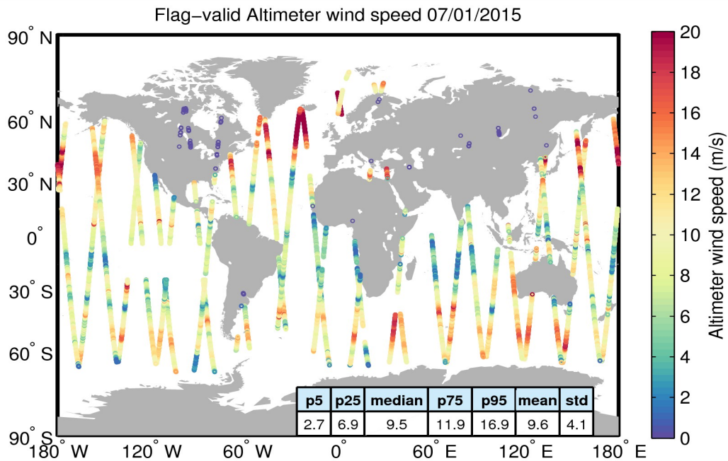
Figure 31. Geographical distribution of flag-valid wind data over oceans and lakes for 07/01/2015. The statistical values shown in the table refer to the wind in m/s and are calculated over all measurements shown in the figure.
