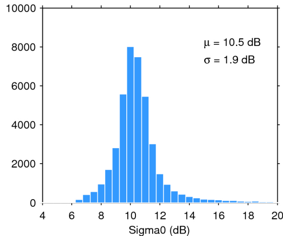
Figure 25. Histogram of flag-valid sigma0 over oceans and lakes for 07/01/2015. The mean ( \mu ) and standard deviation ( \sigma ) are also shown. Note that values outside [4 20] dB are excluded from the histogram for the sake of readability but not from the computation of \mu and \sigma .
