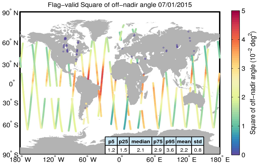
Figure 37. Geographical distribution of flag-valid mispointing data over oceans and lakes for 07/01/2015. The statistical values shown in the table refer to the mispointing in 10^{-2} \text{deg}^2 and are calculated over all measurements shown in the figure.
