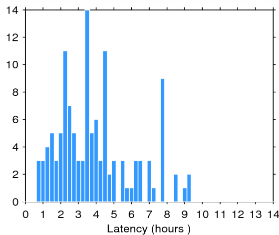
Figure 2. Histogram of the data latency for 07/01/2015. The y-axis denotes the number of files that are made available with a delay of x-hours with respect to the mean time of the records stored in the file.
