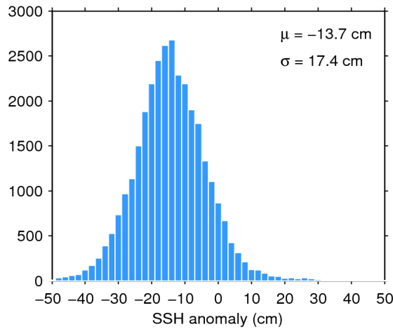
Figure 11. Histogram of science-valid SSH anomaly over oceans and lakes for 07/01/2015. The mean ( \mu ) and standard deviation ( \sigma ) are also shown. Note that values outside [-50 50] cm are excluded from the histogram for the sake of readability but not from the computation of \mu and \sigma .
