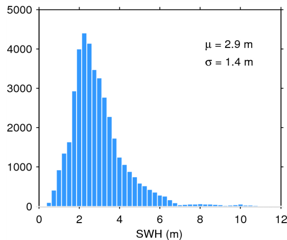
Figure 20. Histogram of science-valid SWH over oceans and lakes for 07/01/2015. The mean ( \mu ) and standard deviation ( \sigma ) are also shown. Note that values larger than 12 m are excluded from the histogram for the sake of readability but not from the computation of \mu and \sigma .
