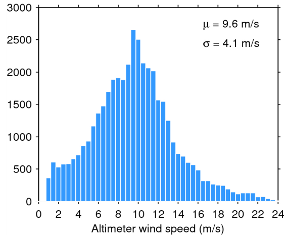
Figure 33. Histogram of flag-valid wind over oceans and lakes for 07/01/2015. The mean ( \mu ) and standard deviation ( \sigma ) are also shown. Note that values larger than 24 m/s are excluded from the histogram for the sake of readability but not from the computation of \mu and \sigma .
