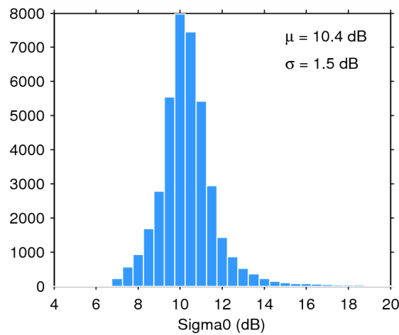
Figure 28. Histogram of science-valid sigma0 over oceans and lakes for 07/01/2015. The mean ( \mu ) and standard deviation ( \sigma ) are also shown. Note that values outside [4 20] dB are excluded from the histogram for the sake of readability but not from the computation of \mu and \sigma .
