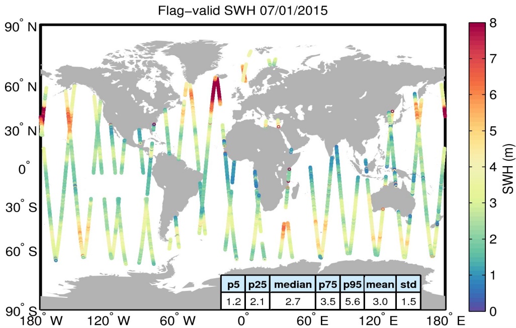
Figure 15. Geographical distribution of flag-valid SWH data over oceans and lakes for 07/01/2015. The statistical values shown in the table refer to the SWH in m and are calculated over all measurements shown in the figure.
