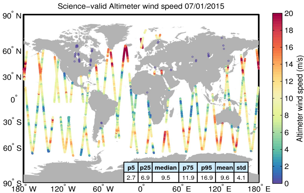
Figure 34. Geographical distribution of science-valid wind data over oceans and lakes for 07/01/2015. The statistical values shown in the table refer to the wind in m/s and are calculated over all measurements shown in the figure. Gray circles denote records that have been rejected based on the editing criteria described in Table 5.
