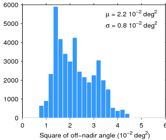
Figure 39. Histogram of flag-valid mispointing over oceans and lakes for 07/01/2015. The mean ( \mu ) and standard deviation ( \sigma ) are also shown. Note that values than 6 \cdot 10^{-2} \text{ deg}^2 are excluded from the histogram for the sake of readability but not from the computation of \mu and \sigma .
