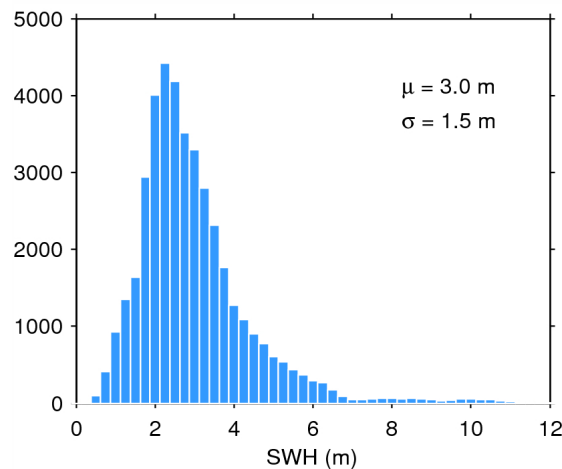
Figure 17. Histogram of flag-valid SWH over oceans and lakes for 07/01/2015. The mean ( \mu ) and standard deviation ( \sigma ) are also shown. Note that values larger than 12 m are excluded from the histogram for the sake of readability but not from the computation of \mu and \sigma .
