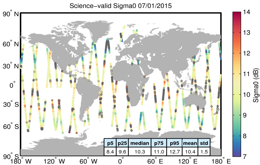
Figure 27. Geographical distribution of science-valid sigma0 data over oceans and lakes for 07/01/2015. The statistical values shown in the table refer to the sigma0 in dB and are calculated over all measurements shown in the figure. Gray circles denote records that have been rejected based on the editing criteria described in Table 4.
