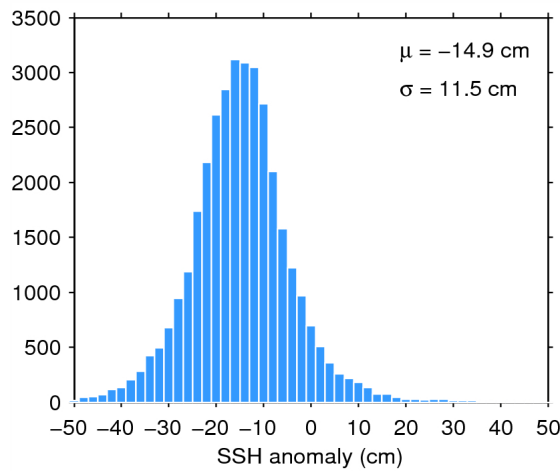
Figure 11. Histogram of science-valid SSH anomaly over oceans and lakes for 05/01/2015. The mean ( \mu ) and standard deviation ( \sigma ) are also shown. Note that values outside [-50 50] cm are excluded from the histogram for the sake of readability but not from the computation of \mu and \sigma .
