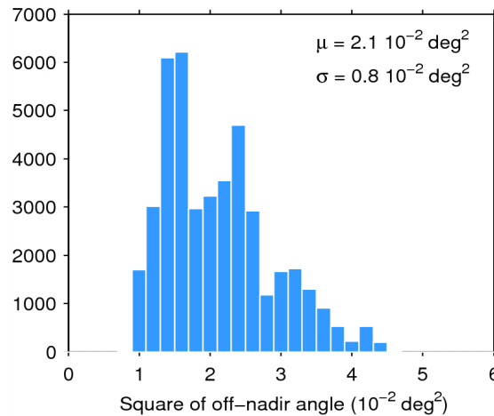
Figure 39. Histogram of flag-valid mispointing over oceans and lakes for 05/01/2015. The mean ( \mu ) and standard deviation ( \sigma ) are also shown. Note that values than 6 \cdot 10^{-2} \text{ deg}^2 are excluded from the histogram for the sake of readability but not from the computation of \mu and \sigma .
