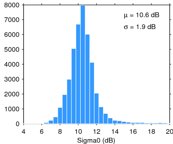
Figure 25. Histogram of flag-valid sigma0 over oceans and lakes for 05/01/2015. The mean ( \mu ) and standard deviation ( \sigma ) are also shown. Note that values outside [4 20] dB are excluded from the histogram for the sake of readability but not from the computation of \mu and \sigma .
