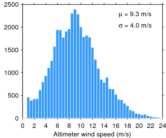
Figure 33. Histogram of flag-valid wind over oceans and lakes for 05/01/2015. The mean ( \mu ) and standard deviation ( \sigma ) are also shown. Note that values larger than 24 m/s are excluded from the histogram for the sake of readability but not from the computation of \mu and \sigma .
