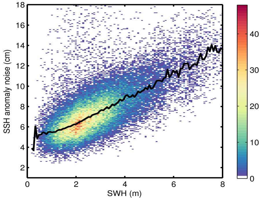
Figure 9. 2D histogram showing flag-valid SSH anomaly noise as a function of SWH for 05/01/2015. The black line denotes the median SSH anomaly as a function of SWH.
