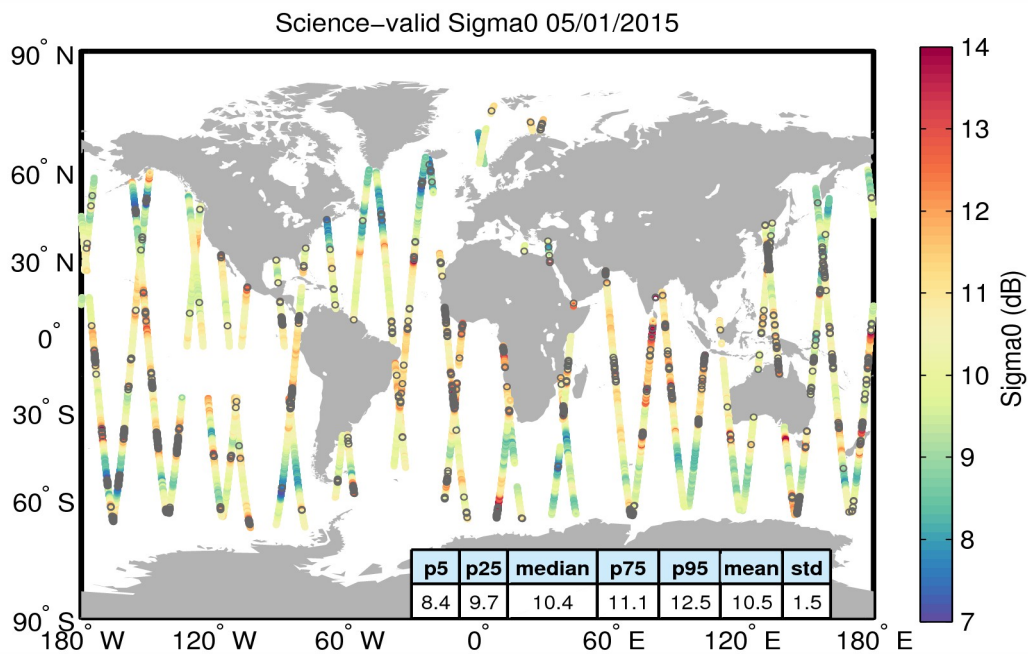
Figure 27. Geographical distribution of science-valid sigma0 data over oceans and lakes for 05/01/2015. The statistical values shown in the table refer to the sigma0 in dB and are calculated over all measurements shown in the figure. Gray circles denote records that have been rejected based on the editing criteria described in Table 4.
