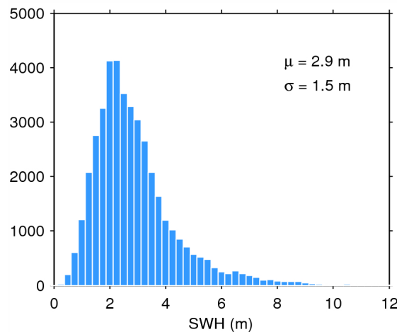
Figure 17. Histogram of flag-valid SWH over oceans and lakes for 05/01/2015. The mean ( \mu ) and standard deviation ( \sigma ) are also shown. Note that values larger than 12 m are excluded from the histogram for the sake of readability but not from the computation of \mu and \sigma .
