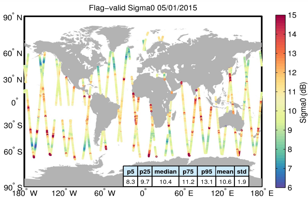
Figure 23. Geographical distribution of flag-valid sigma0 data over oceans and lakes for 05/01/2015. The statistical values shown in the table refer to the sigma0 in dB and are calculated over all measurements shown in the figure.
