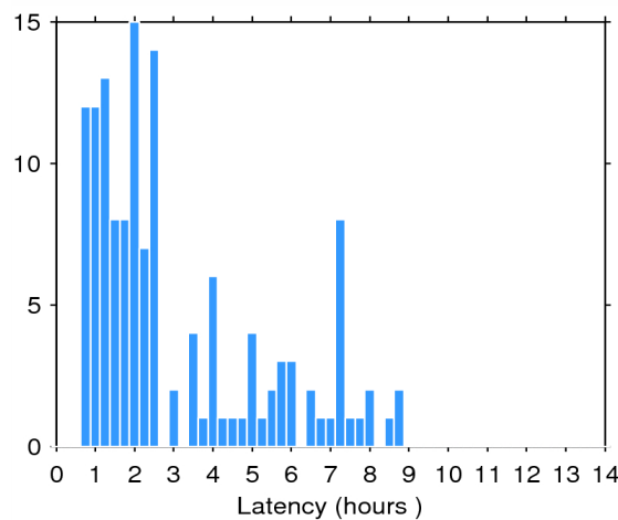
Figure 2. Histogram of the data latency for 05/01/2015. The y-axis denotes the number of files that are made available with a delay of x-hours with respect to the mean time of the records stored in the file.
