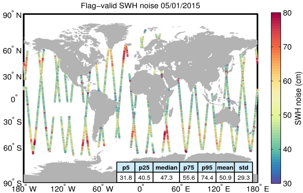
Figure 18. Geographical distribution of flag-valid 20-Hz SWH measurement noise over oceans and lakes for 05/01/2015. The statistical values shown in the figure refer to the SWH noise and are calculated over all measurements shown in the figure.
