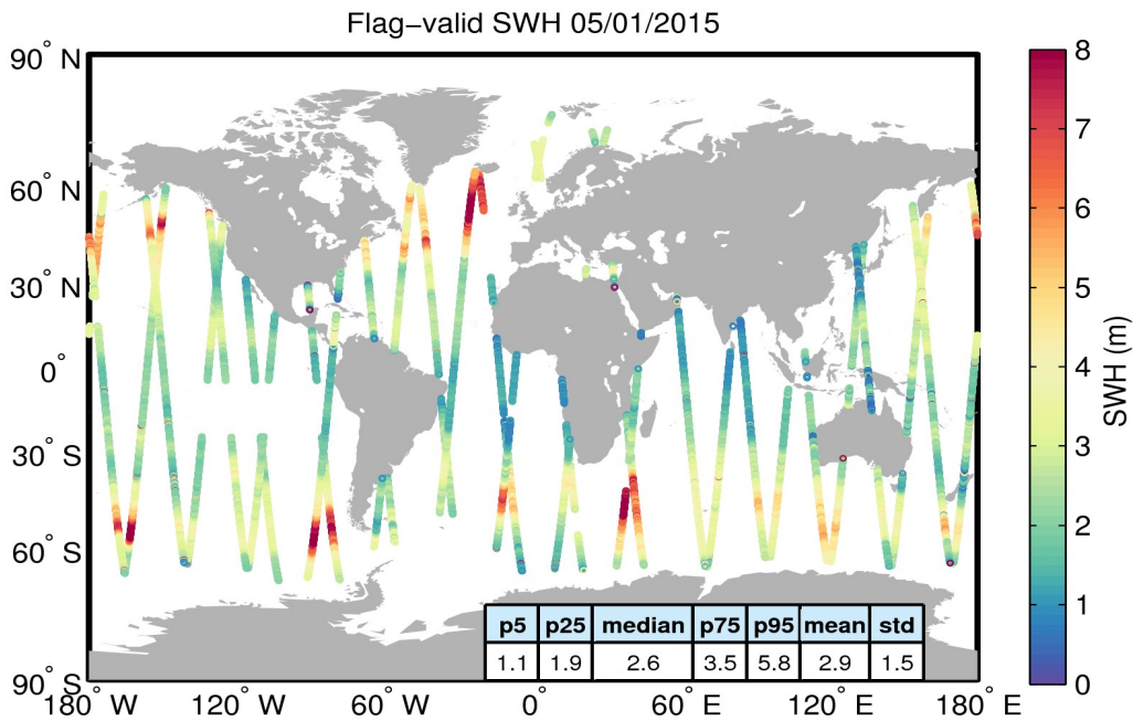
Figure 15. Geographical distribution of flag-valid SWH data over oceans and lakes for 05/01/2015. The statistical values shown in the table refer to the SWH in m and are calculated over all measurements shown in the figure.
