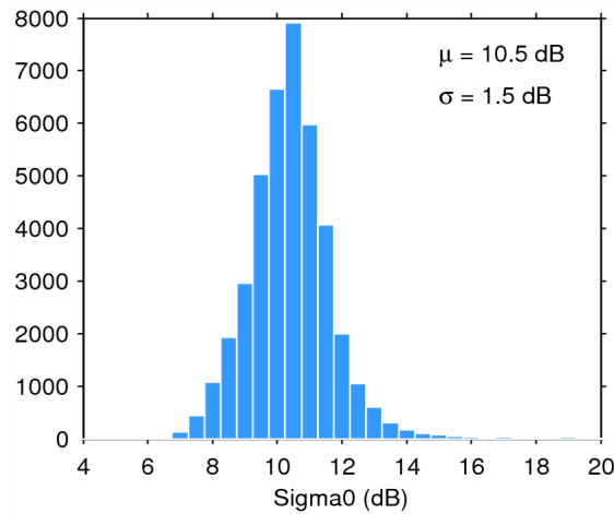
Figure 28. Histogram of science-valid sigma0 over oceans and lakes for 05/01/2015. The mean ( \mu ) and standard deviation ( \sigma ) are also shown. Note that values outside [4 20] dB are excluded from the histogram for the sake of readability but not from the computation of \mu and \sigma .
