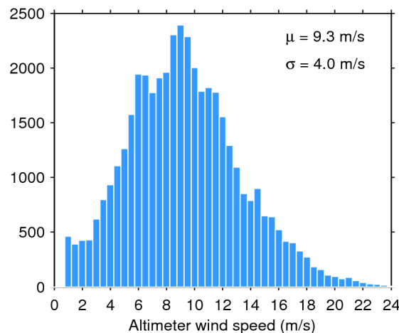
Figure 35. Histogram of science-valid wind over oceans and lakes for 05/01/2015. The mean ( \mu ) and standard deviation ( \sigma ) are also shown. Note that values larger than 24 m/s are excluded from the histogram for the sake of readability but not from the computation of \mu and \sigma .
