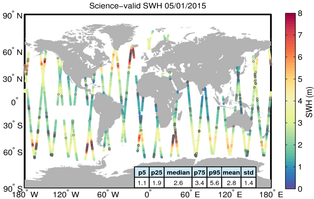
Figure 19. Geographical distribution of science-valid SWH data over oceans and lakes for 05/01/2015. The statistical values shown in the table refer to the SWH in m and are calculated over all measurements shown in the figure. Gray circles denote records that have been rejected based on the editing criteria described in Table 3.
