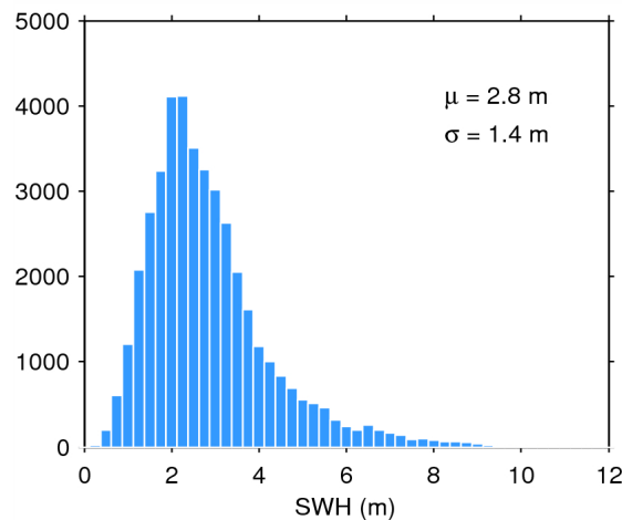
Figure 20. Histogram of science-valid SWH over oceans and lakes for 05/01/2015. The mean ( \mu ) and standard deviation ( \sigma ) are also shown. Note that values larger than 12 m are excluded from the histogram for the sake of readability but not from the computation of \mu and \sigma .
