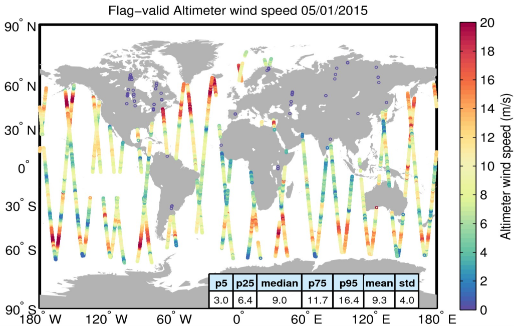
Figure 31. Geographical distribution of flag-valid wind data over oceans and lakes for 05/01/2015. The statistical values shown in the table refer to the wind in m/s and are calculated over all measurements shown in the figure.
