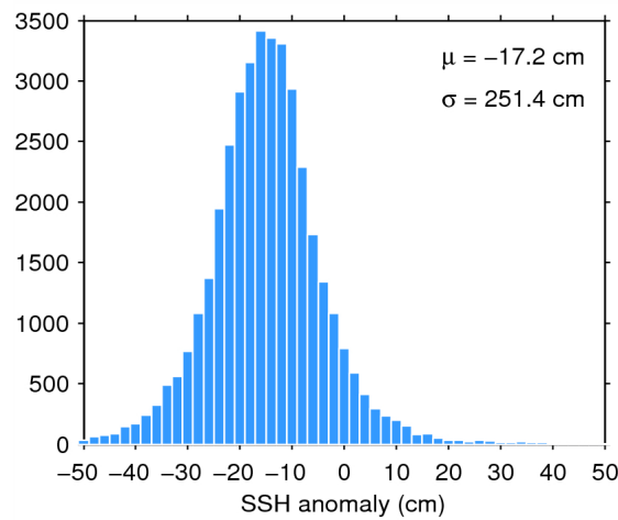
Figure 7. Histogram of flag-valid SSH anomaly over oceans and lakes for 05/01/2015. The mean ( \mu ) and standard deviation ( \sigma ) are also shown. Note that values outside [-50\ 50] cm are excluded from the histogram for the sake of readability but not from the computation of \mu and \sigma .
