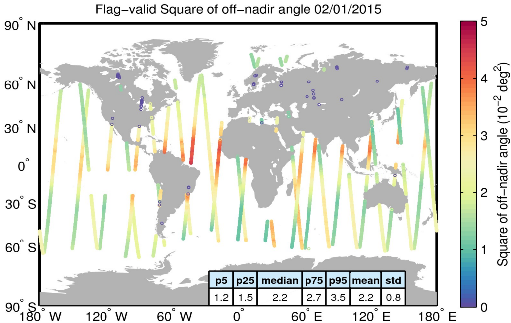
Figure 37. Geographical distribution of flag-valid mispointing data over oceans and lakes for 02/01/2015. The statistical values shown in the table refer to the mispointing in 10^{-2} \text{deg}^2 and are calculated over all measurements shown in the figure.
