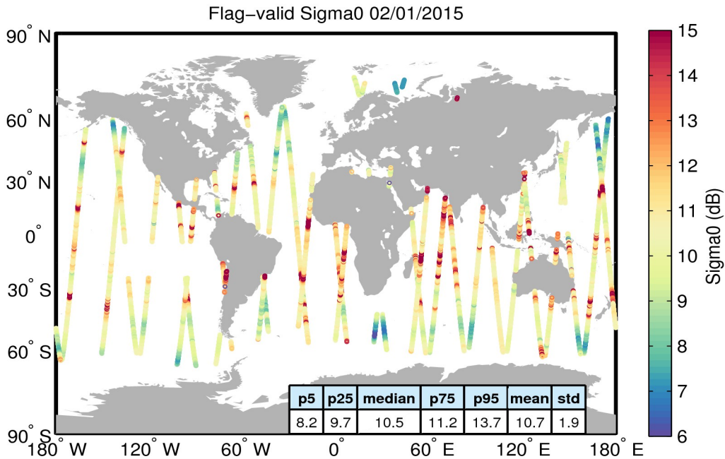
Figure 23. Geographical distribution of flag-valid sigma0 data over oceans and lakes for 02/01/2015. The statistical values shown in the table refer to the sigma0 in dB and are calculated over all measurements shown in the figure.
