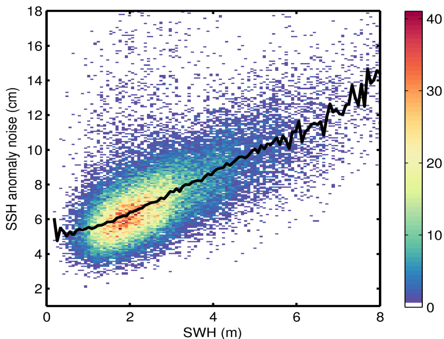
Figure 9. 2D histogram showing flag-valid SSH anomaly noise as a function of SWH for 02/01/2015. The black line denotes the median SSH anomaly as a function of SWH.
