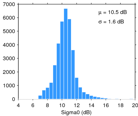
Figure 28. Histogram of science-valid sigma0 over oceans and lakes for 02/01/2015. The mean ( \mu ) and standard deviation ( \sigma ) are also shown. Note that values outside [4 20] dB are excluded from the histogram for the sake of readability but not from the computation of \mu and \sigma .
