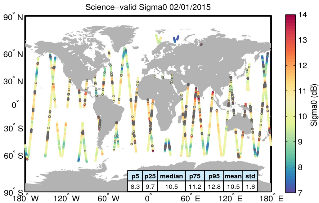
Figure 27. Geographical distribution of science-valid sigma0 data over oceans and lakes for 02/01/2015. The statistical values shown in the table refer to the sigma0 in dB and are calculated over all measurements shown in the figure. Gray circles denote records that have been rejected based on the editing criteria described in Table 4.
