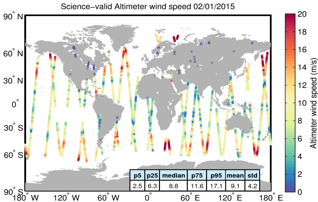
Figure 34. Geographical distribution of science-valid wind data over oceans and lakes for 02/01/2015. The statistical values shown in the table refer to the wind in m/s and are calculated over all measurements shown in the figure. Gray circles denote records that have been rejected based on the editing criteria described in Table 5.
