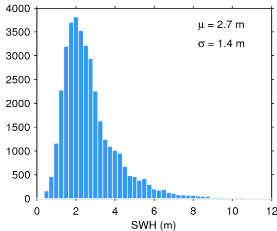
Figure 20. Histogram of science-valid SWH over oceans and lakes for 02/01/2015. The mean ( \mu ) and standard deviation ( \sigma ) are also shown. Note that values larger than 12 m are excluded from the histogram for the sake of readability but not from the computation of \mu and \sigma .
