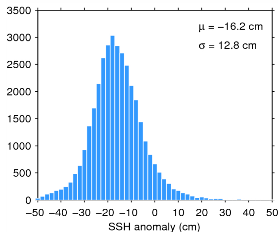
Figure 11. Histogram of science-valid SSH anomaly over oceans and lakes for 02/01/2015. The mean ( \mu ) and standard deviation ( \sigma ) are also shown. Note that values outside [-50 50] cm are excluded from the histogram for the sake of readability but not from the computation of \mu and \sigma .
