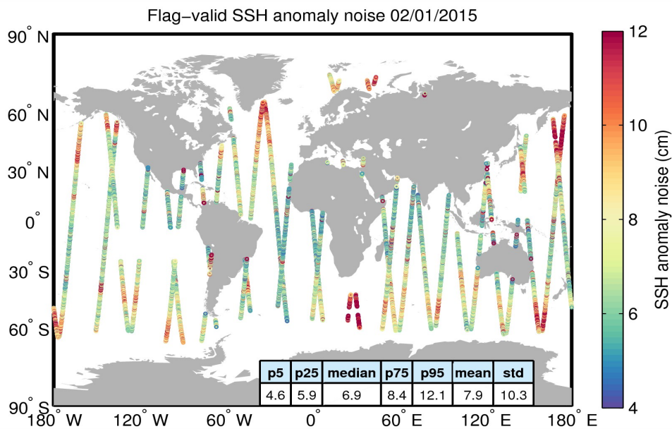
Figure 8. Geographical distribution of flag-valid 20-Hz SSH anomaly measurement noise over oceans and lakes for 02/01/2015. The statistical values shown in the table refer to the SSH anomaly noise and are calculated over all measurements shown in the figure.
