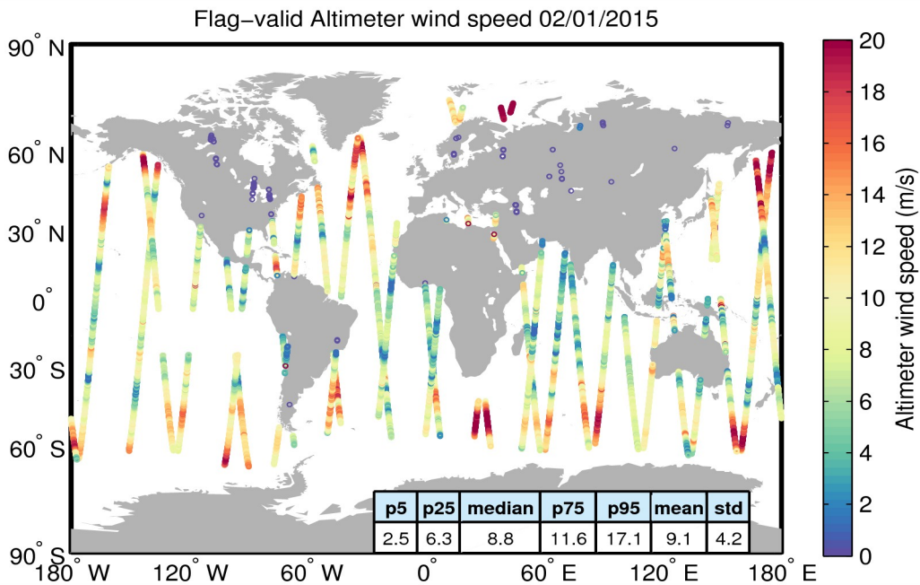
Figure 31. Geographical distribution of flag-valid wind data over oceans and lakes for 02/01/2015. The statistical values shown in the table refer to the wind in m/s and are calculated over all measurements shown in the figure.
