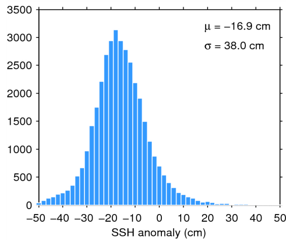
Figure 7. Histogram of flag-valid SSH anomaly over oceans and lakes for 02/01/2015. The mean ( \mu ) and standard deviation ( \sigma ) are also shown. Note that values outside [-50 50] cm are excluded from the histogram for the sake of readability but not from the computation of \mu and \sigma .
