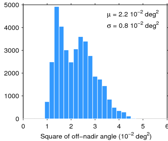
Figure 39. Histogram of flag-valid mispointing over oceans and lakes for 02/01/2015. The mean ( \mu ) and standard deviation ( \sigma ) are also shown. Note that values than 6 \cdot 10^{-2} \text{ deg}^2 are excluded from the histogram for the sake of readability but not from the computation of \mu and \sigma .
