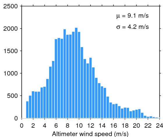
Figure 35. Histogram of science-valid wind over oceans and lakes for 02/01/2015. The mean ( \mu ) and standard deviation ( \sigma ) are also shown. Note that values larger than 24 m/s are excluded from the histogram for the sake of readability but not from the computation of \mu and \sigma .
