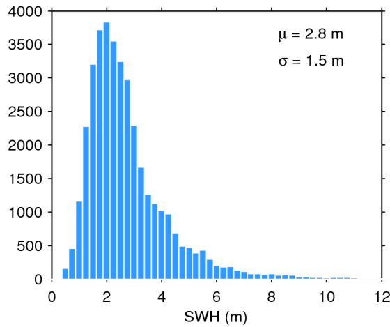
Figure 17. Histogram of flag-valid SWH over oceans and lakes for 02/01/2015. The mean ( \mu ) and standard deviation ( \sigma ) are also shown. Note that values larger than 12 m are excluded from the histogram for the sake of readability but not from the computation of \mu and \sigma .
