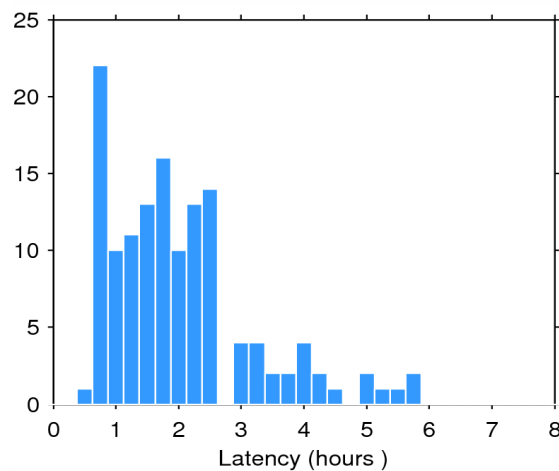
Figure 2. Histogram of the data latency for 02/01/2015. The y-axis denotes the number of files that are made available with a delay of x-hours with respect to the mean time of the records stored in the file.
