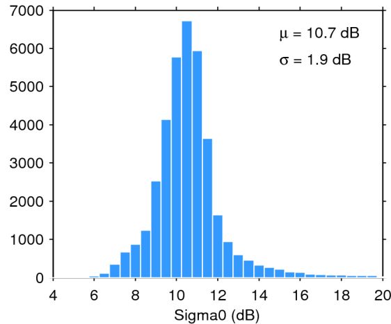
Figure 25. Histogram of flag-valid sigma0 over oceans and lakes for 02/01/2015. The mean ( \mu ) and standard deviation ( \sigma ) are also shown. Note that values outside [4 20] dB are excluded from the histogram for the sake of readability but not from the computation of \mu and \sigma .
