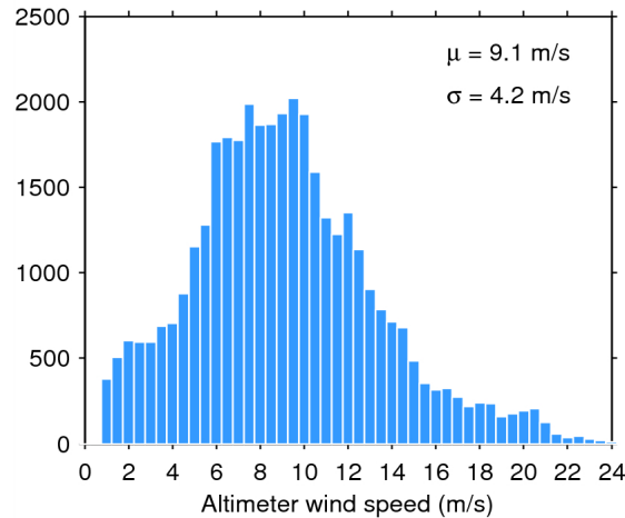
Figure 33. Histogram of flag-valid wind over oceans and lakes for 02/01/2015. The mean ( \mu ) and standard deviation ( \sigma ) are also shown. Note that values larger than 24 m/s are excluded from the histogram for the sake of readability but not from the computation of \mu and \sigma .
