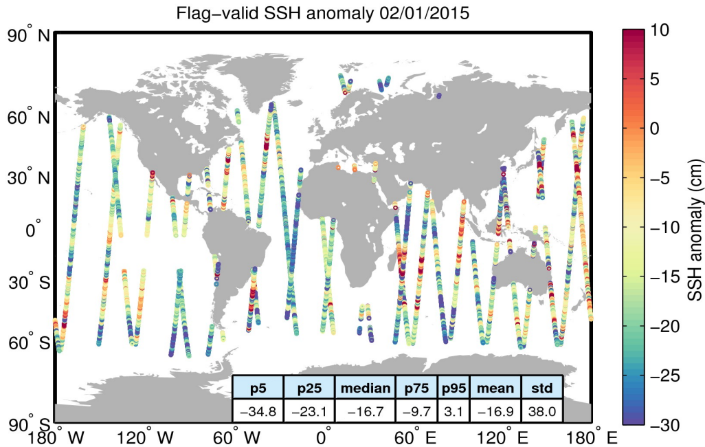
Figure 5. Geographical distribution of flag-valid 1-Hz SSH anomaly data over oceans and lakes for 02/01/2015. The statistical values shown in the table refer to the SSH anomaly in cm and are calculated over all measurements shown in the figure.
