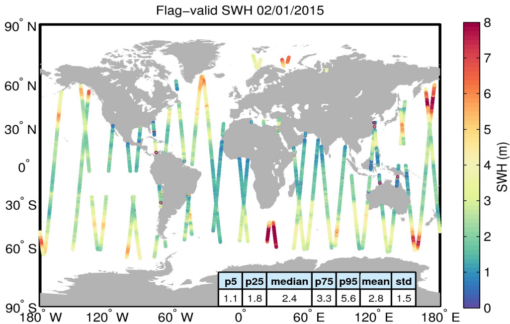
Figure 15. Geographical distribution of flag-valid SWH data over oceans and lakes for 02/01/2015. The statistical values shown in the table refer to the SWH in m and are calculated over all measurements shown in the figure.
