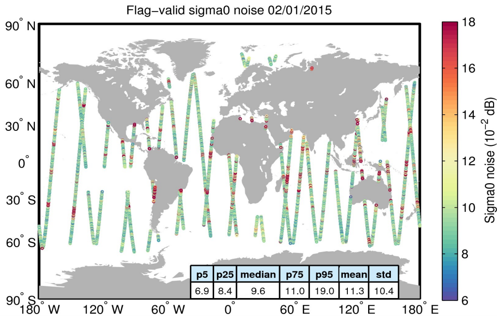
Figure 26. Geographical distribution of flag-valid 20-Hz sigma0 measurement noise over oceans and lakes for 02/01/2015. The statistical values shown in the table refer to the sigma0 noise and are calculated over all measurements shown in the figure.
