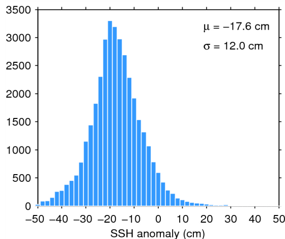
Figure 11. Histogram of science-valid SSH anomaly over oceans and lakes for 01/01/2015. The mean ( \mu ) and standard deviation ( \sigma ) are also shown. Note that values outside [-50 50] cm are excluded from the histogram for the sake of readability but not from the computation of \mu and \sigma .
