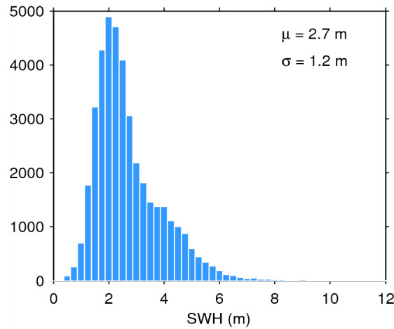
Figure 17. Histogram of flag-valid SWH over oceans and lakes for 01/01/2015. The mean ( \mu ) and standard deviation ( \sigma ) are also shown. Note that values larger than 12 m are excluded from the histogram for the sake of readability but not from the computation of \mu and \sigma .
