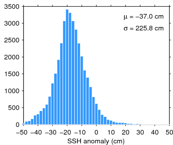
Figure 7. Histogram of flag-valid SSH anomaly over oceans and lakes for 01/01/2015. The mean ( \mu ) and standard deviation ( \sigma ) are also shown. Note that values outside [-50 50] cm are excluded from the histogram for the sake of readability but not from the computation of \mu and \sigma .
