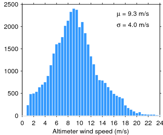
Figure 33. Histogram of flag-valid wind over oceans and lakes for 01/01/2015. The mean ( \mu ) and standard deviation ( \sigma ) are also shown. Note that values larger than 24 m/s are excluded from the histogram for the sake of readability but not from the computation of \mu and \sigma .
