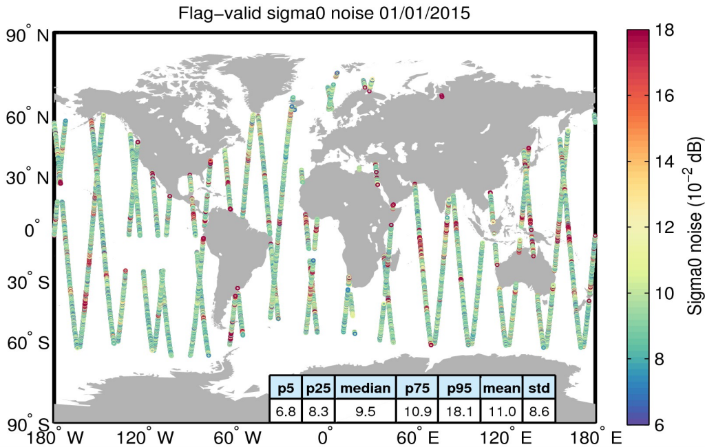
Figure 26. Geographical distribution of flag-valid 20-Hz sigma0 measurement noise over oceans and lakes for 01/01/2015. The statistical values shown in the table refer to the sigma0 noise and are calculated over all measurements shown in the figure.
