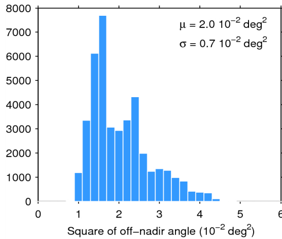
Figure 39. Histogram of flag-valid mispointing over oceans and lakes for 01/01/2015. The mean ( \mu ) and standard deviation ( \sigma ) are also shown. Note that values than 6 \cdot 10^{-2} \text{ deg}^2 are excluded from the histogram for the sake of readability but not from the computation of \mu and \sigma .
