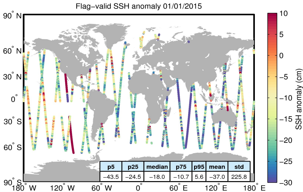
Figure 5. Geographical distribution of flag-valid 1-Hz SSH anomaly data over oceans and lakes for 01/01/2015. The statistical values shown in the table refer to the SSH anomaly in cm and are calculated over all measurements shown in the figure.
