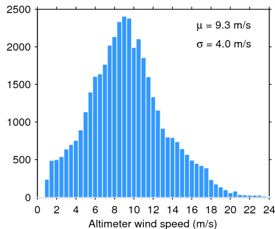
Figure 35. Histogram of science-valid wind over oceans and lakes for 01/01/2015. The mean ( \mu ) and standard deviation ( \sigma ) are also shown. Note that values larger than 24 m/s are excluded from the histogram for the sake of readability but not from the computation of \mu and \sigma .
