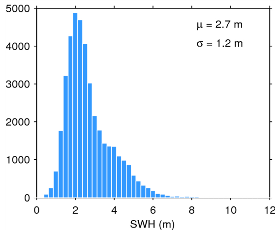
Figure 20. Histogram of science-valid SWH over oceans and lakes for 01/01/2015. The mean ( \mu ) and standard deviation ( \sigma ) are also shown. Note that values larger than 12 m are excluded from the histogram for the sake of readability but not from the computation of \mu and \sigma .
