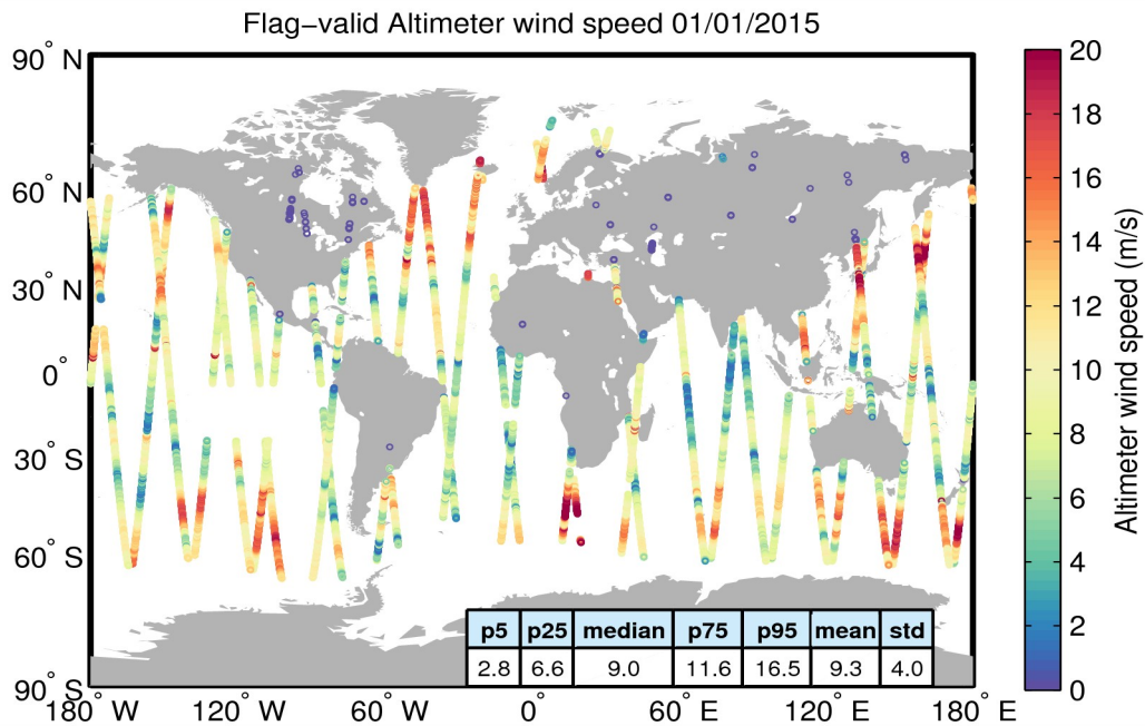
Figure 31. Geographical distribution of flag-valid wind data over oceans and lakes for 01/01/2015. The statistical values shown in the table refer to the wind in m/s and are calculated over all measurements shown in the figure.
