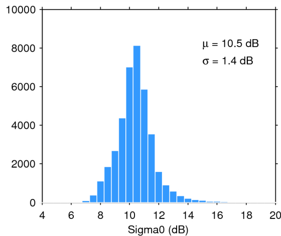
Figure 28. Histogram of science-valid sigma0 over oceans and lakes for 01/01/2015. The mean ( \mu ) and standard deviation ( \sigma ) are also shown. Note that values outside [4 20] dB are excluded from the histogram for the sake of readability but not from the computation of \mu and \sigma .
