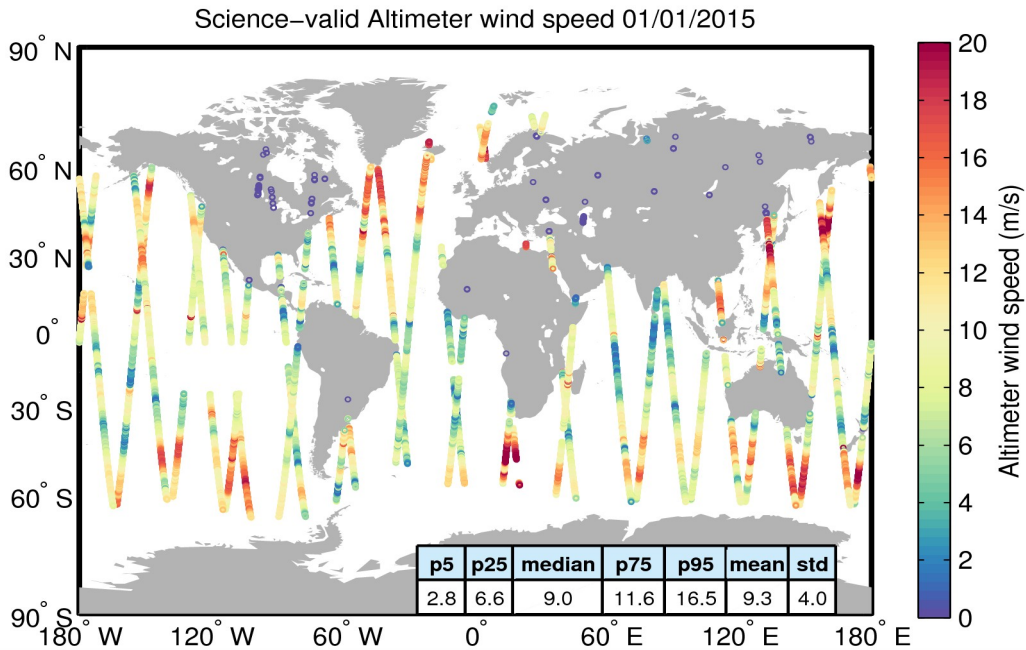
Figure 34. Geographical distribution of science-valid wind data over oceans and lakes for 01/01/2015. The statistical values shown in the table refer to the wind in m/s and are calculated over all measurements shown in the figure. Gray circles denote records that have been rejected based on the editing criteria described in Table 5.
