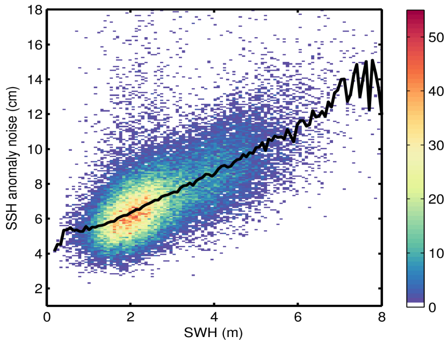
Figure 9. 2D histogram showing flag-valid SSH anomaly noise as a function of SWH for 01/01/2015. The black line denotes the median SSH anomaly as a function of SWH.
