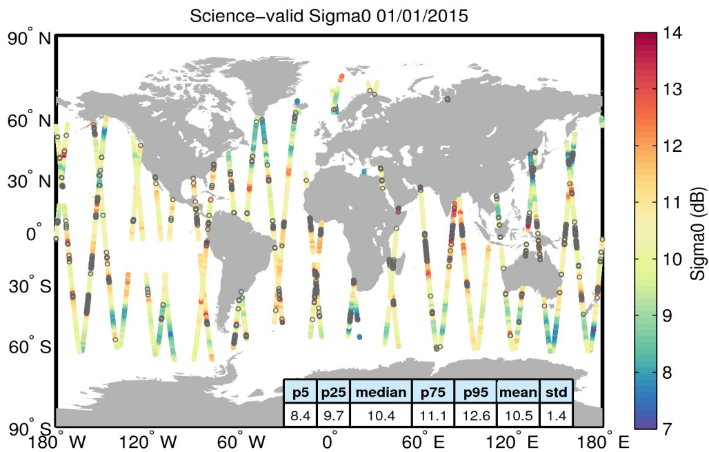
Figure 27. Geographical distribution of science-valid sigma0 data over oceans and lakes for 01/01/2015. The statistical values shown in the table refer to the sigma0 in dB and are calculated over all measurements shown in the figure. Gray circles denote records that have been rejected based on the editing criteria described in Table 4.
