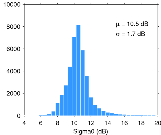
Figure 25. Histogram of flag-valid sigma0 over oceans and lakes for 01/01/2015. The mean ( \mu ) and standard deviation ( \sigma ) are also shown. Note that values outside [4 20] dB are excluded from the histogram for the sake of readability but not from the computation of \mu and \sigma .
