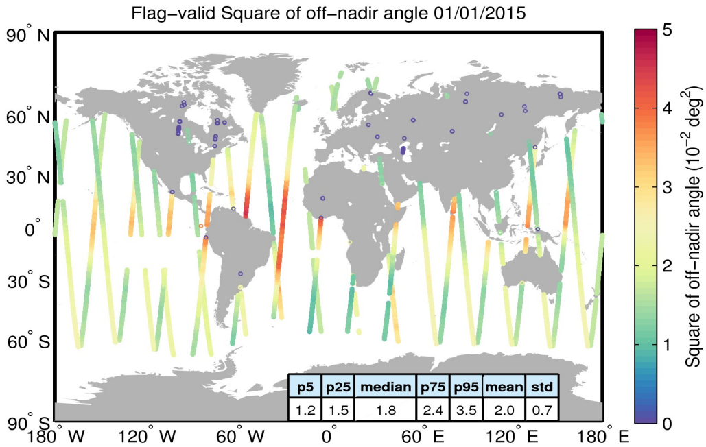
Figure 37. Geographical distribution of flag-valid mispointing data over oceans and lakes for 01/01/2015. The statistical values shown in the table refer to the mispointing in 10^{-2} \text{ deg}^2 and are calculated over all measurements shown in the figure.
