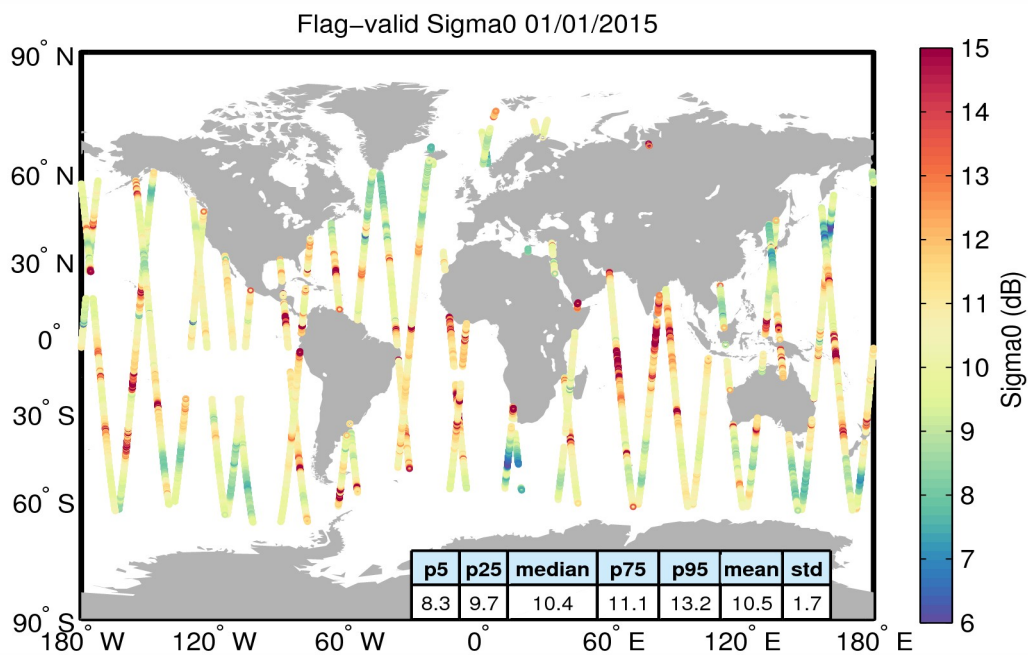
Figure 23. Geographical distribution of flag-valid sigma0 data over oceans and lakes for 01/01/2015. The statistical values shown in the table refer to the sigma0 in dB and are calculated over all measurements shown in the figure.
