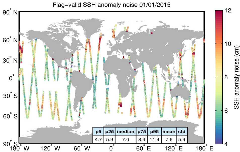
Figure 8. Geographical distribution of flag-valid 20-Hz SSH anomaly measurement noise over oceans and lakes for 01/01/2015. The statistical values shown in the table refer to the SSH anomaly noise and are calculated over all measurements shown in the figure.
