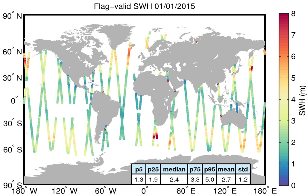
Figure 15. Geographical distribution of flag-valid SWH data over oceans and lakes for 01/01/2015. The statistical values shown in the figure refer to the SWH in m and are calculated over all measurements shown in the figure.
