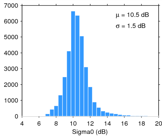
Figure 28. Histogram of science-valid sigma0 over oceans and lakes for 31/12/2014. The mean ( \mu ) and standard deviation ( \sigma ) are also shown. Note that values outside [4 20] dB are excluded from the histogram for the sake of readability but not from the computation of \mu and \sigma .
