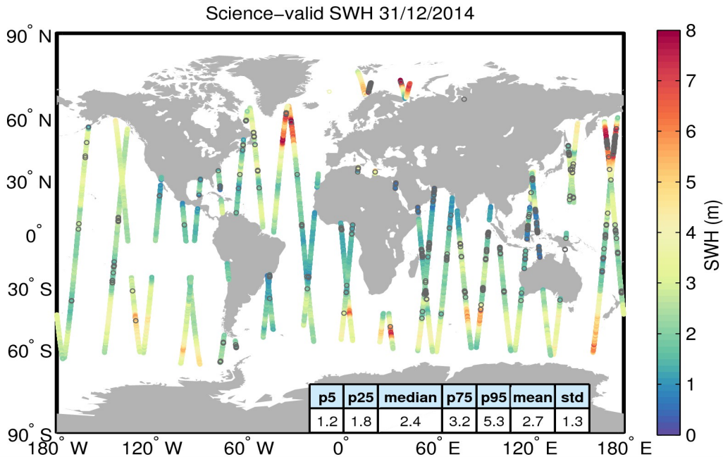
Figure 19. Geographical distribution of science-valid SWH data over oceans and lakes for 31/12/2014. The statistical values shown in the table refer to the SWH in m and are calculated over all measurements shown in the figure. Gray circles denote records that have been rejected based on the editing criteria described in Table 3.
