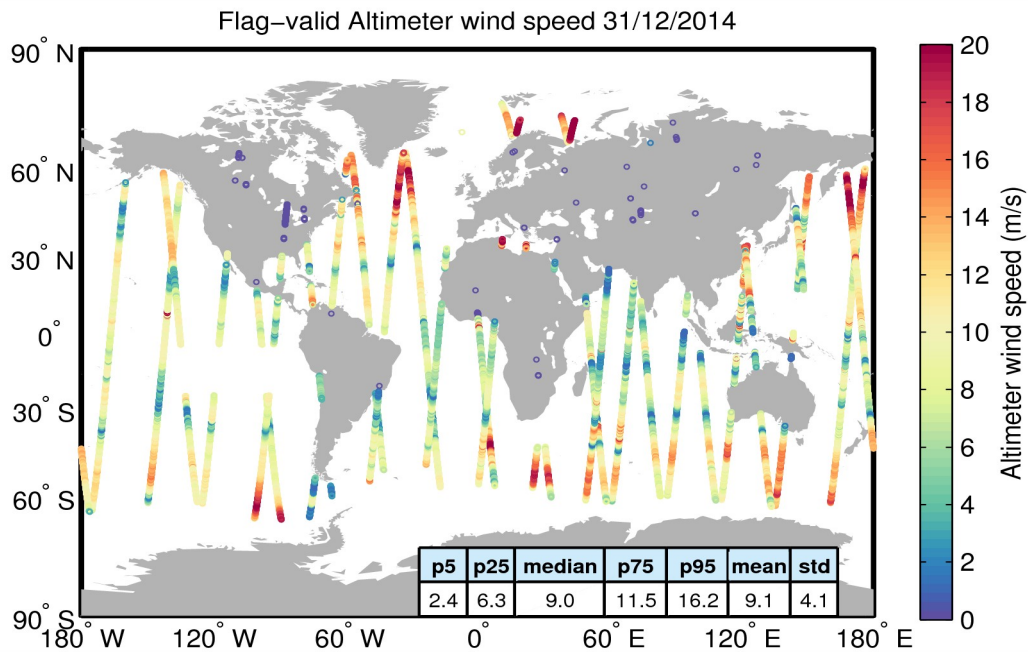
Figure 31. Geographical distribution of flag-valid wind data over oceans and lakes for 31/12/2014. The statistical values shown in the table refer to the wind in m/s and are calculated over all measurements shown in the figure.
