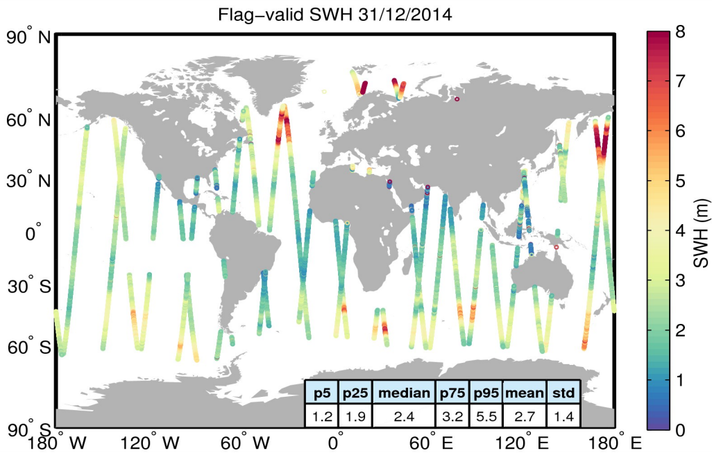
Figure 15. Geographical distribution of flag-valid SWH data over oceans and lakes for 31/12/2014. The statistical values shown in the table refer to the SWH in m and are calculated over all measurements shown in the figure.
