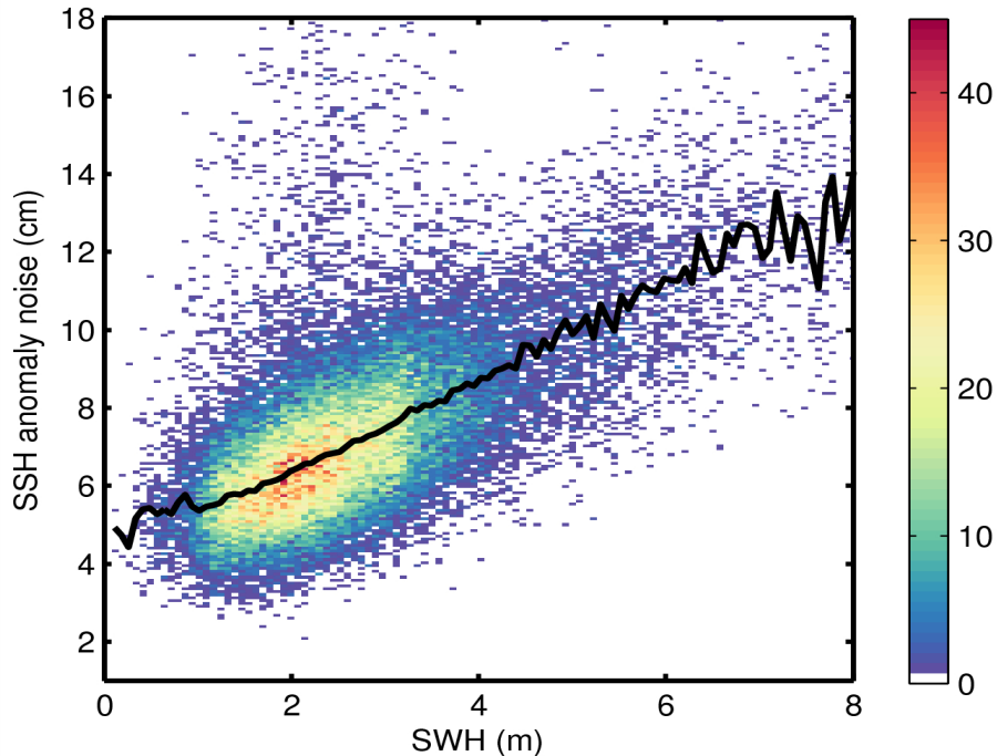
Figure 9. 2D histogram showing flag-valid SSH anomaly noise as a function of SWH for 31/12/2014. The black line denotes the median SSH anomaly as a function of SWH.
