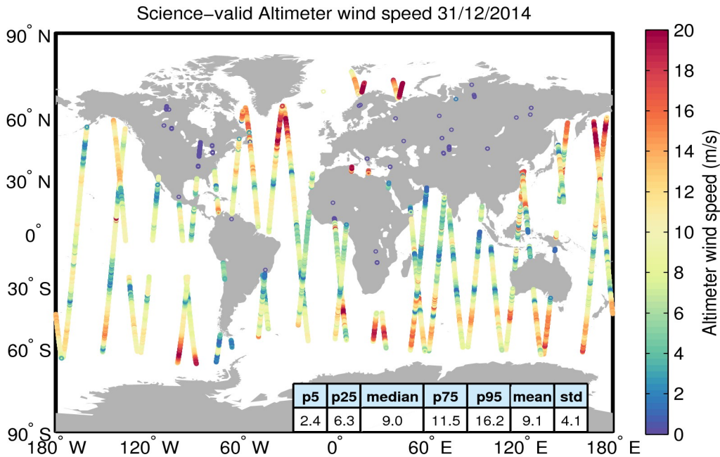
Figure 34. Geographical distribution of science-valid wind data over oceans and lakes for 31/12/2014. The statistical values shown in the table refer to the wind in m/s and are calculated over all measurements shown in the figure. Gray circles denote records that have been rejected based on the editing criteria described in Table 5.
