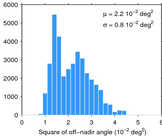
Figure 39. Histogram of flag-valid mispointing over oceans and lakes for 31/12/2014. The mean ( \mu ) and standard deviation ( \sigma ) are also shown. Note that values than 6 \cdot 10^{-2} \text{ deg}^2 are excluded from the histogram for the sake of readability but not from the computation of \mu and \sigma .
