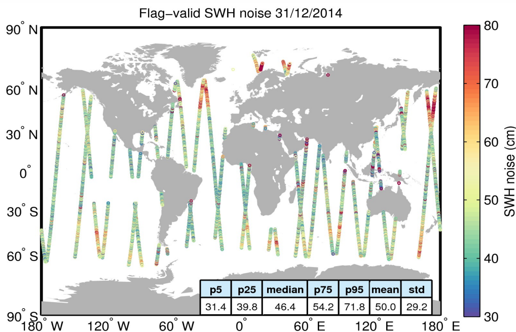
Figure 18. Geographical distribution of flag-valid 20-Hz SWH measurement noise over oceans and lakes for 31/12/2014. The statistical values shown in the figure refer to the SWH noise and are calculated over all measurements shown in the figure.
