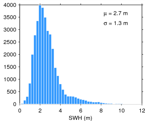
Figure 20. Histogram of science-valid SWH over oceans and lakes for 31/12/2014. The mean ( \mu ) and standard deviation ( \sigma ) are also shown. Note that values larger than 12 m are excluded from the histogram for the sake of readability but not from the computation of \mu and \sigma .
