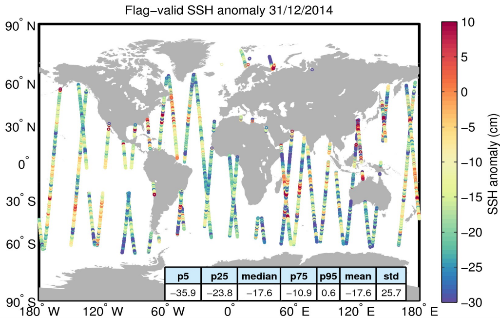
Figure 5. Geographical distribution of flag-valid 1-Hz SSH anomaly data over oceans and lakes for 31/12/2014. The statistical values shown in the table refer to the SSH anomaly in cm and are calculated over all measurements shown in the figure.
