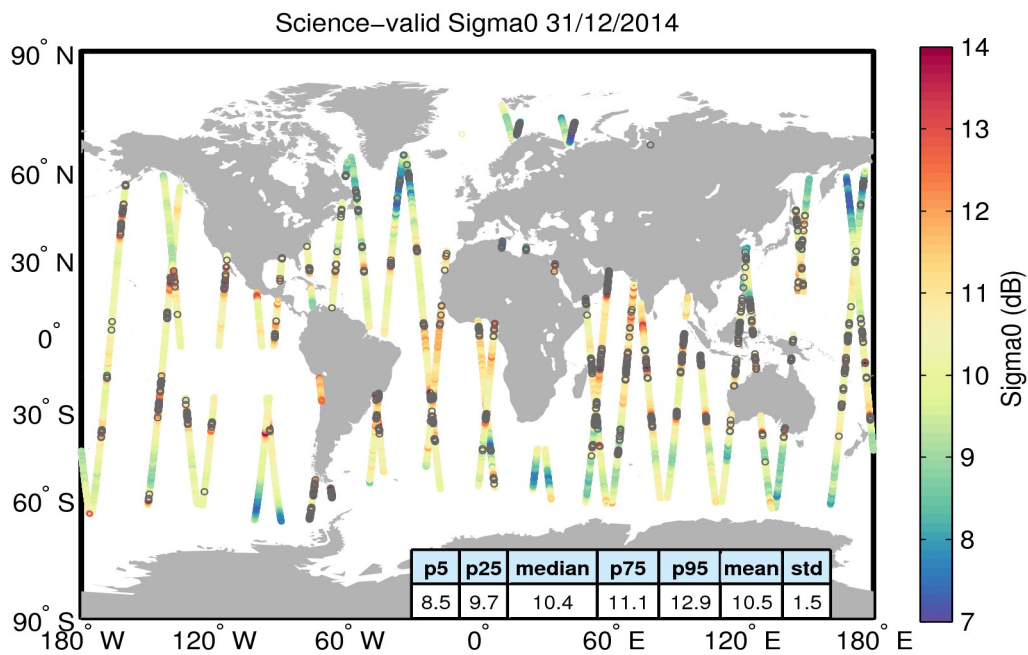
Figure 27. Geographical distribution of science-valid sigma0 data over oceans and lakes for 31/12/2014. The statistical values shown in the table refer to the sigma0 in dB and are calculated over all measurements shown in the figure. Gray circles denote records that have been rejected based on the editing criteria described in Table 4.
