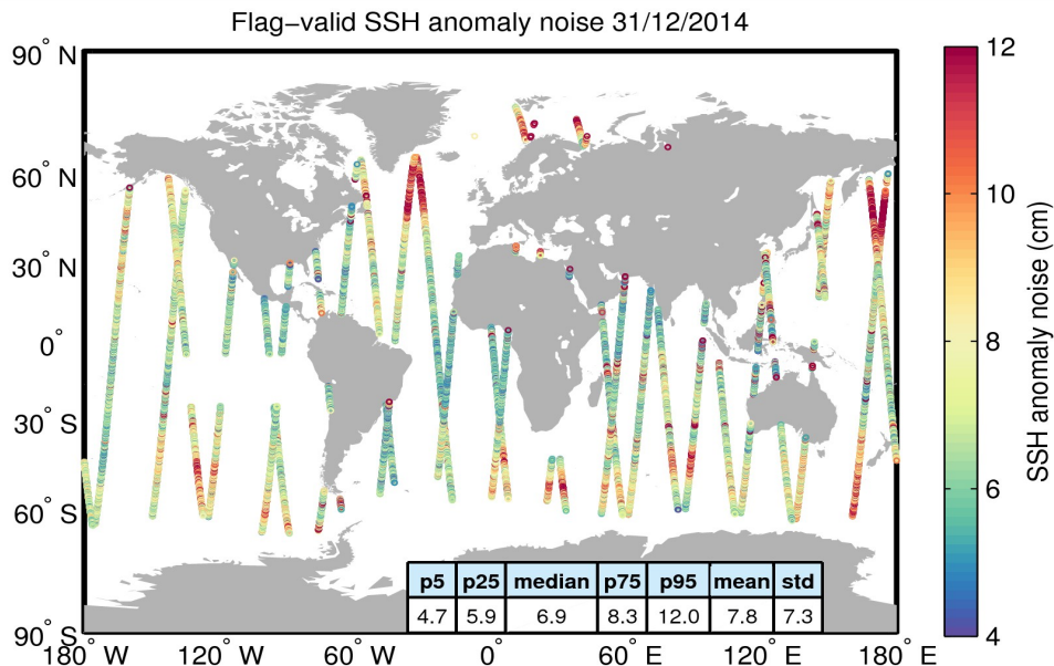
Figure 8. Geographical distribution of flag-valid 20-Hz SSH anomaly measurement noise over oceans and lakes for 31/12/2014. The statistical values shown in the table refer to the SSH anomaly noise and are calculated over all measurements shown in the figure.
