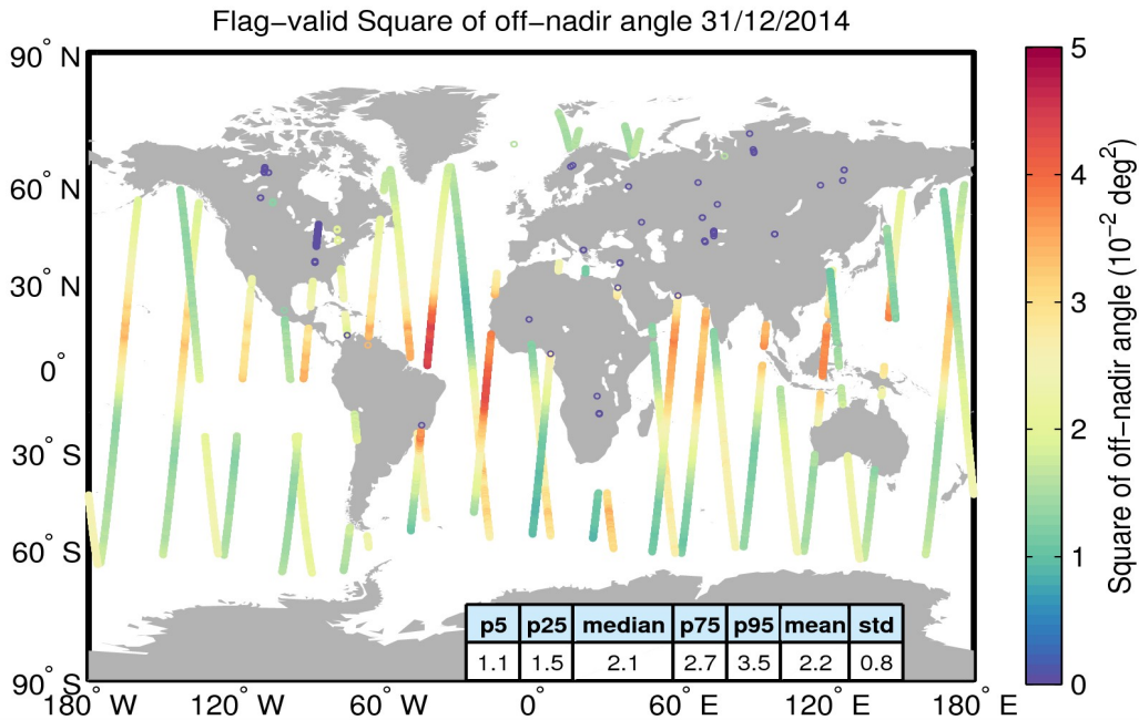
Figure 37. Geographical distribution of flag-valid mispointing data over oceans and lakes for 31/12/2014. The statistical values shown in the table refer to the mispointing in 10^{-2} \text{ deg}^2 and are calculated over all measurements shown in the figure.
