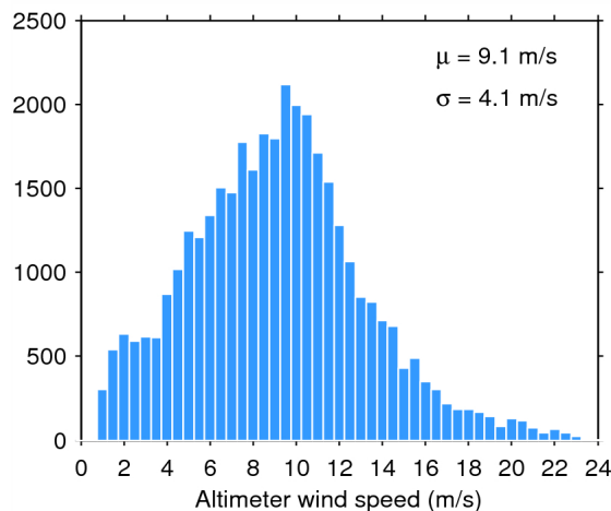
Figure 33. Histogram of flag-valid wind over oceans and lakes for 31/12/2014. The mean ( \mu ) and standard deviation ( \sigma ) are also shown. Note that values larger than 24 m/s are excluded from the histogram for the sake of readability but not from the computation of \mu and \sigma .
