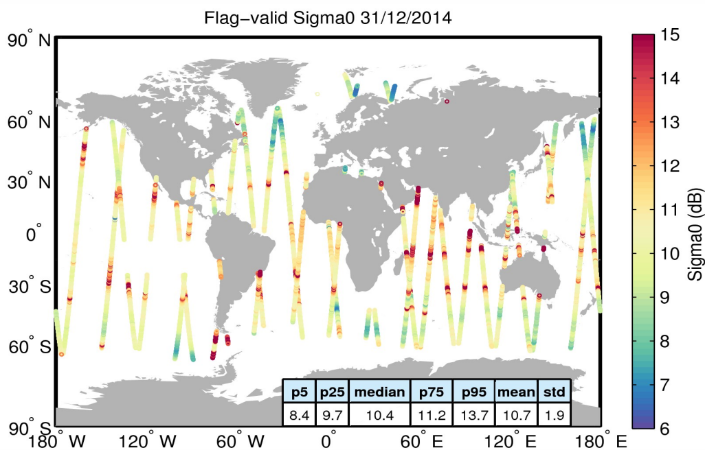
Figure 23. Geographical distribution of flag-valid sigma0 data over oceans and lakes for 31/12/2014. The statistical values shown in the table refer to the sigma0 in dB and are calculated over all measurements shown in the figure.
