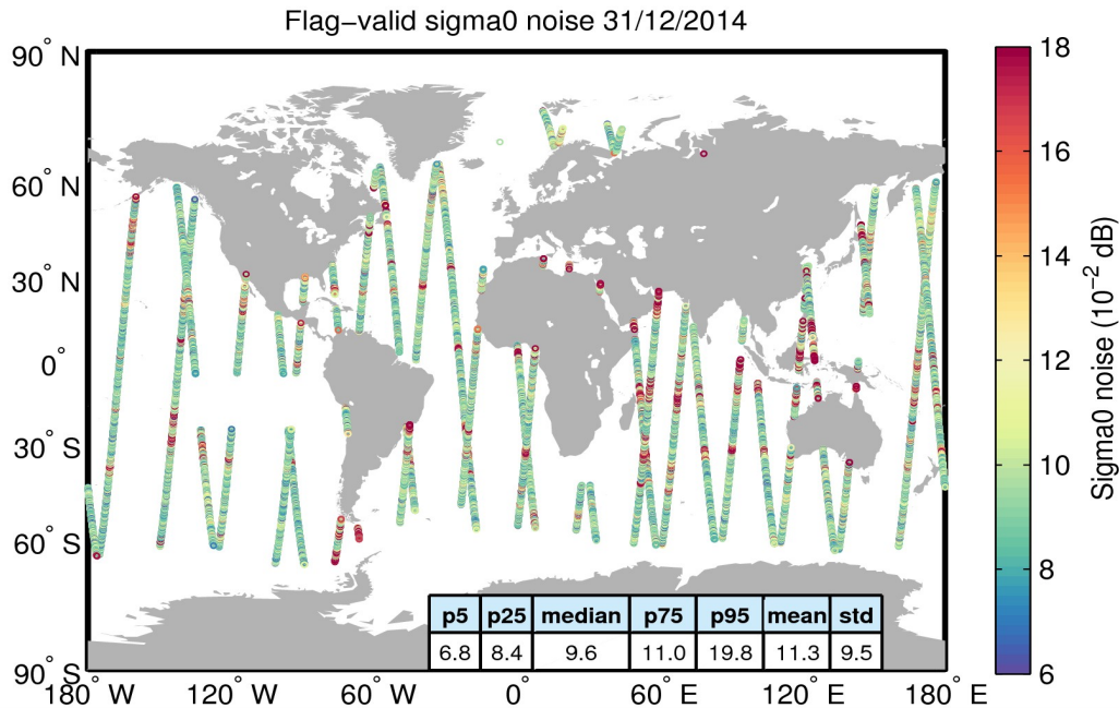
Figure 26. Geographical distribution of flag-valid 20-Hz sigma0 measurement noise over oceans and lakes for 31/12/2014. The statistical values shown in the table refer to the sigma0 noise and are calculated over all measurements shown in the figure.
