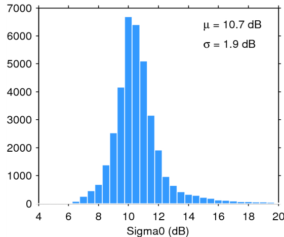
Figure 25. Histogram of flag-valid sigma0 over oceans and lakes for 31/12/2014. The mean ( \mu ) and standard deviation ( \sigma ) are also shown. Note that values outside [4 20] dB are excluded from the histogram for the sake of readability but not from the computation of \mu and \sigma .
