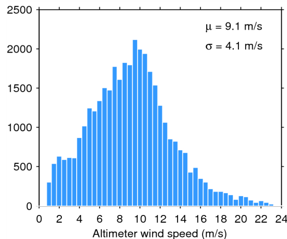
Figure 35. Histogram of science-valid wind over oceans and lakes for 31/12/2014. The mean ( \mu ) and standard deviation ( \sigma ) are also shown. Note that values larger than 24 m/s are excluded from the histogram for the sake of readability but not from the computation of \mu and \sigma .
