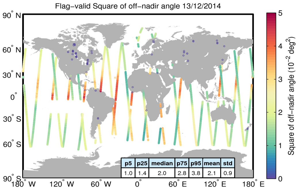
Figure 37. Geographical distribution of flag-valid mispointing data over oceans and lakes for 13/12/2014. The statistical values shown in the table refer to the mispointing in 10^{-2} \text{ deg}^2 and are calculated over all measurements shown in the figure.
