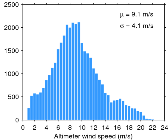
Figure 33. Histogram of flag-valid wind over oceans and lakes for 13/12/2014. The mean ( \mu ) and standard deviation ( \sigma ) are also shown. Note that values larger than 24 m/s are excluded from the histogram for the sake of readability but not from the computation of \mu and \sigma .
