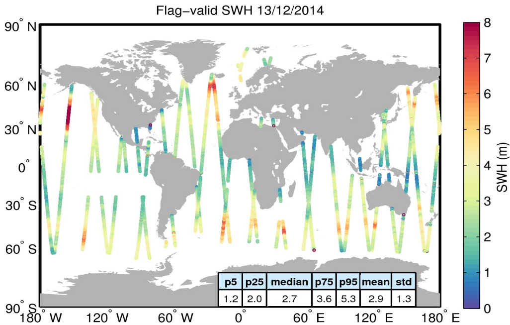
Figure 15. Geographical distribution of flag-valid SWH data over oceans and lakes for 13/12/2014. The statistical values shown in the table refer to the SWH in m and are calculated over all measurements shown in the figure.
