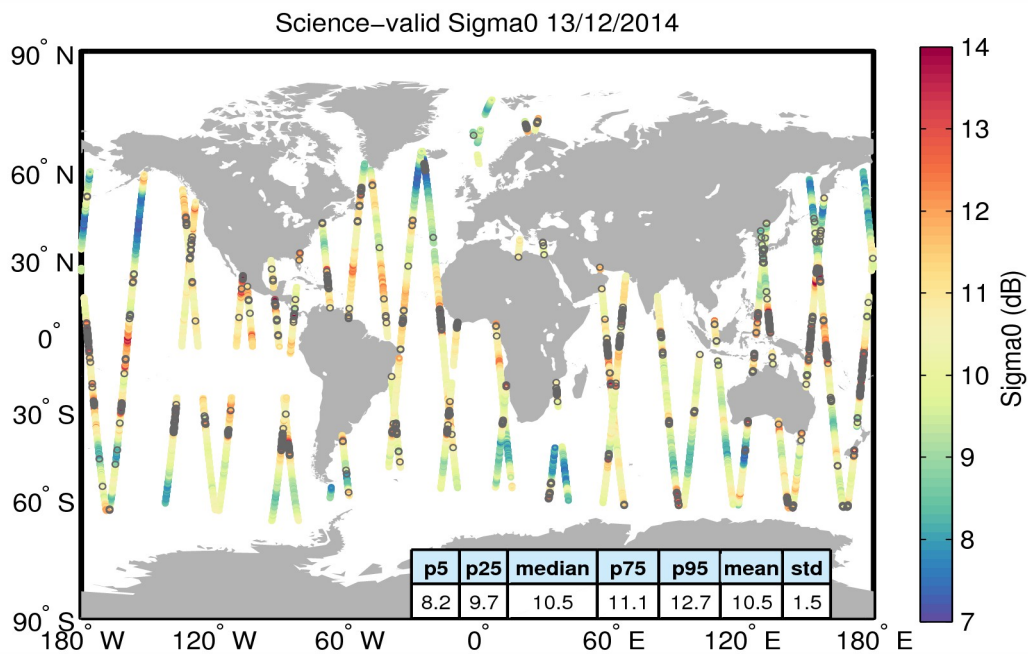
Figure 27. Geographical distribution of science-valid sigma0 data over oceans and lakes for 13/12/2014. The statistical values shown in the table refer to the sigma0 in dB and are calculated over all measurements shown in the figure. Gray circles denote records that have been rejected based on the editing criteria described in Table 4.
