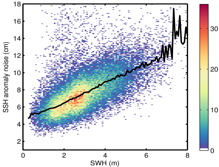
Figure 9. 2D histogram showing flag-valid SSH anomaly noise as a function of SWH for 13/12/2014. The black line denotes the median SSH anomaly as a function of SWH.
