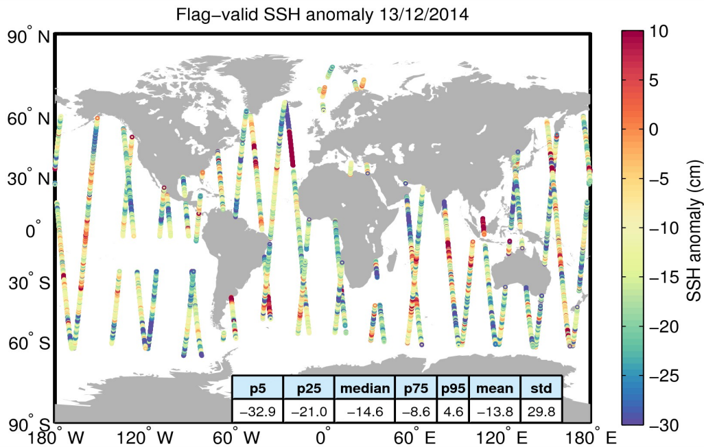
Figure 5. Geographical distribution of flag-valid 1-Hz SSH anomaly data over oceans and lakes for 13/12/2014. The statistical values shown in the table refer to the SSH anomaly in cm and are calculated over all measurements shown in the figure.
