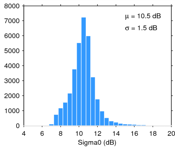
Figure 28. Histogram of science-valid sigma0 over oceans and lakes for 13/12/2014. The mean ( \mu ) and standard deviation ( \sigma ) are also shown. Note that values outside [4 20] dB are excluded from the histogram for the sake of readability but not from the computation of \mu and \sigma .
