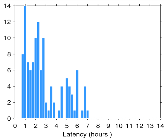
Figure 2. Histogram of the data latency for 13/12/2014. The y-axis denotes the number of files that are made available with a delay of x-hours with respect to the mean time of the records stored in the file.
