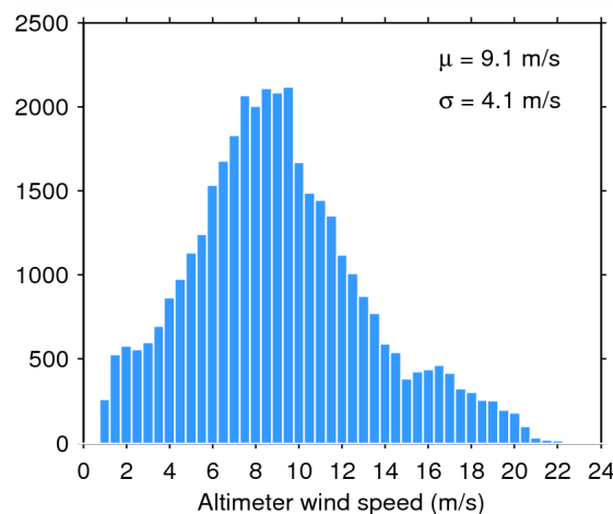
Figure 35. Histogram of science-valid wind over oceans and lakes for 13/12/2014. The mean ( \mu ) and standard deviation ( \sigma ) are also shown. Note that values larger than 24 m/s are excluded from the histogram for the sake of readability but not from the computation of \mu and \sigma .
