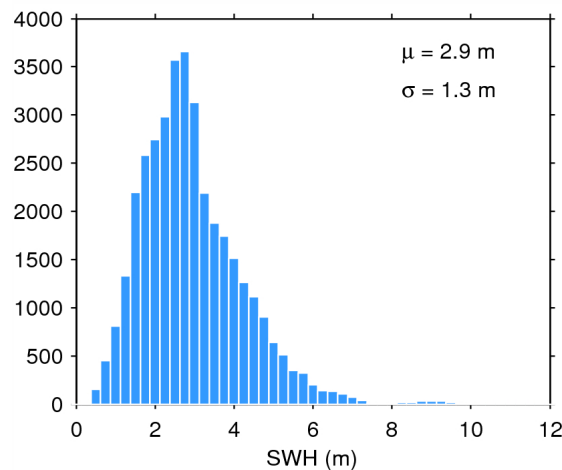
Figure 20. Histogram of science-valid SWH over oceans and lakes for 13/12/2014. The mean ( \mu ) and standard deviation ( \sigma ) are also shown. Note that values larger than 12 m are excluded from the histogram for the sake of readability but not from the computation of \mu and \sigma .
