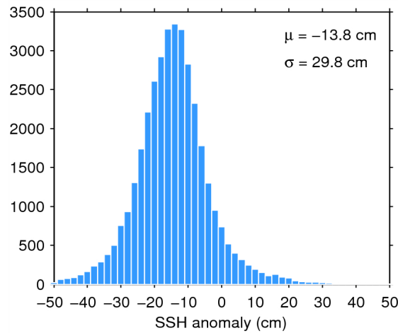
Figure 7. Histogram of flag-valid SSH anomaly over oceans and lakes for 13/12/2014. The mean ( \mu ) and standard deviation ( \sigma ) are also shown. Note that values outside [-50\ 50] cm are excluded from the histogram for the sake of readability but not from the computation of \mu and \sigma .
