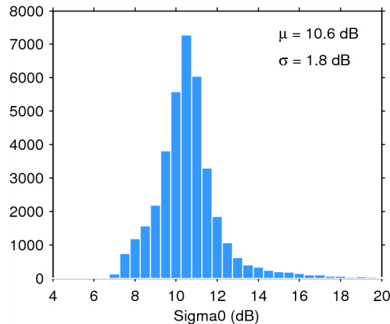
Figure 25. Histogram of flag-valid sigma0 over oceans and lakes for 13/12/2014. The mean ( \mu ) and standard deviation ( \sigma ) are also shown. Note that values outside [4 20] dB are excluded from the histogram for the sake of readability but not from the computation of \mu and \sigma .
