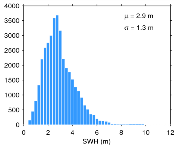
Figure 17. Histogram of flag-valid SWH over oceans and lakes for 13/12/2014. The mean ( \mu ) and standard deviation ( \sigma ) are also shown. Note that values larger than 12 m are excluded from the histogram for the sake of readability but not from the computation of \mu and \sigma .
