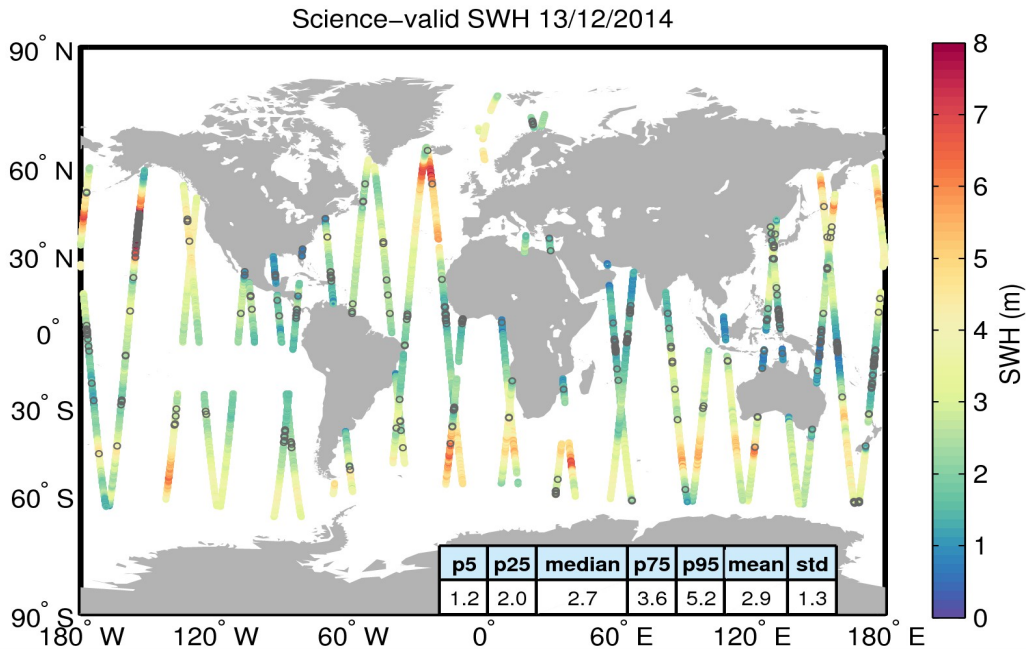
Figure 19. Geographical distribution of science-valid SWH data over oceans and lakes for 13/12/2014. The statistical values shown in the table refer to the SWH in m and are calculated over all measurements shown in the figure. Gray circles denote records that have been rejected based on the editing criteria described in Table 3.
