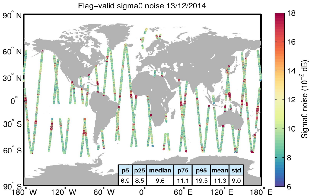
Figure 26. Geographical distribution of flag-valid 20-Hz sigma0 measurement noise over oceans and lakes for 13/12/2014. The statistical values shown in the table refer to the sigma0 noise and are calculated over all measurements shown in the figure.
