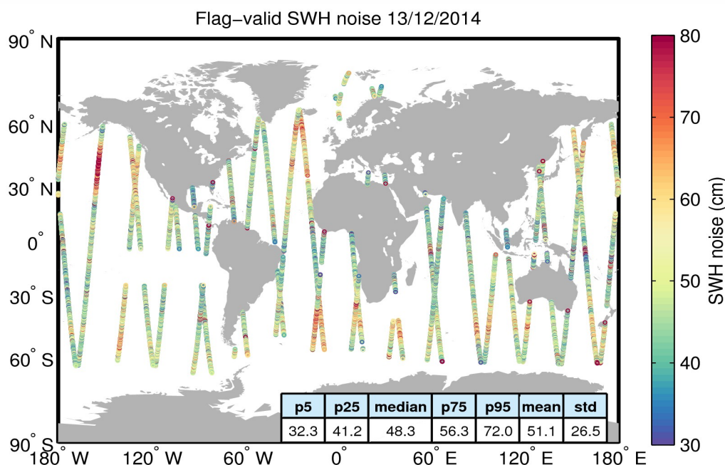
Figure 18. Geographical distribution of flag-valid 20-Hz SWH measurement noise over oceans and lakes for 13/12/2014. The statistical values shown in the figure refer to the SWH noise and are calculated over all measurements shown in the figure.
