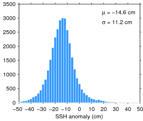
Figure 11. Histogram of science-valid SSH anomaly over oceans and lakes for 13/12/2014. The mean ( \mu ) and standard deviation ( \sigma ) are also shown. Note that values outside [-50 50] cm are excluded from the histogram for the sake of readability but not from the computation of \mu and \sigma .
