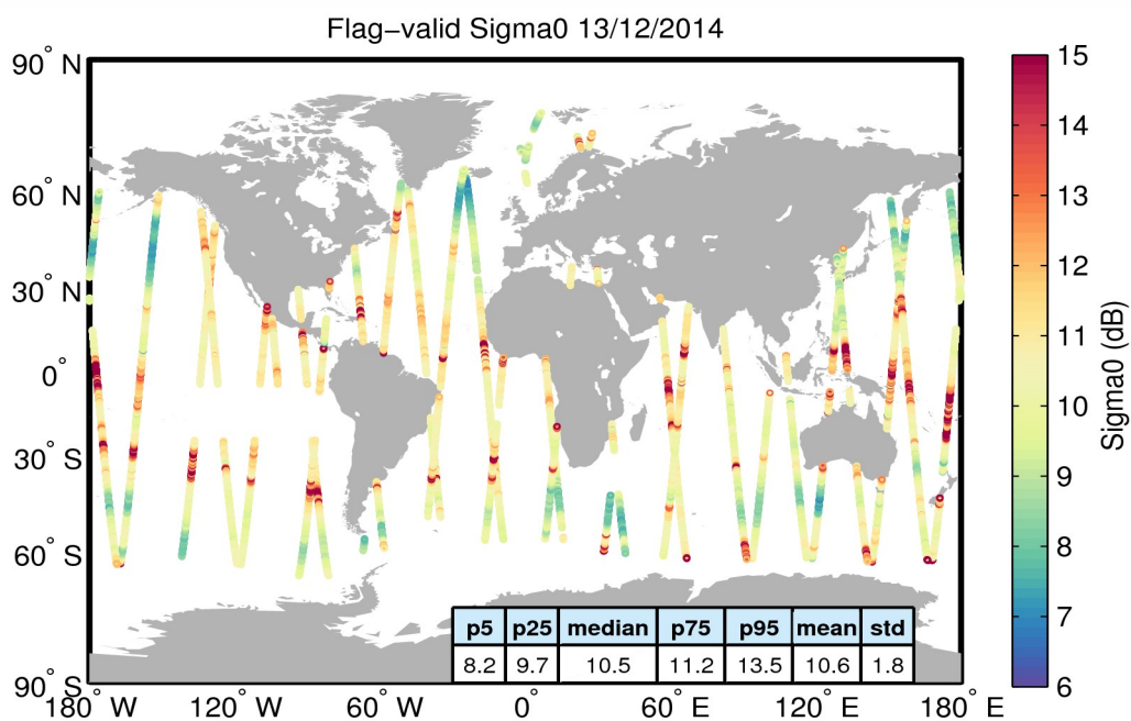
Figure 23. Geographical distribution of flag-valid sigma0 data over oceans and lakes for 13/12/2014. The statistical values shown in the table refer to the sigma0 in dB and are calculated over all measurements shown in the figure.
