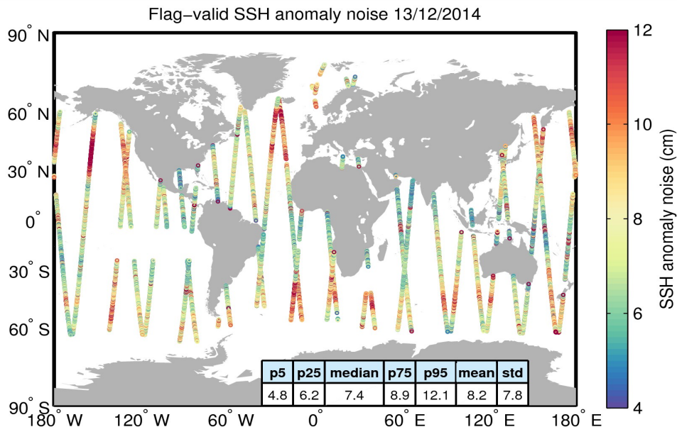
Figure 8. Geographical distribution of flag-valid 20-Hz SSH anomaly measurement noise over oceans and lakes for 13/12/2014. The statistical values shown in the table refer to the SSH anomaly noise and are calculated over all measurements shown in the figure.
