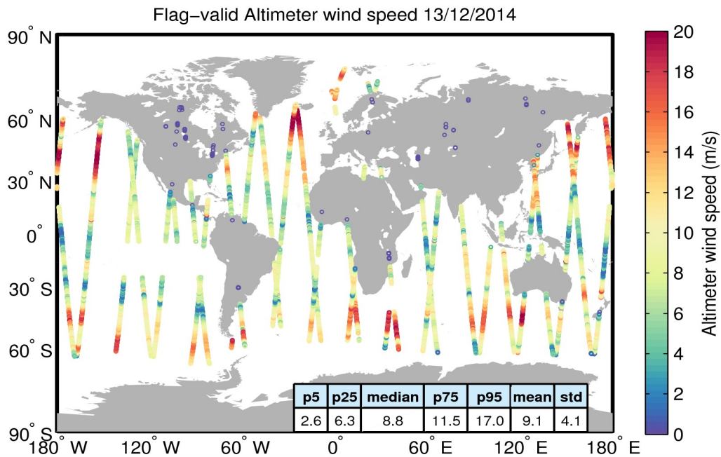
Figure 31. Geographical distribution of flag-valid wind data over oceans and lakes for 13/12/2014. The statistical values shown in the table refer to the wind in m/s and are calculated over all measurements shown in the figure.
