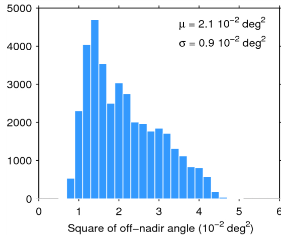
Figure 39. Histogram of flag-valid mispointing over oceans and lakes for 13/12/2014. The mean ( \mu ) and standard deviation ( \sigma ) are also shown. Note that values than 6 \cdot 10^{-2} \text{ deg}^2 are excluded from the histogram for the sake of readability but not from the computation of \mu and \sigma .
