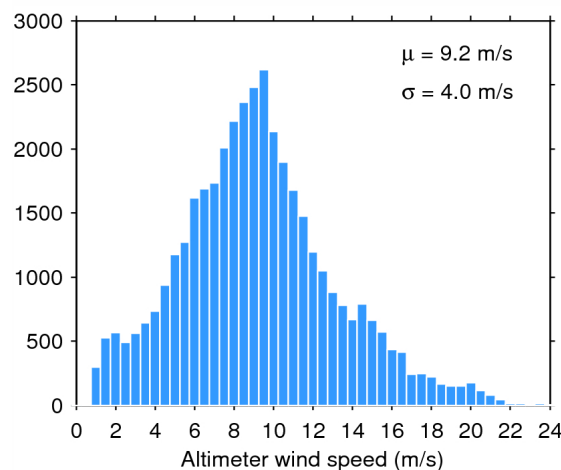
Figure 35. Histogram of science-valid wind over oceans and lakes for 05/12/2014. The mean ( \mu ) and standard deviation ( \sigma ) are also shown. Note that values larger than 24 m/s are excluded from the histogram for the sake of readability but not from the computation of \mu and \sigma .
