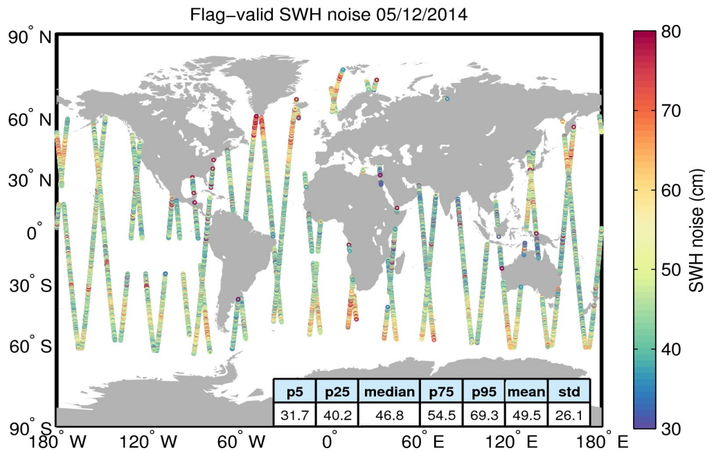
Figure 18. Geographical distribution of flag-valid 20-Hz SWH measurement noise over oceans and lakes for 05/12/2014. The statistical values shown in the figure refer to the SWH noise and are calculated over all measurements shown in the figure.
