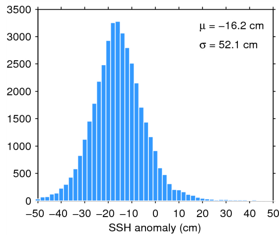
Figure 7. Histogram of flag-valid SSH anomaly over oceans and lakes for 05/12/2014. The mean ( \mu ) and standard deviation ( \sigma ) are also shown. Note that values outside [-50 50] cm are excluded from the histogram for the sake of readability but not from the computation of \mu and \sigma .
