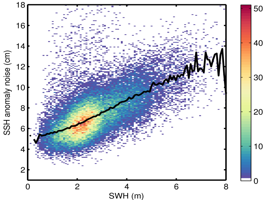
Figure 9. 2D histogram showing flag-valid SSH anomaly noise as a function of SWH for 05/12/2014. The black line denotes the median SSH anomaly as a function of SWH.
