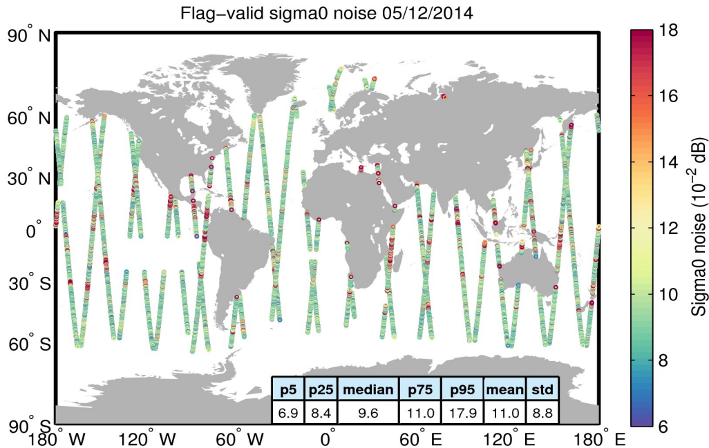
Figure 26. Geographical distribution of flag-valid 20-Hz sigma0 measurement noise over oceans and lakes for 05/12/2014. The statistical values shown in the table refer to the sigma0 noise and are calculated over all measurements shown in the figure.
