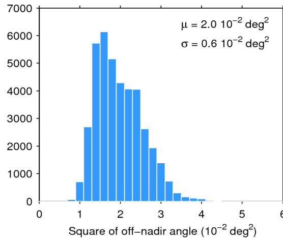
Figure 39. Histogram of flag-valid mispointing over oceans and lakes for 05/12/2014. The mean ( \mu ) and standard deviation ( \sigma ) are also shown. Note that values than 6 \cdot 10^{-2} \text{ deg}^2 are excluded from the histogram for the sake of readability but not from the computation of \mu and \sigma .
