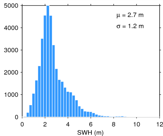
Figure 20. Histogram of science-valid SWH over oceans and lakes for 05/12/2014. The mean ( \mu ) and standard deviation ( \sigma ) are also shown. Note that values larger than 12 m are excluded from the histogram for the sake of readability but not from the computation of \mu and \sigma .
