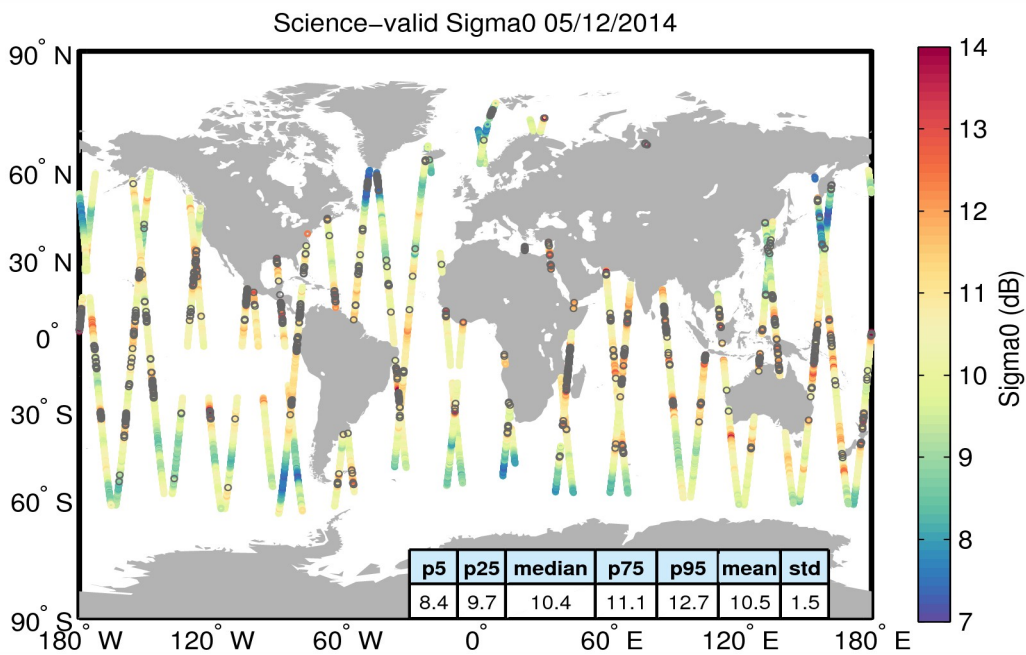
Figure 27. Geographical distribution of science-valid sigma0 data over oceans and lakes for 05/12/2014. The statistical values shown in the table refer to the sigma0 in dB and are calculated over all measurements shown in the figure. Gray circles denote records that have been rejected based on the editing criteria described in Table 4.
