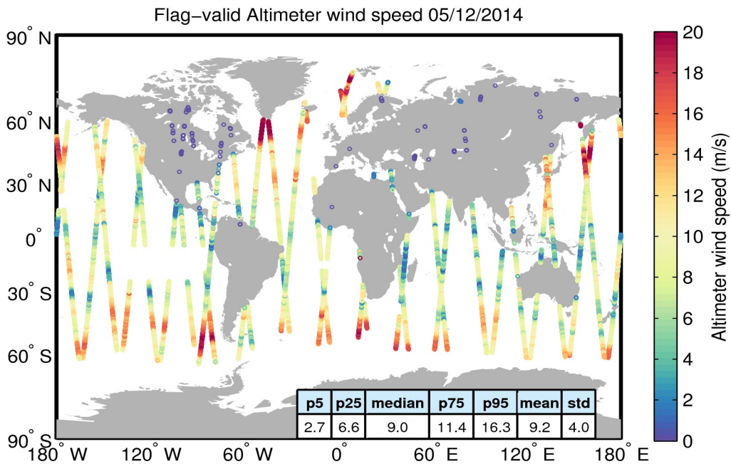
Figure 31. Geographical distribution of flag-valid wind data over oceans and lakes for 05/12/2014. The statistical values shown in the table refer to the wind in m/s and are calculated over all measurements shown in the figure.
