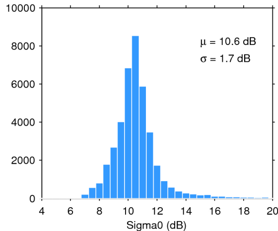
Figure 25. Histogram of flag-valid sigma0 over oceans and lakes for 05/12/2014. The mean ( \mu ) and standard deviation ( \sigma ) are also shown. Note that values outside [4 20] dB are excluded from the histogram for the sake of readability but not from the computation of \mu and \sigma .
