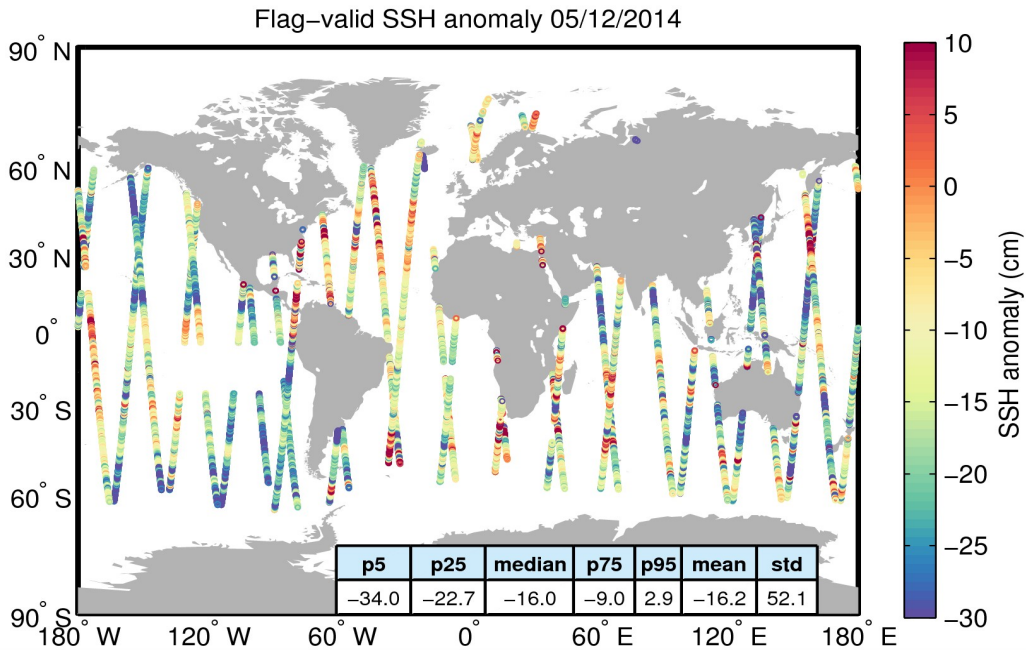
Figure 5. Geographical distribution of flag-valid 1-Hz SSH anomaly data over oceans and lakes for 05/12/2014. The statistical values shown in the table refer to the SSH anomaly in cm and are calculated over all measurements shown in the figure.
