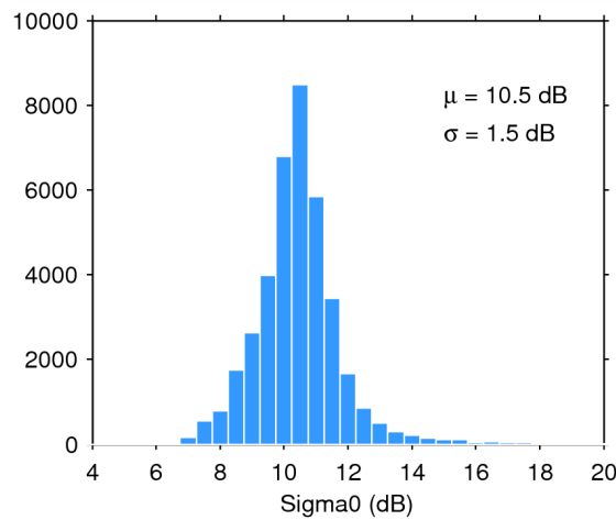
Figure 28. Histogram of science-valid sigma0 over oceans and lakes for 05/12/2014. The mean ( \mu ) and standard deviation ( \sigma ) are also shown. Note that values outside [4 20] dB are excluded from the histogram for the sake of readability but not from the computation of \mu and \sigma .
