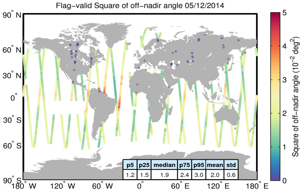
Figure 37. Geographical distribution of flag-valid mispointing data over oceans and lakes for 05/12/2014. The statistical values shown in the table refer to the mispointing in 10^{-2} \text{ deg}^2 and are calculated over all measurements shown in the figure.
