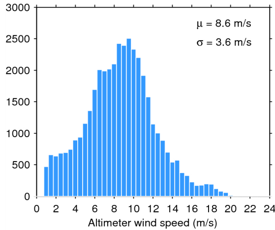
Figure 33. Histogram of flag-valid wind over oceans and lakes for 28/11/2014. The mean ( \mu ) and standard deviation ( \sigma ) are also shown. Note that values larger than 24 m/s are excluded from the histogram for the sake of readability but not from the computation of \mu and \sigma .
