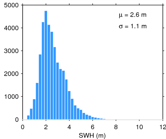
Figure 20. Histogram of science-valid SWH over oceans and lakes for 28/11/2014. The mean ( \mu ) and standard deviation ( \sigma ) are also shown. Note that values larger than 12 m are excluded from the histogram for the sake of readability but not from the computation of \mu and \sigma .
