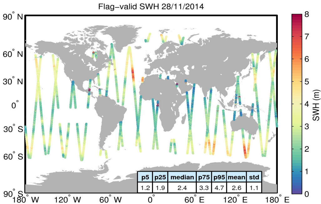
Figure 15. Geographical distribution of flag-valid SWH data over oceans and lakes for 28/11/2014. The statistical values shown in the table refer to the SWH in m and are calculated over all measurements shown in the figure.
