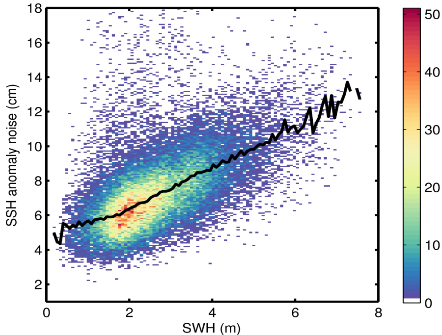
Figure 9. 2D histogram showing flag-valid SSH anomaly noise as a function of SWH for 28/11/2014. The black line denotes the median SSH anomaly as a function of SWH.
