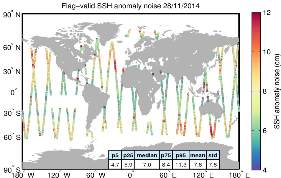
Figure 8. Geographical distribution of flag-valid 20-Hz SSH anomaly measurement noise over oceans and lakes for 28/11/2014. The statistical values shown in the table refer to the SSH anomaly noise and are calculated over all measurements shown in the figure.
