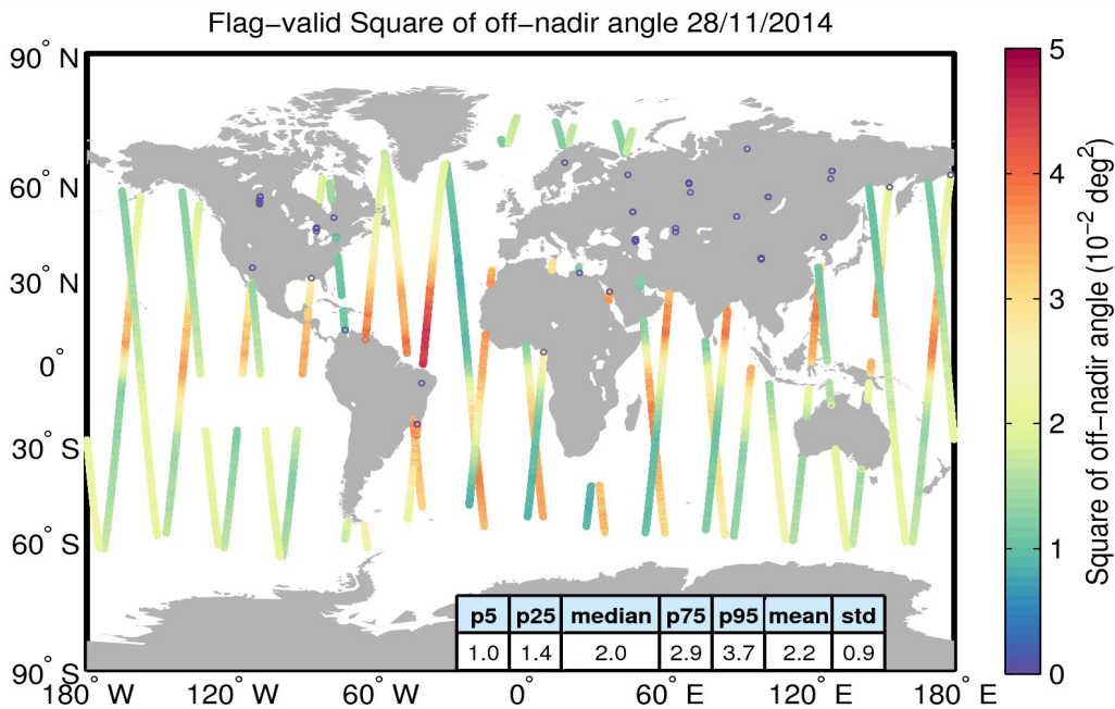
Figure 37. Geographical distribution of flag-valid mispointing data over oceans and lakes for 28/11/2014. The statistical values shown in the table refer to the mispointing in 10^{-2} \text{ deg}^2 and are calculated over all measurements shown in the figure.
