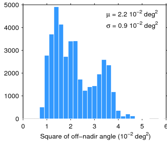
Figure 39. Histogram of flag-valid mispointing over oceans and lakes for 28/11/2014. The mean ( \mu ) and standard deviation ( \sigma ) are also shown. Note that values than 6 \cdot 10^{-2} \text{ deg}^2 are excluded from the histogram for the sake of readability but not from the computation of \mu and \sigma .
