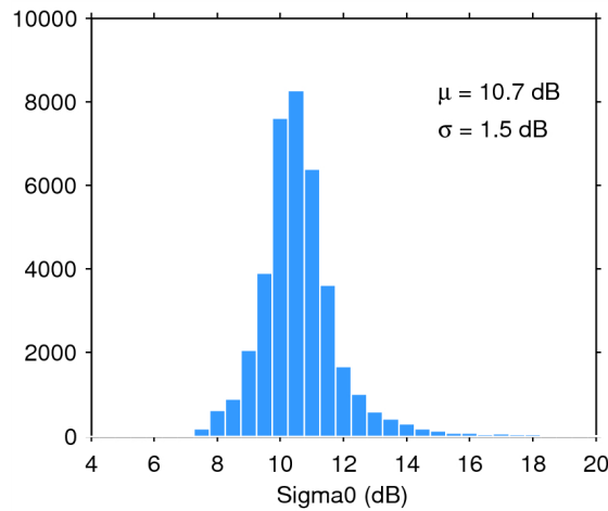
Figure 28. Histogram of science-valid sigma0 over oceans and lakes for 28/11/2014. The mean ( \mu ) and standard deviation ( \sigma ) are also shown. Note that values outside [4 20] dB are excluded from the histogram for the sake of readability but not from the computation of \mu and \sigma .
