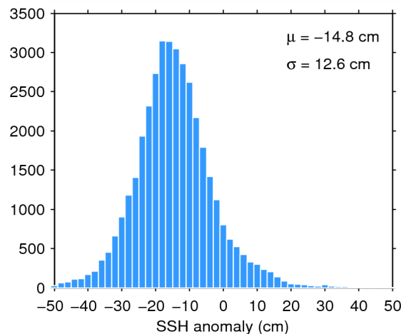
Figure 11. Histogram of science-valid SSH anomaly over oceans and lakes for 28/11/2014. The mean ( \mu ) and standard deviation ( \sigma ) are also shown. Note that values outside [-50 50] cm are excluded from the histogram for the sake of readability but not from the computation of \mu and \sigma .
