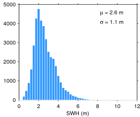
Figure 17. Histogram of flag-valid SWH over oceans and lakes for 28/11/2014. The mean ( \mu ) and standard deviation ( \sigma ) are also shown. Note that values larger than 12 m are excluded from the histogram for the sake of readability but not from the computation of \mu and \sigma .
