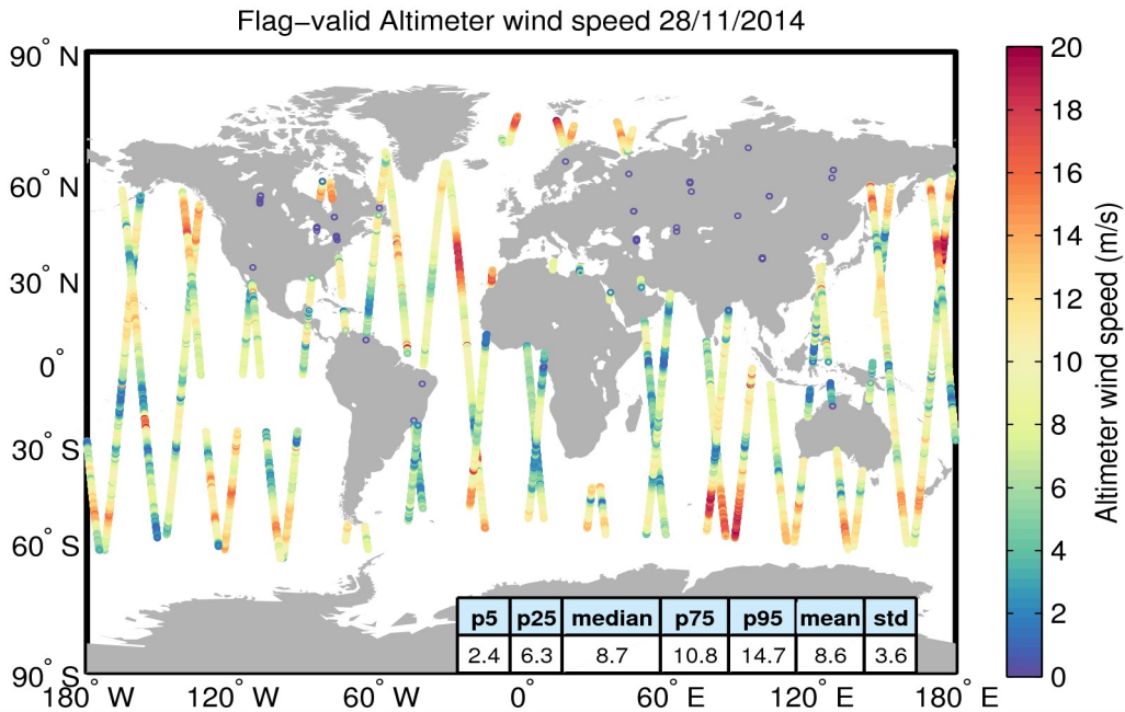
Figure 31. Geographical distribution of flag-valid wind data over oceans and lakes for 28/11/2014. The statistical values shown in the table refer to the wind in m/s and are calculated over all measurements shown in the figure.
