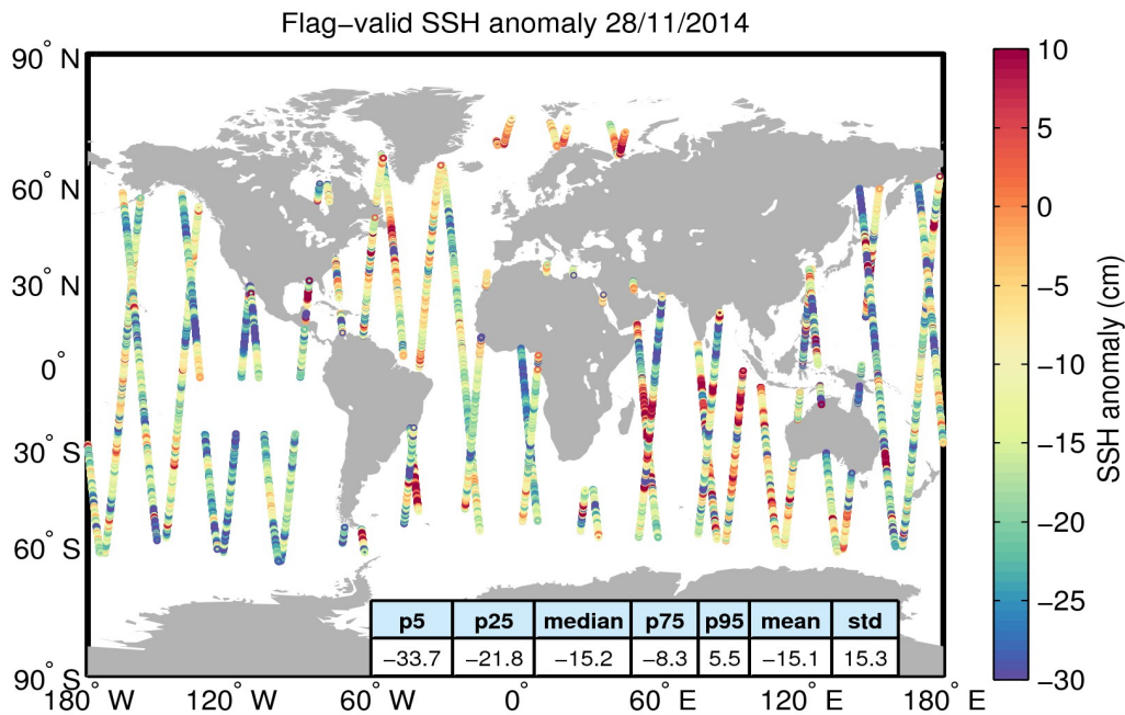
Figure 5. Geographical distribution of flag-valid 1-Hz SSH anomaly data over oceans and lakes for 28/11/2014. The statistical values shown in the table refer to the SSH anomaly in cm and are calculated over all measurements shown in the figure.
