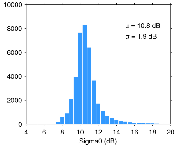
Figure 25. Histogram of flag-valid sigma0 over oceans and lakes for 28/11/2014. The mean ( \mu ) and standard deviation ( \sigma ) are also shown. Note that values outside [4 20] dB are excluded from the histogram for the sake of readability but not from the computation of \mu and \sigma .
