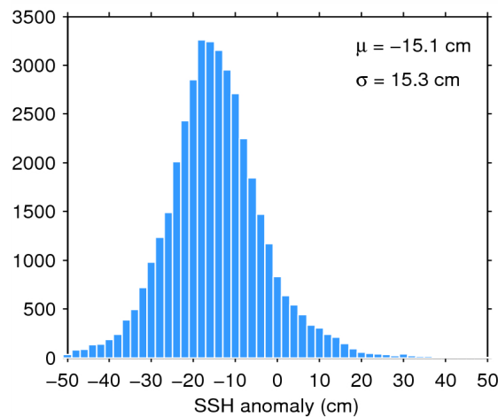
Figure 7. Histogram of flag-valid SSH anomaly over oceans and lakes for 28/11/2014. The mean ( \mu ) and standard deviation ( \sigma ) are also shown. Note that values outside [-50 50] cm are excluded from the histogram for the sake of readability but not from the computation of \mu and \sigma .
