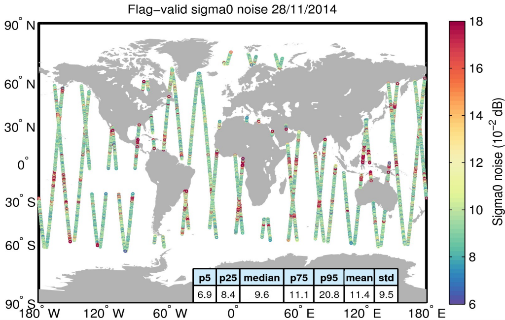
Figure 26. Geographical distribution of flag-valid 20-Hz sigma0 measurement noise over oceans and lakes for 28/11/2014. The statistical values shown in the table refer to the sigma0 noise and are calculated over all measurements shown in the figure.
