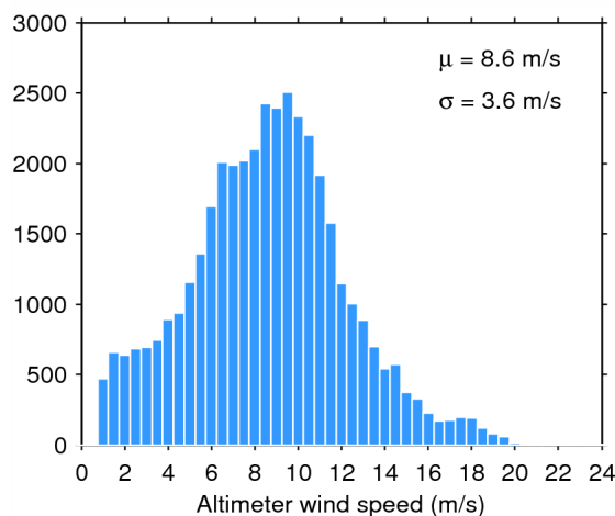
Figure 35. Histogram of science-valid wind over oceans and lakes for 28/11/2014. The mean ( \mu ) and standard deviation ( \sigma ) are also shown. Note that values larger than 24 m/s are excluded from the histogram for the sake of readability but not from the computation of \mu and \sigma .
