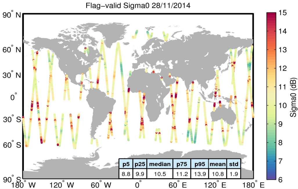
Figure 23. Geographical distribution of flag-valid sigma0 data over oceans and lakes for 28/11/2014. The statistical values shown in the table refer to the sigma0 in dB and are calculated over all measurements shown in the figure.
