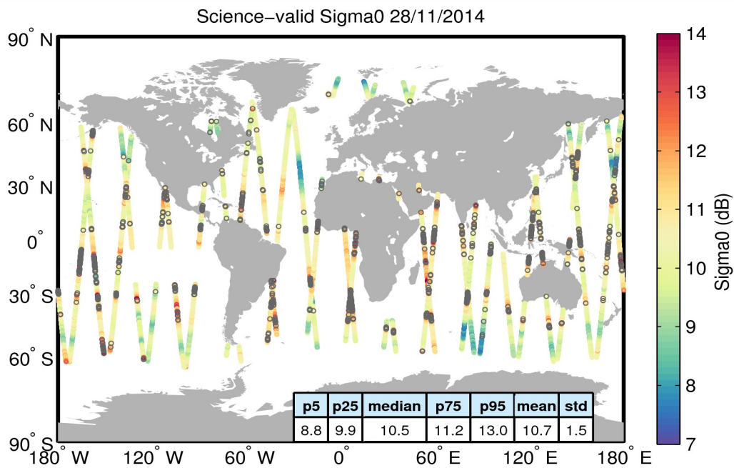
Figure 27. Geographical distribution of science-valid sigma0 data over oceans and lakes for 28/11/2014. The statistical values shown in the table refer to the sigma0 in dB and are calculated over all measurements shown in the figure. Gray circles denote records that have been rejected based on the editing criteria described in Table 4.
