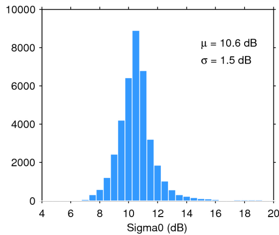
Figure 28. Histogram of science-valid sigma0 over oceans and lakes for 27/11/2014. The mean ( \mu ) and standard deviation ( \sigma ) are also shown. Note that values outside [4 20] dB are excluded from the histogram for the sake of readability but not from the computation of \mu and \sigma .
