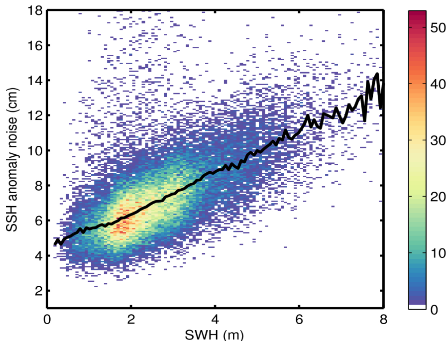
Figure 9. 2D histogram showing flag-valid SSH anomaly noise as a function of SWH for 27/11/2014. The black line denotes the median SSH anomaly as a function of SWH.
