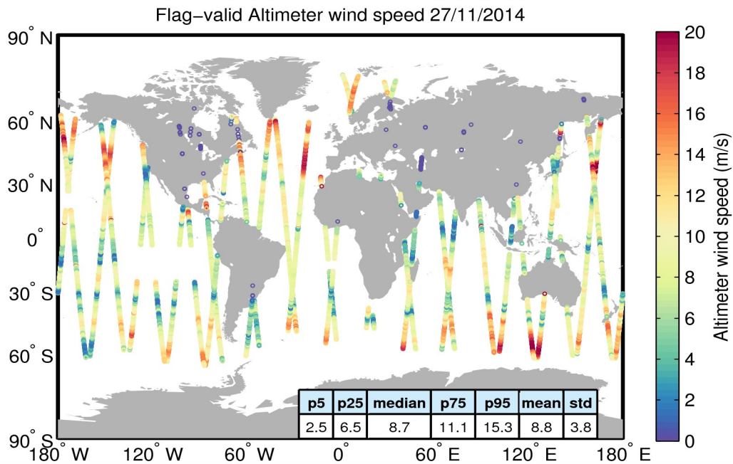
Figure 31. Geographical distribution of flag-valid wind data over oceans and lakes for 27/11/2014. The statistical values shown in the figure refer to the wind in m/s and are calculated over all measurements shown in the figure.
