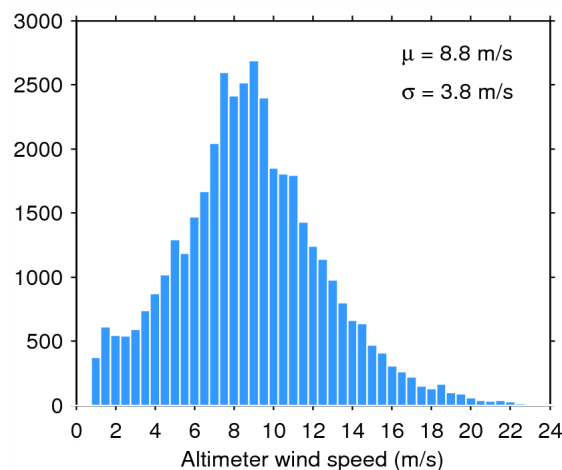
Figure 35. Histogram of science-valid wind over oceans and lakes for 27/11/2014. The mean ( \mu ) and standard deviation ( \sigma ) are also shown. Note that values larger than 24 m/s are excluded from the histogram for the sake of readability but not from the computation of \mu and \sigma .
