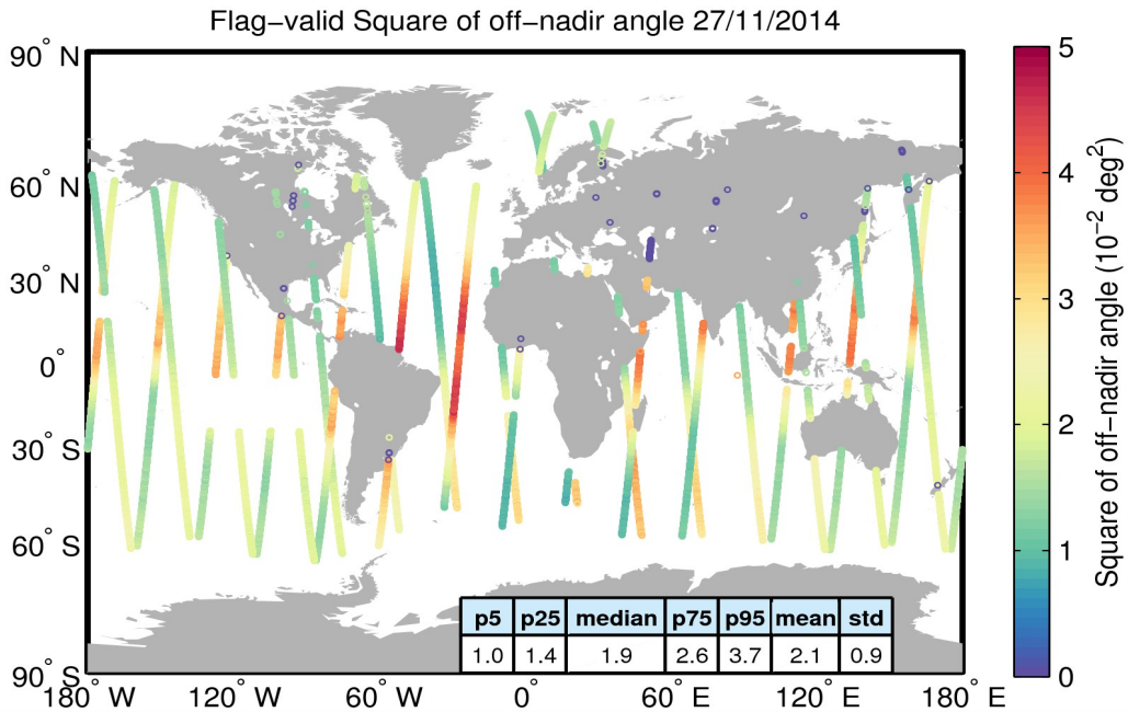
Figure 37. Geographical distribution of flag-valid mispointing data over oceans and lakes for 27/11/2014. The statistical values shown in the table refer to the mispointing in 10^{-2} \text{ deg}^2 and are calculated over all measurements shown in the figure.
