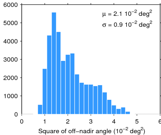
Figure 39. Histogram of flag-valid mispointing over oceans and lakes for 27/11/2014. The mean ( \mu ) and standard deviation ( \sigma ) are also shown. Note that values than 6 \cdot 10^{-2} \text{ deg}^2 are excluded from the histogram for the sake of readability but not from the computation of \mu and \sigma .
