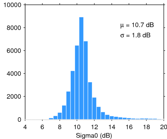
Figure 25. Histogram of flag-valid sigma0 over oceans and lakes for 27/11/2014. The mean ( \mu ) and standard deviation ( \sigma ) are also shown. Note that values outside [4 20] dB are excluded from the histogram for the sake of readability but not from the computation of \mu and \sigma .
