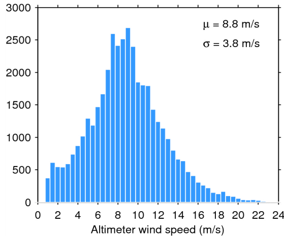
Figure 33. Histogram of flag-valid wind over oceans and lakes for 27/11/2014. The mean ( \mu ) and standard deviation ( \sigma ) are also shown. Note that values larger than 24 m/s are excluded from the histogram for the sake of readability but not from the computation of \mu and \sigma .
