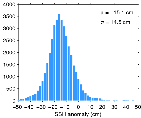
Figure 7. Histogram of flag-valid SSH anomaly over oceans and lakes for 27/11/2014. The mean ( \mu ) and standard deviation ( \sigma ) are also shown. Note that values outside [-50 \ 50] cm are excluded from the histogram for the sake of readability but not from the computation of \mu and \sigma .
