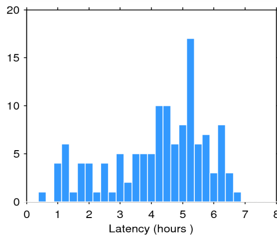
Figure 2. Histogram of the data latency for 27/11/2014. The y-axis denotes the number of files that are made available with a delay of x-hours with respect to the mean time of the records stored in the file.
