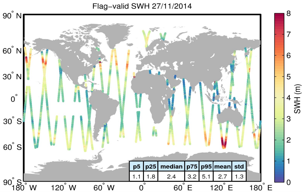
Figure 15. Geographical distribution of flag-valid SWH data over oceans and lakes for 27/11/2014. The statistical values shown in the table refer to the SWH in m and are calculated over all measurements shown in the figure.
