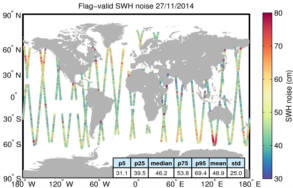
Figure 18. Geographical distribution of flag-valid 20-Hz SWH measurement noise over oceans and lakes for 27/11/2014. The statistical values shown in the figure refer to the SWH noise and are calculated over all measurements shown in the figure.
