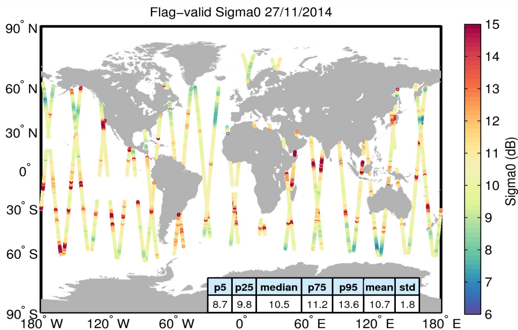
Figure 23. Geographical distribution of flag-valid sigma0 data over oceans and lakes for 27/11/2014. The statistical values shown in the table refer to the sigma0 in dB and are calculated over all measurements shown in the figure.
