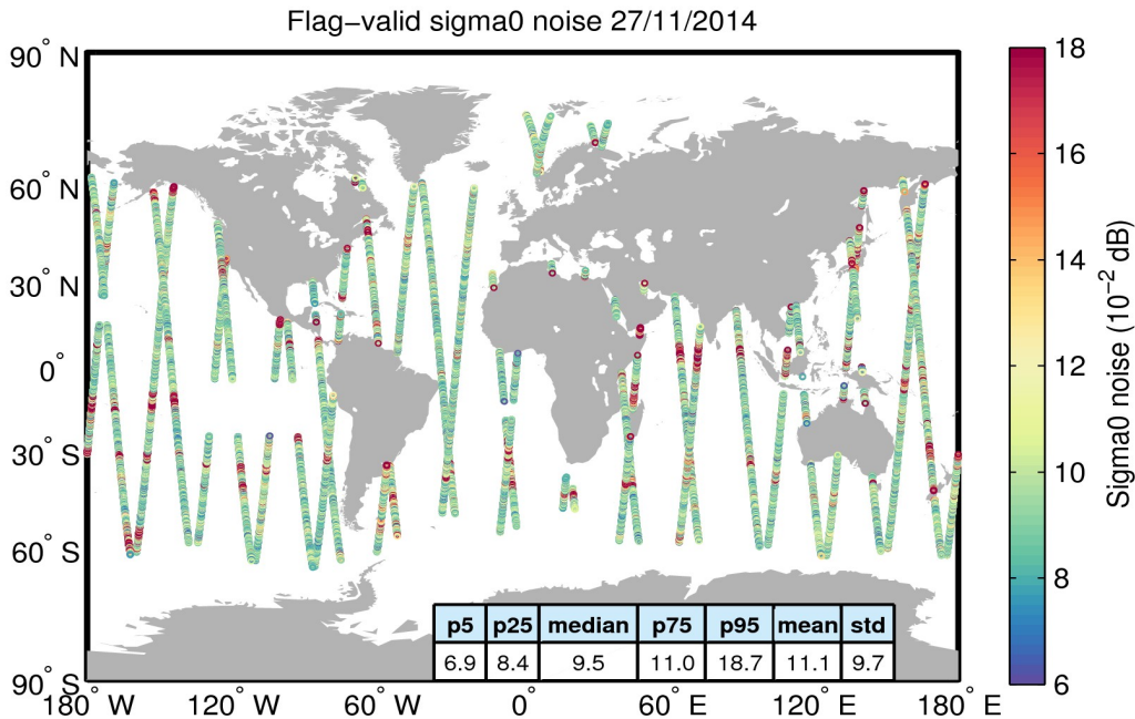
Figure 26. Geographical distribution of flag-valid 20-Hz sigma0 measurement noise over oceans and lakes for 27/11/2014. The statistical values shown in the table refer to the sigma0 noise and are calculated over all measurements shown in the figure.
