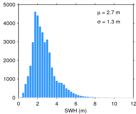
Figure 17. Histogram of flag-valid SWH over oceans and lakes for 27/11/2014. The mean ( \mu ) and standard deviation ( \sigma ) are also shown. Note that values larger than 12 m are excluded from the histogram for the sake of readability but not from the computation of \mu and \sigma .
