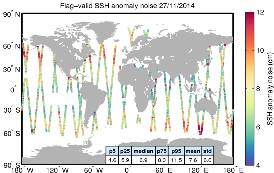
Figure 8. Geographical distribution of flag-valid 20-Hz SSH anomaly measurement noise over oceans and lakes for 27/11/2014. The statistical values shown in the table refer to the SSH anomaly noise and are calculated over all measurements shown in the figure.
