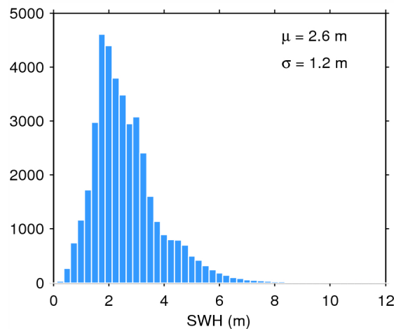
Figure 20. Histogram of science-valid SWH over oceans and lakes for 27/11/2014. The mean ( \mu ) and standard deviation ( \sigma ) are also shown. Note that values larger than 12 m are excluded from the histogram for the sake of readability but not from the computation of \mu and \sigma .
