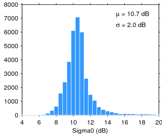
Figure 25. Histogram of flag-valid sigma0 over oceans and lakes for 24/11/2014. The mean ( \mu ) and standard deviation ( \sigma ) are also shown. Note that values outside [4 20] dB are excluded from the histogram for the sake of readability but not from the computation of \mu and \sigma .
