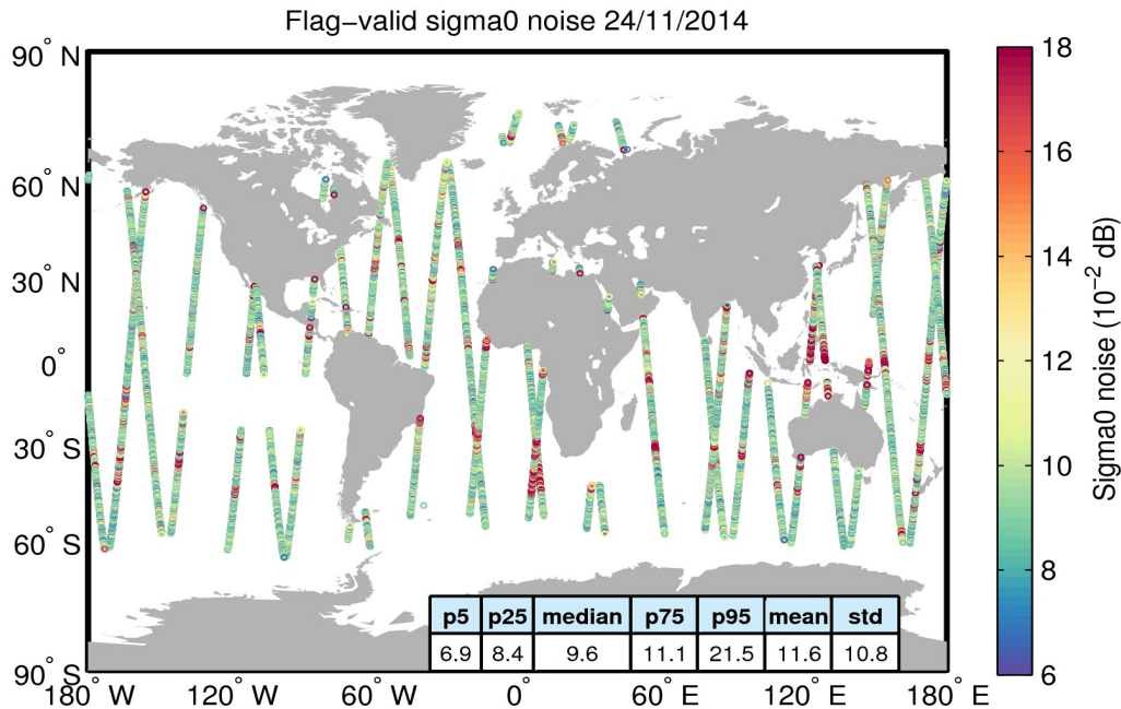
Figure 26. Geographical distribution of flag-valid 20-Hz sigma0 measurement noise over oceans and lakes for 24/11/2014. The statistical values shown in the table refer to the sigma0 noise and are calculated over all measurements shown in the figure.
