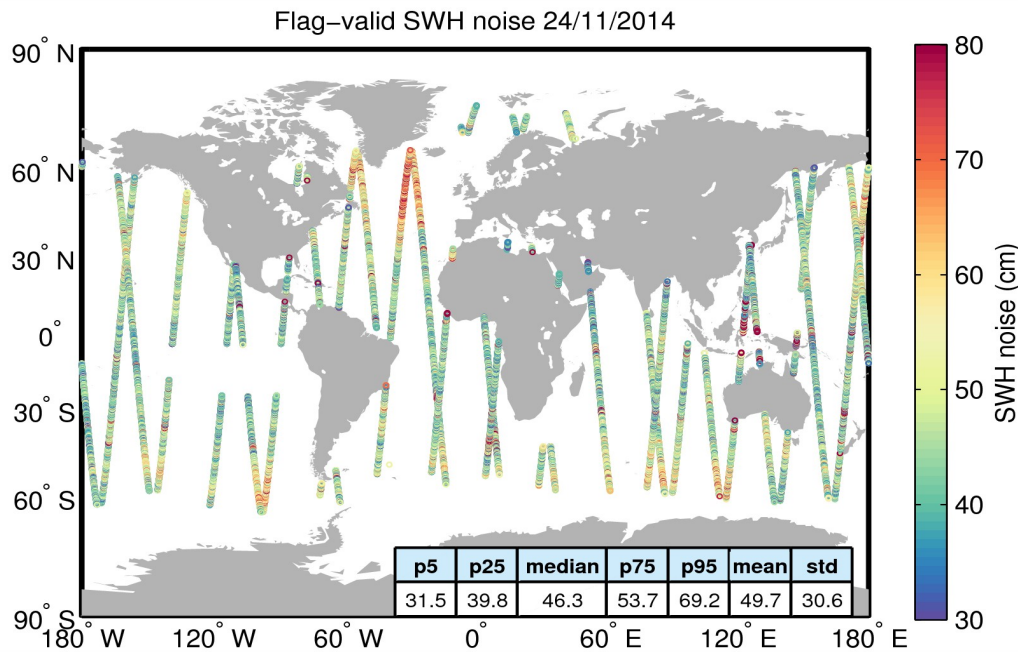
Figure 18. Geographical distribution of flag-valid 20-Hz SWH measurement noise over oceans and lakes for 24/11/2014. The statistical values shown in the figure refer to the SWH noise and are calculated over all measurements shown in the figure.
