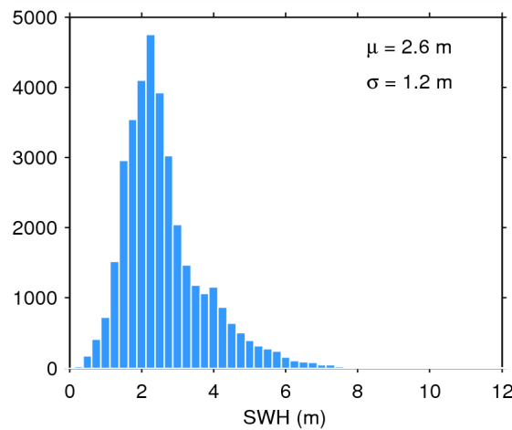
Figure 17. Histogram of flag-valid SWH over oceans and lakes for 24/11/2014. The mean ( \mu ) and standard deviation ( \sigma ) are also shown. Note that values larger than 12 m are excluded from the histogram for the sake of readability but not from the computation of \mu and \sigma .
