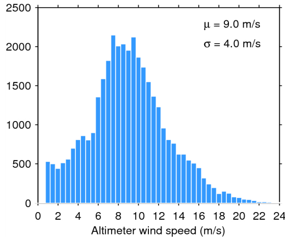
Figure 33. Histogram of flag-valid wind over oceans and lakes for 24/11/2014. The mean ( \mu ) and standard deviation ( \sigma ) are also shown. Note that values larger than 24 m/s are excluded from the histogram for the sake of readability but not from the computation of \mu and \sigma .
