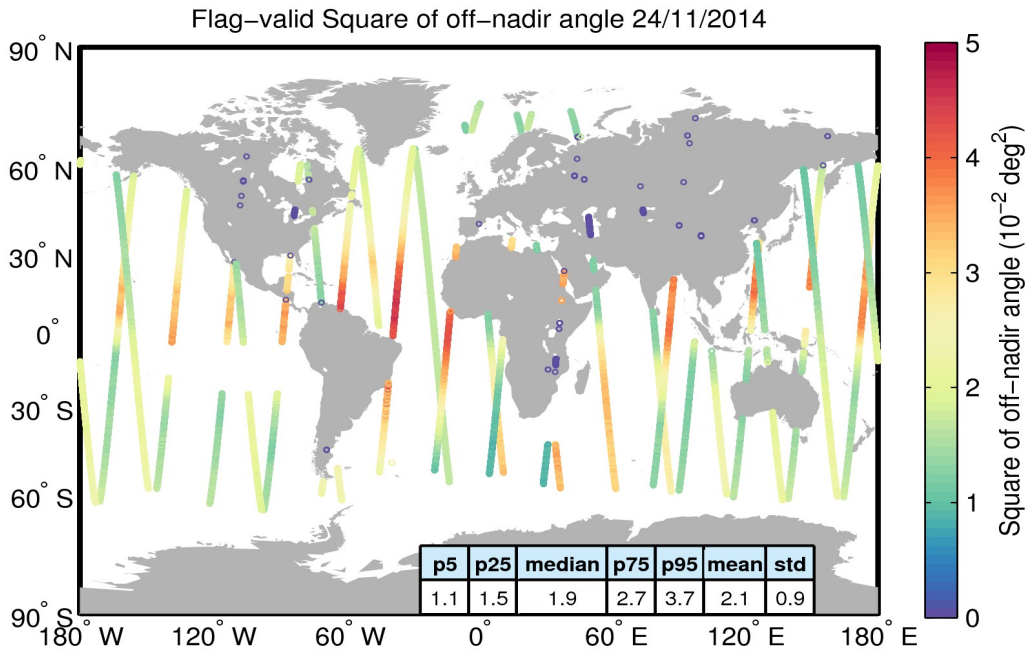
Figure 37. Geographical distribution of flag-valid mispointing data over oceans and lakes for 24/11/2014. The statistical values shown in the table refer to the mispointing in 10^{-2} \text{ deg}^2 and are calculated over all measurements shown in the figure.
