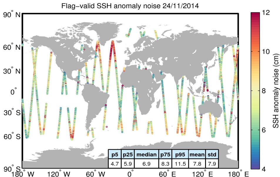
Figure 8. Geographical distribution of flag-valid 20-Hz SSH anomaly measurement noise over oceans and lakes for 24/11/2014. The statistical values shown in the table refer to the SSH anomaly noise and are calculated over all measurements shown in the figure.
