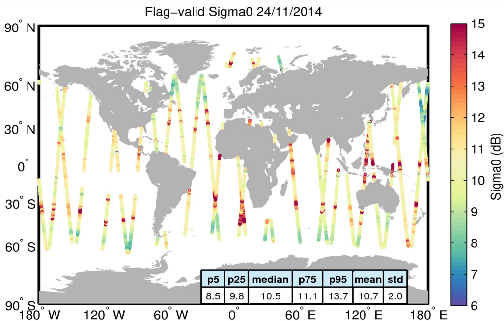
Figure 23. Geographical distribution of flag-valid sigma0 data over oceans and lakes for 24/11/2014. The statistical values shown in the table refer to the sigma0 in dB and are calculated over all measurements shown in the figure.
