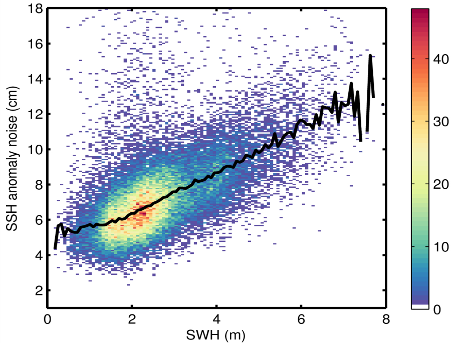
Figure 9. 2D histogram showing flag-valid SSH anomaly noise as a function of SWH for 24/11/2014. The black line denotes the median SSH anomaly as a function of SWH.
