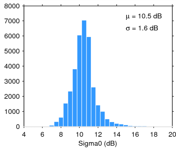
Figure 28. Histogram of science-valid sigma0 over oceans and lakes for 24/11/2014. The mean ( \mu ) and standard deviation ( \sigma ) are also shown. Note that values outside [4 20] dB are excluded from the histogram for the sake of readability but not from the computation of \mu and \sigma .
