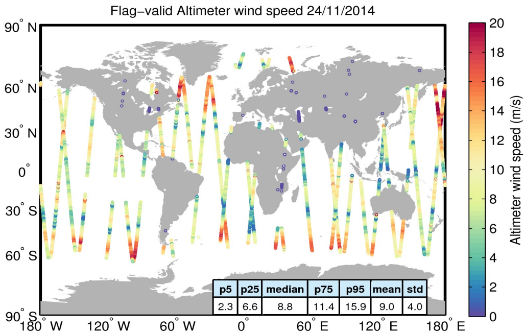
Figure 31. Geographical distribution of flag-valid wind data over oceans and lakes for 24/11/2014. The statistical values shown in the table refer to the wind in m/s and are calculated over all measurements shown in the figure.
