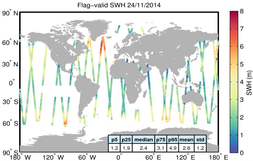
Figure 15. Geographical distribution of flag-valid SWH data over oceans and lakes for 24/11/2014. The statistical values shown in the table refer to the SWH in m and are calculated over all measurements shown in the figure.
