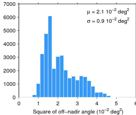
Figure 39. Histogram of flag-valid mispointing over oceans and lakes for 24/11/2014. The mean ( \mu ) and standard deviation ( \sigma ) are also shown. Note that values than 6 \cdot 10^{-2} \text{ deg}^2 are excluded from the histogram for the sake of readability but not from the computation of \mu and \sigma .
