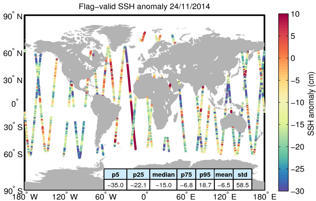
Figure 5. Geographical distribution of flag-valid 1-Hz SSH anomaly data over oceans and lakes for 24/11/2014. The statistical values shown in the table refer to the SSH anomaly in cm and are calculated over all measurements shown in the figure.
