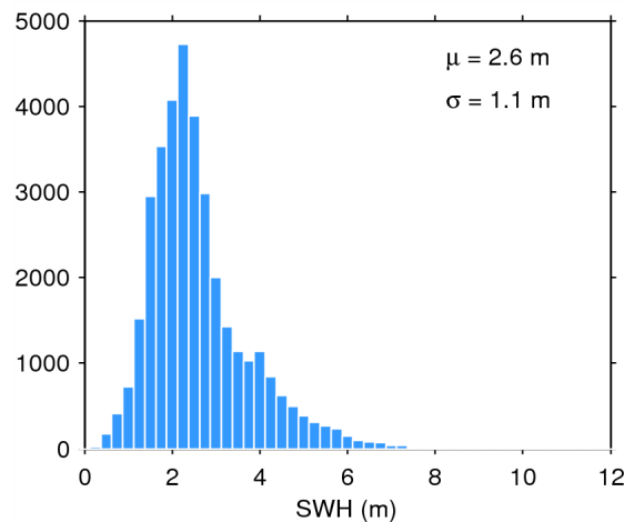
Figure 20. Histogram of science-valid SWH over oceans and lakes for 24/11/2014. The mean ( \mu ) and standard deviation ( \sigma ) are also shown. Note that values larger than 12 m are excluded from the histogram for the sake of readability but not from the computation of \mu and \sigma .
