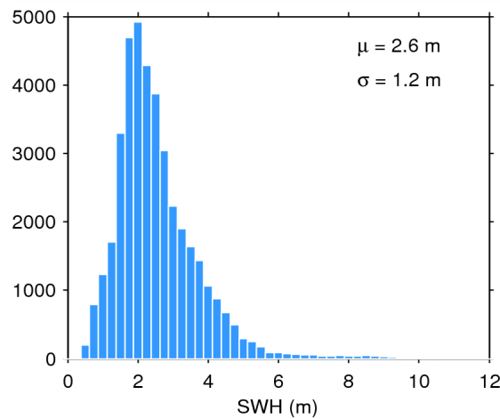
Figure 17. Histogram of flag-valid SWH over oceans and lakes for 23/11/2014. The mean ( \mu ) and standard deviation ( \sigma ) are also shown. Note that values larger than 12 m are excluded from the histogram for the sake of readability but not from the computation of \mu and \sigma .
