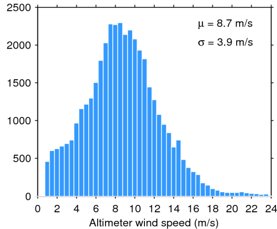
Figure 33. Histogram of flag-valid wind over oceans and lakes for 23/11/2014. The mean ( \mu ) and standard deviation ( \sigma ) are also shown. Note that values larger than 24 m/s are excluded from the histogram for the sake of readability but not from the computation of \mu and \sigma .
