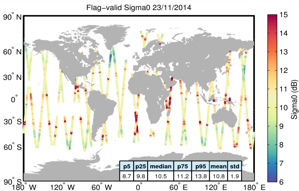
Figure 23. Geographical distribution of flag-valid sigma0 data over oceans and lakes for 23/11/2014. The statistical values shown in the table refer to the sigma0 in dB and are calculated over all measurements shown in the figure.
