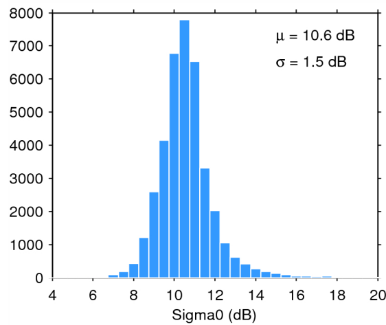
Figure 28. Histogram of science-valid sigma0 over oceans and lakes for 23/11/2014. The mean ( \mu ) and standard deviation ( \sigma ) are also shown. Note that values outside [4 20] dB are excluded from the histogram for the sake of readability but not from the computation of \mu and \sigma .
