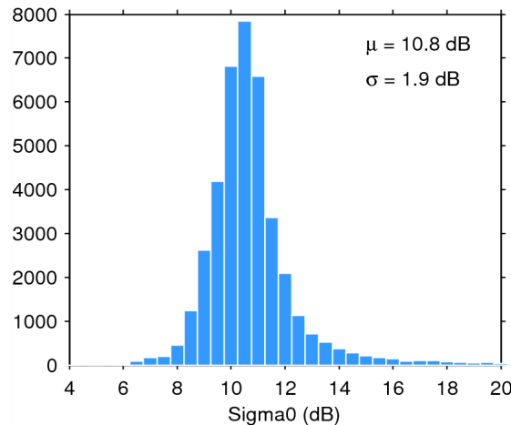
Figure 25. Histogram of flag-valid sigma0 over oceans and lakes for 23/11/2014. The mean ( \mu ) and standard deviation ( \sigma ) are also shown. Note that values outside [4 20] dB are excluded from the histogram for the sake of readability but not from the computation of \mu and \sigma .
