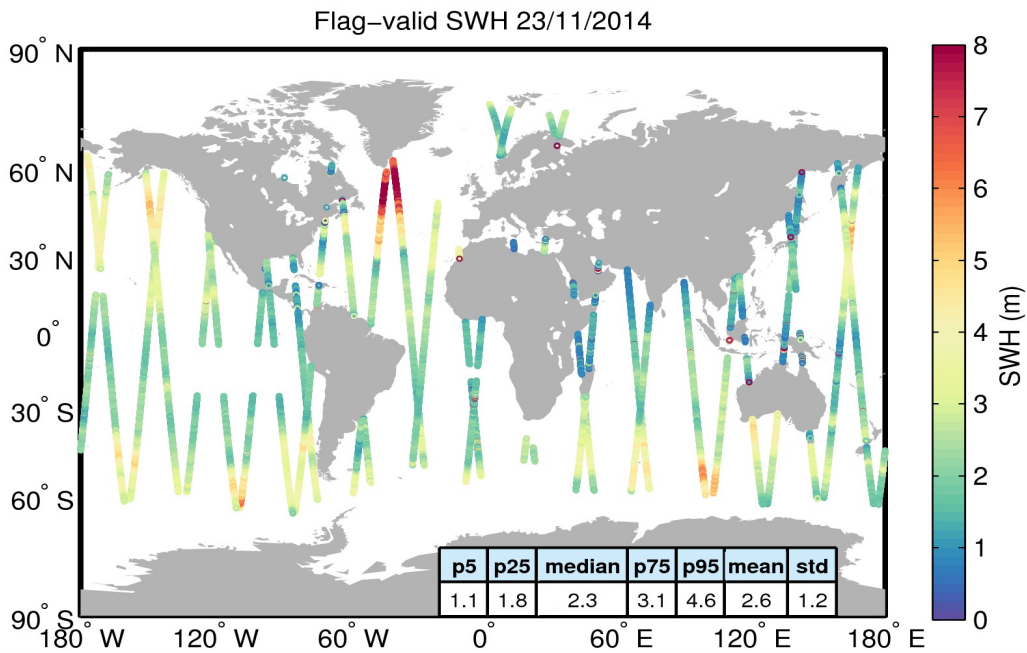
Figure 15. Geographical distribution of flag-valid SWH data over oceans and lakes for 23/11/2014. The statistical values shown in the table refer to the SWH in m and are calculated over all measurements shown in the figure.
