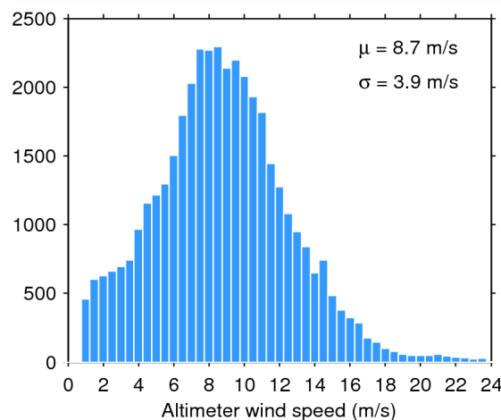
Figure 35. Histogram of science-valid wind over oceans and lakes for 23/11/2014. The mean ( \mu ) and standard deviation ( \sigma ) are also shown. Note that values larger than 24 m/s are excluded from the histogram for the sake of readability but not from the computation of \mu and \sigma .
