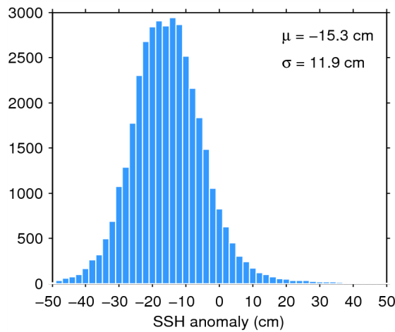
Figure 11. Histogram of science-valid SSH anomaly over oceans and lakes for 23/11/2014. The mean ( \mu ) and standard deviation ( \sigma ) are also shown. Note that values outside [-50 50] cm are excluded from the histogram for the sake of readability but not from the computation of \mu and \sigma .
