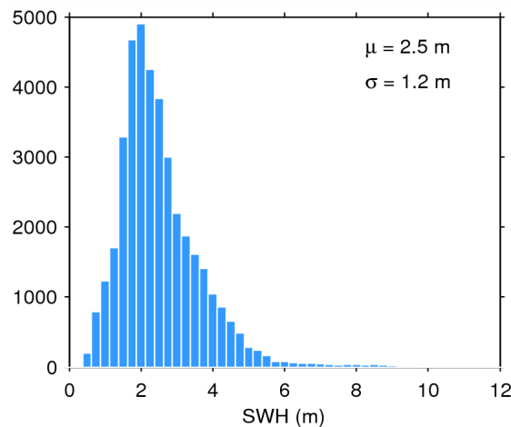
Figure 20. Histogram of science-valid SWH over oceans and lakes for 23/11/2014. The mean ( \mu ) and standard deviation ( \sigma ) are also shown. Note that values larger than 12 m are excluded from the histogram for the sake of readability but not from the computation of \mu and \sigma .
