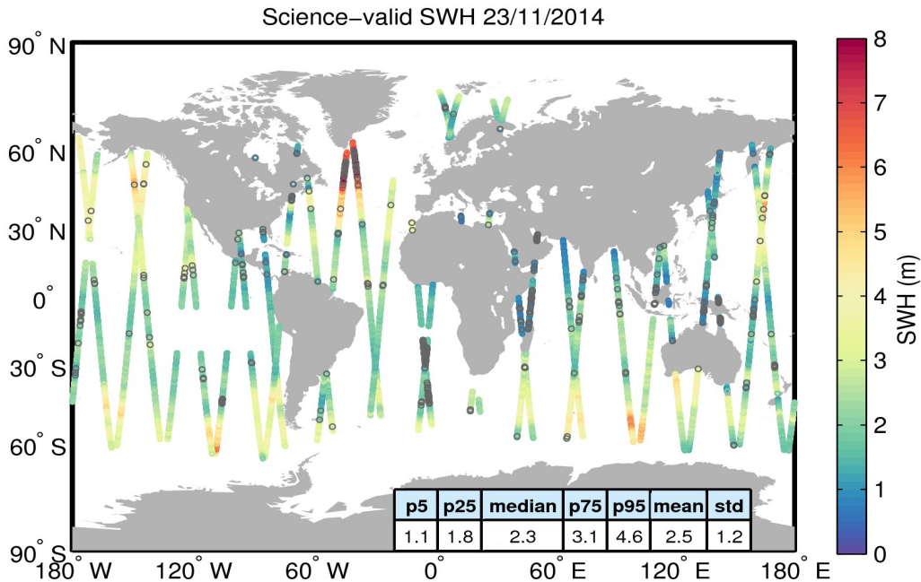
Figure 19. Geographical distribution of science-valid SWH data over oceans and lakes for 23/11/2014. The statistical values shown in the table refer to the SWH in m and are calculated over all measurements shown in the figure. Gray circles denote records that have been rejected based on the editing criteria described in Table 3.
