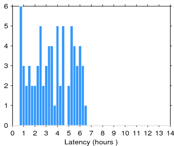
Figure 2. Histogram of the data latency for 23/11/2014. The y-axis denotes the number of files that are made available with a delay of x-hours with respect to the mean time of the records stored in the file.
