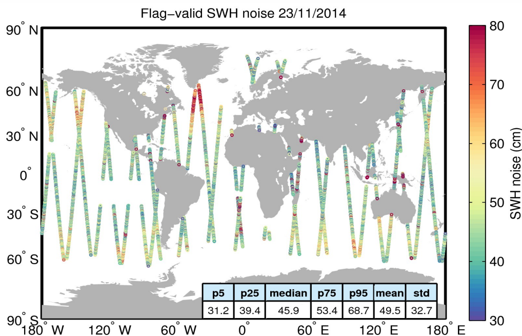
Figure 18. Geographical distribution of flag-valid 20-Hz SWH measurement noise over oceans and lakes for 23/11/2014. The statistical values shown in the figure refer to the SWH noise and are calculated over all measurements shown in the figure.
