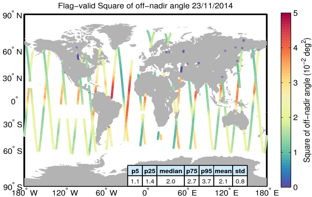
Figure 37. Geographical distribution of flag-valid mispointing data over oceans and lakes for 23/11/2014. The statistical values shown in the table refer to the mispointing in 10^{-2} \text{deg}^2 and are calculated over all measurements shown in the figure.
