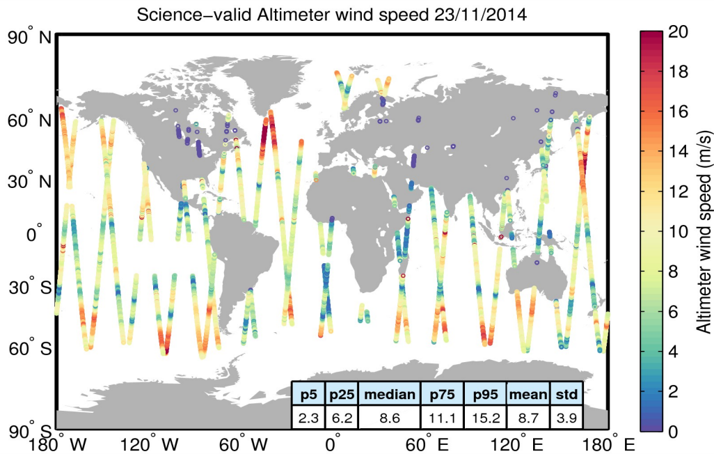
Figure 34. Geographical distribution of science-valid wind data over oceans and lakes for 23/11/2014. The statistical values shown in the table refer to the wind in m/s and are calculated over all measurements shown in the figure. Gray circles denote records that have been rejected based on the editing criteria described in Table 5.
