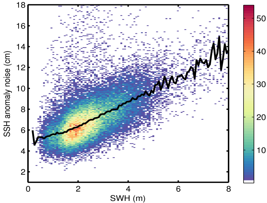
Figure 9. 2D histogram showing flag-valid SSH anomaly noise as a function of SWH for 23/11/2014. The black line denotes the median SSH anomaly as a function of SWH.
