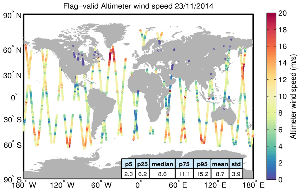
Figure 31. Geographical distribution of flag-valid wind data over oceans and lakes for 23/11/2014. The statistical values shown in the figure refer to the wind in m/s and are calculated over all measurements shown in the figure.
