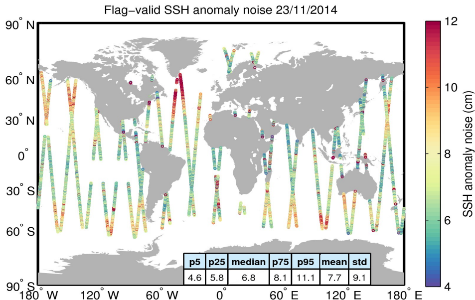
Figure 8. Geographical distribution of flag-valid 20-Hz SSH anomaly measurement noise over oceans and lakes for 23/11/2014. The statistical values shown in the table refer to the SSH anomaly noise and are calculated over all measurements shown in the figure.
