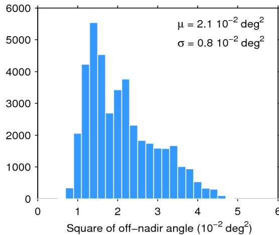
Figure 39. Histogram of flag-valid mispointing over oceans and lakes for 23/11/2014. The mean ( \mu ) and standard deviation ( \sigma ) are also shown. Note that values than 6 \cdot 10^{-2} \text{ deg}^2 are excluded from the histogram for the sake of readability but not from the computation of \mu and \sigma .
