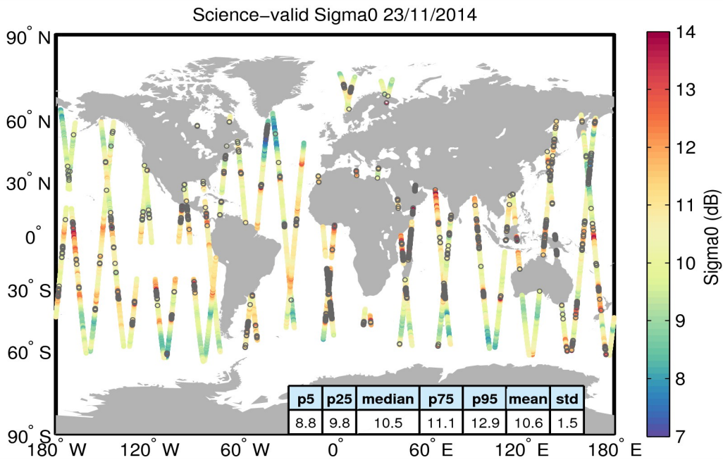
Figure 27. Geographical distribution of science-valid sigma0 data over oceans and lakes for 23/11/2014. The statistical values shown in the table refer to the sigma0 in dB and are calculated over all measurements shown in the figure. Gray circles denote records that have been rejected based on the editing criteria described in Table 4.
