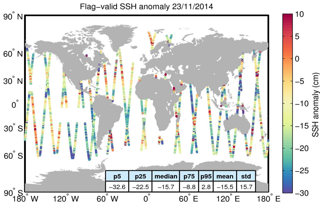
Figure 5. Geographical distribution of flag-valid 1-Hz SSH anomaly data over oceans and lakes for 23/11/2014. The statistical values shown in the table refer to the SSH anomaly in cm and are calculated over all measurements shown in the figure.
