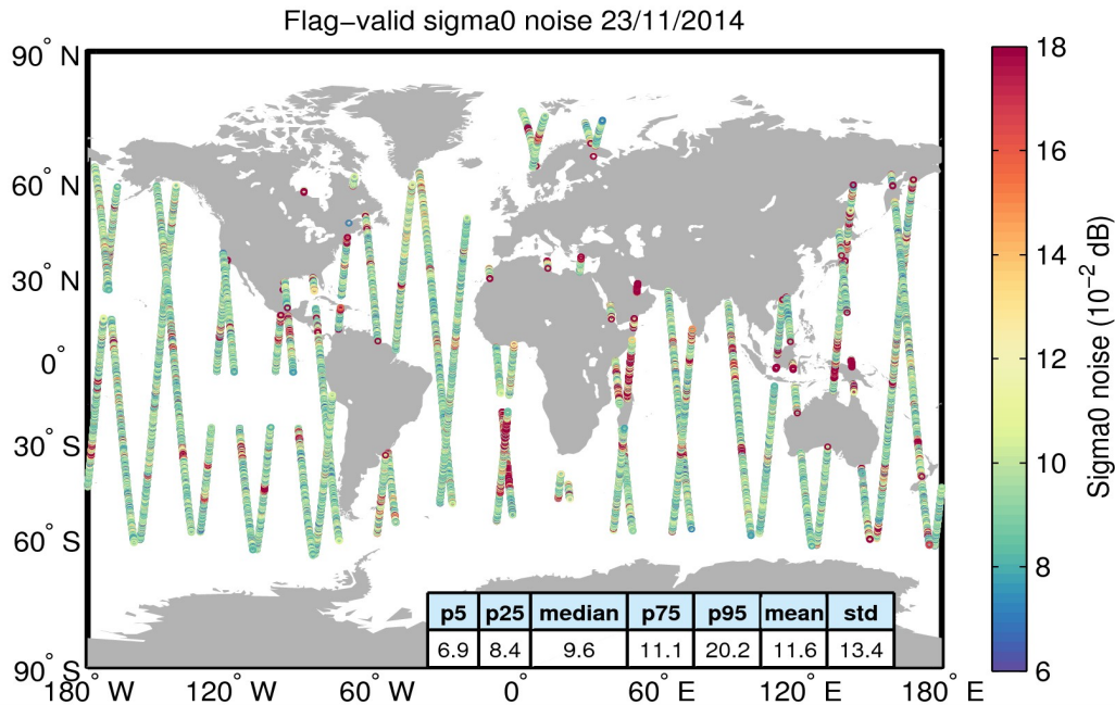
Figure 26. Geographical distribution of flag-valid 20-Hz sigma0 measurement noise over oceans and lakes for 23/11/2014. The statistical values shown in the table refer to the sigma0 noise and are calculated over all measurements shown in the figure.
