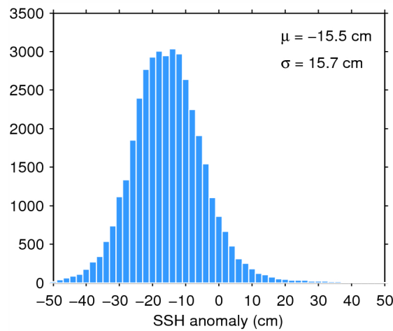
Figure 7. Histogram of flag-valid SSH anomaly over oceans and lakes for 23/11/2014. The mean ( \mu ) and standard deviation ( \sigma ) are also shown. Note that values outside [-50 50] cm are excluded from the histogram for the sake of readability but not from the computation of \mu and \sigma .
