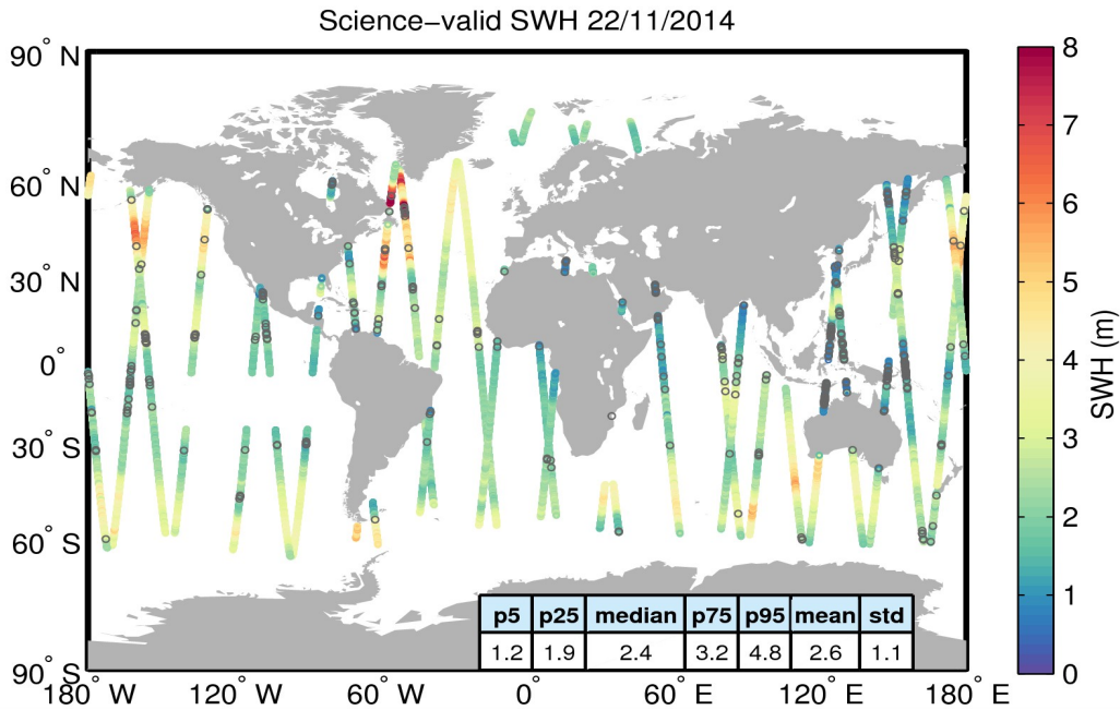
Figure 19. Geographical distribution of science-valid SWH data over oceans and lakes for 22/11/2014. The statistical values shown in the table refer to the SWH in m and are calculated over all measurements shown in the figure. Gray circles denote records that have been rejected based on the editing criteria described in Table 3.
