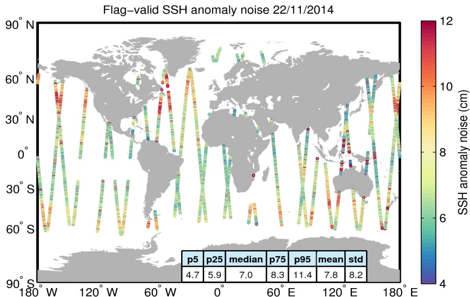
Figure 8. Geographical distribution of flag-valid 20-Hz SSH anomaly measurement noise over oceans and lakes for 22/11/2014. The statistical values shown in the table refer to the SSH anomaly noise and are calculated over all measurements shown in the figure.
