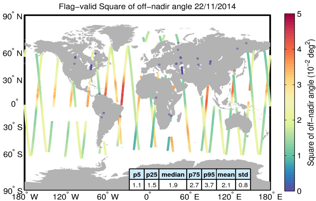
Figure 37. Geographical distribution of flag-valid mispointing data over oceans and lakes for 22/11/2014. The statistical values shown in the table refer to the mispointing in 10^{-2} \text{ deg}^2 and are calculated over all measurements shown in the figure.
