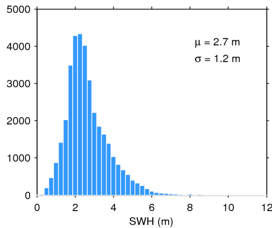
Figure 17. Histogram of flag-valid SWH over oceans and lakes for 22/11/2014. The mean ( \mu ) and standard deviation ( \sigma ) are also shown. Note that values larger than 12 m are excluded from the histogram for the sake of readability but not from the computation of \mu and \sigma .
