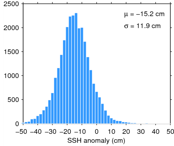
Figure 11. Histogram of science-valid SSH anomaly over oceans and lakes for 22/11/2014. The mean ( \mu ) and standard deviation ( \sigma ) are also shown. Note that values outside [-50 50] cm are excluded from the histogram for the sake of readability but not from the computation of \mu and \sigma .
