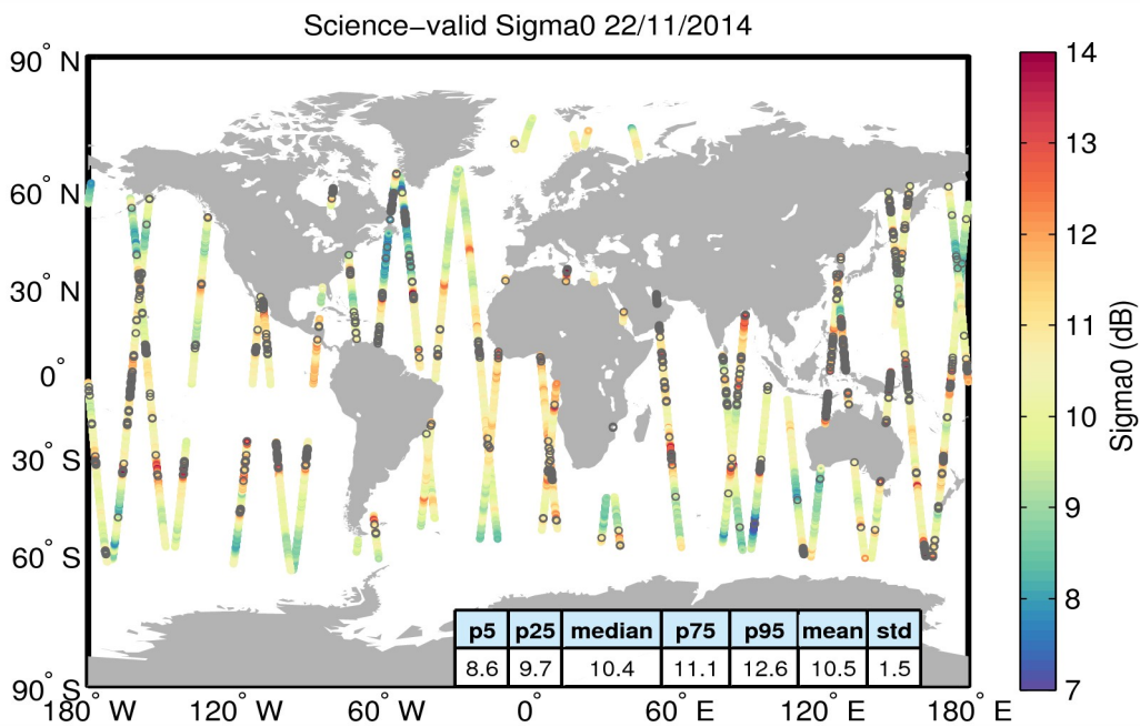
Figure 27. Geographical distribution of science-valid sigma0 data over oceans and lakes for 22/11/2014. The statistical values shown in the table refer to the sigma0 in dB and are calculated over all measurements shown in the figure. Gray circles denote records that have been rejected based on the editing criteria described in Table 4.
