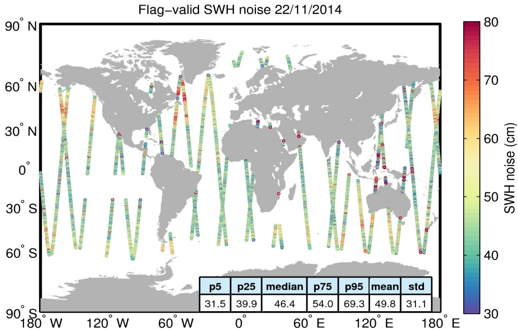
Figure 18. Geographical distribution of flag-valid 20-Hz SWH measurement noise over oceans and lakes for 22/11/2014. The statistical values shown in the figure refer to the SWH noise and are calculated over all measurements shown in the figure.
