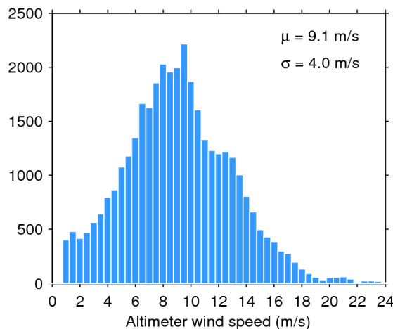
Figure 35. Histogram of science-valid wind over oceans and lakes for 22/11/2014. The mean ( \mu ) and standard deviation ( \sigma ) are also shown. Note that values larger than 24 m/s are excluded from the histogram for the sake of readability but not from the computation of \mu and \sigma .
