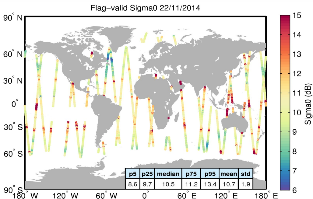
Figure 23. Geographical distribution of flag-valid sigma0 data over oceans and lakes for 22/11/2014. The statistical values shown in the table refer to the sigma0 in dB and are calculated over all measurements shown in the figure.
