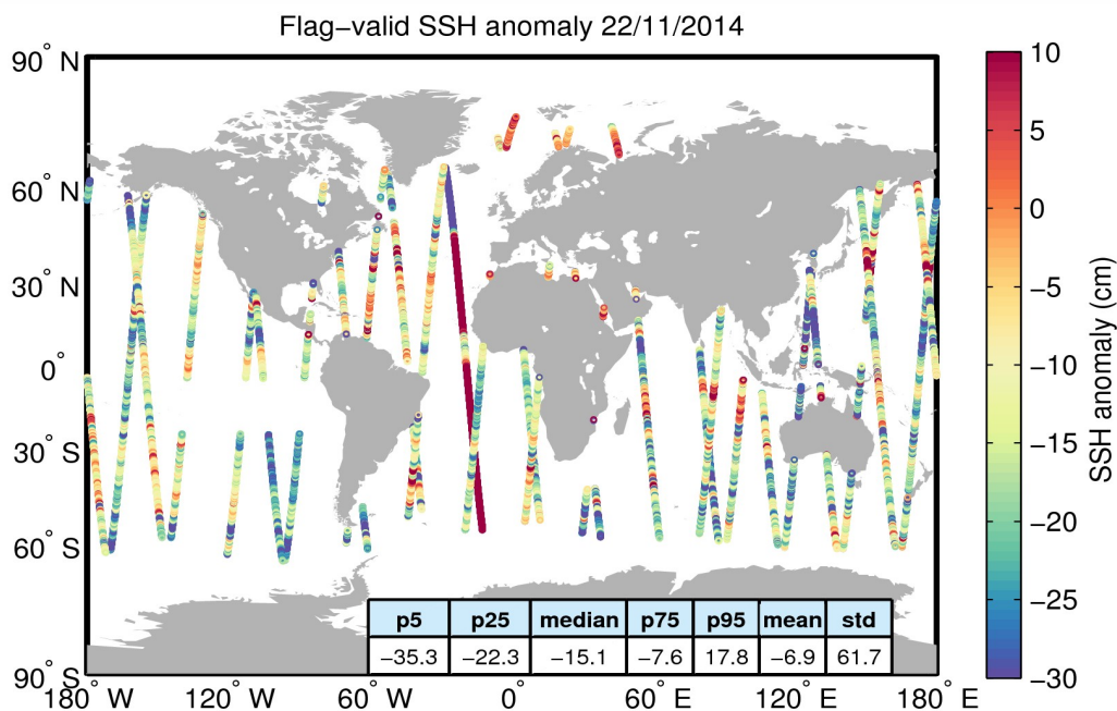
Figure 5. Geographical distribution of flag-valid 1-Hz SSH anomaly data over oceans and lakes for 22/11/2014. The statistical values shown in the table refer to the SSH anomaly in cm and are calculated over all measurements shown in the figure.
