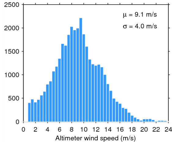
Figure 33. Histogram of flag-valid wind over oceans and lakes for 22/11/2014. The mean ( \mu ) and standard deviation ( \sigma ) are also shown. Note that values larger than 24 m/s are excluded from the histogram for the sake of readability but not from the computation of \mu and \sigma .
