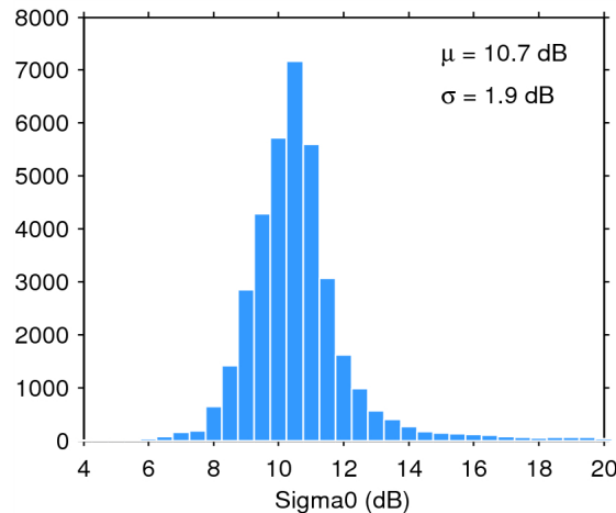
Figure 25. Histogram of flag-valid sigma0 over oceans and lakes for 22/11/2014. The mean ( \mu ) and standard deviation ( \sigma ) are also shown. Note that values outside [4 20] dB are excluded from the histogram for the sake of readability but not from the computation of \mu and \sigma .
