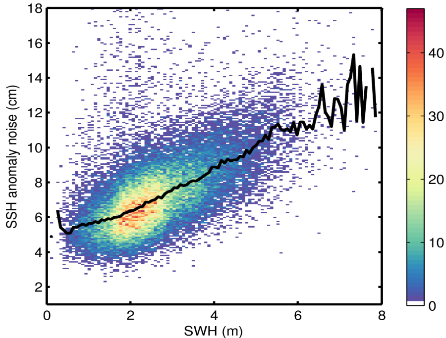
Figure 9. 2D histogram showing flag-valid SSH anomaly noise as a function of SWH for 22/11/2014. The black line denotes the median SSH anomaly as a function of SWH.
