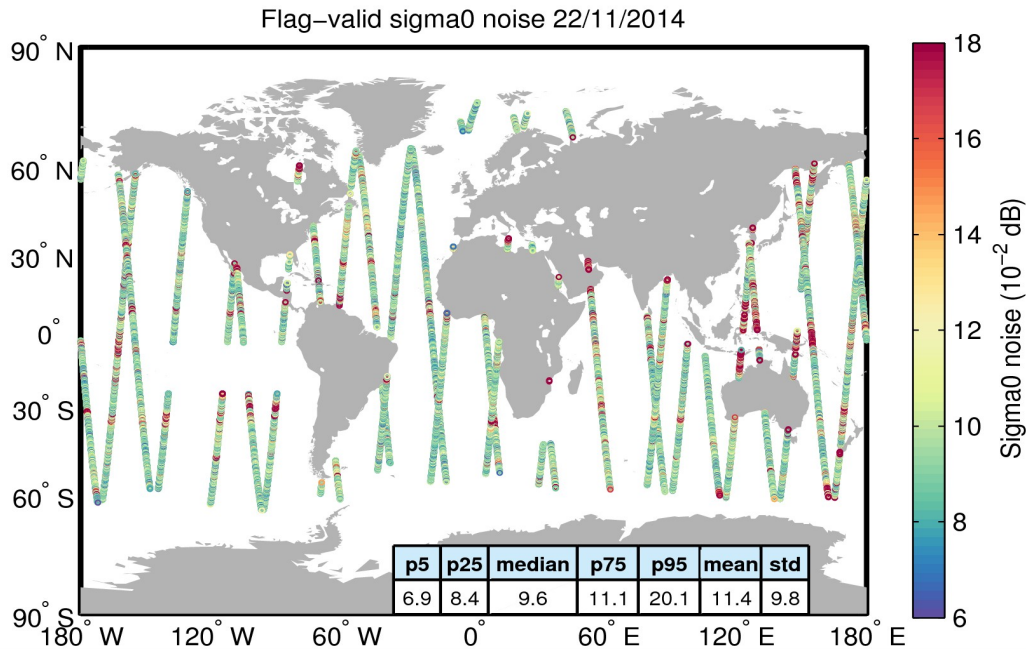
Figure 26. Geographical distribution of flag-valid 20-Hz sigma0 measurement noise over oceans and lakes for 22/11/2014. The statistical values shown in the table refer to the sigma0 noise and are calculated over all measurements shown in the figure.
