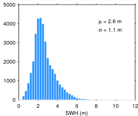
Figure 20. Histogram of science-valid SWH over oceans and lakes for 22/11/2014. The mean ( \mu ) and standard deviation ( \sigma ) are also shown. Note that values larger than 12 m are excluded from the histogram for the sake of readability but not from the computation of \mu and \sigma .
