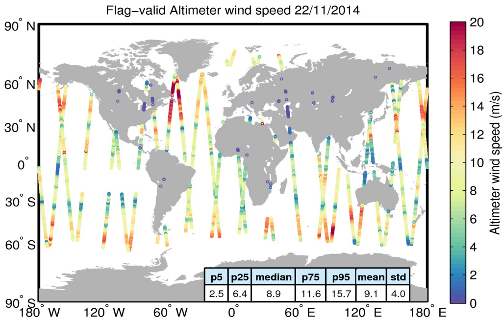
Figure 31. Geographical distribution of flag-valid wind data over oceans and lakes for 22/11/2014. The statistical values shown in the table refer to the wind in m/s and are calculated over all measurements shown in the figure.
