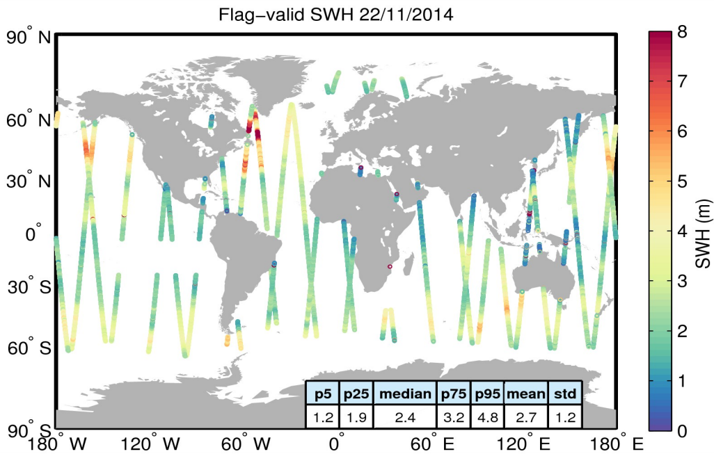
Figure 15. Geographical distribution of flag-valid SWH data over oceans and lakes for 22/11/2014. The statistical values shown in the table refer to the SWH in m and are calculated over all measurements shown in the figure.
