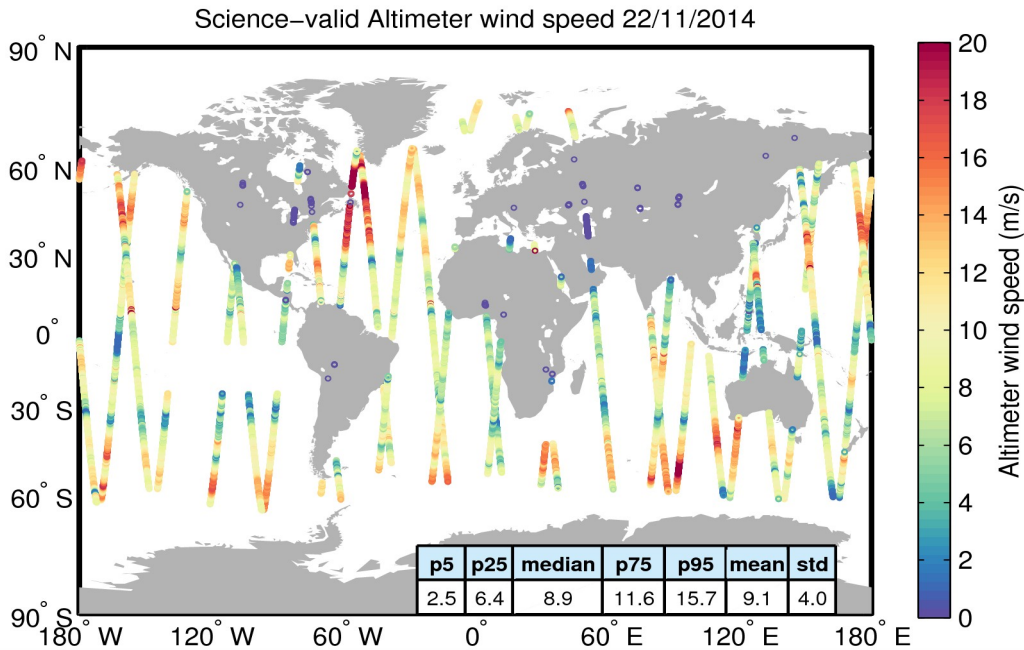
Figure 34. Geographical distribution of science-valid wind data over oceans and lakes for 22/11/2014. The statistical values shown in the table refer to the wind in m/s and are calculated over all measurements shown in the figure. Gray circles denote records that have been rejected based on the editing criteria described in Table 5.
