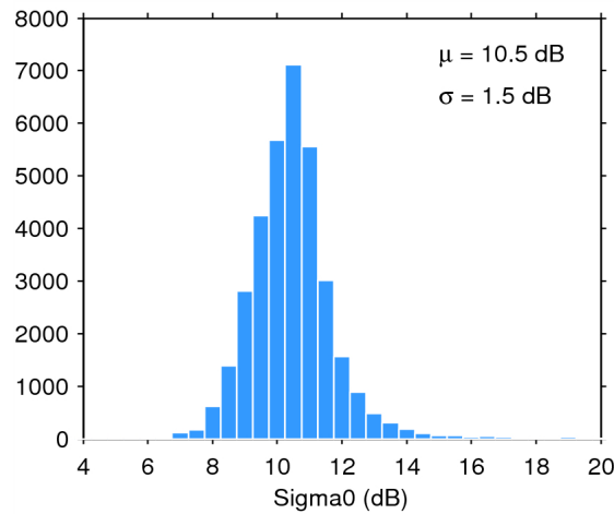
Figure 28. Histogram of science-valid sigma0 over oceans and lakes for 22/11/2014. The mean ( \mu ) and standard deviation ( \sigma ) are also shown. Note that values outside [4 20] dB are excluded from the histogram for the sake of readability but not from the computation of \mu and \sigma .
