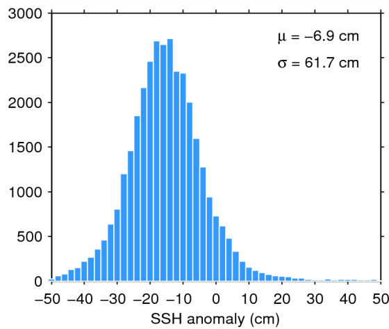
Figure 7. Histogram of flag-valid SSH anomaly over oceans and lakes for 22/11/2014. The mean ( \mu ) and standard deviation ( \sigma ) are also shown. Note that values outside [-50\ 50] cm are excluded from the histogram for the sake of readability but not from the computation of \mu and \sigma .
