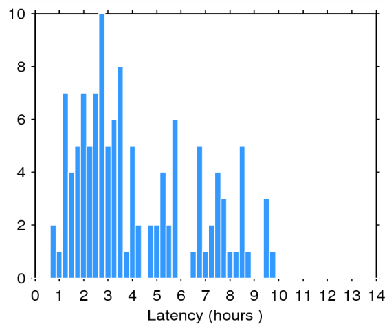
Figure 2. Histogram of the data latency for 22/11/2014. The y-axis denotes the number of files that are made available with a delay of x-hours with respect to the mean time of the records stored in the file.
