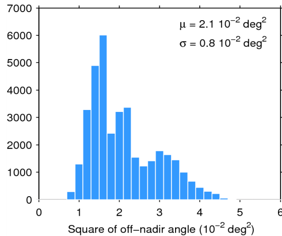
Figure 39. Histogram of flag-valid mispointing over oceans and lakes for 22/11/2014. The mean ( \mu ) and standard deviation ( \sigma ) are also shown. Note that values than 6 \cdot 10^{-2} \text{ deg}^2 are excluded from the histogram for the sake of readability but not from the computation of \mu and \sigma .
