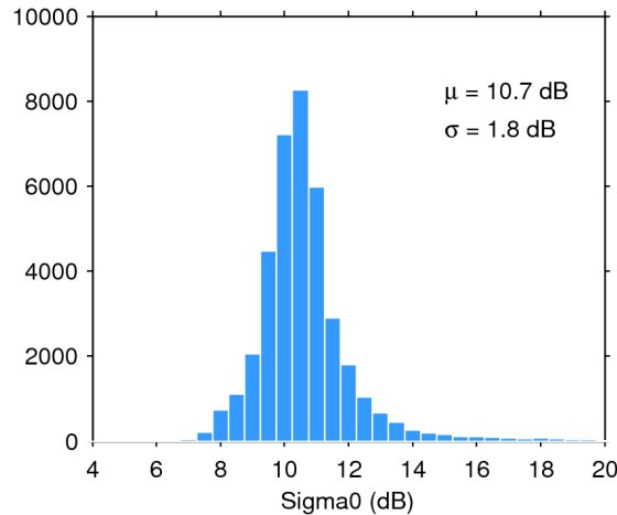
Figure 25. Histogram of flag-valid sigma0 over oceans and lakes for 21/11/2014. The mean ( \mu ) and standard deviation ( \sigma ) are also shown. Note that values outside [4 20] dB are excluded from the histogram for the sake of readability but not from the computation of \mu and \sigma .
