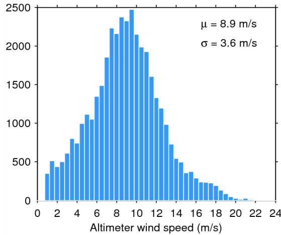
Figure 33. Histogram of flag-valid wind over oceans and lakes for 21/11/2014. The mean ( \mu ) and standard deviation ( \sigma ) are also shown. Note that values larger than 24 m/s are excluded from the histogram for the sake of readability but not from the computation of \mu and \sigma .
