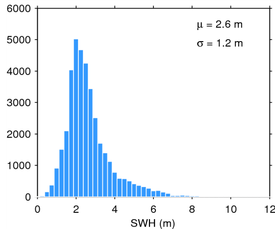
Figure 20. Histogram of science-valid SWH over oceans and lakes for 21/11/2014. The mean ( \mu ) and standard deviation ( \sigma ) are also shown. Note that values larger than 12 m are excluded from the histogram for the sake of readability but not from the computation of \mu and \sigma .
