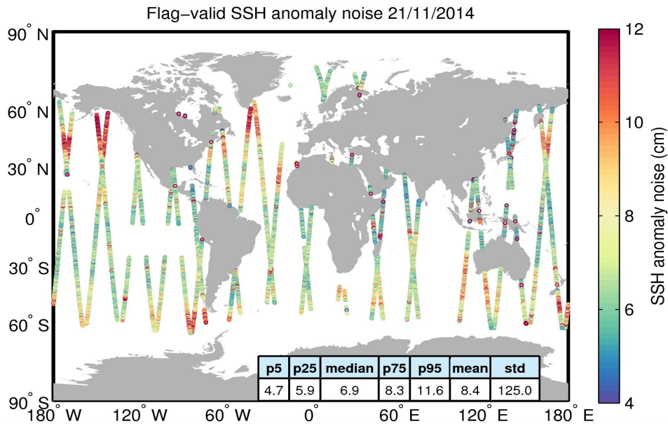
Figure 8. Geographical distribution of flag-valid 20-Hz SSH anomaly measurement noise over oceans and lakes for 21/11/2014. The statistical values shown in the table refer to the SSH anomaly noise and are calculated over all measurements shown in the figure.
