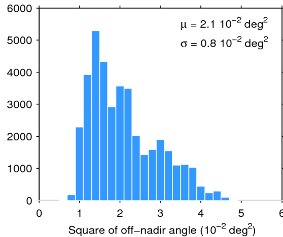
Figure 39. Histogram of flag-valid mispointing over oceans and lakes for 21/11/2014. The mean ( \mu ) and standard deviation ( \sigma ) are also shown. Note that values than 6 \cdot 10^{-2} \text{ deg}^2 are excluded from the histogram for the sake of readability but not from the computation of \mu and \sigma .
