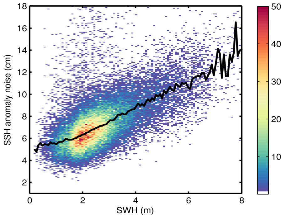
Figure 9. 2D histogram showing flag-valid SSH anomaly noise as a function of SWH for 21/11/2014. The black line denotes the median SSH anomaly as a function of SWH.
