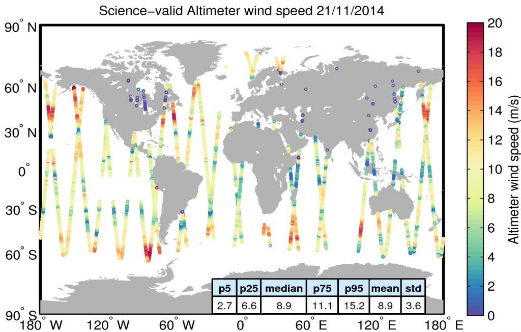
Figure 34. Geographical distribution of science-valid wind data over oceans and lakes for 21/11/2014. The statistical values shown in the table refer to the wind in m/s and are calculated over all measurements shown in the figure. Gray circles denote records that have been rejected based on the editing criteria described in Table 5.
