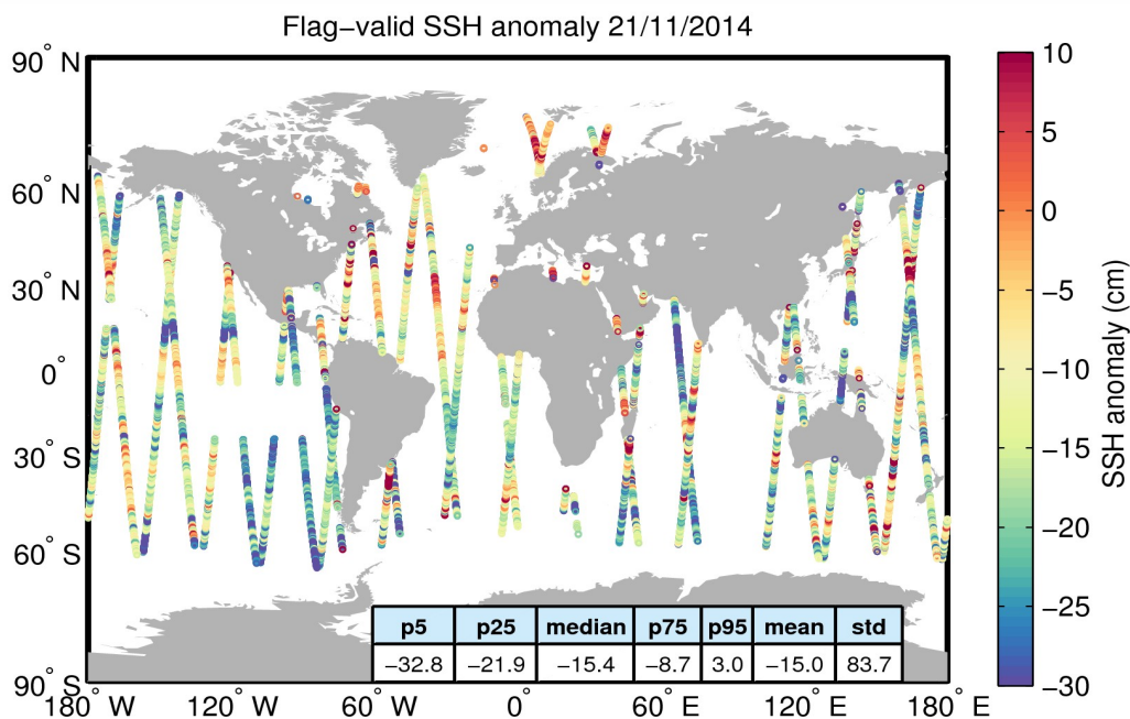
Figure 5. Geographical distribution of flag-valid 1-Hz SSH anomaly data over oceans and lakes for 21/11/2014. The statistical values shown in the table refer to the SSH anomaly in cm and are calculated over all measurements shown in the figure.
