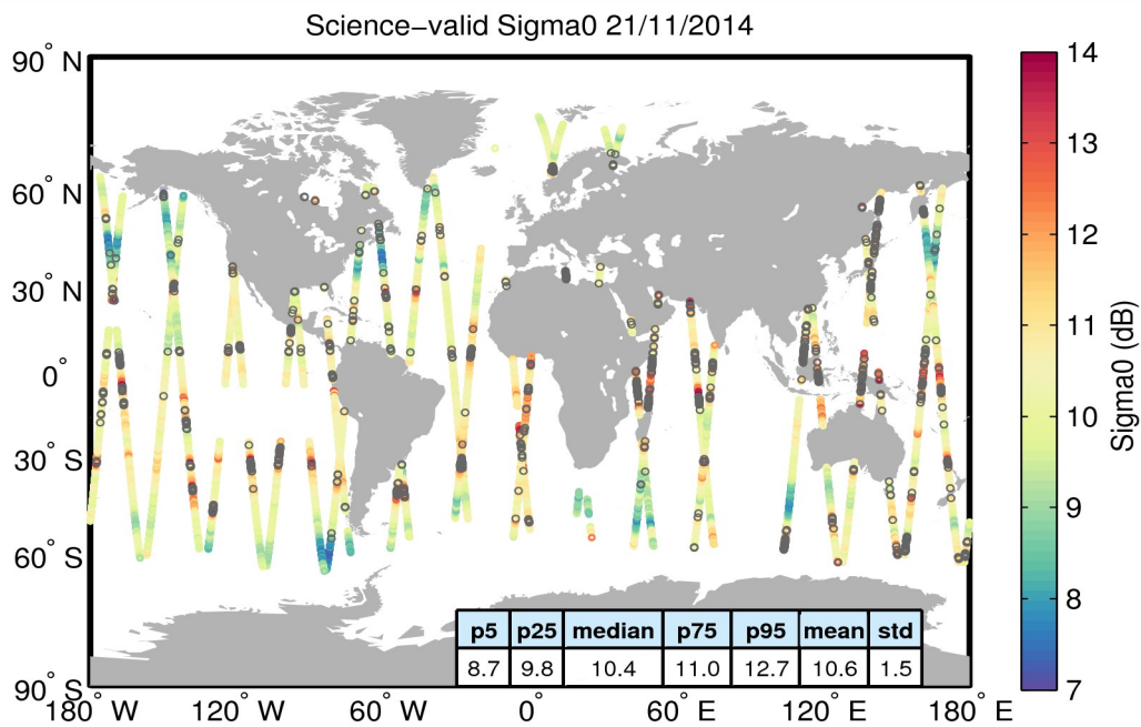
Figure 27. Geographical distribution of science-valid sigma0 data over oceans and lakes for 21/11/2014. The statistical values shown in the table refer to the sigma0 in dB and are calculated over all measurements shown in the figure. Gray circles denote records that have been rejected based on the editing criteria described in Table 4.
