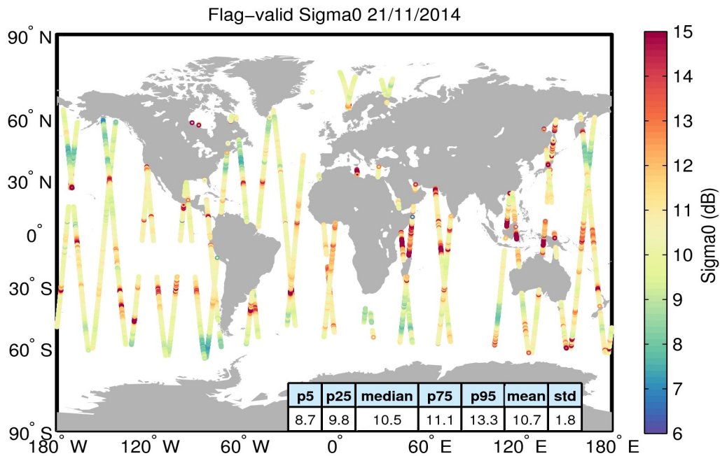
Figure 23. Geographical distribution of flag-valid sigma0 data over oceans and lakes for 21/11/2014. The statistical values shown in the table refer to the sigma0 in dB and are calculated over all measurements shown in the figure.
