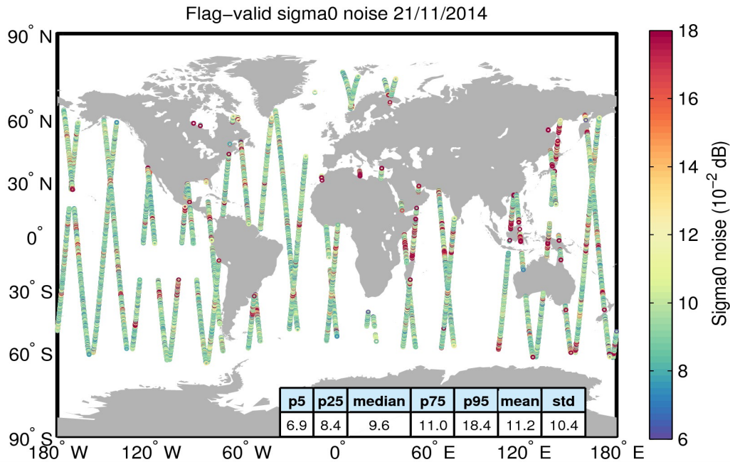
Figure 26. Geographical distribution of flag-valid 20-Hz sigma0 measurement noise over oceans and lakes for 21/11/2014. The statistical values shown in the table refer to the sigma0 noise and are calculated over all measurements shown in the figure.
