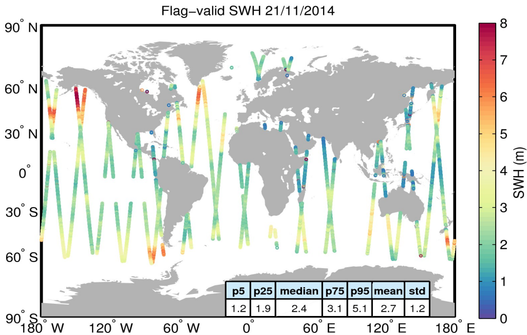
Figure 15. Geographical distribution of flag-valid SWH data over oceans and lakes for 21/11/2014. The statistical values shown in the table refer to the SWH in m and are calculated over all measurements shown in the figure.
