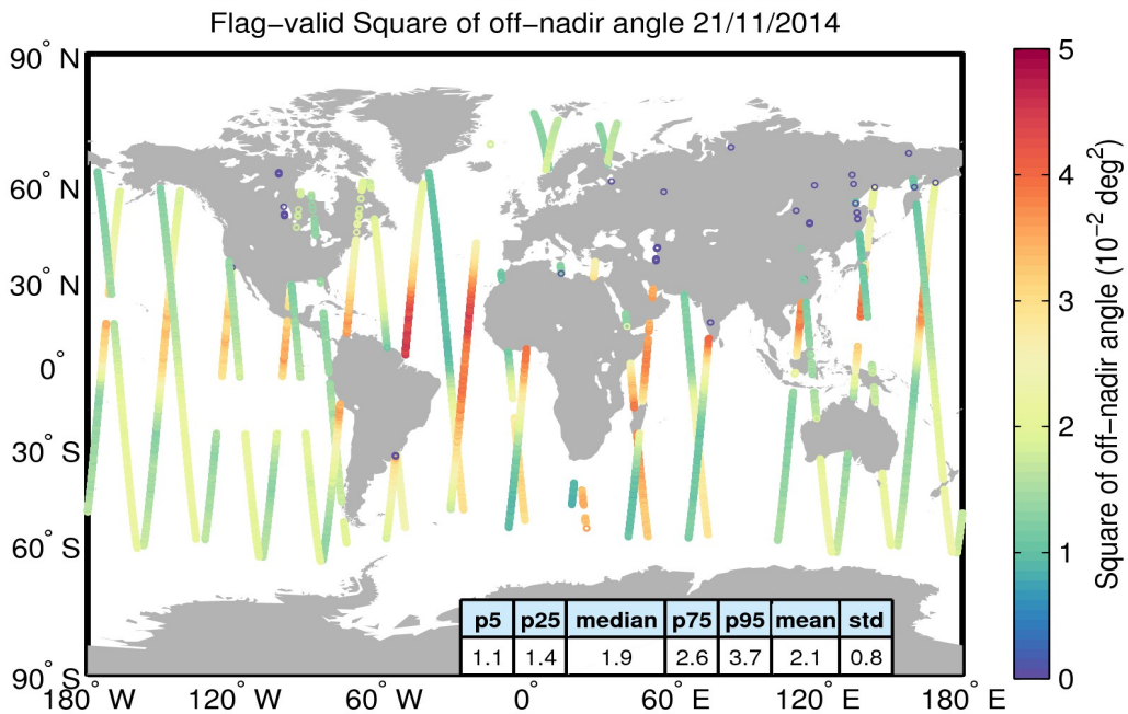
Figure 37. Geographical distribution of flag-valid mispointing data over oceans and lakes for 21/11/2014. The statistical values shown in the table refer to the mispointing in 10^{-2} \text{deg}^2 and are calculated over all measurements shown in the figure.
