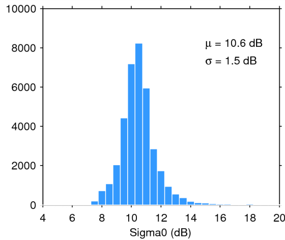
Figure 28. Histogram of science-valid sigma0 over oceans and lakes for 21/11/2014. The mean ( \mu ) and standard deviation ( \sigma ) are also shown. Note that values outside [4 20] dB are excluded from the histogram for the sake of readability but not from the computation of \mu and \sigma .
