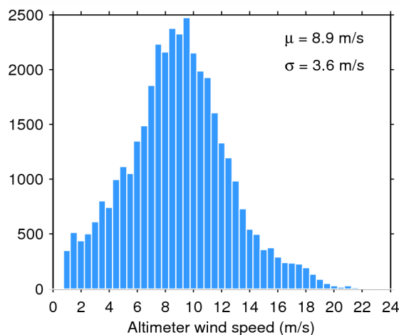
Figure 35. Histogram of science-valid wind over oceans and lakes for 21/11/2014. The mean ( \mu ) and standard deviation ( \sigma ) are also shown. Note that values larger than 24 m/s are excluded from the histogram for the sake of readability but not from the computation of \mu and \sigma .
