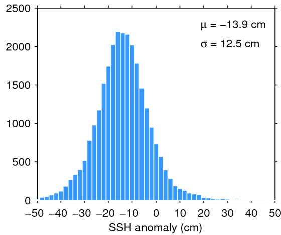
Figure 11. Histogram of science-valid SSH anomaly over oceans and lakes for 20/11/2014. The mean ( \mu ) and standard deviation ( \sigma ) are also shown. Note that values outside [-50 50] cm are excluded from the histogram for the sake of readability but not from the computation of \mu and \sigma .
