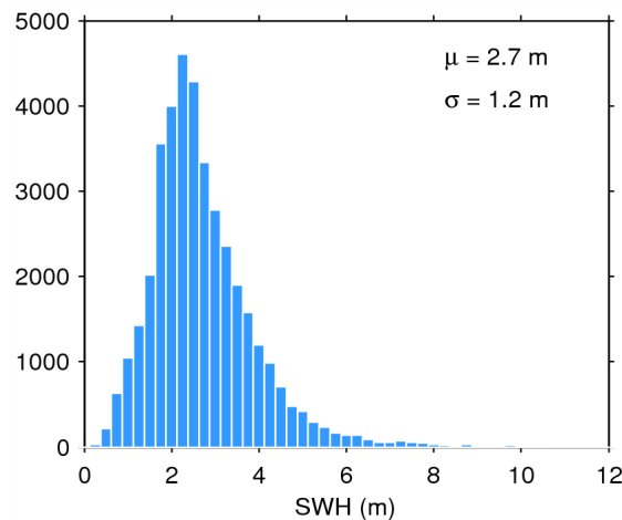
Figure 20. Histogram of science-valid SWH over oceans and lakes for 20/11/2014. The mean ( \mu ) and standard deviation ( \sigma ) are also shown. Note that values larger than 12 m are excluded from the histogram for the sake of readability but not from the computation of \mu and \sigma .
