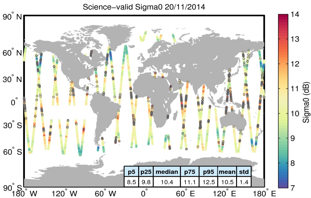
Figure 27. Geographical distribution of science-valid sigma0 data over oceans and lakes for 20/11/2014. The statistical values shown in the table refer to the sigma0 in dB and are calculated over all measurements shown in the figure. Gray circles denote records that have been rejected based on the editing criteria described in Table 4.
