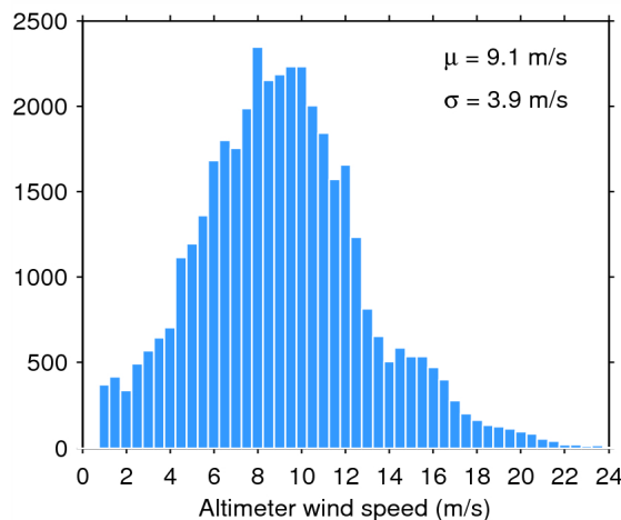
Figure 35. Histogram of science-valid wind over oceans and lakes for 20/11/2014. The mean ( \mu ) and standard deviation ( \sigma ) are also shown. Note that values larger than 24 m/s are excluded from the histogram for the sake of readability but not from the computation of \mu and \sigma .
