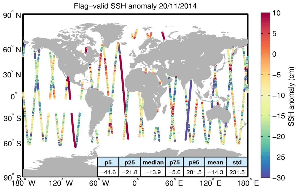
Figure 5. Geographical distribution of flag-valid 1-Hz SSH anomaly data over oceans and lakes for 20/11/2014. The statistical values shown in the table refer to the SSH anomaly in cm and are calculated over all measurements shown in the figure.
