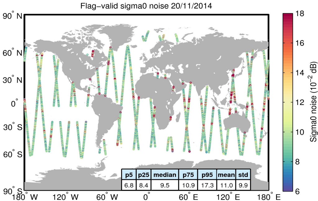
Figure 26. Geographical distribution of flag-valid 20-Hz sigma0 measurement noise over oceans and lakes for 20/11/2014. The statistical values shown in the table refer to the sigma0 noise and are calculated over all measurements shown in the figure.
