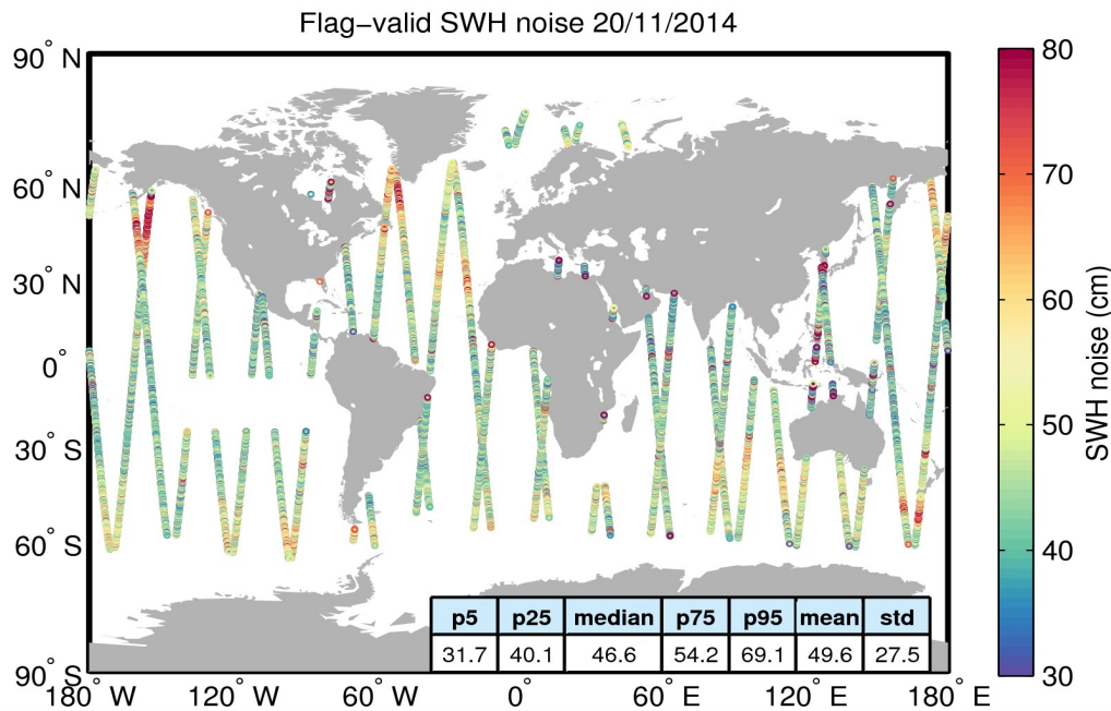
Figure 18. Geographical distribution of flag-valid 20-Hz SWH measurement noise over oceans and lakes for 20/11/2014. The statistical values shown in the figure refer to the SWH noise and are calculated over all measurements shown in the figure.
