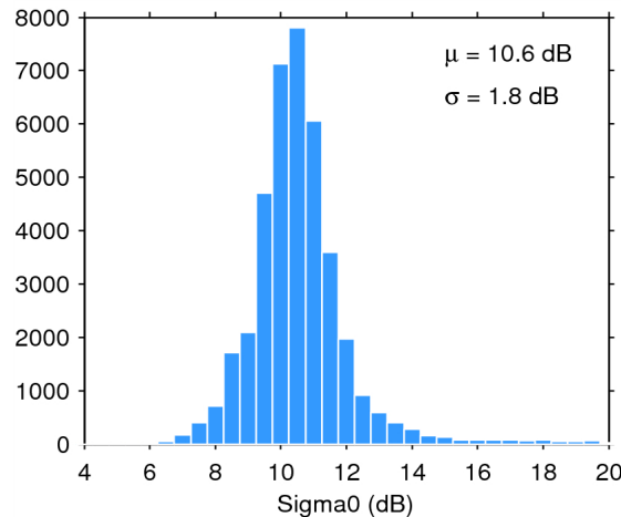
Figure 25. Histogram of flag-valid sigma0 over oceans and lakes for 20/11/2014. The mean ( \mu ) and standard deviation ( \sigma ) are also shown. Note that values outside [4 20] dB are excluded from the histogram for the sake of readability but not from the computation of \mu and \sigma .
