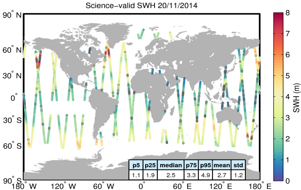
Figure 19. Geographical distribution of science-valid SWH data over oceans and lakes for 20/11/2014. The statistical values shown in the table refer to the SWH in m and are calculated over all measurements shown in the figure. Gray circles denote records that have been rejected based on the editing criteria described in Table 3.
