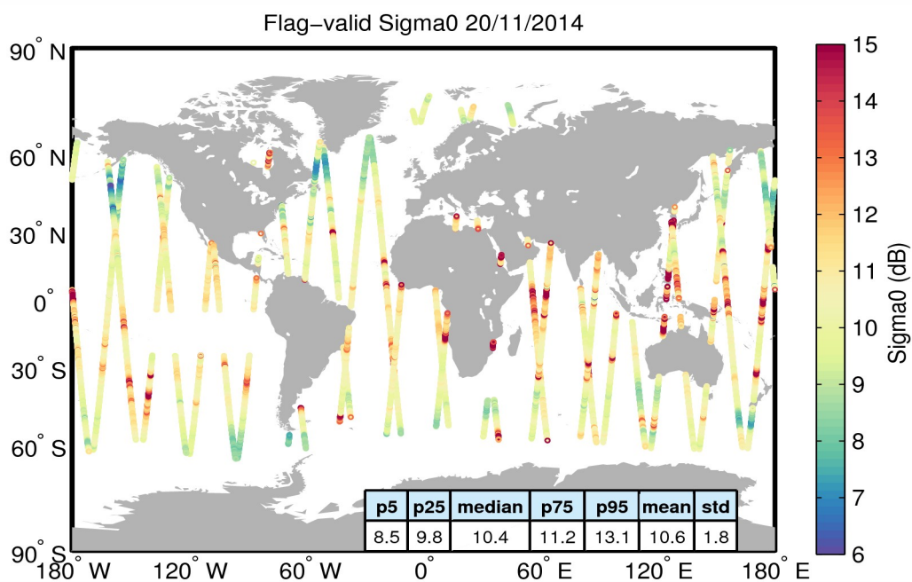
Figure 23. Geographical distribution of flag-valid sigma0 data over oceans and lakes for 20/11/2014. The statistical values shown in the table refer to the sigma0 in dB and are calculated over all measurements shown in the figure.
