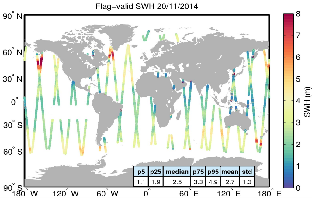
Figure 15. Geographical distribution of flag-valid SWH data over oceans and lakes for 20/11/2014. The statistical values shown in the table refer to the SWH in m and are calculated over all measurements shown in the figure.
