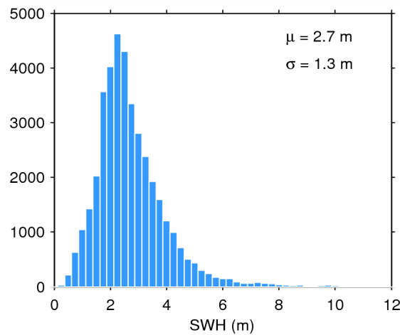
Figure 17. Histogram of flag-valid SWH over oceans and lakes for 20/11/2014. The mean ( \mu ) and standard deviation ( \sigma ) are also shown. Note that values larger than 12 m are excluded from the histogram for the sake of readability but not from the computation of \mu and \sigma .
