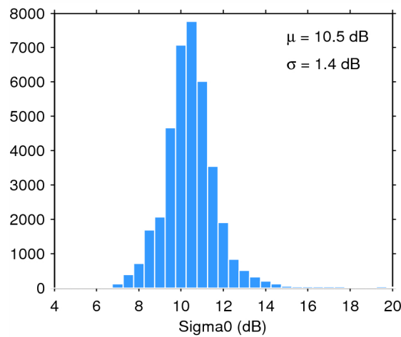
Figure 28. Histogram of science-valid sigma0 over oceans and lakes for 20/11/2014. The mean ( \mu ) and standard deviation ( \sigma ) are also shown. Note that values outside [4 20] dB are excluded from the histogram for the sake of readability but not from the computation of \mu and \sigma .
