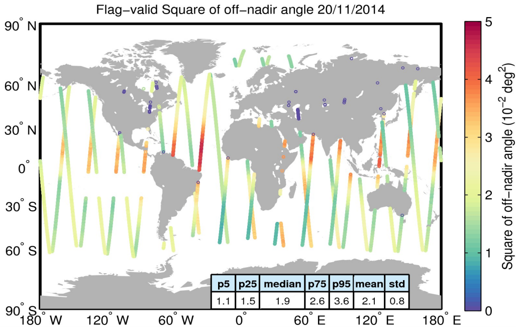
Figure 37. Geographical distribution of flag-valid mispointing data over oceans and lakes for 20/11/2014. The statistical values shown in the table refer to the mispointing in 10^{-2} \text{deg}^2 and are calculated over all measurements shown in the figure.
