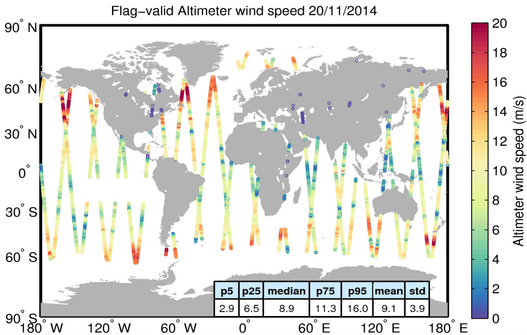
Figure 31. Geographical distribution of flag-valid wind data over oceans and lakes for 20/11/2014. The statistical values shown in the table refer to the wind in m/s and are calculated over all measurements shown in the figure.
