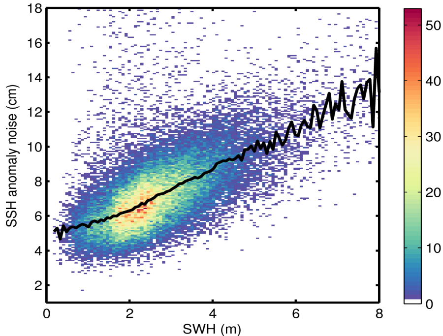
Figure 9. 2D histogram showing flag-valid SSH anomaly noise as a function of SWH for 20/11/2014. The black line denotes the median SSH anomaly as a function of SWH.
