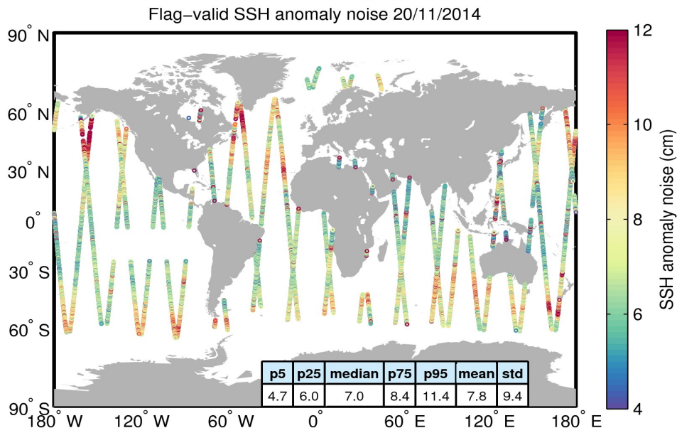
Figure 8. Geographical distribution of flag-valid 20-Hz SSH anomaly measurement noise over oceans and lakes for 20/11/2014. The statistical values shown in the table refer to the SSH anomaly noise and are calculated over all measurements shown in the figure.
