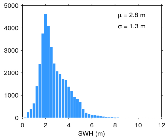
Figure 17. Histogram of flag-valid SWH over oceans and lakes for 18/11/2014. The mean ( \mu ) and standard deviation ( \sigma ) are also shown. Note that values larger than 12 m are excluded from the histogram for the sake of readability but not from the computation of \mu and \sigma .
