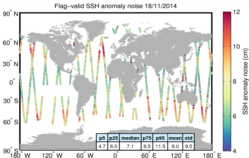
Figure 8. Geographical distribution of flag-valid 20-Hz SSH anomaly measurement noise over oceans and lakes for 18/11/2014. The statistical values shown in the table refer to the SSH anomaly noise and are calculated over all measurements shown in the figure.
