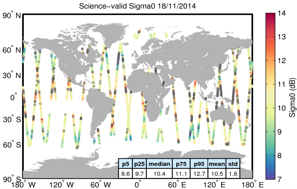
Figure 27. Geographical distribution of science-valid sigma0 data over oceans and lakes for 18/11/2014. The statistical values shown in the table refer to the sigma0 in dB and are calculated over all measurements shown in the figure. Gray circles denote records that have been rejected based on the editing criteria described in Table 4.
