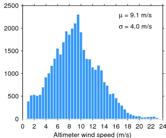
Figure 35. Histogram of science-valid wind over oceans and lakes for 18/11/2014. The mean ( \mu ) and standard deviation ( \sigma ) are also shown. Note that values larger than 24 m/s are excluded from the histogram for the sake of readability but not from the computation of \mu and \sigma .
