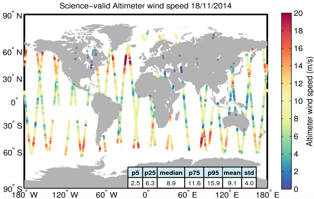
Figure 34. Geographical distribution of science-valid wind data over oceans and lakes for 18/11/2014. The statistical values shown in the table refer to the wind in m/s and are calculated over all measurements shown in the figure. Gray circles denote records that have been rejected based on the editing criteria described in Table 5.
