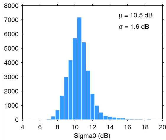
Figure 28. Histogram of science-valid sigma0 over oceans and lakes for 18/11/2014. The mean ( \mu ) and standard deviation ( \sigma ) are also shown. Note that values outside [4 20] dB are excluded from the histogram for the sake of readability but not from the computation of \mu and \sigma .
