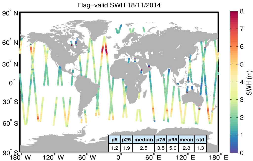
Figure 15. Geographical distribution of flag-valid SWH data over oceans and lakes for 18/11/2014. The statistical values shown in the table refer to the SWH in m and are calculated over all measurements shown in the figure.
