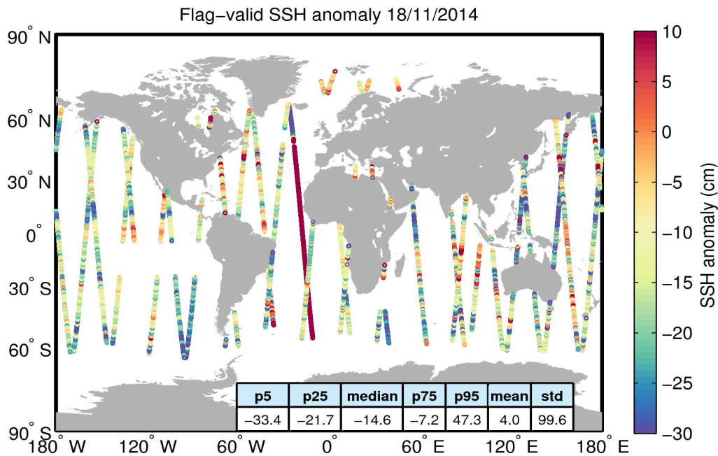
Figure 5. Geographical distribution of flag-valid 1-Hz SSH anomaly data over oceans and lakes for 18/11/2014. The statistical values shown in the table refer to the SSH anomaly in cm and are calculated over all measurements shown in the figure.
