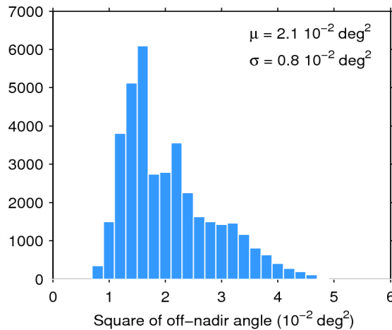
Figure 39. Histogram of flag-valid mispointing over oceans and lakes for 18/11/2014. The mean ( \mu ) and standard deviation ( \sigma ) are also shown. Note that values than 6 \cdot 10^{-2} \text{ deg}^2 are excluded from the histogram for the sake of readability but not from the computation of \mu and \sigma .
