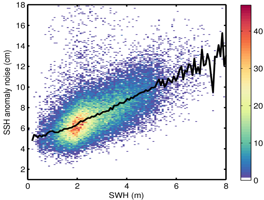
Figure 9. 2D histogram showing flag-valid SSH anomaly noise as a function of SWH for 18/11/2014. The black line denotes the median SSH anomaly as a function of SWH.
