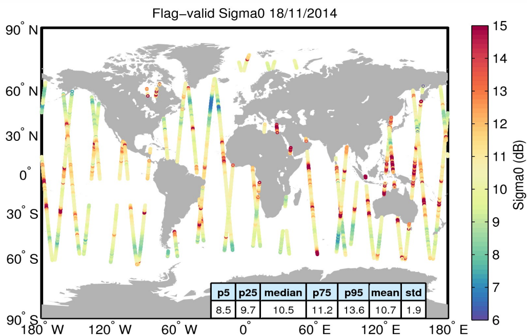
Figure 23. Geographical distribution of flag-valid sigma0 data over oceans and lakes for 18/11/2014. The statistical values shown in the table refer to the sigma0 in dB and are calculated over all measurements shown in the figure.
