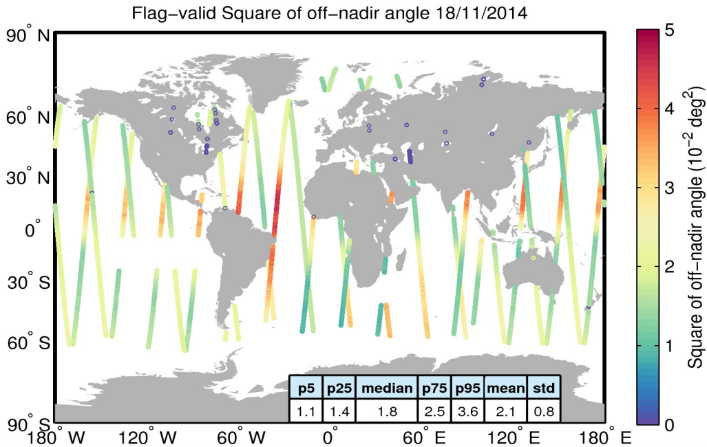
Figure 37. Geographical distribution of flag-valid mispointing data over oceans and lakes for 18/11/2014. The statistical values shown in the table refer to the mispointing in 10^{-2} \text{ deg}^2 and are calculated over all measurements shown in the figure.
