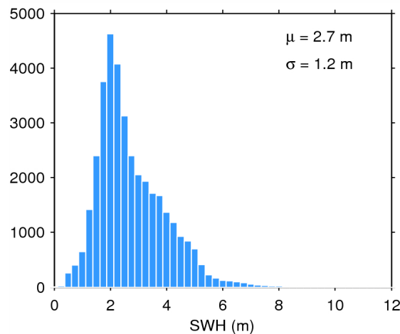
Figure 20. Histogram of science-valid SWH over oceans and lakes for 18/11/2014. The mean ( \mu ) and standard deviation ( \sigma ) are also shown. Note that values larger than 12 m are excluded from the histogram for the sake of readability but not from the computation of \mu and \sigma .
