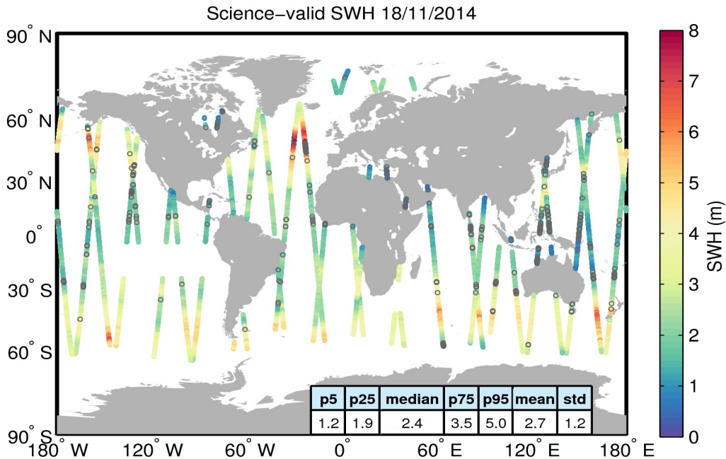
Figure 19. Geographical distribution of science-valid SWH data over oceans and lakes for 18/11/2014. The statistical values shown in the table refer to the SWH in m and are calculated over all measurements shown in the figure. Gray circles denote records that have been rejected based on the editing criteria described in Table 3.
