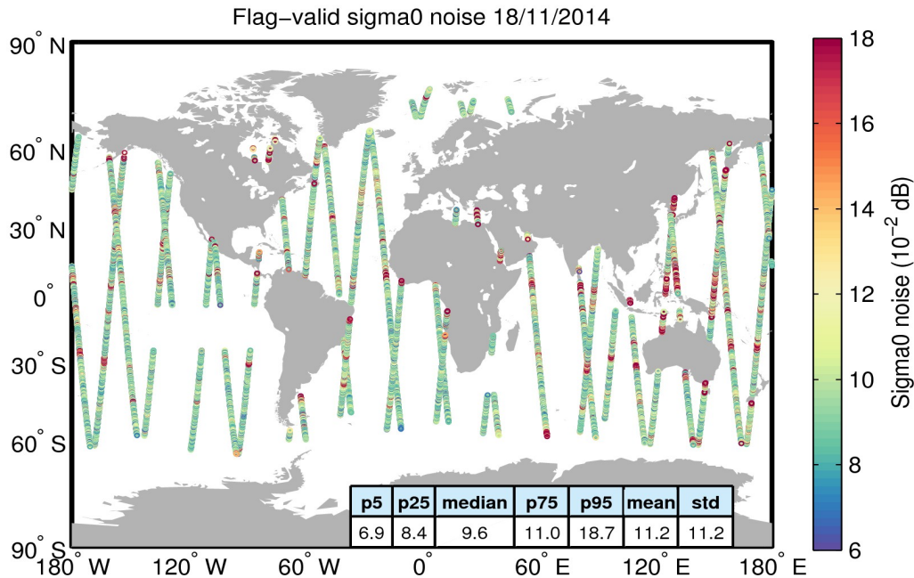
Figure 26. Geographical distribution of flag-valid 20-Hz sigma0 measurement noise over oceans and lakes for 18/11/2014. The statistical values shown in the table refer to the sigma0 noise and are calculated over all measurements shown in the figure.
