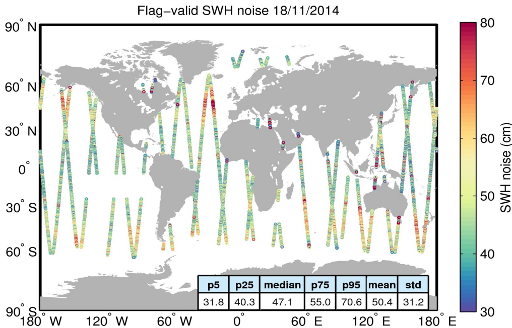
Figure 18. Geographical distribution of flag-valid 20-Hz SWH measurement noise over oceans and lakes for 18/11/2014. The statistical values shown in the figure refer to the SWH noise and are calculated over all measurements shown in the figure.
