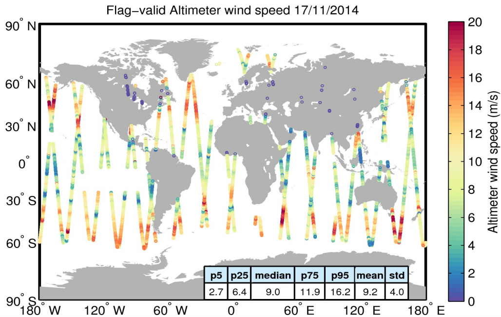
Figure 31. Geographical distribution of flag-valid wind data over oceans and lakes for 17/11/2014. The statistical values shown in the table refer to the wind in m/s and are calculated over all measurements shown in the figure.
