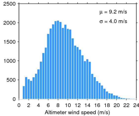
Figure 33. Histogram of flag-valid wind over oceans and lakes for 17/11/2014. The mean ( \mu ) and standard deviation ( \sigma ) are also shown. Note that values larger than 24 m/s are excluded from the histogram for the sake of readability but not from the computation of \mu and \sigma .
