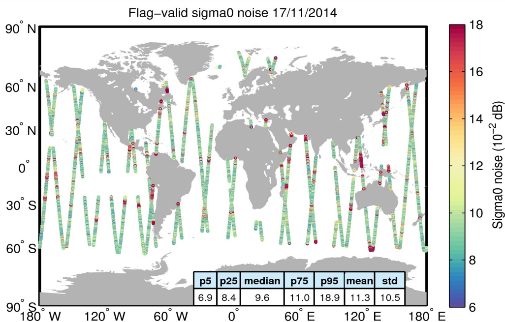
Figure 26. Geographical distribution of flag-valid 20-Hz sigma0 measurement noise over oceans and lakes for 17/11/2014. The statistical values shown in the table refer to the sigma0 noise and are calculated over all measurements shown in the figure.
