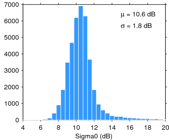
Figure 25. Histogram of flag-valid sigma0 over oceans and lakes for 17/11/2014. The mean ( \mu ) and standard deviation ( \sigma ) are also shown. Note that values outside [4 20] dB are excluded from the histogram for the sake of readability but not from the computation of \mu and \sigma .
