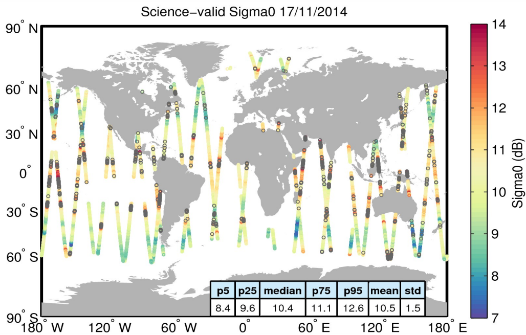
Figure 27. Geographical distribution of science-valid sigma0 data over oceans and lakes for 17/11/2014. The statistical values shown in the table refer to the sigma0 in dB and are calculated over all measurements shown in the figure. Gray circles denote records that have been rejected based on the editing criteria described in Table 4.
