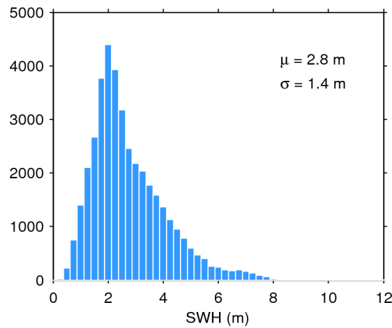
Figure 17. Histogram of flag-valid SWH over oceans and lakes for 17/11/2014. The mean ( \mu ) and standard deviation ( \sigma ) are also shown. Note that values larger than 12 m are excluded from the histogram for the sake of readability but not from the computation of \mu and \sigma .
