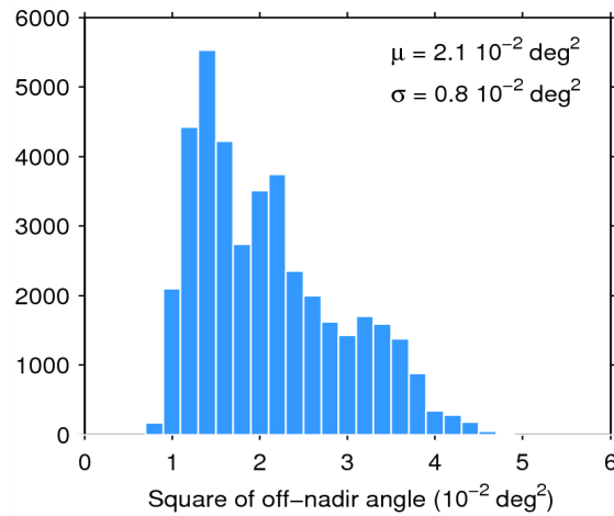
Figure 39. Histogram of flag-valid mispointing over oceans and lakes for 17/11/2014. The mean ( \mu ) and standard deviation ( \sigma ) are also shown. Note that values than 6 \cdot 10^{-2} \text{ deg}^2 are excluded from the histogram for the sake of readability but not from the computation of \mu and \sigma .
