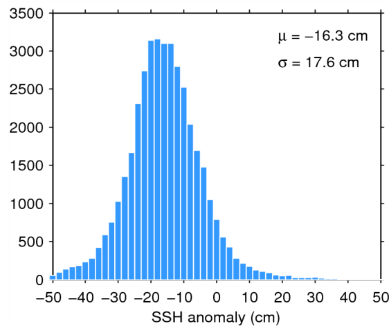
Figure 7. Histogram of flag-valid SSH anomaly over oceans and lakes for 17/11/2014. The mean ( \mu ) and standard deviation ( \sigma ) are also shown. Note that values outside [-50\ 50] cm are excluded from the histogram for the sake of readability but not from the computation of \mu and \sigma .
