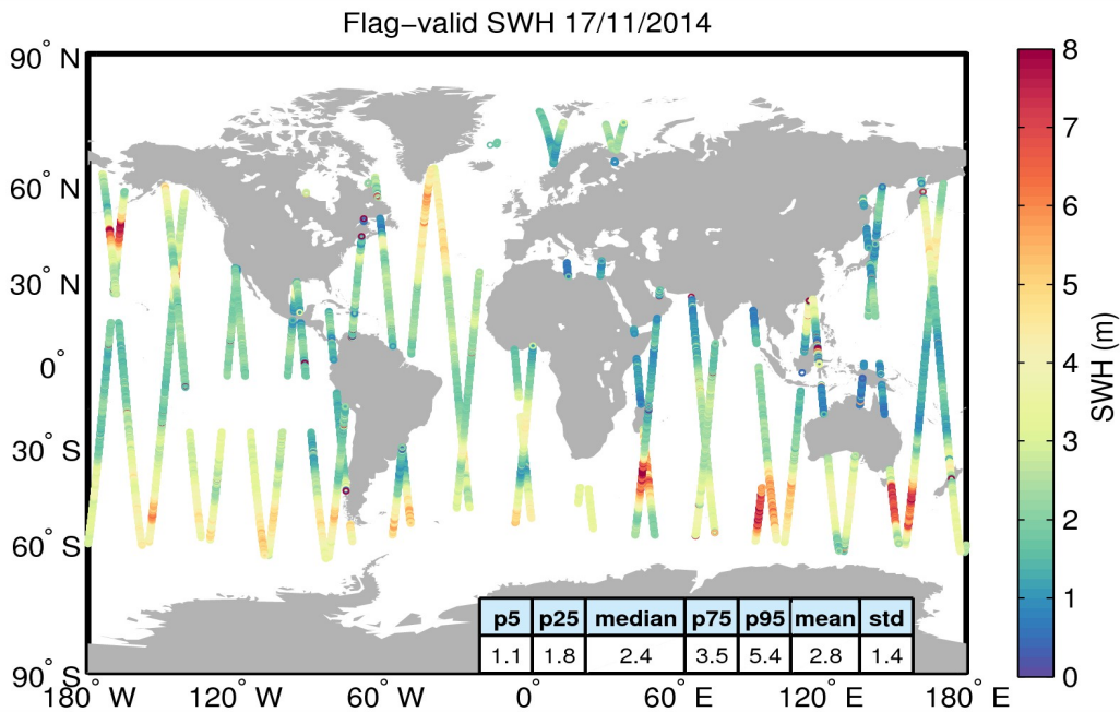
Figure 15. Geographical distribution of flag-valid SWH data over oceans and lakes for 17/11/2014. The statistical values shown in the table refer to the SWH in m and are calculated over all measurements shown in the figure.
