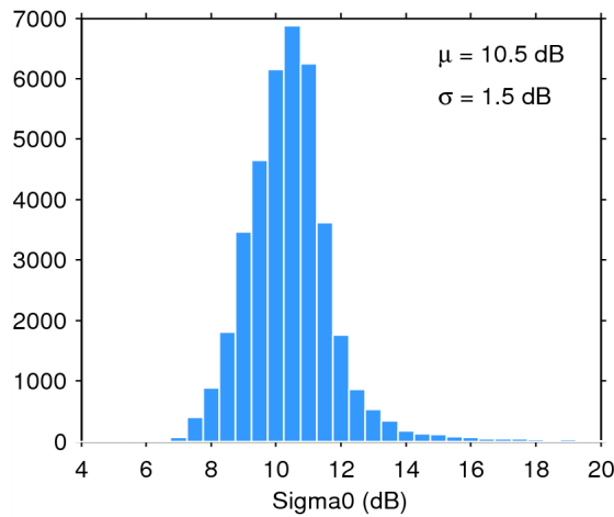
Figure 28. Histogram of science-valid sigma0 over oceans and lakes for 17/11/2014. The mean ( \mu ) and standard deviation ( \sigma ) are also shown. Note that values outside [4 20] dB are excluded from the histogram for the sake of readability but not from the computation of \mu and \sigma .
