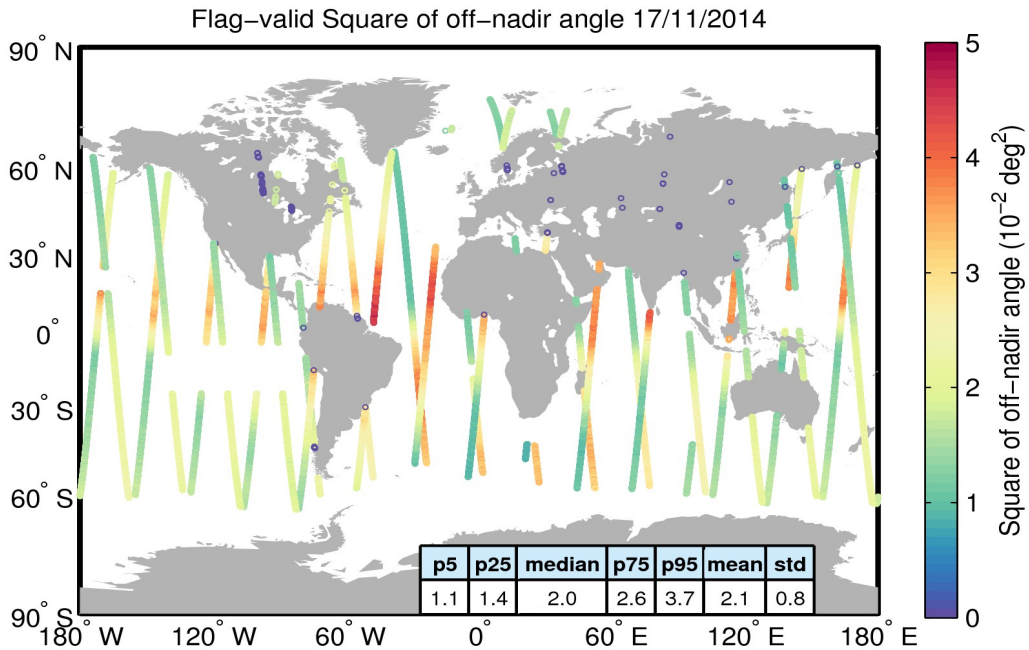
Figure 37. Geographical distribution of flag-valid mispointing data over oceans and lakes for 17/11/2014. The statistical values shown in the table refer to the mispointing in 10^{-2} \text{deg}^2 and are calculated over all measurements shown in the figure.
