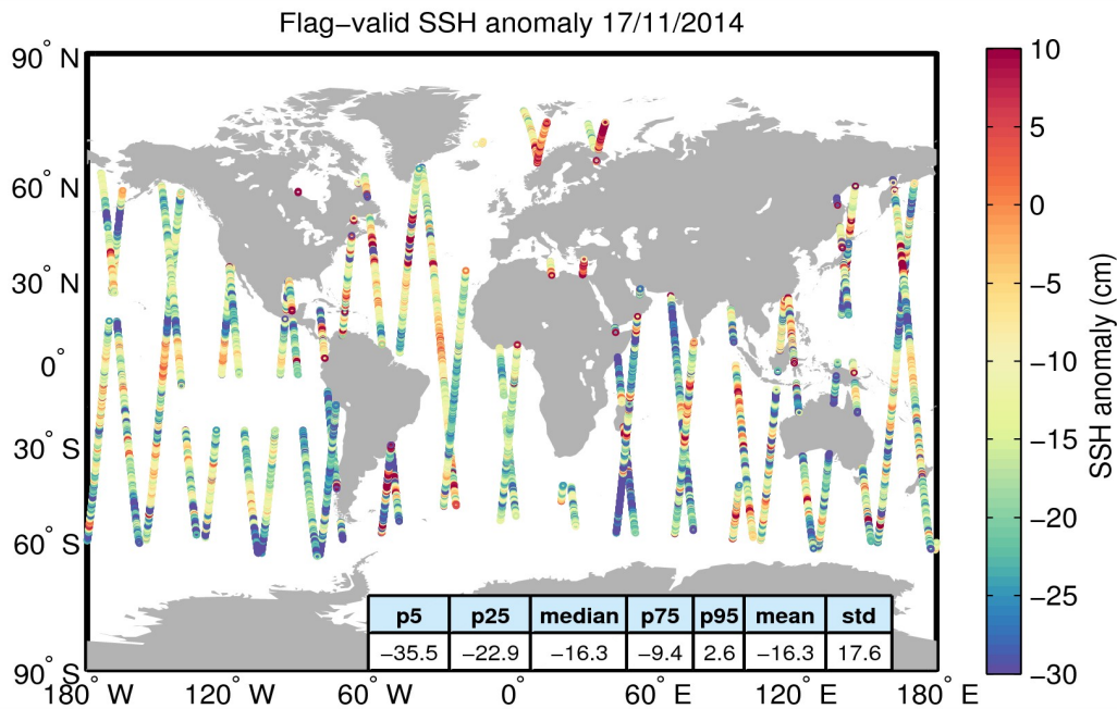
Figure 5. Geographical distribution of flag-valid 1-Hz SSH anomaly data over oceans and lakes for 17/11/2014. The statistical values shown in the table refer to the SSH anomaly in cm and are calculated over all measurements shown in the figure.
