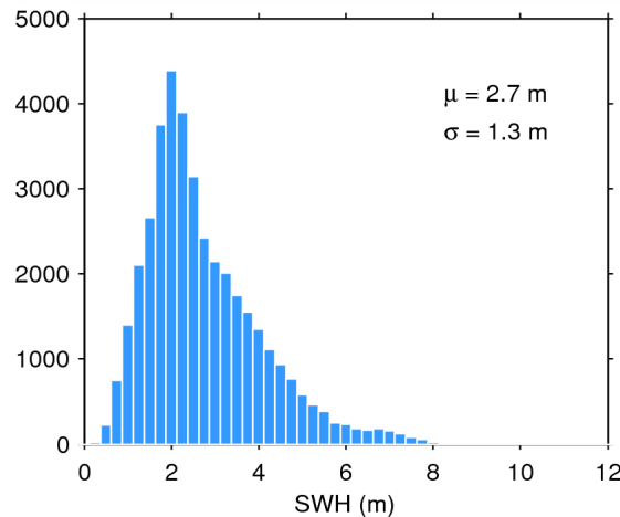
Figure 20. Histogram of science-valid SWH over oceans and lakes for 17/11/2014. The mean ( \mu ) and standard deviation ( \sigma ) are also shown. Note that values larger than 12 m are excluded from the histogram for the sake of readability but not from the computation of \mu and \sigma .
