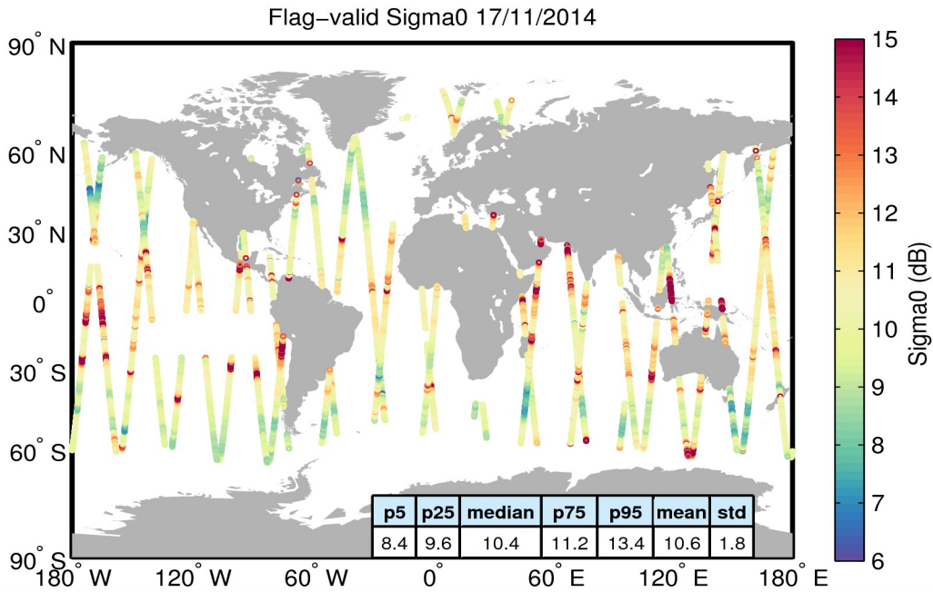
Figure 23. Geographical distribution of flag-valid sigma0 data over oceans and lakes for 17/11/2014. The statistical values shown in the table refer to the sigma0 in dB and are calculated over all measurements shown in the figure.
