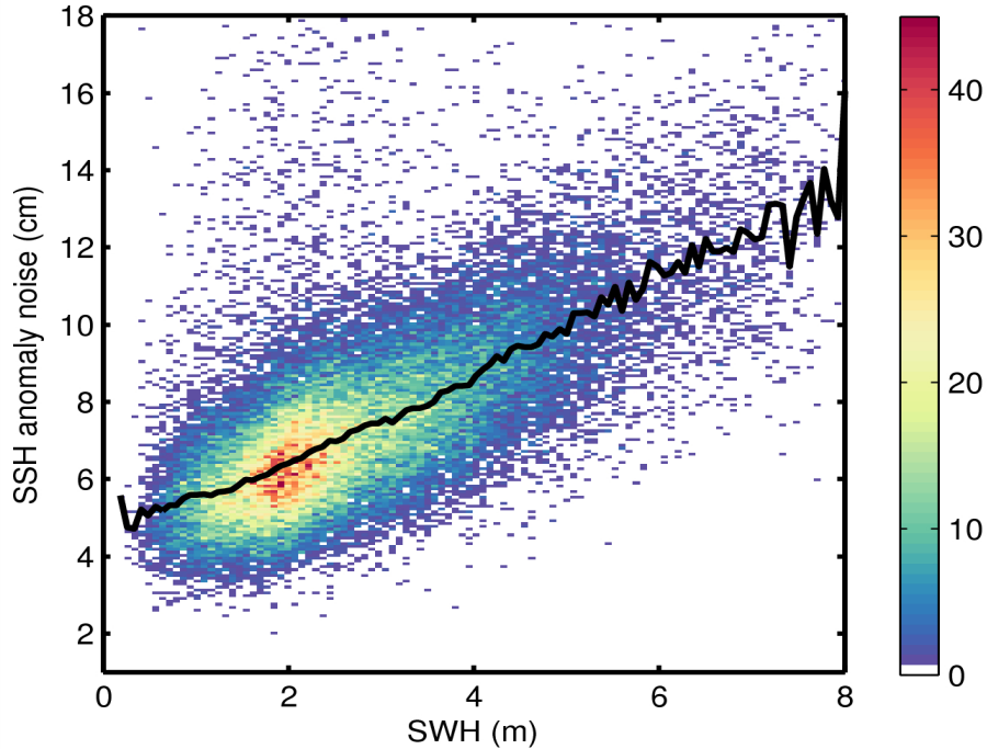
Figure 9. 2D histogram showing flag-valid SSH anomaly noise as a function of SWH for 17/11/2014. The black line denotes the median SSH anomaly as a function of SWH.
