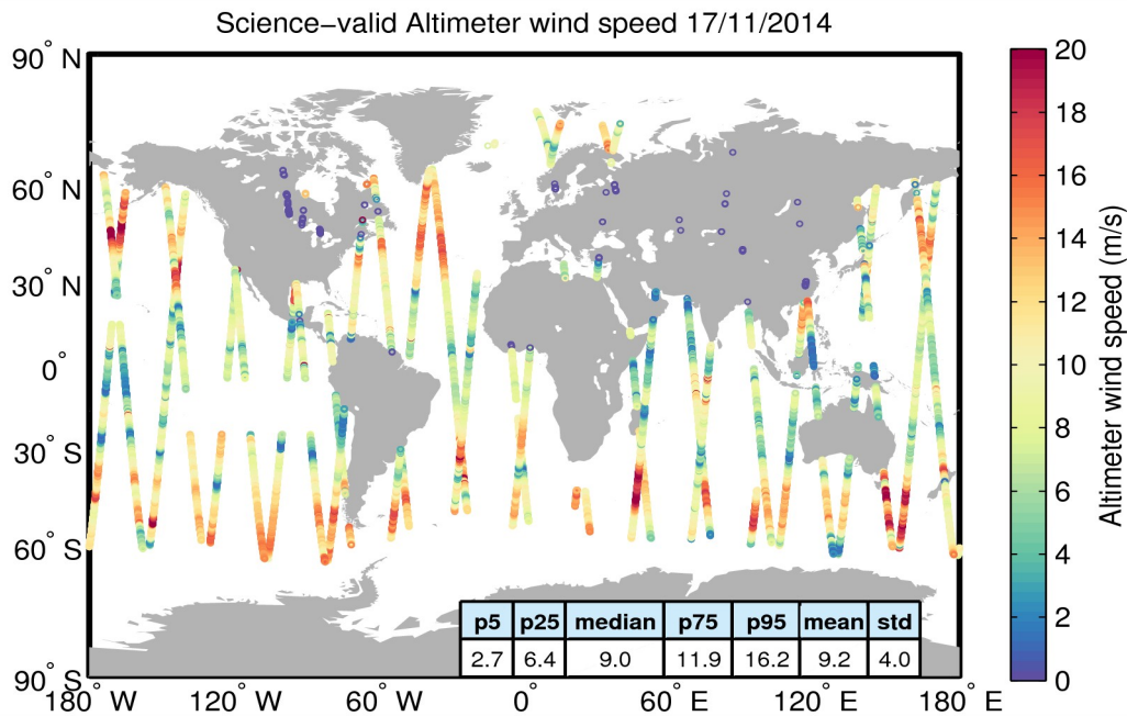
Figure 34. Geographical distribution of science-valid wind data over oceans and lakes for 17/11/2014. The statistical values shown in the table refer to the wind in m/s and are calculated over all measurements shown in the figure. Gray circles denote records that have been rejected based on the editing criteria described in Table 5.
