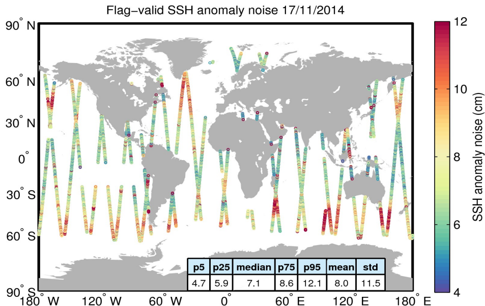
Figure 8. Geographical distribution of flag-valid 20-Hz SSH anomaly measurement noise over oceans and lakes for 17/11/2014. The statistical values shown in the table refer to the SSH anomaly noise and are calculated over all measurements shown in the figure.
