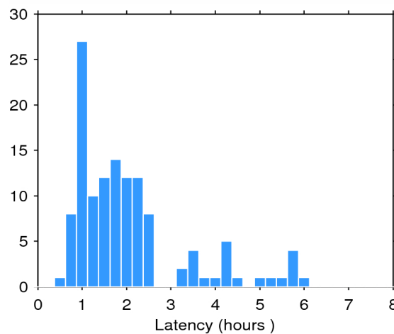
Figure 2. Histogram of the data latency for 17/11/2014. The y-axis denotes the number of files that are made available with a delay of x-hours with respect to the mean time of the records stored in the file.
