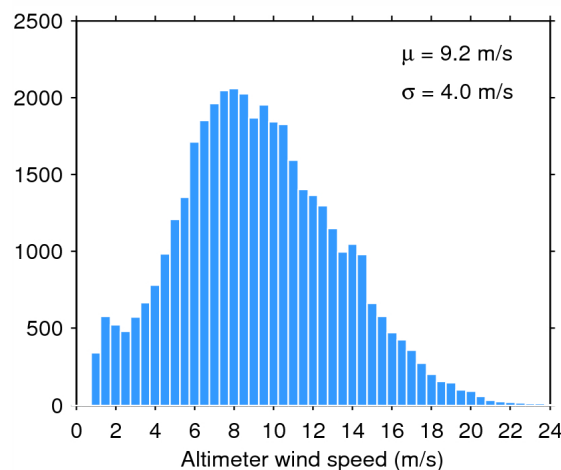
Figure 35. Histogram of science-valid wind over oceans and lakes for 17/11/2014. The mean ( \mu ) and standard deviation ( \sigma ) are also shown. Note that values larger than 24 m/s are excluded from the histogram for the sake of readability but not from the computation of \mu and \sigma .
