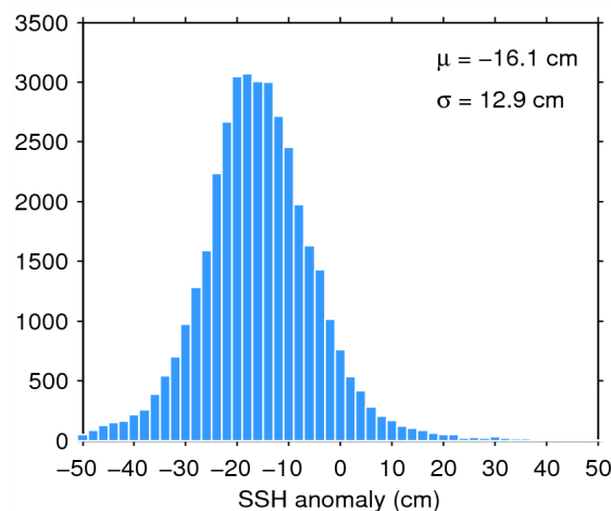
Figure 11. Histogram of science-valid SSH anomaly over oceans and lakes for 17/11/2014. The mean ( \mu ) and standard deviation ( \sigma ) are also shown. Note that values outside [-50 50] cm are excluded from the histogram for the sake of readability but not from the computation of \mu and \sigma .
