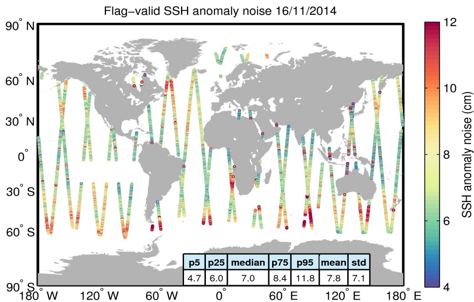
Figure 8. Geographical distribution of flag-valid 20-Hz SSH anomaly measurement noise over oceans and lakes for 16/11/2014. The statistical values shown in the table refer to the SSH anomaly noise and are calculated over all measurements shown in the figure.
