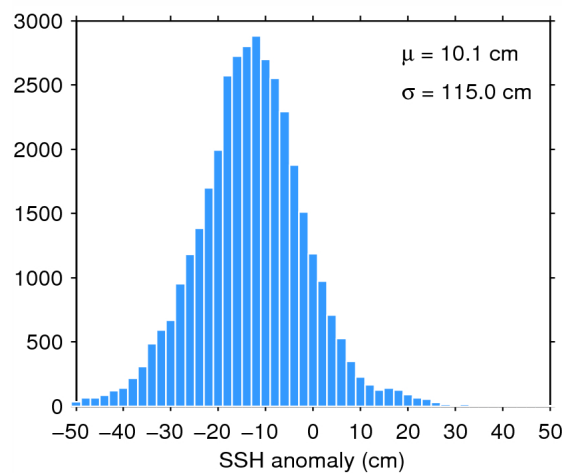
Figure 7. Histogram of flag-valid SSH anomaly over oceans and lakes for 16/11/2014. The mean ( \mu ) and standard deviation ( \sigma ) are also shown. Note that values outside [-50\ 50] cm are excluded from the histogram for the sake of readability but not from the computation of \mu and \sigma .
