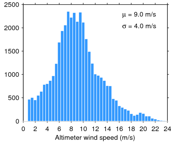
Figure 33. Histogram of flag-valid wind over oceans and lakes for 16/11/2014. The mean ( \mu ) and standard deviation ( \sigma ) are also shown. Note that values larger than 24 m/s are excluded from the histogram for the sake of readability but not from the computation of \mu and \sigma .
