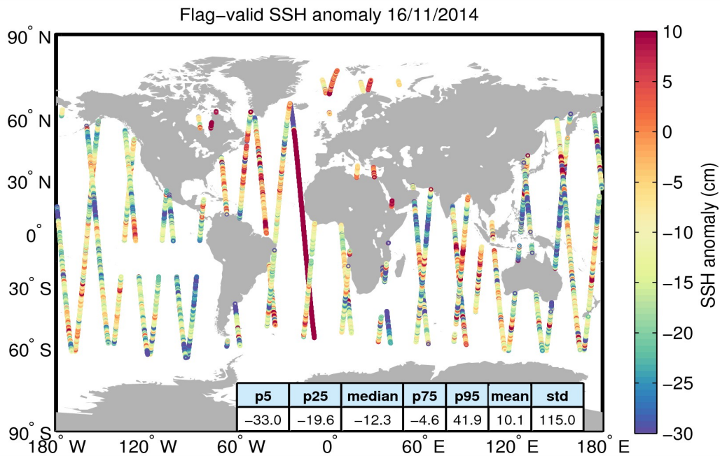
Figure 5. Geographical distribution of flag-valid 1-Hz SSH anomaly data over oceans and lakes for 16/11/2014. The statistical values shown in the table refer to the SSH anomaly in cm and are calculated over all measurements shown in the figure.
