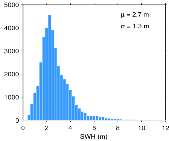
Figure 17. Histogram of flag-valid SWH over oceans and lakes for 16/11/2014. The mean ( \mu ) and standard deviation ( \sigma ) are also shown. Note that values larger than 12 m are excluded from the histogram for the sake of readability but not from the computation of \mu and \sigma .
