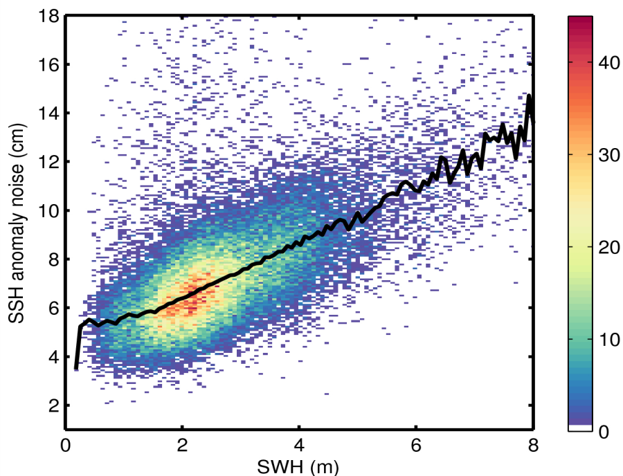
Figure 9. 2D histogram showing flag-valid SSH anomaly noise as a function of SWH for 16/11/2014. The black line denotes the median SSH anomaly as a function of SWH.
