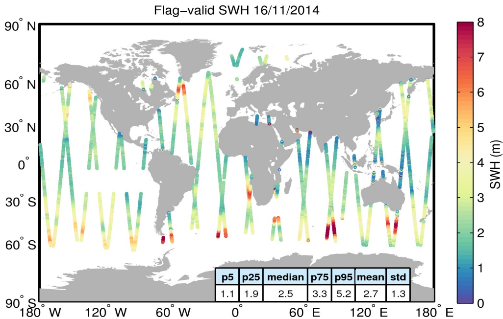
Figure 15. Geographical distribution of flag-valid SWH data over oceans and lakes for 16/11/2014. The statistical values shown in the table refer to the SWH in m and are calculated over all measurements shown in the figure.
