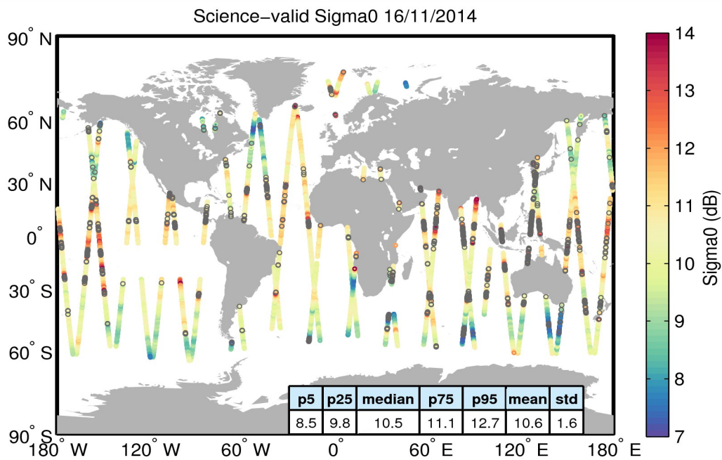
Figure 27. Geographical distribution of science-valid sigma0 data over oceans and lakes for 16/11/2014. The statistical values shown in the table refer to the sigma0 in dB and are calculated over all measurements shown in the figure. Gray circles denote records that have been rejected based on the editing criteria described in Table 4.
