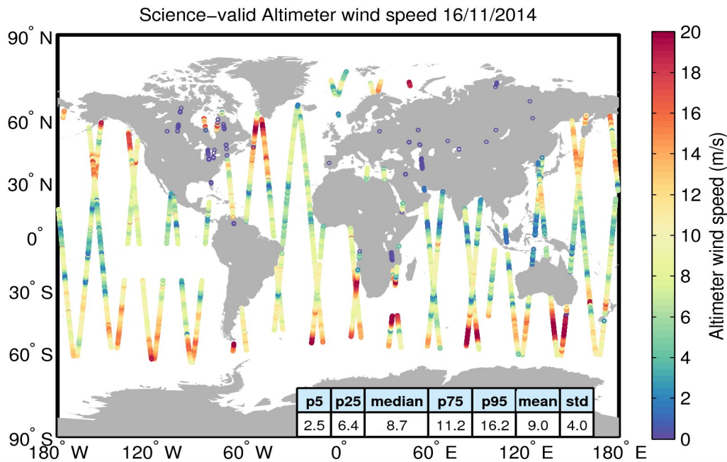
Figure 34. Geographical distribution of science-valid wind data over oceans and lakes for 16/11/2014. The statistical values shown in the table refer to the wind in m/s and are calculated over all measurements shown in the figure. Gray circles denote records that have been rejected based on the editing criteria described in Table 5.
