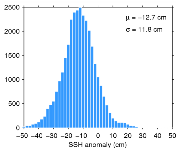
Figure 11. Histogram of science-valid SSH anomaly over oceans and lakes for 16/11/2014. The mean ( \mu ) and standard deviation ( \sigma ) are also shown. Note that values outside [-50 50] cm are excluded from the histogram for the sake of readability but not from the computation of \mu and \sigma .
