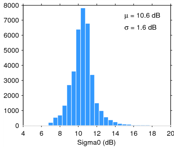
Figure 28. Histogram of science-valid sigma0 over oceans and lakes for 16/11/2014. The mean ( \mu ) and standard deviation ( \sigma ) are also shown. Note that values outside [4 20] dB are excluded from the histogram for the sake of readability but not from the computation of \mu and \sigma .
