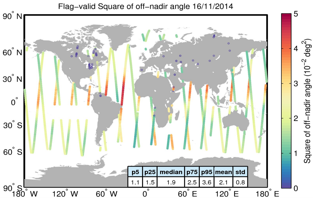
Figure 37. Geographical distribution of flag-valid mispointing data over oceans and lakes for 16/11/2014. The statistical values shown in the table refer to the mispointing in 10^{-2} \text{ deg}^2 and are calculated over all measurements shown in the figure.
