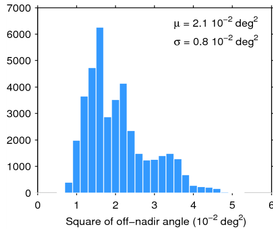
Figure 39. Histogram of flag-valid mispointing over oceans and lakes for 16/11/2014. The mean ( \mu ) and standard deviation ( \sigma ) are also shown. Note that values than 6 \cdot 10^{-2} \text{ deg}^2 are excluded from the histogram for the sake of readability but not from the computation of \mu and \sigma .
