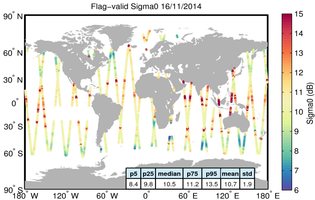
Figure 23. Geographical distribution of flag-valid sigma0 data over oceans and lakes for 16/11/2014. The statistical values shown in the table refer to the sigma0 in dB and are calculated over all measurements shown in the figure.
