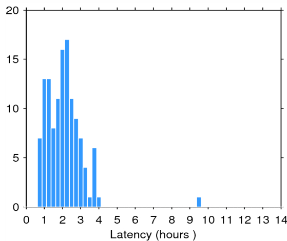
Figure 2. Histogram of the data latency for 16/11/2014. The y-axis denotes the number of files that are made available with a delay of x-hours with respect to the mean time of the records stored in the file.
