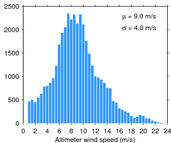
Figure 35. Histogram of science-valid wind over oceans and lakes for 16/11/2014. The mean ( \mu ) and standard deviation ( \sigma ) are also shown. Note that values larger than 24 m/s are excluded from the histogram for the sake of readability but not from the computation of \mu and \sigma .
