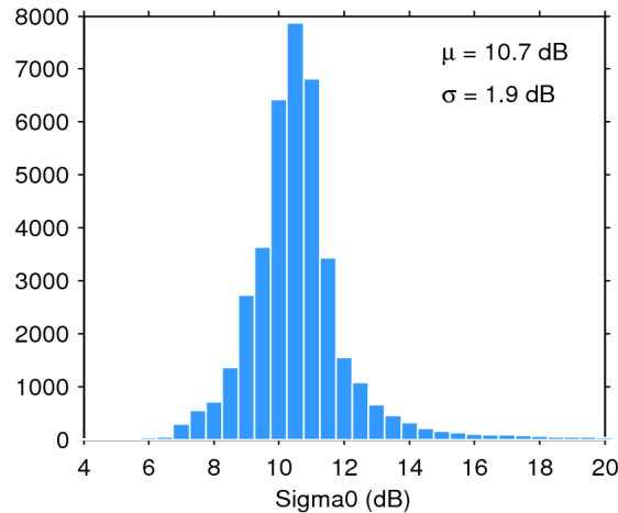
Figure 25. Histogram of flag-valid sigma0 over oceans and lakes for 16/11/2014. The mean ( \mu ) and standard deviation ( \sigma ) are also shown. Note that values outside [4 20] dB are excluded from the histogram for the sake of readability but not from the computation of \mu and \sigma .
