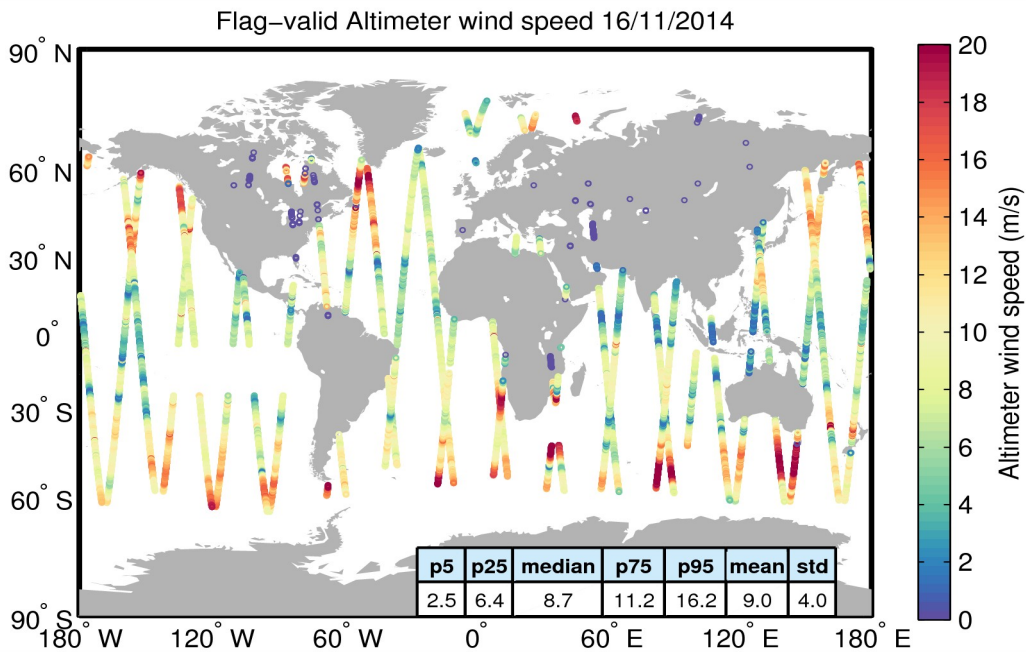
Figure 31. Geographical distribution of flag-valid wind data over oceans and lakes for 16/11/2014. The statistical values shown in the table refer to the wind in m/s and are calculated over all measurements shown in the figure.
