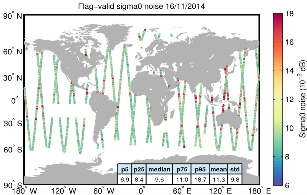
Figure 26. Geographical distribution of flag-valid 20-Hz sigma0 measurement noise over oceans and lakes for 16/11/2014. The statistical values shown in the table refer to the sigma0 noise and are calculated over all measurements shown in the figure.
