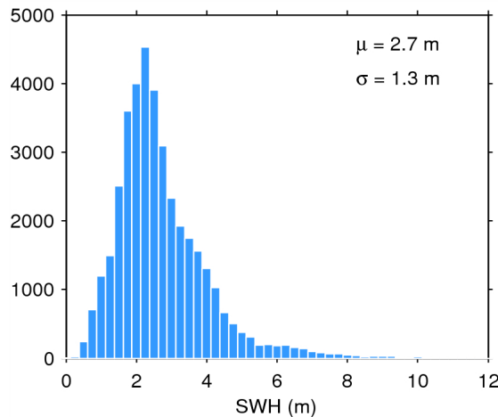
Figure 20. Histogram of science-valid SWH over oceans and lakes for 16/11/2014. The mean ( \mu ) and standard deviation ( \sigma ) are also shown. Note that values larger than 12 m are excluded from the histogram for the sake of readability but not from the computation of \mu and \sigma .
