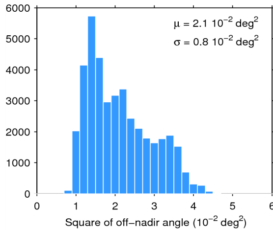
Figure 39. Histogram of flag-valid mispointing over oceans and lakes for 15/11/2014. The mean ( \mu ) and standard deviation ( \sigma ) are also shown. Note that values than 6 \cdot 10^{-2} \text{ deg}^2 are excluded from the histogram for the sake of readability but not from the computation of \mu and \sigma .
