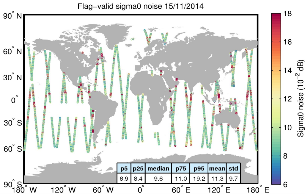
Figure 26. Geographical distribution of flag-valid 20-Hz sigma0 measurement noise over oceans and lakes for 15/11/2014. The statistical values shown in the table refer to the sigma0 noise and are calculated over all measurements shown in the figure.
