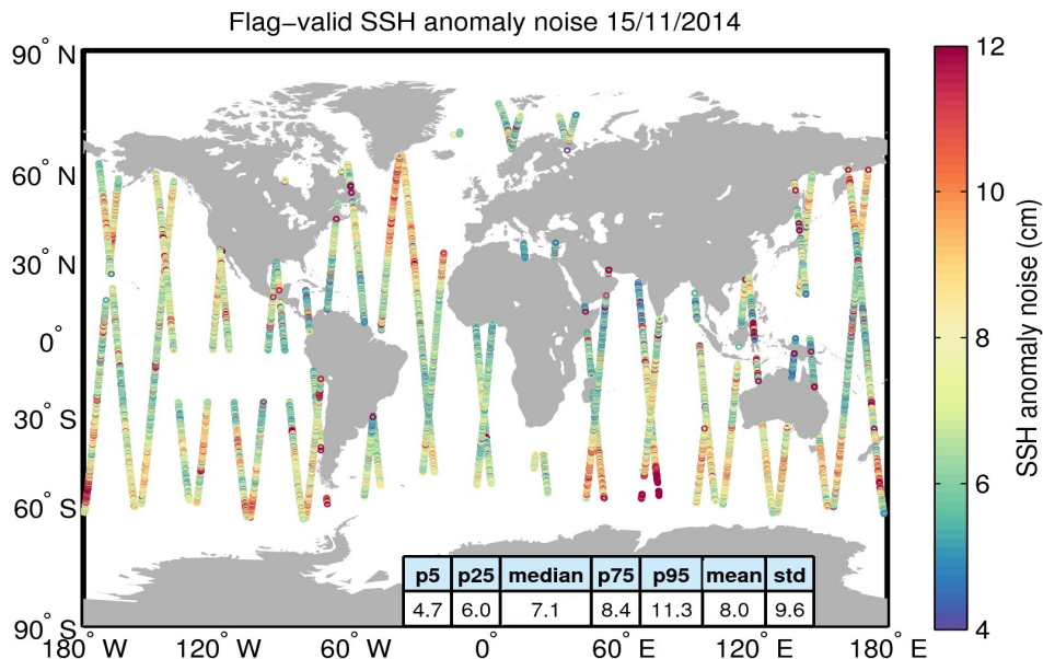
Figure 8. Geographical distribution of flag-valid 20-Hz SSH anomaly measurement noise over oceans and lakes for 15/11/2014. The statistical values shown in the table refer to the SSH anomaly noise and are calculated over all measurements shown in the figure.
