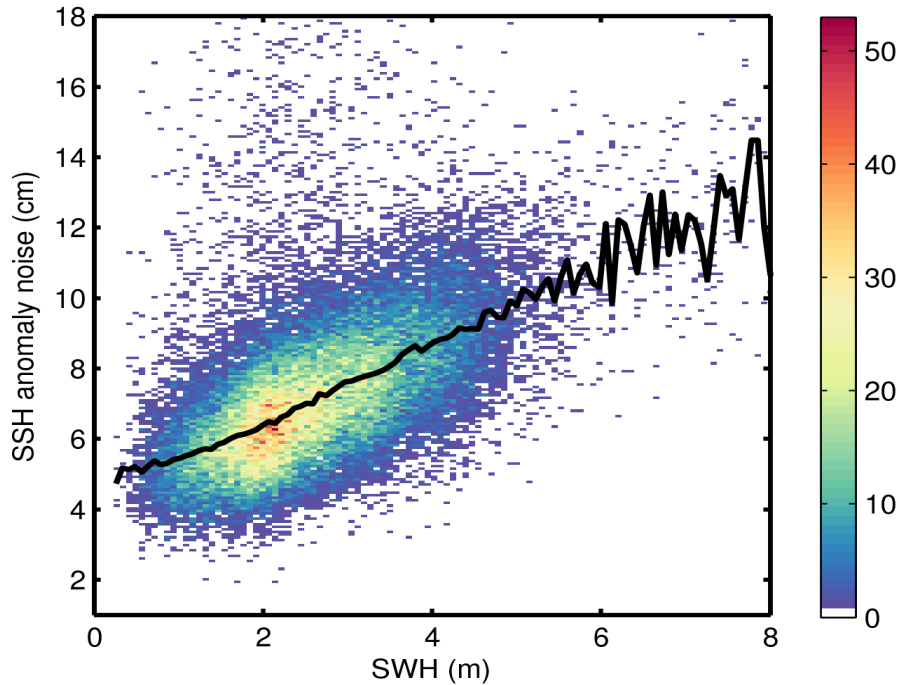
Figure 9. 2D histogram showing flag-valid SSH anomaly noise as a function of SWH for 15/11/2014. The black line denotes the median SSH anomaly as a function of SWH.
