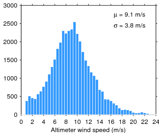
Figure 35. Histogram of science-valid wind over oceans and lakes for 15/11/2014. The mean ( \mu ) and standard deviation ( \sigma ) are also shown. Note that values larger than 24 m/s are excluded from the histogram for the sake of readability but not from the computation of \mu and \sigma .
