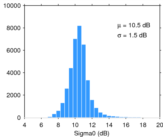
Figure 28. Histogram of science-valid sigma0 over oceans and lakes for 15/11/2014. The mean ( \mu ) and standard deviation ( \sigma ) are also shown. Note that values outside [4 20] dB are excluded from the histogram for the sake of readability but not from the computation of \mu and \sigma .
