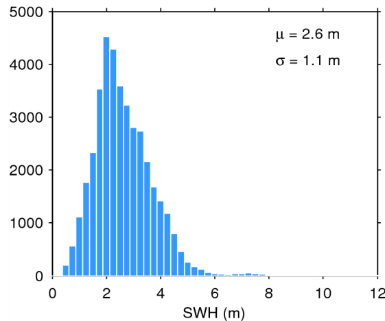
Figure 20. Histogram of science-valid SWH over oceans and lakes for 15/11/2014. The mean ( \mu ) and standard deviation ( \sigma ) are also shown. Note that values larger than 12 m are excluded from the histogram for the sake of readability but not from the computation of \mu and \sigma .
