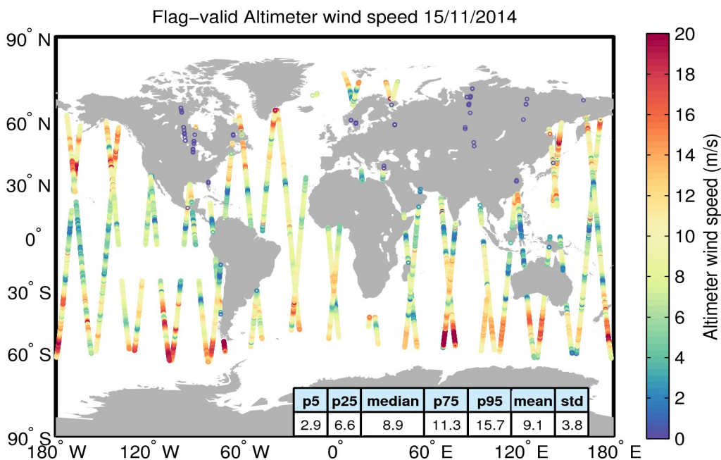
Figure 31. Geographical distribution of flag-valid wind data over oceans and lakes for 15/11/2014. The statistical values shown in the table refer to the wind in m/s and are calculated over all measurements shown in the figure.
