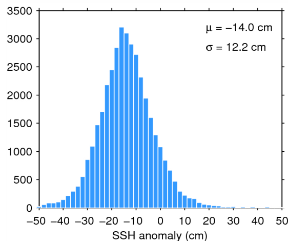
Figure 11. Histogram of science-valid SSH anomaly over oceans and lakes for 15/11/2014. The mean ( \mu ) and standard deviation ( \sigma ) are also shown. Note that values outside [-50 50] cm are excluded from the histogram for the sake of readability but not from the computation of \mu and \sigma .
