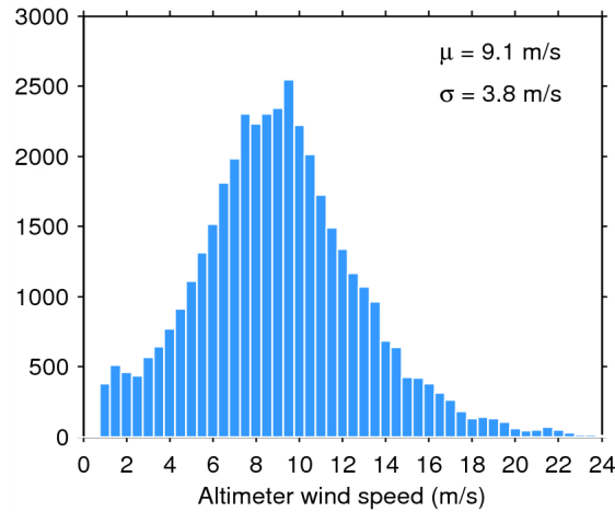
Figure 33. Histogram of flag-valid wind over oceans and lakes for 15/11/2014. The mean ( \mu ) and standard deviation ( \sigma ) are also shown. Note that values larger than 24 m/s are excluded from the histogram for the sake of readability but not from the computation of \mu and \sigma .
