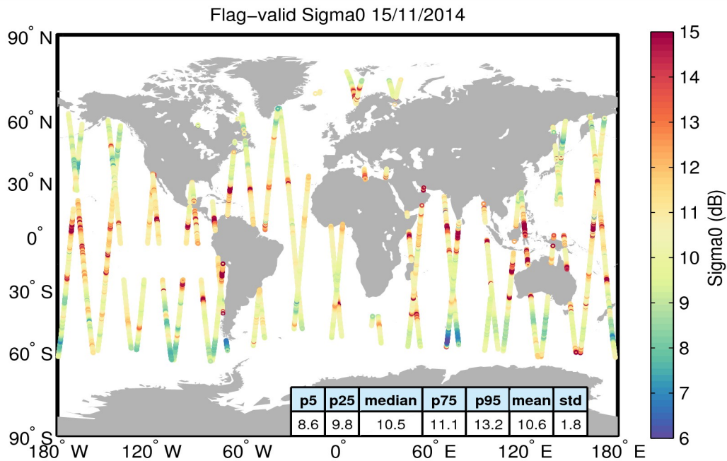
Figure 23. Geographical distribution of flag-valid sigma0 data over oceans and lakes for 15/11/2014. The statistical values shown in the table refer to the sigma0 in dB and are calculated over all measurements shown in the figure.
