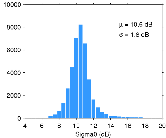
Figure 25. Histogram of flag-valid sigma0 over oceans and lakes for 15/11/2014. The mean ( \mu ) and standard deviation ( \sigma ) are also shown. Note that values outside [4 20] dB are excluded from the histogram for the sake of readability but not from the computation of \mu and \sigma .
