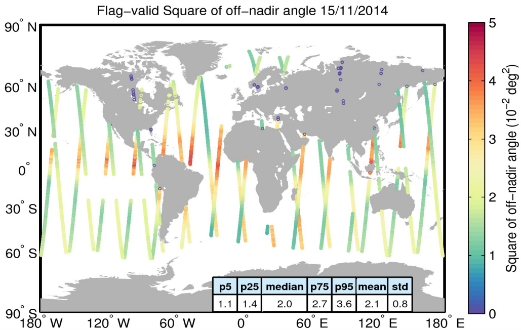
Figure 37. Geographical distribution of flag-valid mispointing data over oceans and lakes for 15/11/2014. The statistical values shown in the table refer to the mispointing in 10^{-2} \text{ deg}^2 and are calculated over all measurements shown in the figure.
