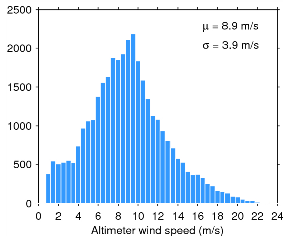
Figure 35. Histogram of science-valid wind over oceans and lakes for 14/11/2014. The mean ( \mu ) and standard deviation ( \sigma ) are also shown. Note that values larger than 24 m/s are excluded from the histogram for the sake of readability but not from the computation of \mu and \sigma .
