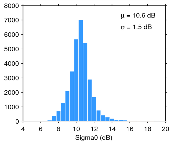
Figure 28. Histogram of science-valid sigma0 over oceans and lakes for 14/11/2014. The mean ( \mu ) and standard deviation ( \sigma ) are also shown. Note that values outside [4 20] dB are excluded from the histogram for the sake of readability but not from the computation of \mu and \sigma .
