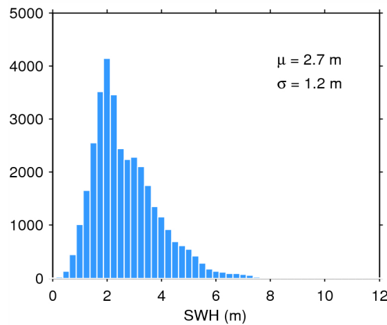
Figure 17. Histogram of flag-valid SWH over oceans and lakes for 14/11/2014. The mean ( \mu ) and standard deviation ( \sigma ) are also shown. Note that values larger than 12 m are excluded from the histogram for the sake of readability but not from the computation of \mu and \sigma .
