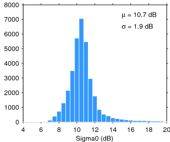
Figure 25. Histogram of flag-valid sigma0 over oceans and lakes for 14/11/2014. The mean ( \mu ) and standard deviation ( \sigma ) are also shown. Note that values outside [4 20] dB are excluded from the histogram for the sake of readability but not from the computation of \mu and \sigma .
