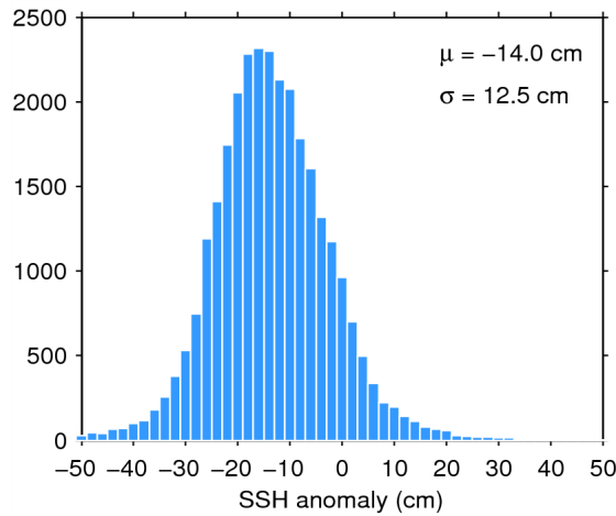
Figure 11. Histogram of science-valid SSH anomaly over oceans and lakes for 14/11/2014. The mean ( \mu ) and standard deviation ( \sigma ) are also shown. Note that values outside [-50 50] cm are excluded from the histogram for the sake of readability but not from the computation of \mu and \sigma .
