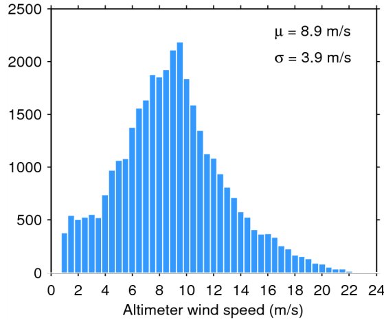
Figure 33. Histogram of flag-valid wind over oceans and lakes for 14/11/2014. The mean ( \mu ) and standard deviation ( \sigma ) are also shown. Note that values larger than 24 m/s are excluded from the histogram for the sake of readability but not from the computation of \mu and \sigma .
