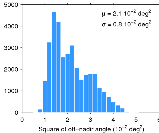
Figure 39. Histogram of flag-valid mispointing over oceans and lakes for 14/11/2014. The mean ( \mu ) and standard deviation ( \sigma ) are also shown. Note that values than 6 \cdot 10^{-2} \text{ deg}^2 are excluded from the histogram for the sake of readability but not from the computation of \mu and \sigma .
