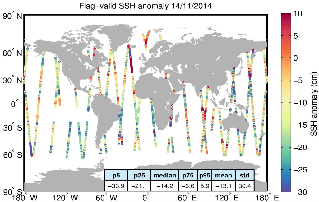
Figure 5. Geographical distribution of flag-valid 1-Hz SSH anomaly data over oceans and lakes for 14/11/2014. The statistical values shown in the table refer to the SSH anomaly in cm and are calculated over all measurements shown in the figure.
