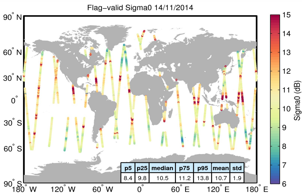
Figure 23. Geographical distribution of flag-valid sigma0 data over oceans and lakes for 14/11/2014. The statistical values shown in the table refer to the sigma0 in dB and are calculated over all measurements shown in the figure.
