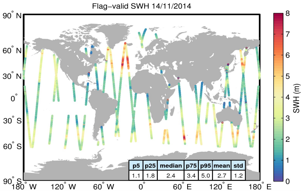
Figure 15. Geographical distribution of flag-valid SWH data over oceans and lakes for 14/11/2014. The statistical values shown in the table refer to the SWH in m and are calculated over all measurements shown in the figure.
