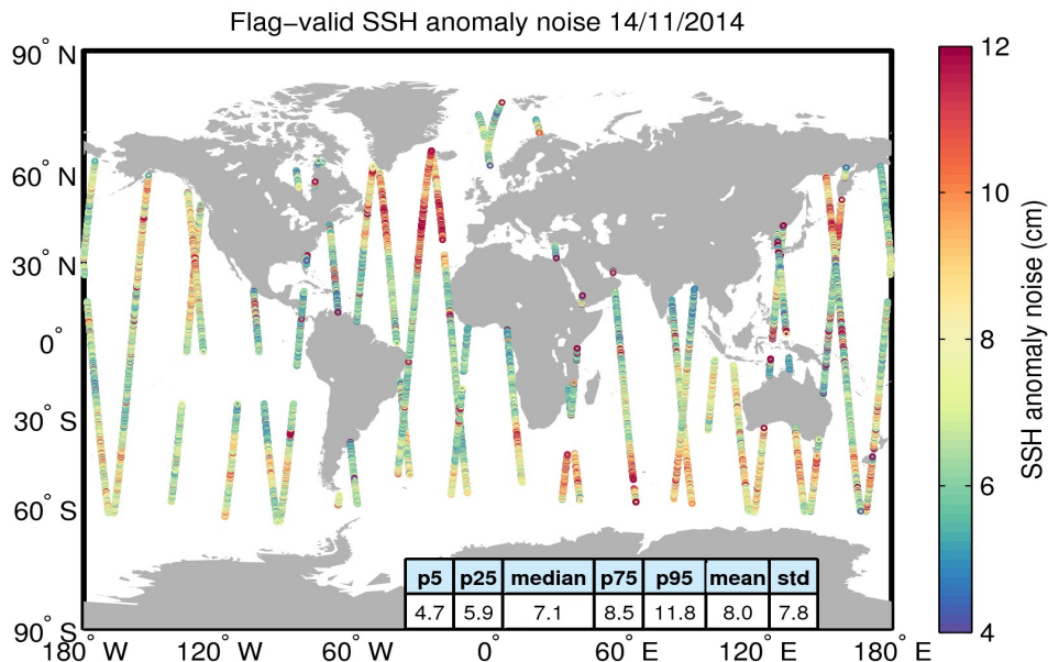
Figure 8. Geographical distribution of flag-valid 20-Hz SSH anomaly measurement noise over oceans and lakes for 14/11/2014. The statistical values shown in the table refer to the SSH anomaly noise and are calculated over all measurements shown in the figure.
