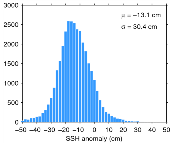
Figure 7. Histogram of flag-valid SSH anomaly over oceans and lakes for 14/11/2014. The mean ( \mu ) and standard deviation ( \sigma ) are also shown. Note that values outside [-50 50] cm are excluded from the histogram for the sake of readability but not from the computation of \mu and \sigma .
