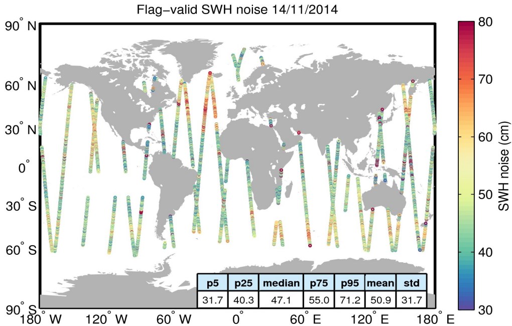
Figure 18. Geographical distribution of flag-valid 20-Hz SWH measurement noise over oceans and lakes for 14/11/2014. The statistical values shown in the figure refer to the SWH noise and are calculated over all measurements shown in the figure.
