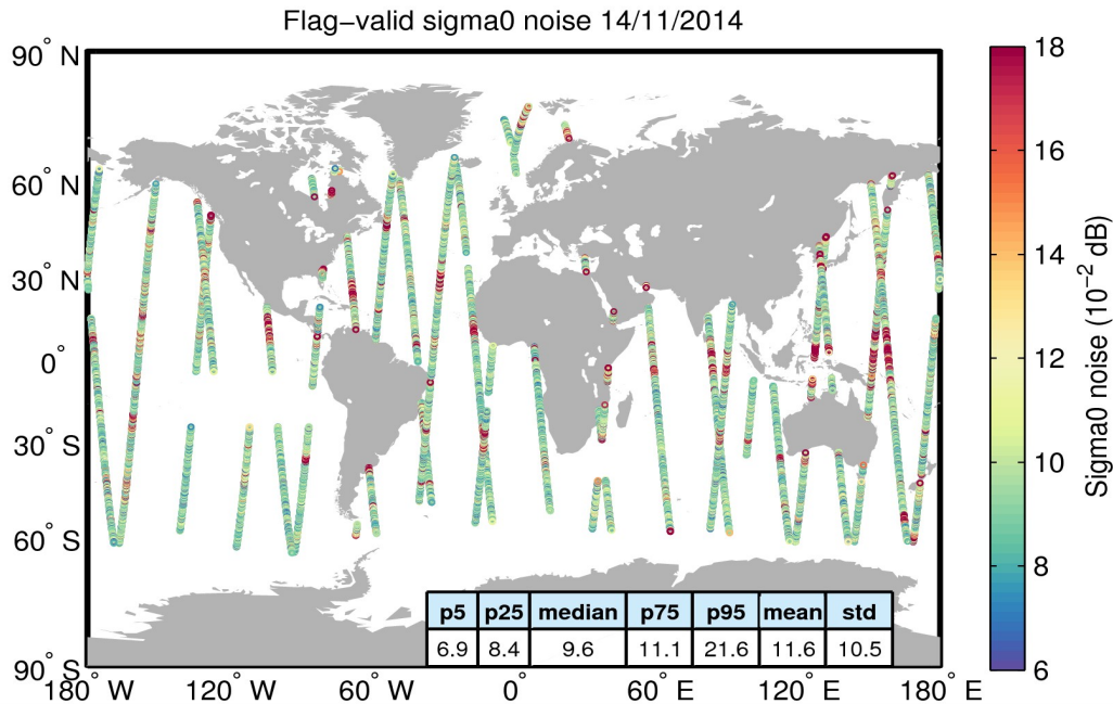
Figure 26. Geographical distribution of flag-valid 20-Hz sigma0 measurement noise over oceans and lakes for 14/11/2014. The statistical values shown in the table refer to the sigma0 noise and are calculated over all measurements shown in the figure.
