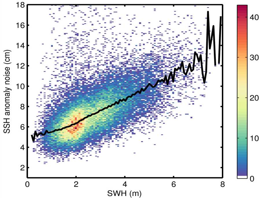
Figure 9. 2D histogram showing flag-valid SSH anomaly noise as a function of SWH for 14/11/2014. The black line denotes the median SSH anomaly as a function of SWH.
