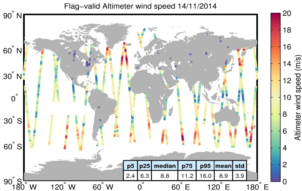
Figure 31. Geographical distribution of flag-valid wind data over oceans and lakes for 14/11/2014. The statistical values shown in the table refer to the wind in m/s and are calculated over all measurements shown in the figure.
