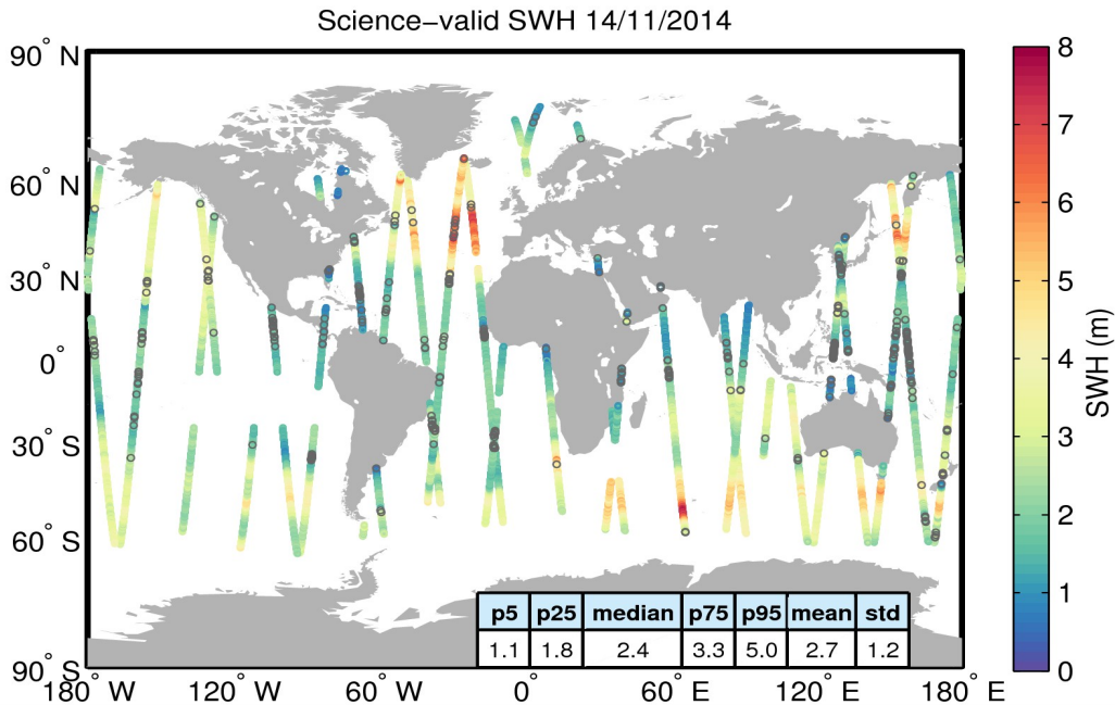
Figure 19. Geographical distribution of science-valid SWH data over oceans and lakes for 14/11/2014. The statistical values shown in the table refer to the SWH in m and are calculated over all measurements shown in the figure. Gray circles denote records that have been rejected based on the editing criteria described in Table 3.
