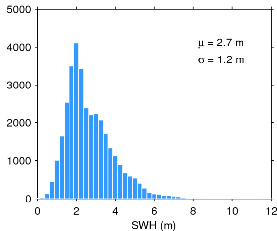
Figure 20. Histogram of science-valid SWH over oceans and lakes for 14/11/2014. The mean ( \mu ) and standard deviation ( \sigma ) are also shown. Note that values larger than 12 m are excluded from the histogram for the sake of readability but not from the computation of \mu and \sigma .
