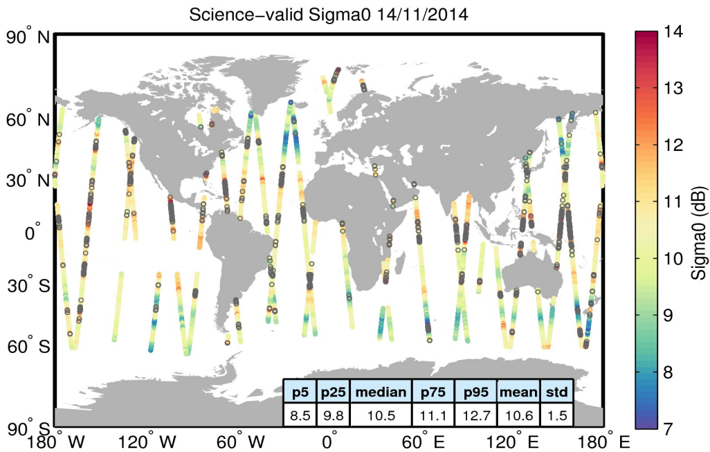
Figure 27. Geographical distribution of science-valid sigma0 data over oceans and lakes for 14/11/2014. The statistical values shown in the table refer to the sigma0 in dB and are calculated over all measurements shown in the figure. Gray circles denote records that have been rejected based on the editing criteria described in Table 4.
