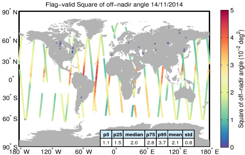
Figure 37. Geographical distribution of flag-valid mispointing data over oceans and lakes for 14/11/2014. The statistical values shown in the table refer to the mispointing in 10^{-2} \text{deg}^2 and are calculated over all measurements shown in the figure.
