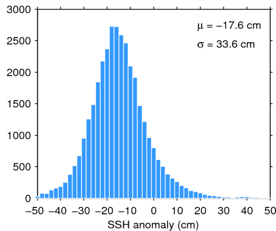
Figure 7. Histogram of flag-valid SSH anomaly over oceans and lakes for 12/11/2014. The mean ( \mu ) and standard deviation ( \sigma ) are also shown. Note that values outside [-50\ 50] cm are excluded from the histogram for the sake of readability but not from the computation of \mu and \sigma .
