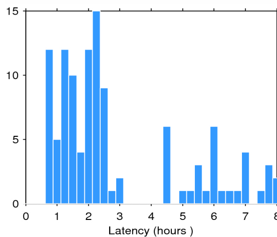
Figure 2. Histogram of the data latency for 12/11/2014. The y-axis denotes the number of files that are made available with a delay of x-hours with respect to the mean time of the records stored in the file.
