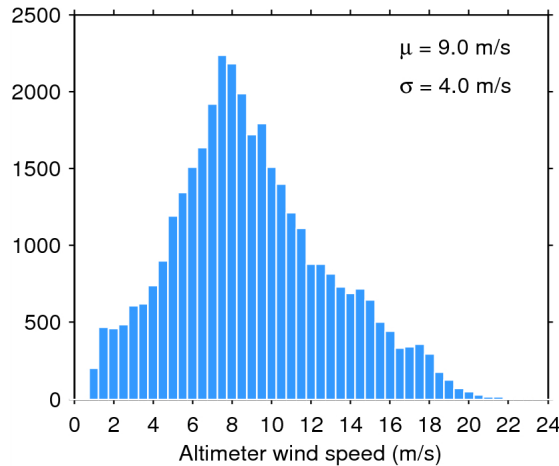
Figure 33. Histogram of flag-valid wind over oceans and lakes for 12/11/2014. The mean ( \mu ) and standard deviation ( \sigma ) are also shown. Note that values larger than 24 m/s are excluded from the histogram for the sake of readability but not from the computation of \mu and \sigma .
