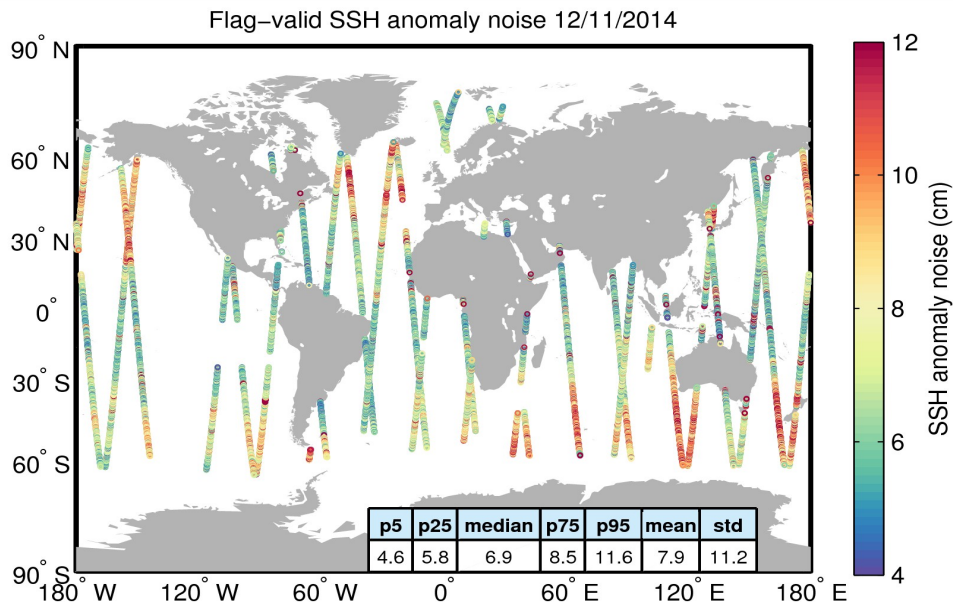
Figure 8. Geographical distribution of flag-valid 20-Hz SSH anomaly measurement noise over oceans and lakes for 12/11/2014. The statistical values shown in the table refer to the SSH anomaly noise and are calculated over all measurements shown in the figure.
