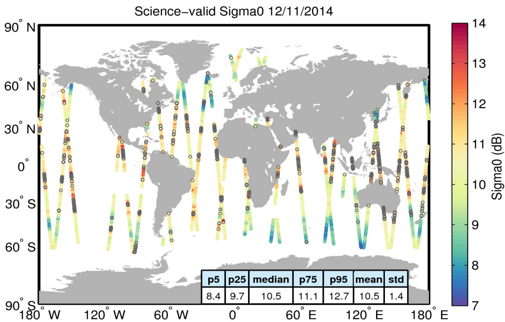
Figure 27. Geographical distribution of science-valid sigma0 data over oceans and lakes for 12/11/2014. The statistical values shown in the table refer to the sigma0 in dB and are calculated over all measurements shown in the figure. Gray circles denote records that have been rejected based on the editing criteria described in Table 4.
