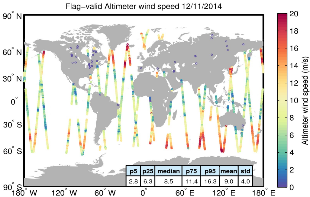
Figure 31. Geographical distribution of flag-valid wind data over oceans and lakes for 12/11/2014. The statistical values shown in the table refer to the wind in m/s and are calculated over all measurements shown in the figure.
