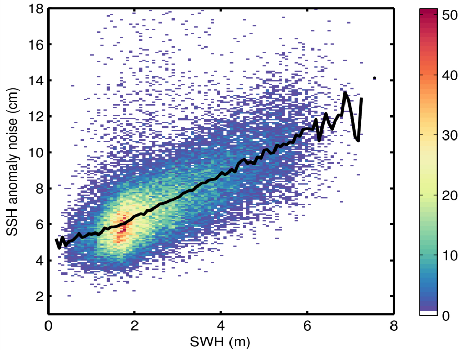
Figure 9. 2D histogram showing flag-valid SSH anomaly noise as a function of SWH for 12/11/2014. The black line denotes the median SSH anomaly as a function of SWH.
