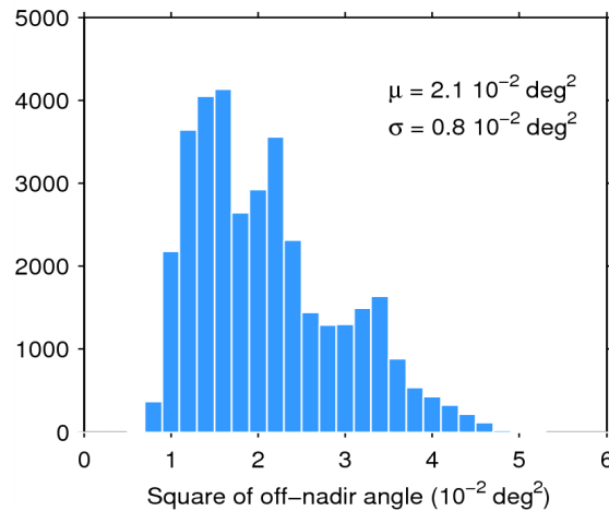
Figure 39. Histogram of flag-valid mispointing over oceans and lakes for 12/11/2014. The mean ( \mu ) and standard deviation ( \sigma ) are also shown. Note that values than 6 \cdot 10^{-2} \text{ deg}^2 are excluded from the histogram for the sake of readability but not from the computation of \mu and \sigma .
