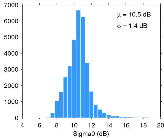
Figure 28. Histogram of science-valid sigma0 over oceans and lakes for 12/11/2014. The mean ( \mu ) and standard deviation ( \sigma ) are also shown. Note that values outside [4 20] dB are excluded from the histogram for the sake of readability but not from the computation of \mu and \sigma .
