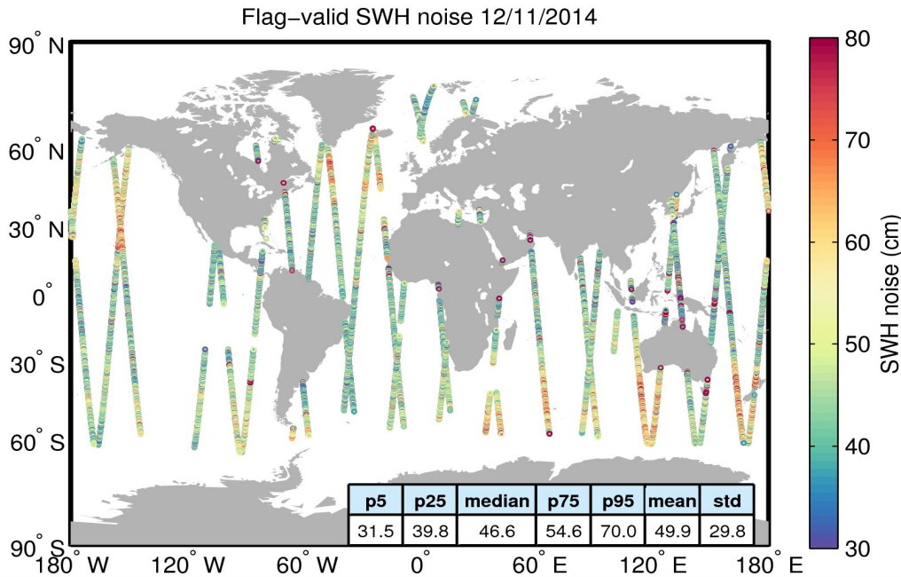
Figure 18. Geographical distribution of flag-valid 20-Hz SWH measurement noise over oceans and lakes for 12/11/2014. The statistical values shown in the figure refer to the SWH noise and are calculated over all measurements shown in the figure.
