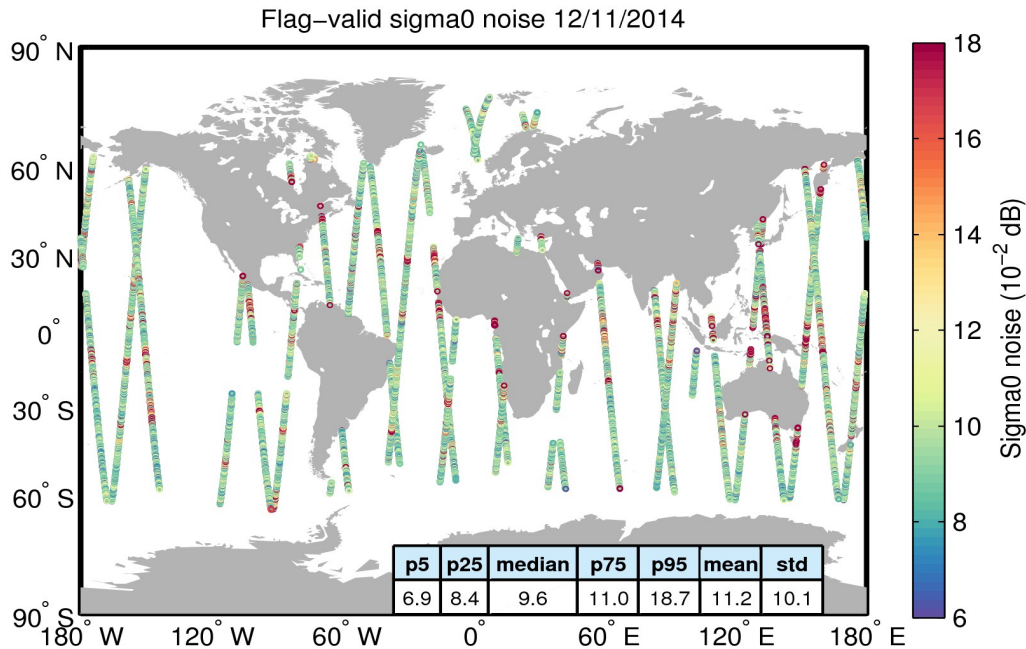
Figure 26. Geographical distribution of flag-valid 20-Hz sigma0 measurement noise over oceans and lakes for 12/11/2014. The statistical values shown in the table refer to the sigma0 noise and are calculated over all measurements shown in the figure.
