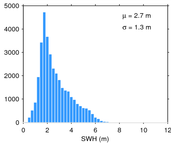
Figure 17. Histogram of flag-valid SWH over oceans and lakes for 12/11/2014. The mean ( \mu ) and standard deviation ( \sigma ) are also shown. Note that values larger than 12 m are excluded from the histogram for the sake of readability but not from the computation of \mu and \sigma .
