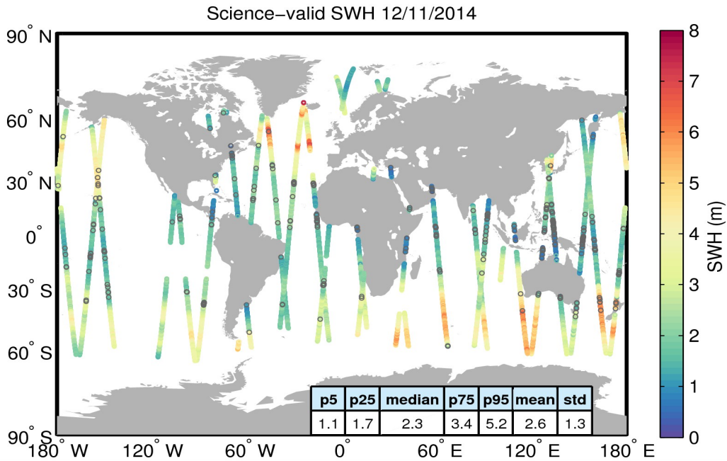
Figure 19. Geographical distribution of science-valid SWH data over oceans and lakes for 12/11/2014. The statistical values shown in the table refer to the SWH in m and are calculated over all measurements shown in the figure. Gray circles denote records that have been rejected based on the editing criteria described in Table 3.
