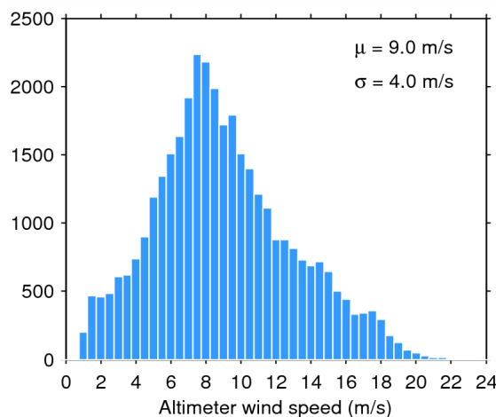
Figure 35. Histogram of science-valid wind over oceans and lakes for 12/11/2014. The mean ( \mu ) and standard deviation ( \sigma ) are also shown. Note that values larger than 24 m/s are excluded from the histogram for the sake of readability but not from the computation of \mu and \sigma .
