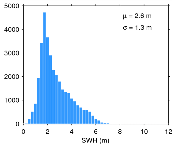
Figure 20. Histogram of science-valid SWH over oceans and lakes for 12/11/2014. The mean ( \mu ) and standard deviation ( \sigma ) are also shown. Note that values larger than 12 m are excluded from the histogram for the sake of readability but not from the computation of \mu and \sigma .
