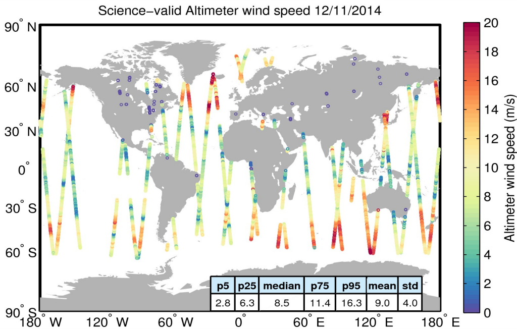
Figure 34. Geographical distribution of science-valid wind data over oceans and lakes for 12/11/2014. The statistical values shown in the table refer to the wind in m/s and are calculated over all measurements shown in the figure. Gray circles denote records that have been rejected based on the editing criteria described in Table 5.
