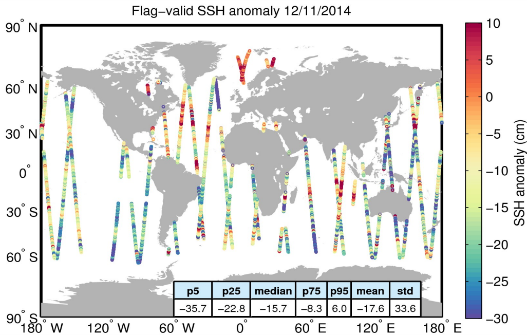
Figure 5. Geographical distribution of flag-valid 1-Hz SSH anomaly data over oceans and lakes for 12/11/2014. The statistical values shown in the table refer to the SSH anomaly in cm and are calculated over all measurements shown in the figure.
