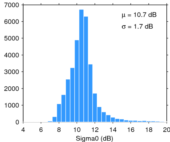
Figure 25. Histogram of flag-valid sigma0 over oceans and lakes for 12/11/2014. The mean ( \mu ) and standard deviation ( \sigma ) are also shown. Note that values outside [4 20] dB are excluded from the histogram for the sake of readability but not from the computation of \mu and \sigma .
