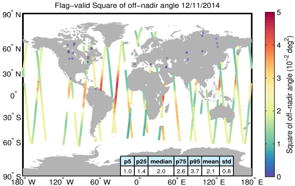
Figure 37. Geographical distribution of flag-valid mispointing data over oceans and lakes for 12/11/2014. The statistical values shown in the table refer to the mispointing in 10^{-2} deg 2 and are calculated over all measurements shown in the figure.
