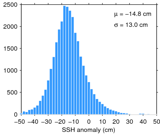
Figure 11. Histogram of science-valid SSH anomaly over oceans and lakes for 12/11/2014. The mean ( \mu ) and standard deviation ( \sigma ) are also shown. Note that values outside [-50 50] cm are excluded from the histogram for the sake of readability but not from the computation of \mu and \sigma .
