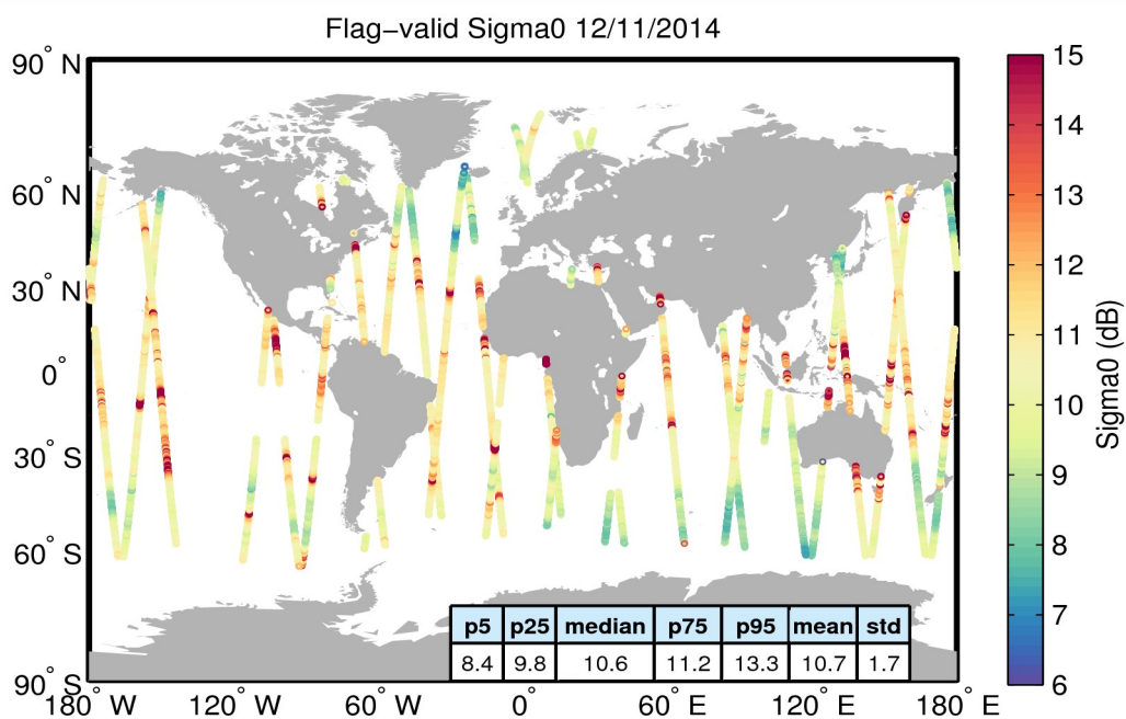
Figure 23. Geographical distribution of flag-valid sigma0 data over oceans and lakes for 12/11/2014. The statistical values shown in the table refer to the sigma0 in dB and are calculated over all measurements shown in the figure.
