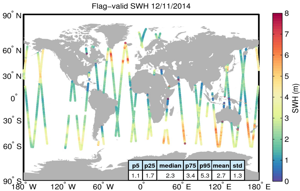
Figure 15. Geographical distribution of flag-valid SWH data over oceans and lakes for 12/11/2014. The statistical values shown in the table refer to the SWH in m and are calculated over all measurements shown in the figure.
