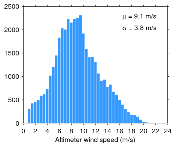
Figure 35. Histogram of science-valid wind over oceans and lakes for 11/11/2014. The mean ( \mu ) and standard deviation ( \sigma ) are also shown. Note that values larger than 24 m/s are excluded from the histogram for the sake of readability but not from the computation of \mu and \sigma .
