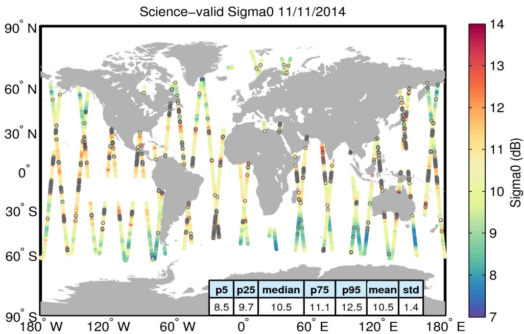
Figure 27. Geographical distribution of science-valid sigma0 data over oceans and lakes for 11/11/2014. The statistical values shown in the table refer to the sigma0 in dB and are calculated over all measurements shown in the figure. Gray circles denote records that have been rejected based on the editing criteria described in Table 4.
