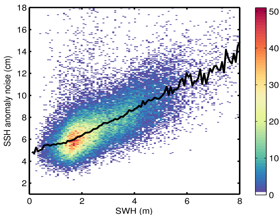
Figure 9. 2D histogram showing flag-valid SSH anomaly noise as a function of SWH for 11/11/2014. The black line denotes the median SSH anomaly as a function of SWH.
