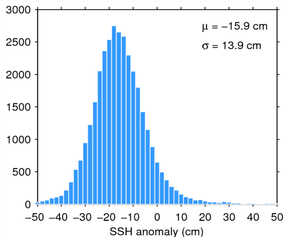
Figure 11. Histogram of science-valid SSH anomaly over oceans and lakes for 11/11/2014. The mean ( \mu ) and standard deviation ( \sigma ) are also shown. Note that values outside [-50 50] cm are excluded from the histogram for the sake of readability but not from the computation of \mu and \sigma .
