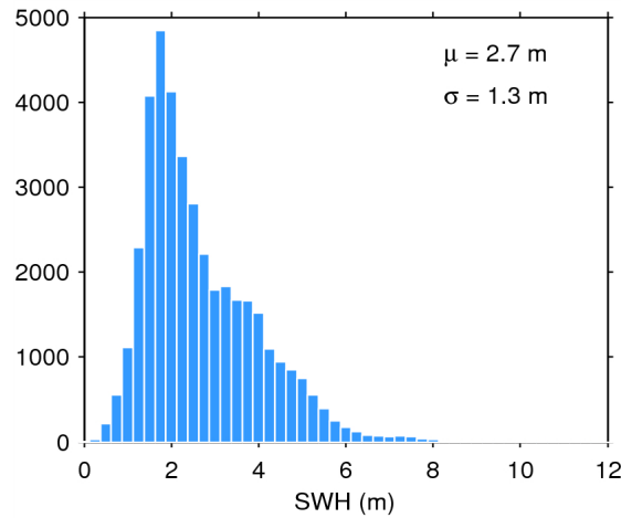
Figure 17. Histogram of flag-valid SWH over oceans and lakes for 11/11/2014. The mean ( \mu ) and standard deviation ( \sigma ) are also shown. Note that values larger than 12 m are excluded from the histogram for the sake of readability but not from the computation of \mu and \sigma .
