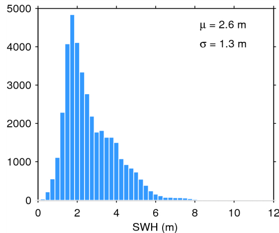
Figure 20. Histogram of science-valid SWH over oceans and lakes for 11/11/2014. The mean ( \mu ) and standard deviation ( \sigma ) are also shown. Note that values larger than 12 m are excluded from the histogram for the sake of readability but not from the computation of \mu and \sigma .
