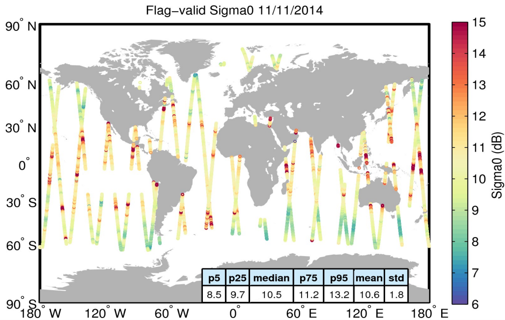
Figure 23. Geographical distribution of flag-valid sigma0 data over oceans and lakes for 11/11/2014. The statistical values shown in the table refer to the sigma0 in dB and are calculated over all measurements shown in the figure.
