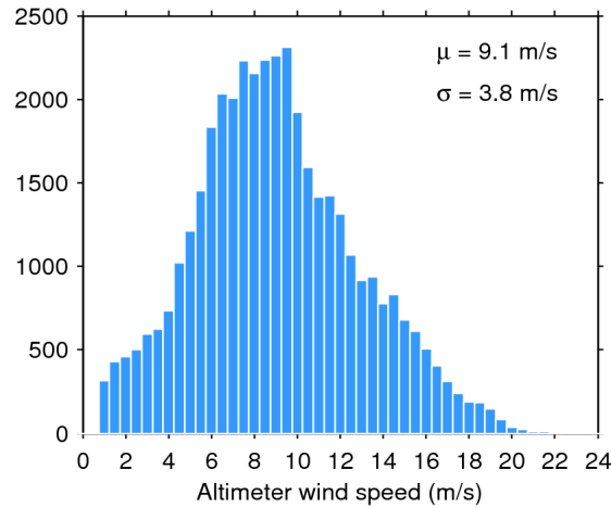
Figure 33. Histogram of flag-valid wind over oceans and lakes for 11/11/2014. The mean ( \mu ) and standard deviation ( \sigma ) are also shown. Note that values larger than 24 m/s are excluded from the histogram for the sake of readability but not from the computation of \mu and \sigma .
