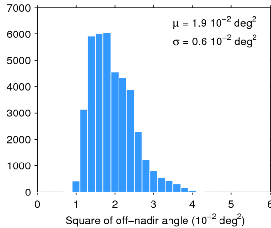
Figure 39. Histogram of flag-valid mispointing over oceans and lakes for 11/11/2014. The mean ( \mu ) and standard deviation ( \sigma ) are also shown. Note that values than 6 \cdot 10^{-2} \text{ deg}^2 are excluded from the histogram for the sake of readability but not from the computation of \mu and \sigma .
