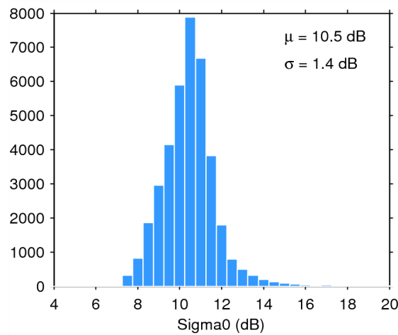
Figure 28. Histogram of science-valid sigma0 over oceans and lakes for 11/11/2014. The mean ( \mu ) and standard deviation ( \sigma ) are also shown. Note that values outside [4 20] dB are excluded from the histogram for the sake of readability but not from the computation of \mu and \sigma .
