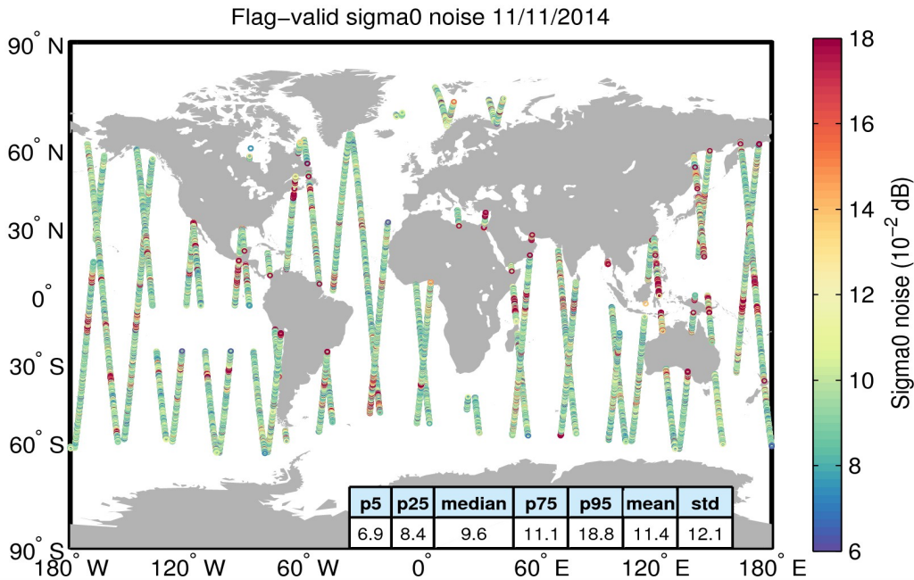
Figure 26. Geographical distribution of flag-valid 20-Hz sigma0 measurement noise over oceans and lakes for 11/11/2014. The statistical values shown in the table refer to the sigma0 noise and are calculated over all measurements shown in the figure.
