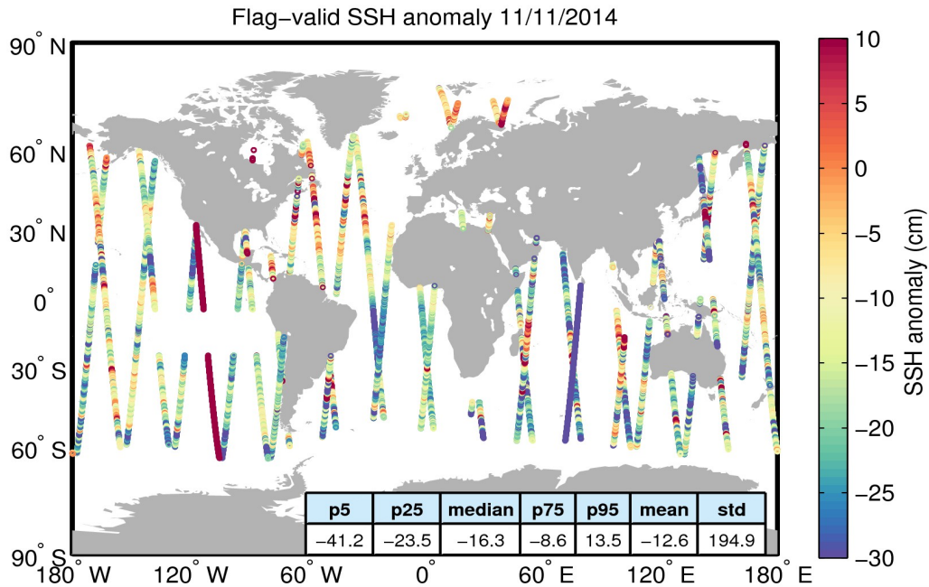
Figure 5. Geographical distribution of flag-valid 1-Hz SSH anomaly data over oceans and lakes for 11/11/2014. The statistical values shown in the table refer to the SSH anomaly in cm and are calculated over all measurements shown in the figure.
