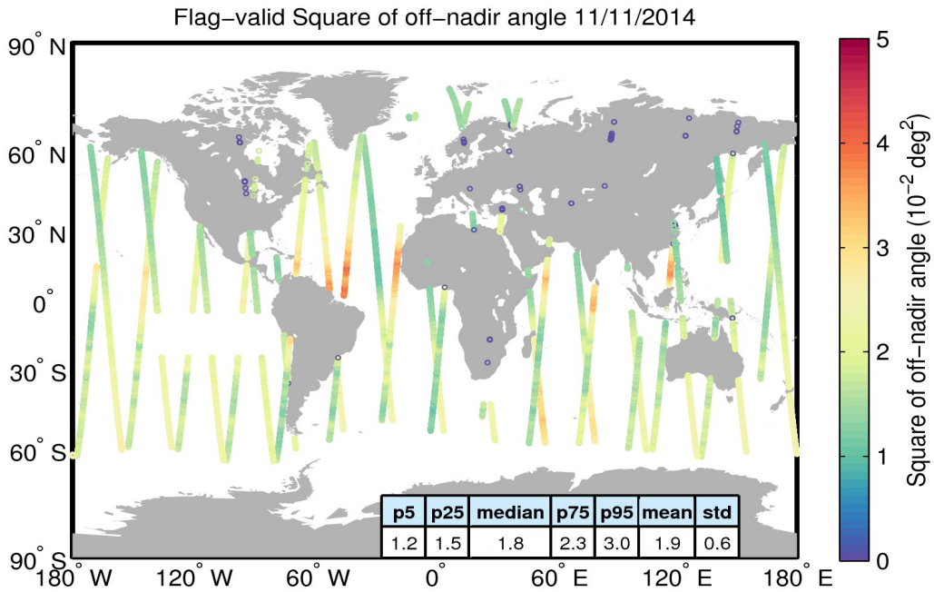
Figure 37. Geographical distribution of flag-valid mispointing data over oceans and lakes for 11/11/2014. The statistical values shown in the table refer to the mispointing in 10^{-2} \text{deg}^2 and are calculated over all measurements shown in the figure.
