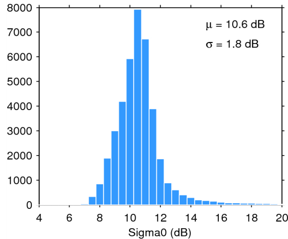
Figure 25. Histogram of flag-valid sigma0 over oceans and lakes for 11/11/2014. The mean ( \mu ) and standard deviation ( \sigma ) are also shown. Note that values outside [4 20] dB are excluded from the histogram for the sake of readability but not from the computation of \mu and \sigma .
