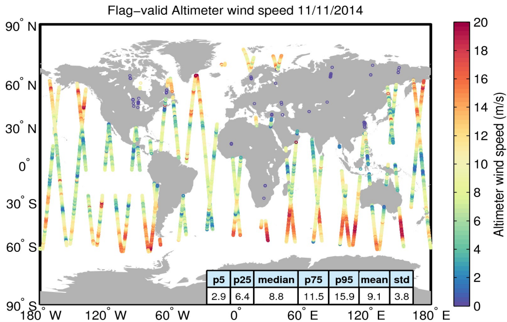
Figure 31. Geographical distribution of flag-valid wind data over oceans and lakes for 11/11/2014. The statistical values shown in the table refer to the wind in m/s and are calculated over all measurements shown in the figure.
