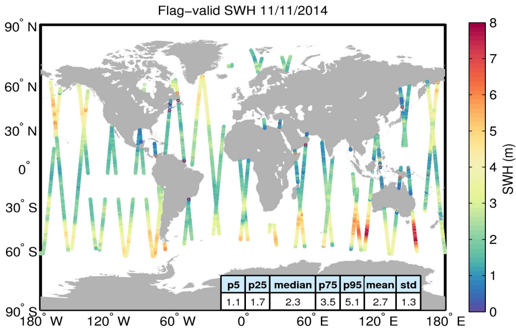
Figure 15. Geographical distribution of flag-valid SWH data over oceans and lakes for 11/11/2014. The statistical values shown in the table refer to the SWH in m and are calculated over all measurements shown in the figure.
