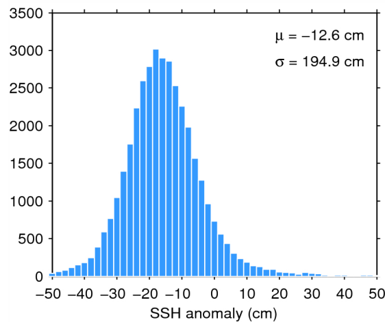
Figure 7. Histogram of flag-valid SSH anomaly over oceans and lakes for 11/11/2014. The mean ( \mu ) and standard deviation ( \sigma ) are also shown. Note that values outside [-50 50] cm are excluded from the histogram for the sake of readability but not from the computation of \mu and \sigma .
