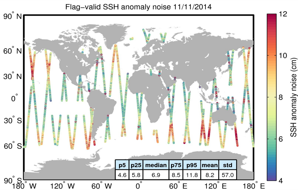
Figure 8. Geographical distribution of flag-valid 20-Hz SSH anomaly measurement noise over oceans and lakes for 11/11/2014. The statistical values shown in the table refer to the SSH anomaly noise and are calculated over all measurements shown in the figure.
