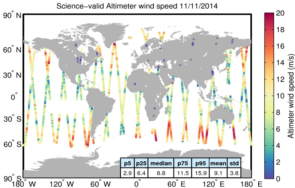
Figure 34. Geographical distribution of science-valid wind data over oceans and lakes for 11/11/2014. The statistical values shown in the table refer to the wind in m/s and are calculated over all measurements shown in the figure. Gray circles denote records that have been rejected based on the editing criteria described in Table 5.
