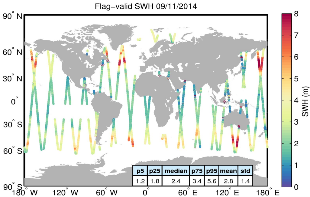
Figure 15. Geographical distribution of flag-valid SWH data over oceans and lakes for 09/11/2014. The statistical values shown in the table refer to the SWH in m and are calculated over all measurements shown in the figure.
