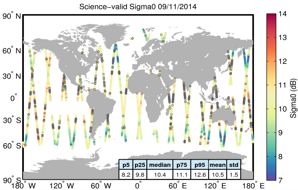
Figure 27. Geographical distribution of science-valid sigma0 data over oceans and lakes for 09/11/2014. The statistical values shown in the table refer to the sigma0 in dB and are calculated over all measurements shown in the figure. Gray circles denote records that have been rejected based on the editing criteria described in Table 4.
