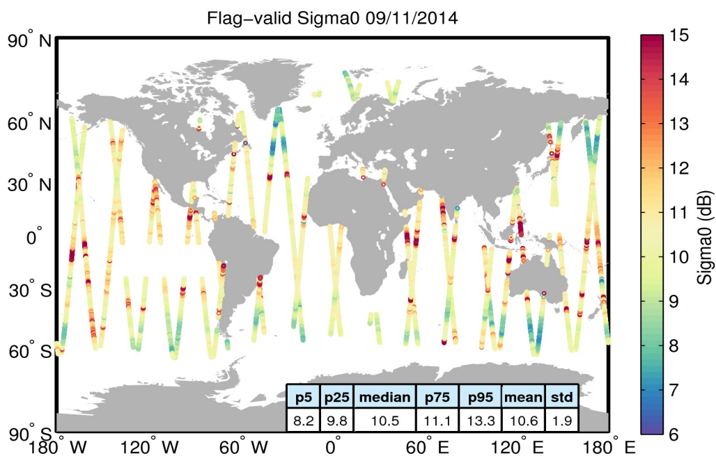
Figure 23. Geographical distribution of flag-valid sigma0 data over oceans and lakes for 09/11/2014. The statistical values shown in the table refer to the sigma0 in dB and are calculated over all measurements shown in the figure.
