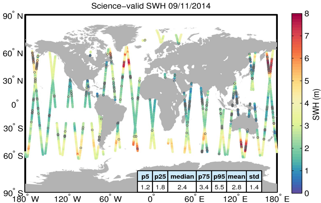
Figure 19. Geographical distribution of science-valid SWH data over oceans and lakes for 09/11/2014. The statistical values shown in the table refer to the SWH in m and are calculated over all measurements shown in the figure. Gray circles denote records that have been rejected based on the editing criteria described in Table 3.
