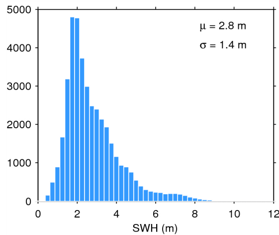
Figure 17. Histogram of flag-valid SWH over oceans and lakes for 09/11/2014. The mean ( \mu ) and standard deviation ( \sigma ) are also shown. Note that values larger than 12 m are excluded from the histogram for the sake of readability but not from the computation of \mu and \sigma .
