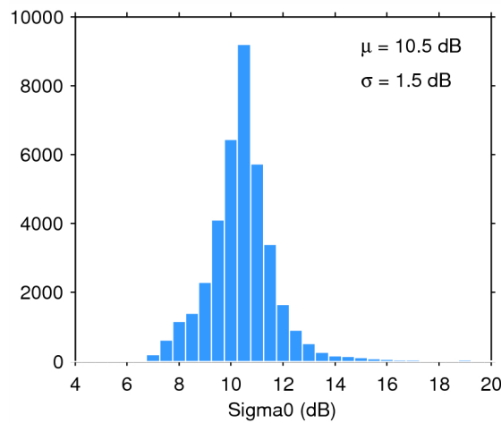
Figure 28. Histogram of science-valid sigma0 over oceans and lakes for 09/11/2014. The mean ( \mu ) and standard deviation ( \sigma ) are also shown. Note that values outside [4 20] dB are excluded from the histogram for the sake of readability but not from the computation of \mu and \sigma .
