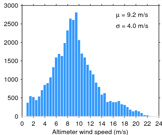
Figure 35. Histogram of science-valid wind over oceans and lakes for 09/11/2014. The mean ( \mu ) and standard deviation ( \sigma ) are also shown. Note that values larger than 24 m/s are excluded from the histogram for the sake of readability but not from the computation of \mu and \sigma .
