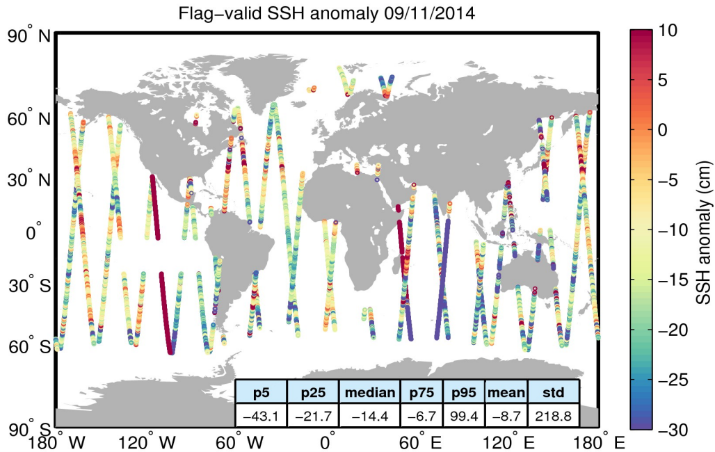
Figure 5. Geographical distribution of flag-valid 1-Hz SSH anomaly data over oceans and lakes for 09/11/2014. The statistical values shown in the table refer to the SSH anomaly in cm and are calculated over all measurements shown in the figure.
