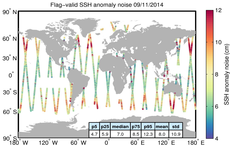
Figure 8. Geographical distribution of flag-valid 20-Hz SSH anomaly measurement noise over oceans and lakes for 09/11/2014. The statistical values shown in the table refer to the SSH anomaly noise and are calculated over all measurements shown in the figure.
