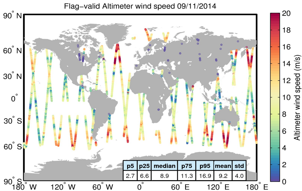
Figure 31. Geographical distribution of flag-valid wind data over oceans and lakes for 09/11/2014. The statistical values shown in the table refer to the wind in m/s and are calculated over all measurements shown in the figure.
