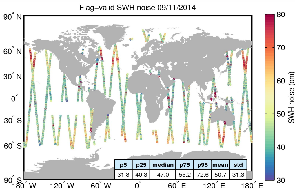
Figure 18. Geographical distribution of flag-valid 20-Hz SWH measurement noise over oceans and lakes for 09/11/2014. The statistical values shown in the figure refer to the SWH noise and are calculated over all measurements shown in the figure.
