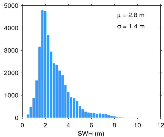
Figure 20. Histogram of science-valid SWH over oceans and lakes for 09/11/2014. The mean ( \mu ) and standard deviation ( \sigma ) are also shown. Note that values larger than 12 m are excluded from the histogram for the sake of readability but not from the computation of \mu and \sigma .
