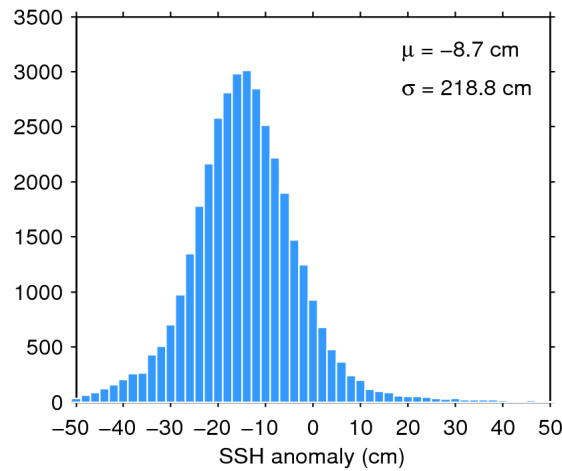
Figure 7. Histogram of flag-valid SSH anomaly over oceans and lakes for 09/11/2014. The mean ( \mu ) and standard deviation ( \sigma ) are also shown. Note that values outside [-50\ 50] cm are excluded from the histogram for the sake of readability but not from the computation of \mu and \sigma .
