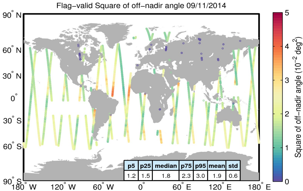
Figure 37. Geographical distribution of flag-valid mispointing data over oceans and lakes for 09/11/2014. The statistical values shown in the table refer to the mispointing in 10^{-2} \text{deg}^2 and are calculated over all measurements shown in the figure.
