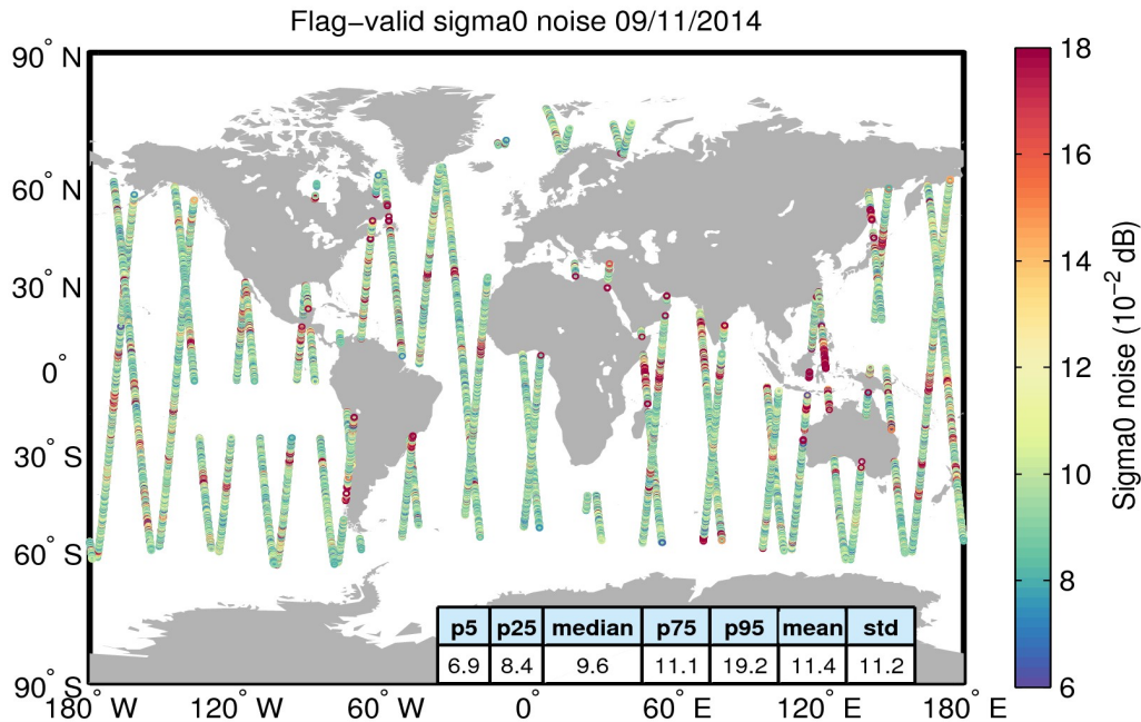
Figure 26. Geographical distribution of flag-valid 20-Hz sigma0 measurement noise over oceans and lakes for 09/11/2014. The statistical values shown in the table refer to the sigma0 noise and are calculated over all measurements shown in the figure.
