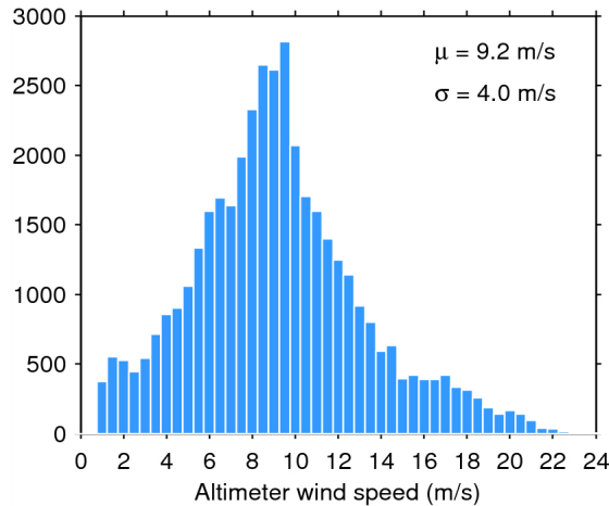
Figure 33. Histogram of flag-valid wind over oceans and lakes for 09/11/2014. The mean ( \mu ) and standard deviation ( \sigma ) are also shown. Note that values larger than 24 m/s are excluded from the histogram for the sake of readability but not from the computation of \mu and \sigma .
