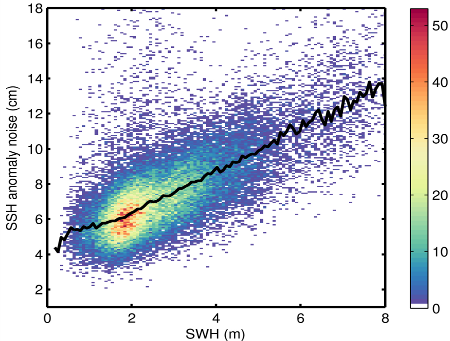
Figure 9. 2D histogram showing flag-valid SSH anomaly noise as a function of SWH for 09/11/2014. The black line denotes the median SSH anomaly as a function of SWH.
