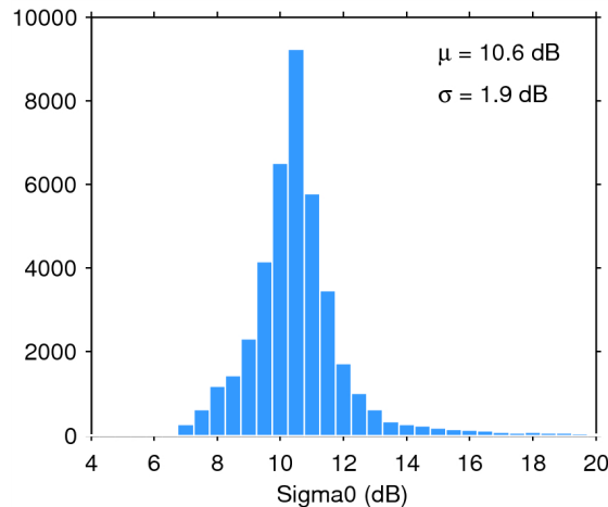
Figure 25. Histogram of flag-valid sigma0 over oceans and lakes for 09/11/2014. The mean ( \mu ) and standard deviation ( \sigma ) are also shown. Note that values outside [4 20] dB are excluded from the histogram for the sake of readability but not from the computation of \mu and \sigma .
