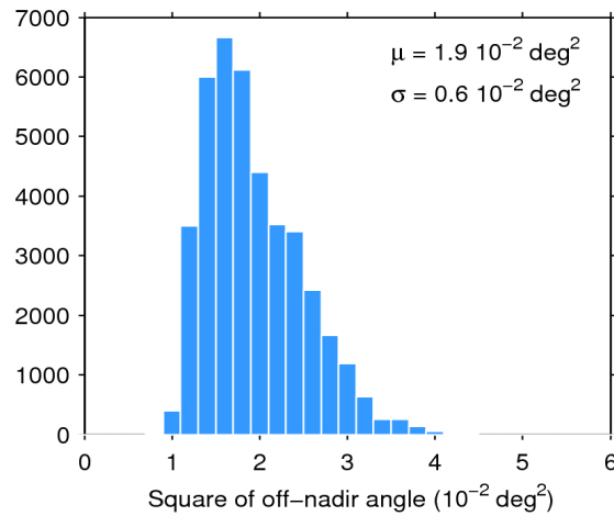
Figure 39. Histogram of flag-valid mispointing over oceans and lakes for 09/11/2014. The mean ( \mu ) and standard deviation ( \sigma ) are also shown. Note that values than 6 \cdot 10^{-2} \text{ deg}^2 are excluded from the histogram for the sake of readability but not from the computation of \mu and \sigma .
