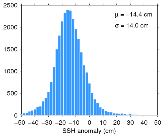
Figure 11. Histogram of science-valid SSH anomaly over oceans and lakes for 09/11/2014. The mean ( \mu ) and standard deviation ( \sigma ) are also shown. Note that values outside [-50 50] cm are excluded from the histogram for the sake of readability but not from the computation of \mu and \sigma .
