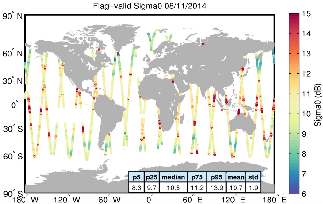
Figure 23. Geographical distribution of flag-valid sigma0 data over oceans and lakes for 08/11/2014. The statistical values shown in the table refer to the sigma0 in dB and are calculated over all measurements shown in the figure.
