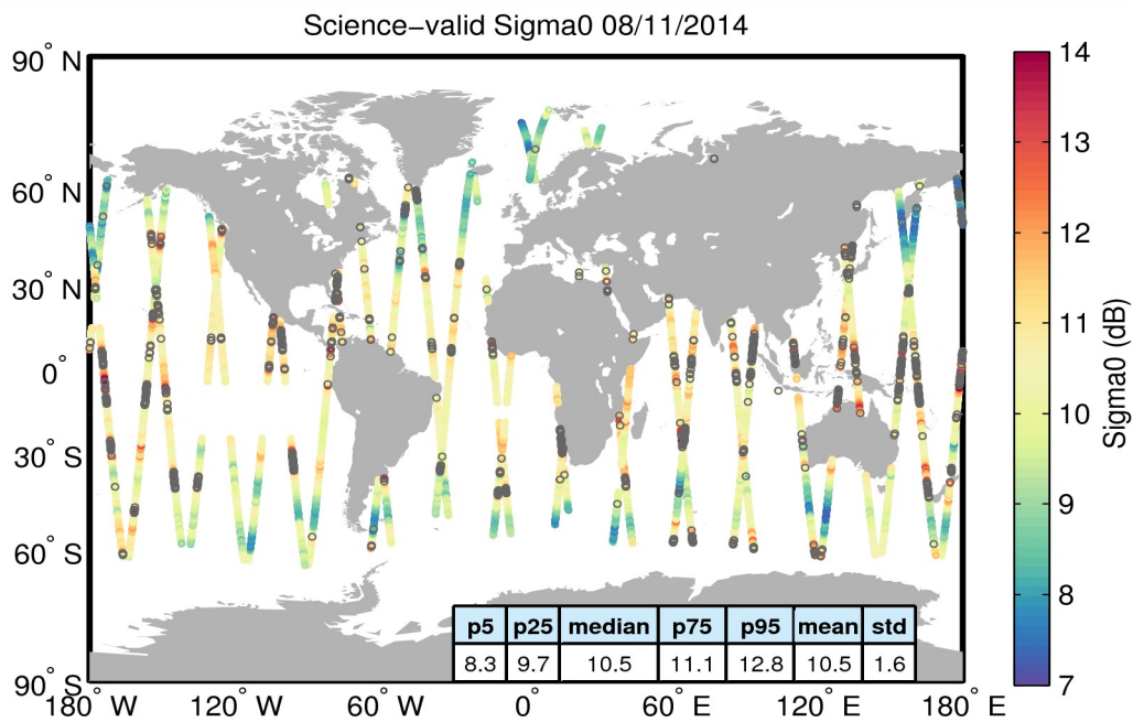
Figure 27. Geographical distribution of science-valid sigma0 data over oceans and lakes for 08/11/2014. The statistical values shown in the table refer to the sigma0 in dB and are calculated over all measurements shown in the figure. Gray circles denote records that have been rejected based on the editing criteria described in Table 4.
