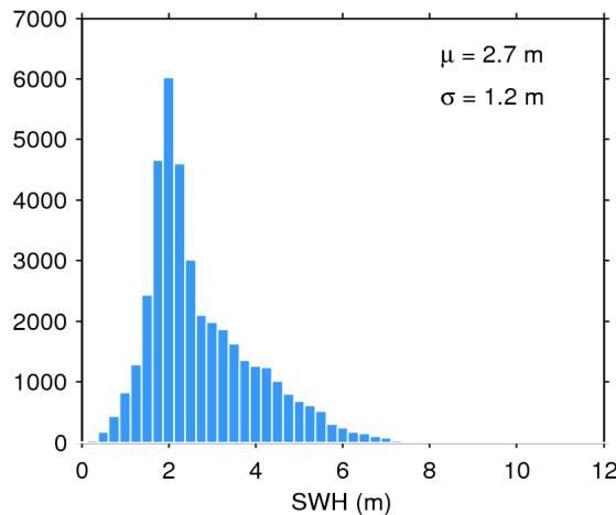
Figure 20. Histogram of science-valid SWH over oceans and lakes for 08/11/2014. The mean ( \mu ) and standard deviation ( \sigma ) are also shown. Note that values larger than 12 m are excluded from the histogram for the sake of readability but not from the computation of \mu and \sigma .
