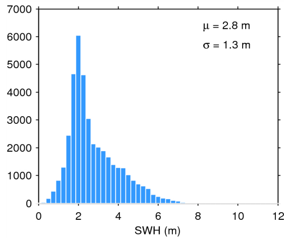
Figure 17. Histogram of flag-valid SWH over oceans and lakes for 08/11/2014. The mean ( \mu ) and standard deviation ( \sigma ) are also shown. Note that values larger than 12 m are excluded from the histogram for the sake of readability but not from the computation of \mu and \sigma .
