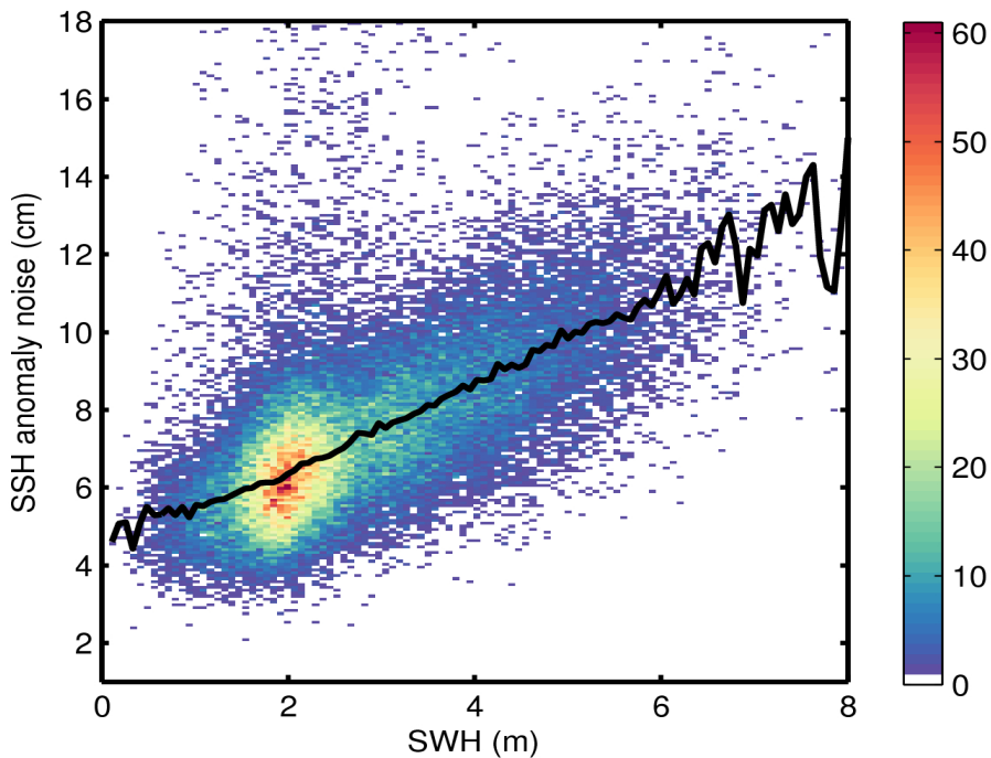
Figure 9. 2D histogram showing flag-valid SSH anomaly noise as a function of SWH for 08/11/2014. The black line denotes the median SSH anomaly as a function of SWH.
