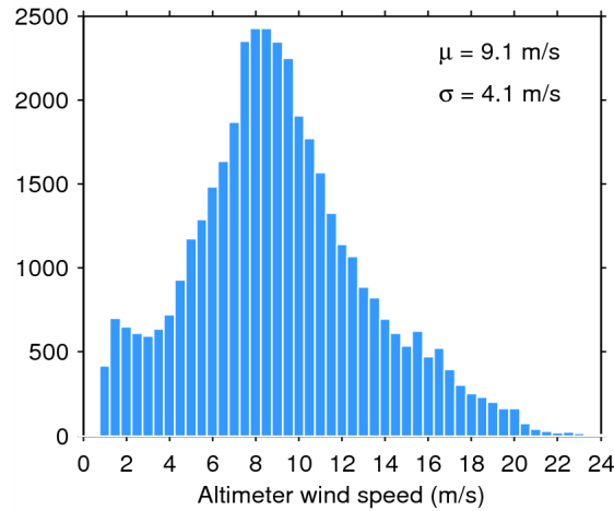
Figure 33. Histogram of flag-valid wind over oceans and lakes for 08/11/2014. The mean ( \mu ) and standard deviation ( \sigma ) are also shown. Note that values larger than 24 m/s are excluded from the histogram for the sake of readability but not from the computation of \mu and \sigma .
