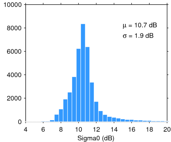
Figure 25. Histogram of flag-valid sigma0 over oceans and lakes for 08/11/2014. The mean ( \mu ) and standard deviation ( \sigma ) are also shown. Note that values outside [4 20] dB are excluded from the histogram for the sake of readability but not from the computation of \mu and \sigma .
