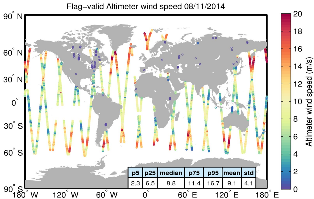
Figure 31. Geographical distribution of flag-valid wind data over oceans and lakes for 08/11/2014. The statistical values shown in the figure refer to the wind in m/s and are calculated over all measurements shown in the figure.
