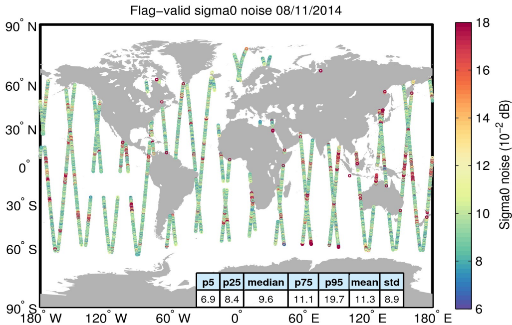
Figure 26. Geographical distribution of flag-valid 20-Hz sigma0 measurement noise over oceans and lakes for 08/11/2014. The statistical values shown in the table refer to the sigma0 noise and are calculated over all measurements shown in the figure.
