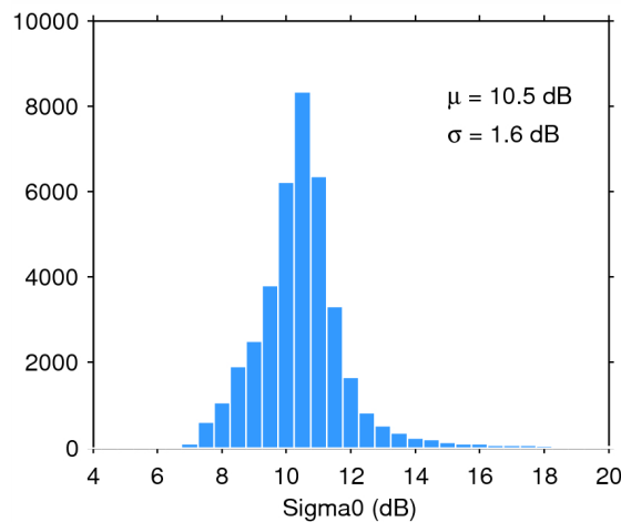
Figure 28. Histogram of science-valid sigma0 over oceans and lakes for 08/11/2014. The mean ( \mu ) and standard deviation ( \sigma ) are also shown. Note that values outside [4 20] dB are excluded from the histogram for the sake of readability but not from the computation of \mu and \sigma .
