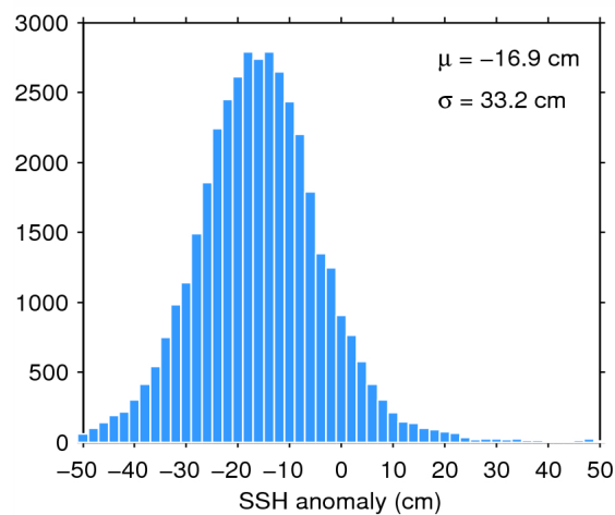
Figure 7. Histogram of flag-valid SSH anomaly over oceans and lakes for 08/11/2014. The mean ( \mu ) and standard deviation ( \sigma ) are also shown. Note that values outside [-50\ 50] cm are excluded from the histogram for the sake of readability but not from the computation of \mu and \sigma .
