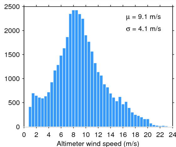
Figure 35. Histogram of science-valid wind over oceans and lakes for 08/11/2014. The mean ( \mu ) and standard deviation ( \sigma ) are also shown. Note that values larger than 24 m/s are excluded from the histogram for the sake of readability but not from the computation of \mu and \sigma .
