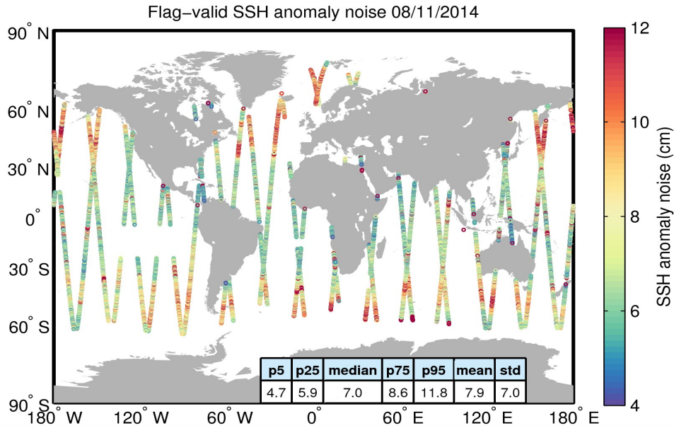
Figure 8. Geographical distribution of flag-valid 20-Hz SSH anomaly measurement noise over oceans and lakes for 08/11/2014. The statistical values shown in the table refer to the SSH anomaly noise and are calculated over all measurements shown in the figure.
