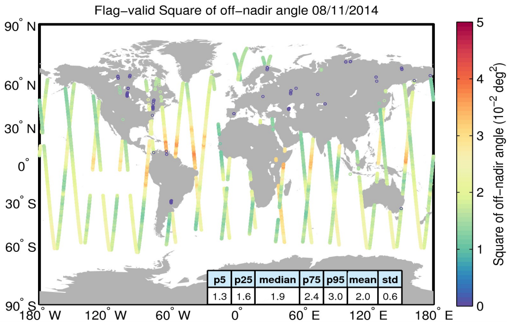
Figure 37. Geographical distribution of flag-valid mispointing data over oceans and lakes for 08/11/2014. The statistical values shown in the table refer to the mispointing in 10^{-2} \text{ deg}^2 and are calculated over all measurements shown in the figure.
