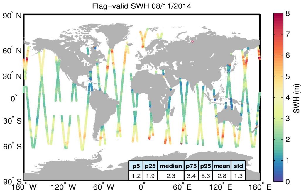
Figure 15. Geographical distribution of flag-valid SWH data over oceans and lakes for 08/11/2014. The statistical values shown in the figure refer to the SWH in m and are calculated over all measurements shown in the figure.
