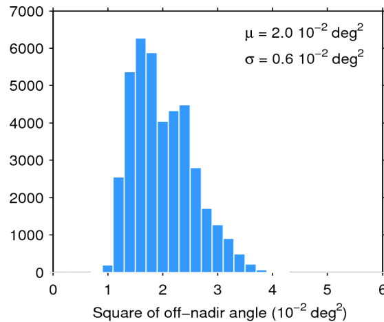
Figure 39. Histogram of flag-valid mispointing over oceans and lakes for 08/11/2014. The mean ( \mu ) and standard deviation ( \sigma ) are also shown. Note that values than 6 \cdot 10^{-2} \text{ deg}^2 are excluded from the histogram for the sake of readability but not from the computation of \mu and \sigma .
