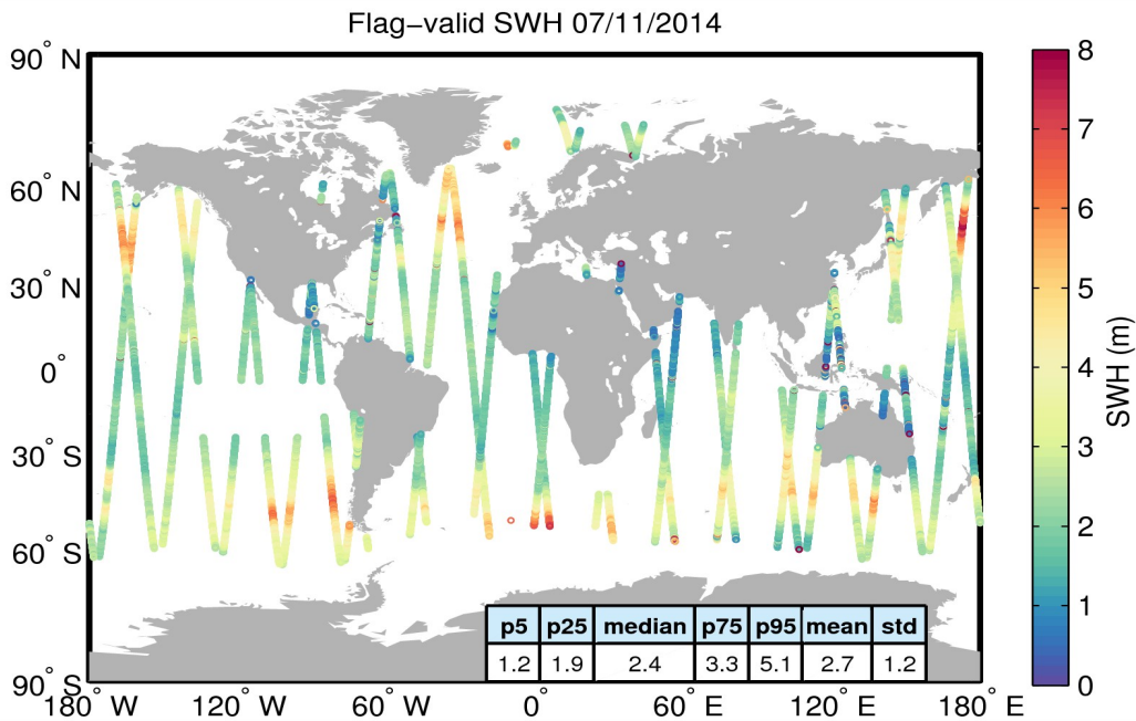
Figure 15. Geographical distribution of flag-valid SWH data over oceans and lakes for 07/11/2014. The statistical values shown in the table refer to the SWH in m and are calculated over all measurements shown in the figure.
