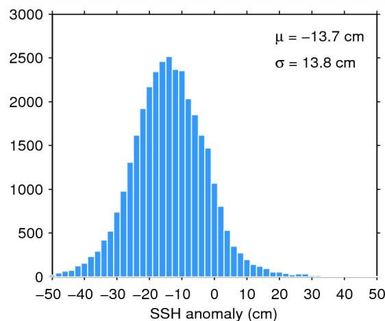
Figure 11. Histogram of science-valid SSH anomaly over oceans and lakes for 07/11/2014. The mean ( \mu ) and standard deviation ( \sigma ) are also shown. Note that values outside [-50 50] cm are excluded from the histogram for the sake of readability but not from the computation of \mu and \sigma .
