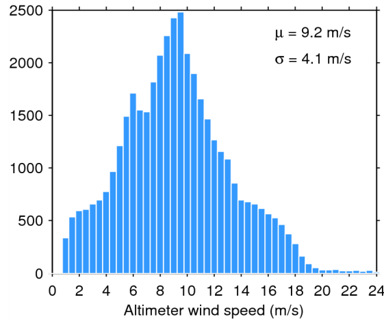
Figure 33. Histogram of flag-valid wind over oceans and lakes for 07/11/2014. The mean ( \mu ) and standard deviation ( \sigma ) are also shown. Note that values larger than 24 m/s are excluded from the histogram for the sake of readability but not from the computation of \mu and \sigma .
