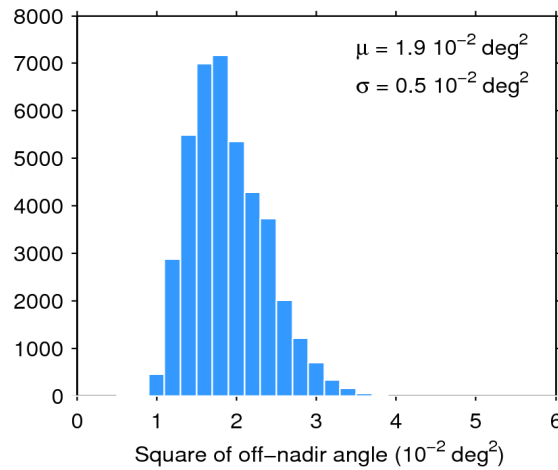
Figure 39. Histogram of flag-valid mispointing over oceans and lakes for 07/11/2014. The mean ( \mu ) and standard deviation ( \sigma ) are also shown. Note that values than 6 \cdot 10^{-2} \text{ deg}^2 are excluded from the histogram for the sake of readability but not from the computation of \mu and \sigma .
