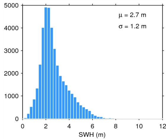
Figure 17. Histogram of flag-valid SWH over oceans and lakes for 07/11/2014. The mean ( \mu ) and standard deviation ( \sigma ) are also shown. Note that values larger than 12 m are excluded from the histogram for the sake of readability but not from the computation of \mu and \sigma .
