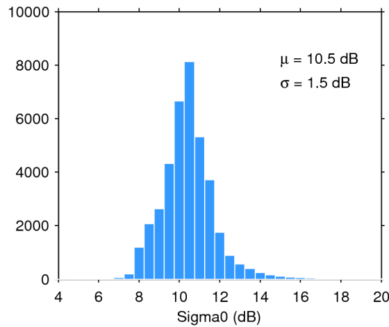
Figure 28. Histogram of science-valid sigma0 over oceans and lakes for 07/11/2014. The mean ( \mu ) and standard deviation ( \sigma ) are also shown. Note that values outside [4 20] dB are excluded from the histogram for the sake of readability but not from the computation of \mu and \sigma .
