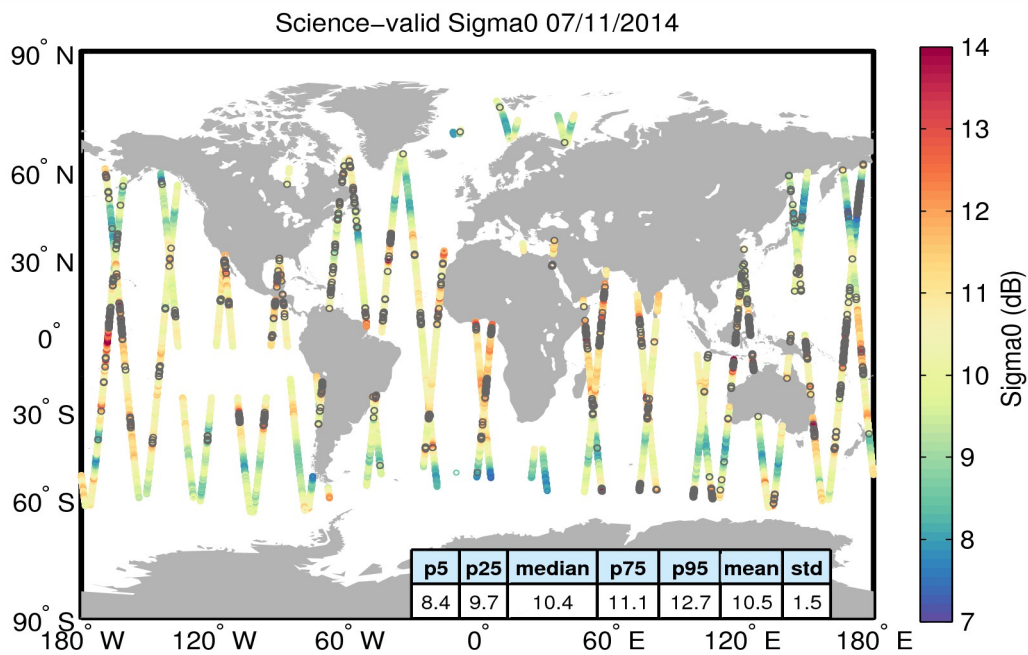
Figure 27. Geographical distribution of science-valid sigma0 data over oceans and lakes for 07/11/2014. The statistical values shown in the table refer to the sigma0 in dB and are calculated over all measurements shown in the figure. Gray circles denote records that have been rejected based on the editing criteria described in Table 4.
