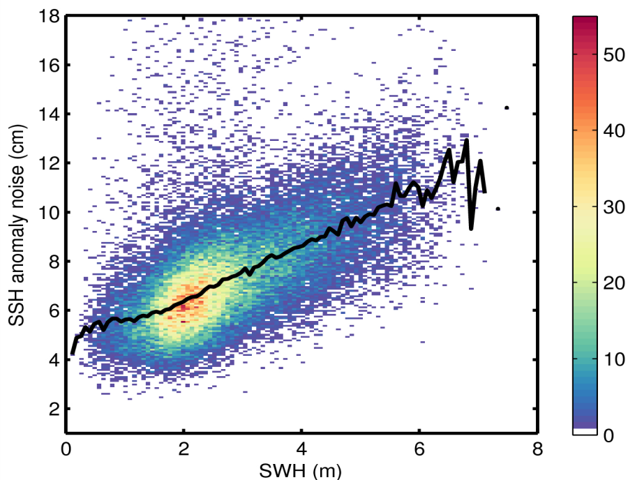
Figure 9. 2D histogram showing flag-valid SSH anomaly noise as a function of SWH for 07/11/2014. The black line denotes the median SSH anomaly as a function of SWH.
