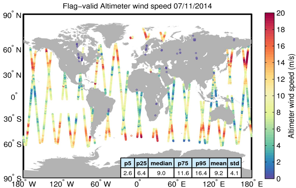
Figure 31. Geographical distribution of flag-valid wind data over oceans and lakes for 07/11/2014. The statistical values shown in the figure refer to the wind in m/s and are calculated over all measurements shown in the figure.
