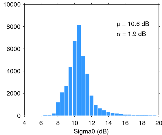
Figure 25. Histogram of flag-valid sigma0 over oceans and lakes for 07/11/2014. The mean ( \mu ) and standard deviation ( \sigma ) are also shown. Note that values outside [4 20] dB are excluded from the histogram for the sake of readability but not from the computation of \mu and \sigma .
