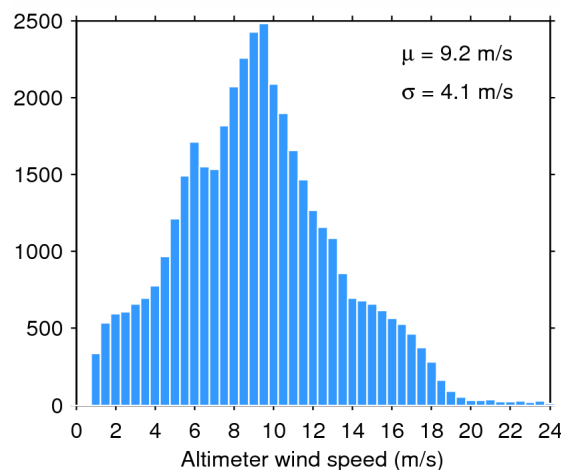
Figure 35. Histogram of science-valid wind over oceans and lakes for 07/11/2014. The mean ( \mu ) and standard deviation ( \sigma ) are also shown. Note that values larger than 24 m/s are excluded from the histogram for the sake of readability but not from the computation of \mu and \sigma .
