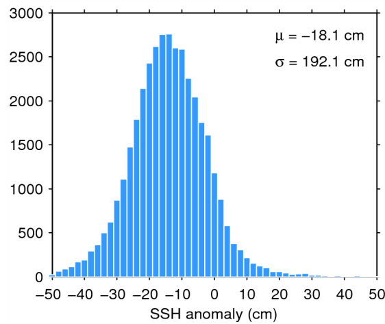
Figure 7. Histogram of flag-valid SSH anomaly over oceans and lakes for 07/11/2014. The mean ( \mu ) and standard deviation ( \sigma ) are also shown. Note that values outside [-50 50] cm are excluded from the histogram for the sake of readability but not from the computation of \mu and \sigma .
