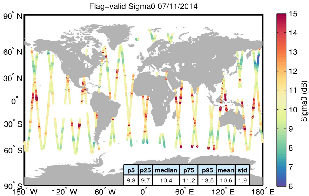
Figure 23. Geographical distribution of flag-valid sigma0 data over oceans and lakes for 07/11/2014. The statistical values shown in the table refer to the sigma0 in dB and are calculated over all measurements shown in the figure.
