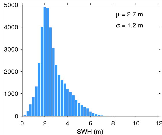
Figure 20. Histogram of science-valid SWH over oceans and lakes for 07/11/2014. The mean ( \mu ) and standard deviation ( \sigma ) are also shown. Note that values larger than 12 m are excluded from the histogram for the sake of readability but not from the computation of \mu and \sigma .
