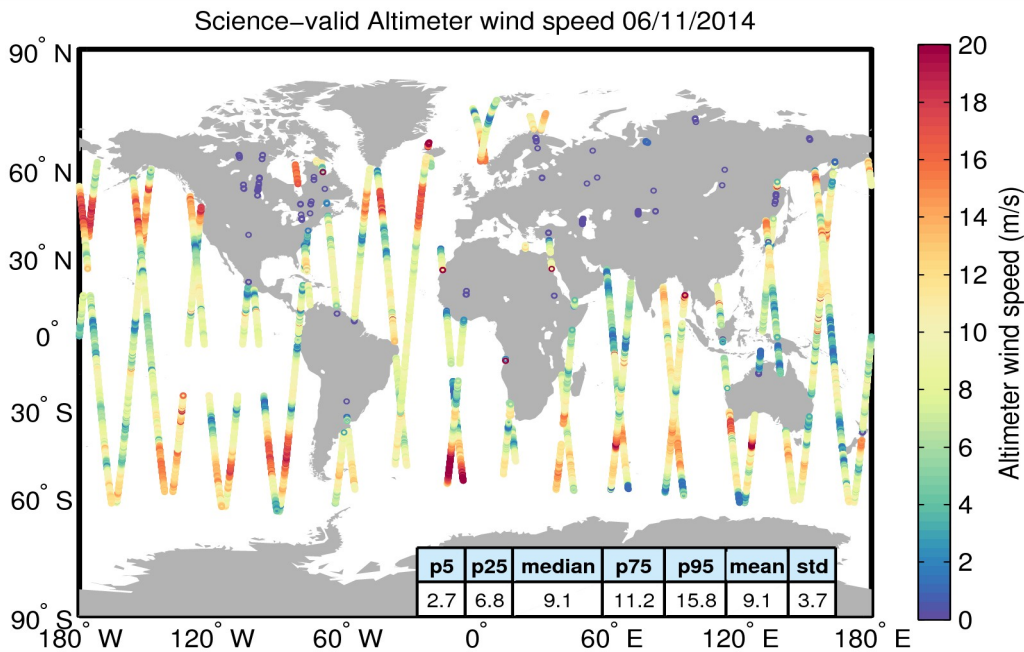
Figure 34. Geographical distribution of science-valid wind data over oceans and lakes for 06/11/2014. The statistical values shown in the table refer to the wind in m/s and are calculated over all measurements shown in the figure. Gray circles denote records that have been rejected based on the editing criteria described in Table 5.
