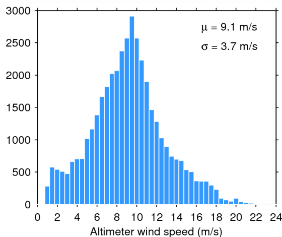
Figure 35. Histogram of science-valid wind over oceans and lakes for 06/11/2014. The mean ( \mu ) and standard deviation ( \sigma ) are also shown. Note that values larger than 24 m/s are excluded from the histogram for the sake of readability but not from the computation of \mu and \sigma .
