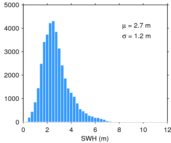
Figure 17. Histogram of flag-valid SWH over oceans and lakes for 06/11/2014. The mean ( \mu ) and standard deviation ( \sigma ) are also shown. Note that values larger than 12 m are excluded from the histogram for the sake of readability but not from the computation of \mu and \sigma .
