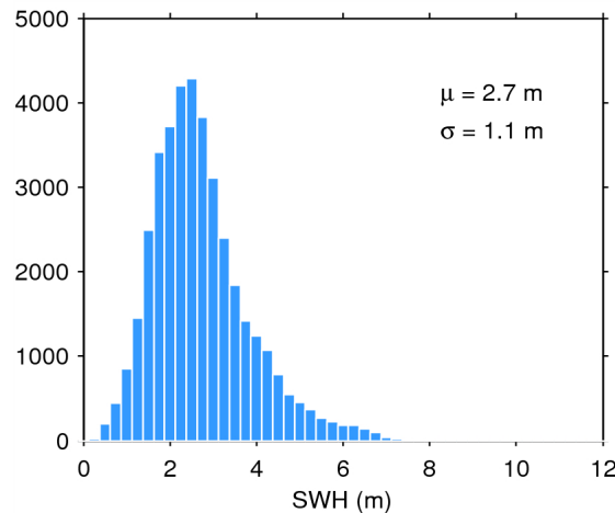
Figure 20. Histogram of science-valid SWH over oceans and lakes for 06/11/2014. The mean ( \mu ) and standard deviation ( \sigma ) are also shown. Note that values larger than 12 m are excluded from the histogram for the sake of readability but not from the computation of \mu and \sigma .
