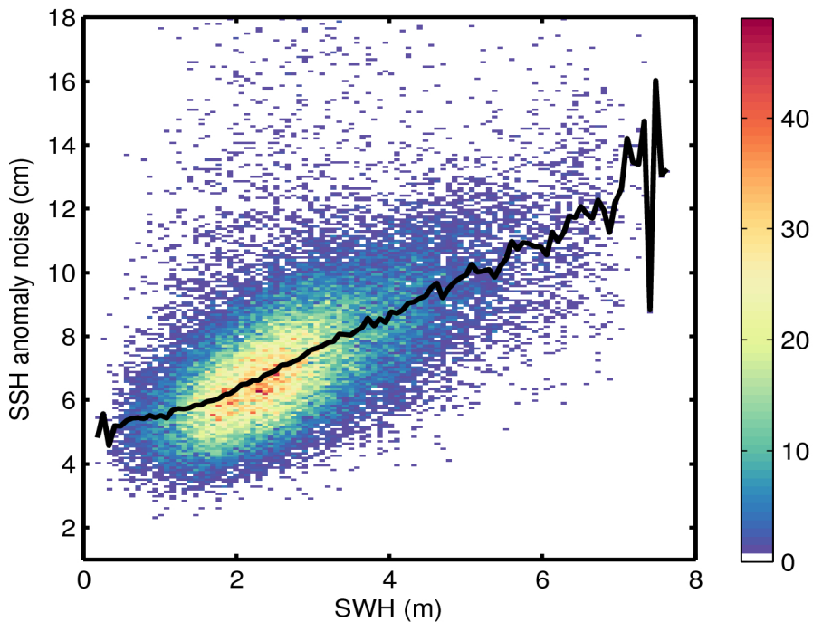
Figure 9. 2D histogram showing flag-valid SSH anomaly noise as a function of SWH for 06/11/2014. The black line denotes the median SSH anomaly as a function of SWH.
