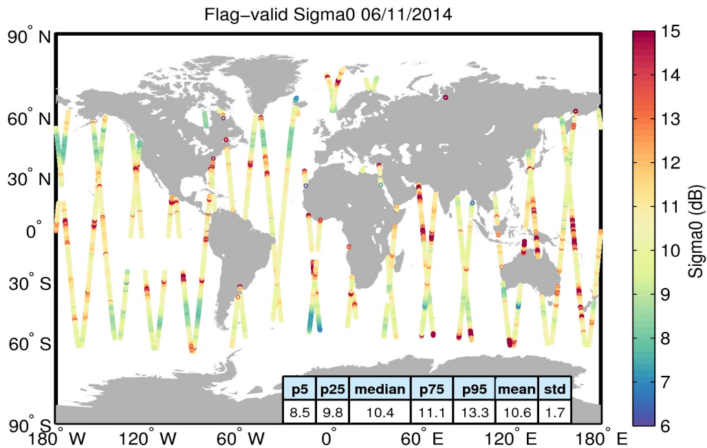
Figure 23. Geographical distribution of flag-valid sigma0 data over oceans and lakes for 06/11/2014. The statistical values shown in the table refer to the sigma0 in dB and are calculated over all measurements shown in the figure.
