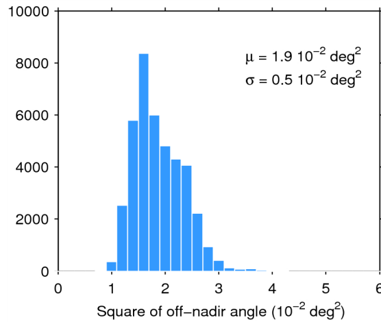
Figure 39. Histogram of flag-valid mispointing over oceans and lakes for 06/11/2014. The mean ( \mu ) and standard deviation ( \sigma ) are also shown. Note that values than 6 \cdot 10^{-2} \text{ deg}^2 are excluded from the histogram for the sake of readability but not from the computation of \mu and \sigma .
