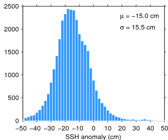
Figure 11. Histogram of science-valid SSH anomaly over oceans and lakes for 06/11/2014. The mean ( \mu ) and standard deviation ( \sigma ) are also shown. Note that values outside [-50 50] cm are excluded from the histogram for the sake of readability but not from the computation of \mu and \sigma .
