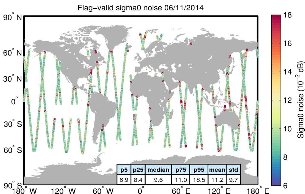
Figure 26. Geographical distribution of flag-valid 20-Hz sigma0 measurement noise over oceans and lakes for 06/11/2014. The statistical values shown in the table refer to the sigma0 noise and are calculated over all measurements shown in the figure.
