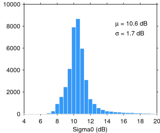
Figure 25. Histogram of flag-valid sigma0 over oceans and lakes for 06/11/2014. The mean ( \mu ) and standard deviation ( \sigma ) are also shown. Note that values outside [4 20] dB are excluded from the histogram for the sake of readability but not from the computation of \mu and \sigma .
