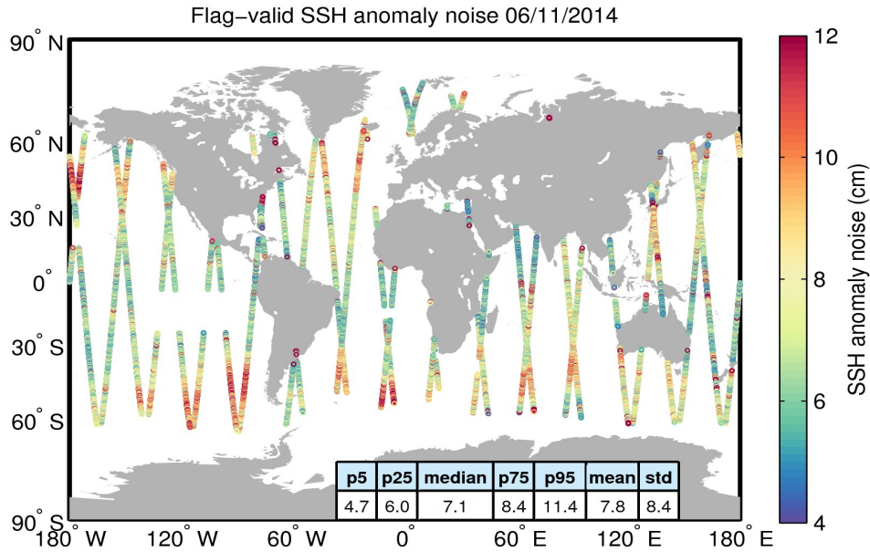
Figure 8. Geographical distribution of flag-valid 20-Hz SSH anomaly measurement noise over oceans and lakes for 06/11/2014. The statistical values shown in the table refer to the SSH anomaly noise and are calculated over all measurements shown in the figure.
