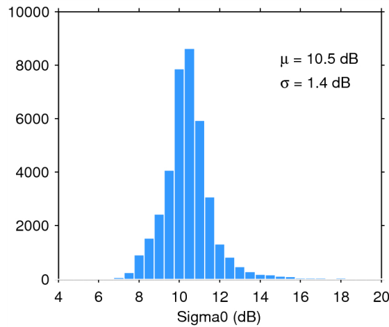
Figure 28. Histogram of science-valid sigma0 over oceans and lakes for 06/11/2014. The mean ( \mu ) and standard deviation ( \sigma ) are also shown. Note that values outside [4 20] dB are excluded from the histogram for the sake of readability but not from the computation of \mu and \sigma .
