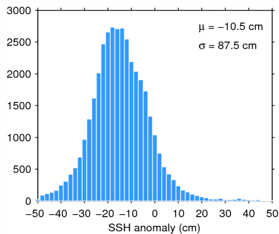
Figure 7. Histogram of flag-valid SSH anomaly over oceans and lakes for 06/11/2014. The mean ( \mu ) and standard deviation ( \sigma ) are also shown. Note that values outside [-50\ 50] cm are excluded from the histogram for the sake of readability but not from the computation of \mu and \sigma .
