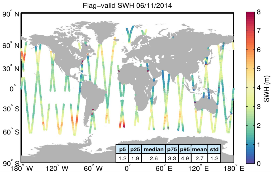
Figure 15. Geographical distribution of flag-valid SWH data over oceans and lakes for 06/11/2014. The statistical values shown in the table refer to the SWH in m and are calculated over all measurements shown in the figure.
