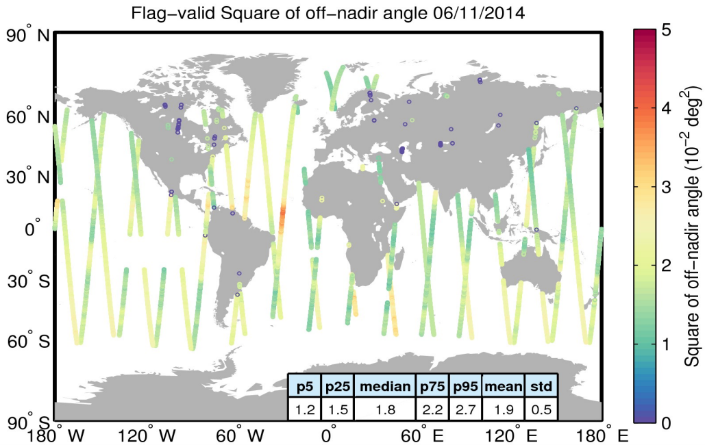
Figure 37. Geographical distribution of flag-valid mispointing data over oceans and lakes for 06/11/2014. The statistical values shown in the table refer to the mispointing in 10^{-2} \text{ deg}^2 and are calculated over all measurements shown in the figure.
