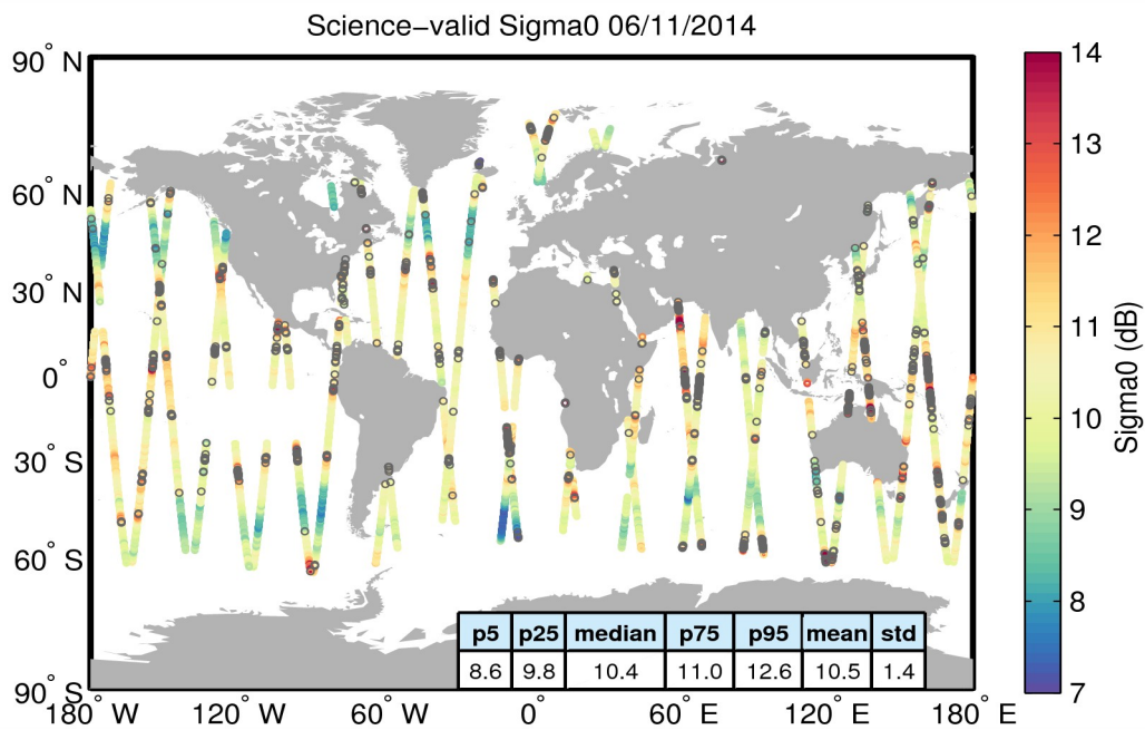
Figure 27. Geographical distribution of science-valid sigma0 data over oceans and lakes for 06/11/2014. The statistical values shown in the table refer to the sigma0 in dB and are calculated over all measurements shown in the figure. Gray circles denote records that have been rejected based on the editing criteria described in Table 4.
