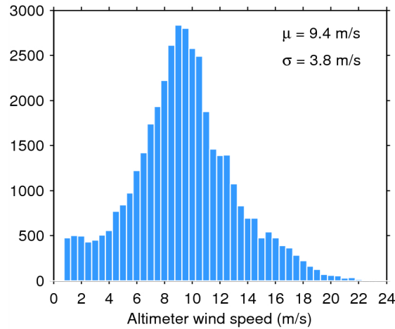
Figure 33. Histogram of flag-valid wind over oceans and lakes for 05/11/2014. The mean ( \mu ) and standard deviation ( \sigma ) are also shown. Note that values larger than 24 m/s are excluded from the histogram for the sake of readability but not from the computation of \mu and \sigma .
