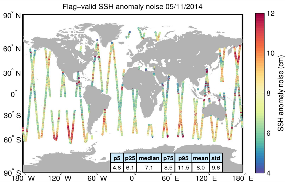
Figure 8. Geographical distribution of flag-valid 20-Hz SSH anomaly measurement noise over oceans and lakes for 05/11/2014. The statistical values shown in the table refer to the SSH anomaly noise and are calculated over all measurements shown in the figure.
