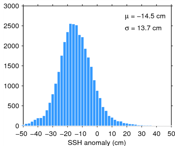
Figure 11. Histogram of science-valid SSH anomaly over oceans and lakes for 05/11/2014. The mean ( \mu ) and standard deviation ( \sigma ) are also shown. Note that values outside [-50 50] cm are excluded from the histogram for the sake of readability but not from the computation of \mu and \sigma .
