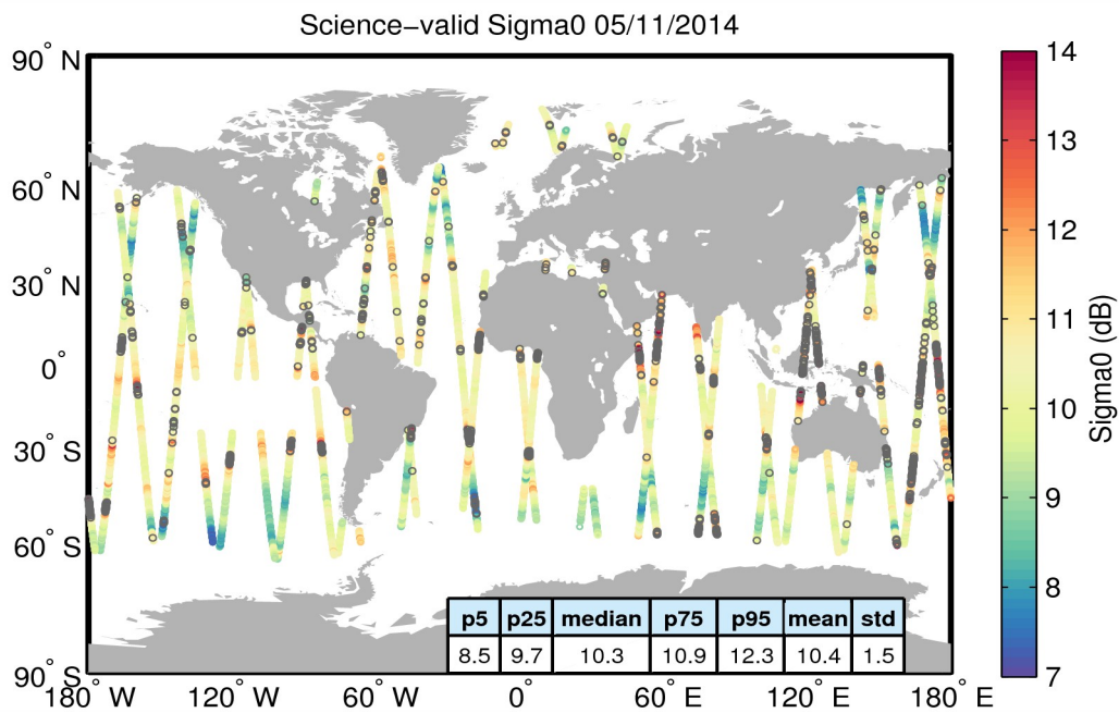
Figure 27. Geographical distribution of science-valid sigma0 data over oceans and lakes for 05/11/2014. The statistical values shown in the table refer to the sigma0 in dB and are calculated over all measurements shown in the figure. Gray circles denote records that have been rejected based on the editing criteria described in Table 4.
