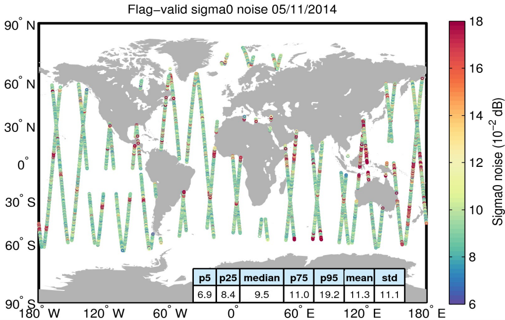
Figure 26. Geographical distribution of flag-valid 20-Hz sigma0 measurement noise over oceans and lakes for 05/11/2014. The statistical values shown in the table refer to the sigma0 noise and are calculated over all measurements shown in the figure.
