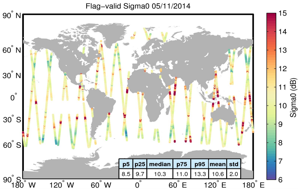
Figure 23. Geographical distribution of flag-valid sigma0 data over oceans and lakes for 05/11/2014. The statistical values shown in the table refer to the sigma0 in dB and are calculated over all measurements shown in the figure.
