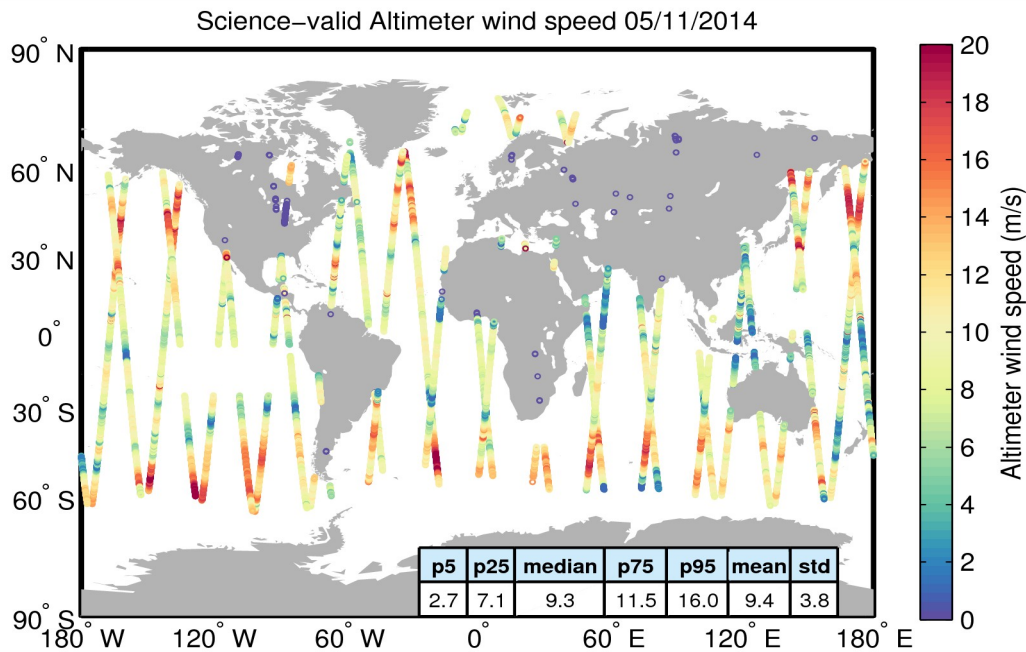
Figure 34. Geographical distribution of science-valid wind data over oceans and lakes for 05/11/2014. The statistical values shown in the table refer to the wind in m/s and are calculated over all measurements shown in the figure. Gray circles denote records that have been rejected based on the editing criteria described in Table 5.
