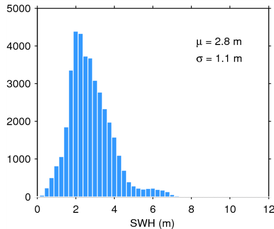
Figure 20. Histogram of science-valid SWH over oceans and lakes for 05/11/2014. The mean ( \mu ) and standard deviation ( \sigma ) are also shown. Note that values larger than 12 m are excluded from the histogram for the sake of readability but not from the computation of \mu and \sigma .
