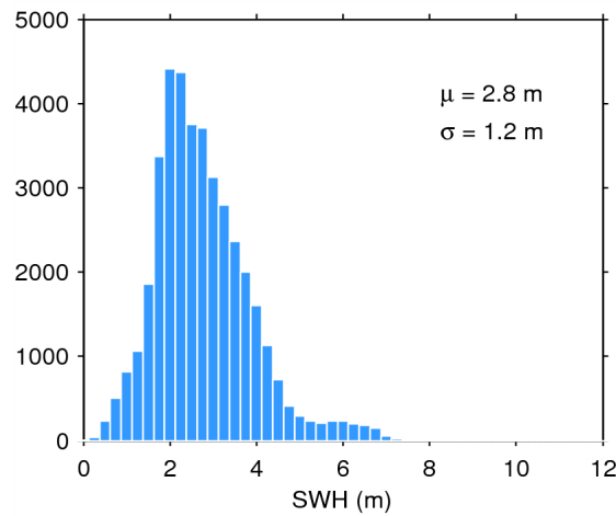
Figure 17. Histogram of flag-valid SWH over oceans and lakes for 05/11/2014. The mean ( \mu ) and standard deviation ( \sigma ) are also shown. Note that values larger than 12 m are excluded from the histogram for the sake of readability but not from the computation of \mu and \sigma .
