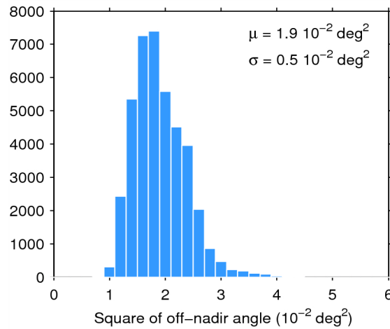
Figure 39. Histogram of flag-valid mispointing over oceans and lakes for 05/11/2014. The mean ( \mu ) and standard deviation ( \sigma ) are also shown. Note that values than 6 \cdot 10^{-2} \text{ deg}^2 are excluded from the histogram for the sake of readability but not from the computation of \mu and \sigma .
