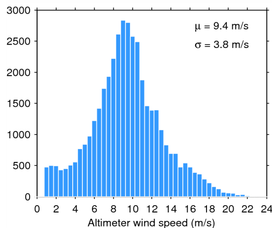
Figure 35. Histogram of science-valid wind over oceans and lakes for 05/11/2014. The mean ( \mu ) and standard deviation ( \sigma ) are also shown. Note that values larger than 24 m/s are excluded from the histogram for the sake of readability but not from the computation of \mu and \sigma .
