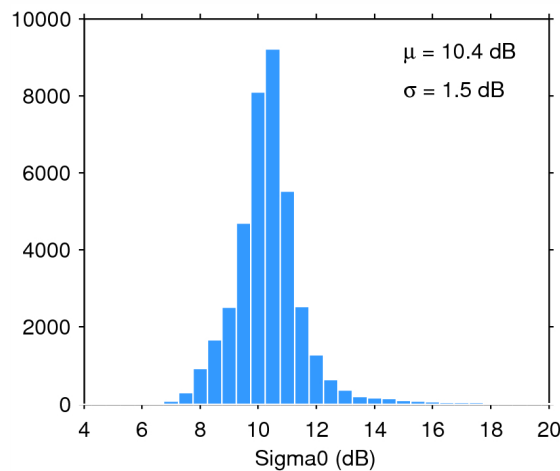
Figure 28. Histogram of science-valid sigma0 over oceans and lakes for 05/11/2014. The mean ( \mu ) and standard deviation ( \sigma ) are also shown. Note that values outside [4 20] dB are excluded from the histogram for the sake of readability but not from the computation of \mu and \sigma .
