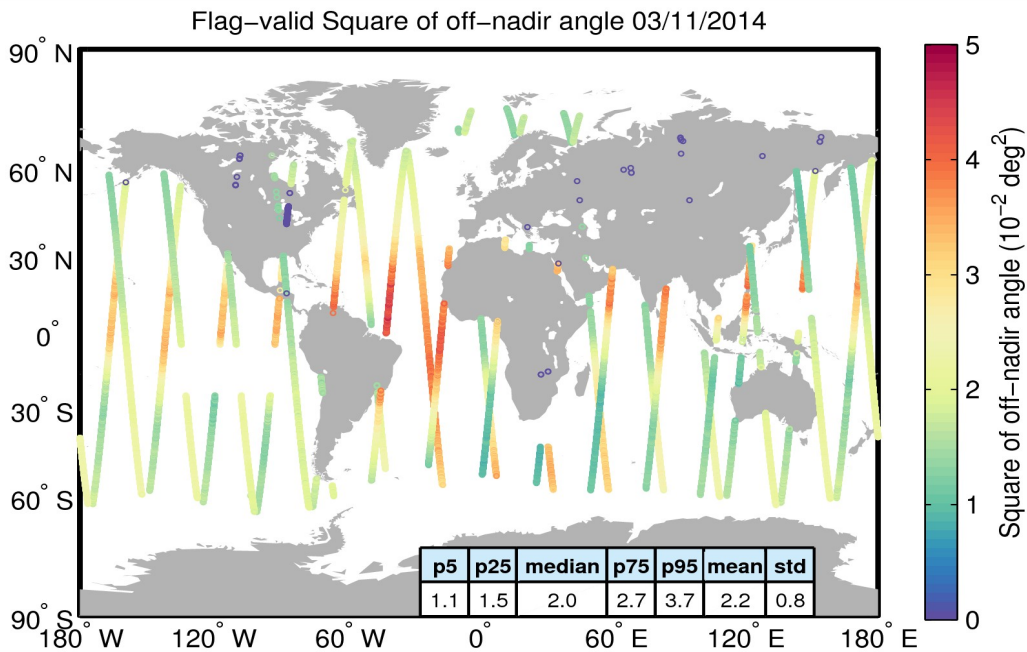
Figure 37. Geographical distribution of flag-valid mispointing data over oceans and lakes for 03/11/2014. The statistical values shown in the table refer to the mispointing in 10^{-2} \text{ deg}^2 and are calculated over all measurements shown in the figure.
