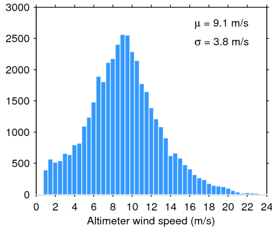
Figure 33. Histogram of flag-valid wind over oceans and lakes for 03/11/2014. The mean ( \mu ) and standard deviation ( \sigma ) are also shown. Note that values larger than 24 m/s are excluded from the histogram for the sake of readability but not from the computation of \mu and \sigma .
