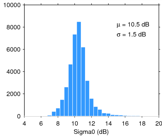
Figure 28. Histogram of science-valid sigma0 over oceans and lakes for 03/11/2014. The mean ( \mu ) and standard deviation ( \sigma ) are also shown. Note that values outside [4 20] dB are excluded from the histogram for the sake of readability but not from the computation of \mu and \sigma .
