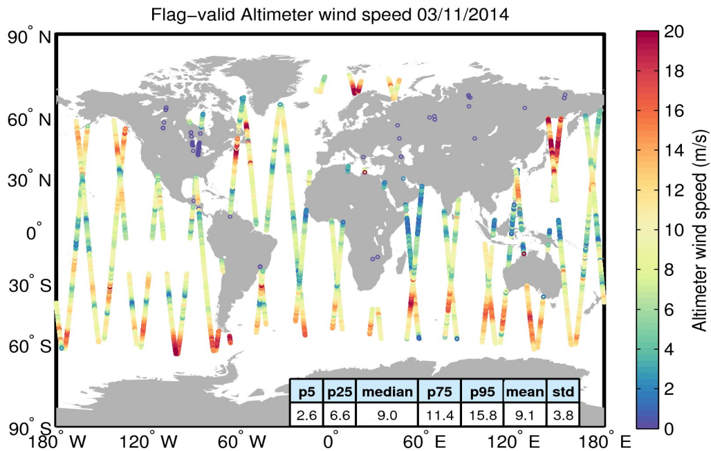
Figure 31. Geographical distribution of flag-valid wind data over oceans and lakes for 03/11/2014. The statistical values shown in the table refer to the wind in m/s and are calculated over all measurements shown in the figure.
