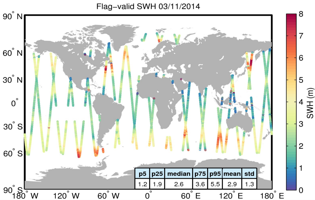
Figure 15. Geographical distribution of flag-valid SWH data over oceans and lakes for 03/11/2014. The statistical values shown in the table refer to the SWH in m and are calculated over all measurements shown in the figure.
