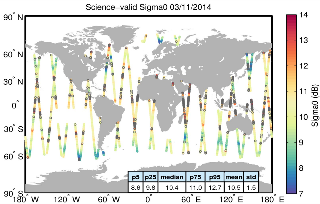
Figure 27. Geographical distribution of science-valid sigma0 data over oceans and lakes for 03/11/2014. The statistical values shown in the table refer to the sigma0 in dB and are calculated over all measurements shown in the figure. Gray circles denote records that have been rejected based on the editing criteria described in Table 4.
