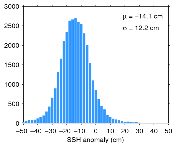
Figure 11. Histogram of science-valid SSH anomaly over oceans and lakes for 03/11/2014. The mean ( \mu ) and standard deviation ( \sigma ) are also shown. Note that values outside [-50 50] cm are excluded from the histogram for the sake of readability but not from the computation of \mu and \sigma .
