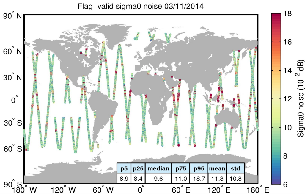
Figure 26. Geographical distribution of flag-valid 20-Hz sigma0 measurement noise over oceans and lakes for 03/11/2014. The statistical values shown in the table refer to the sigma0 noise and are calculated over all measurements shown in the figure.
