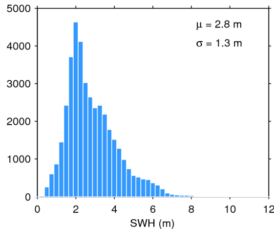
Figure 20. Histogram of science-valid SWH over oceans and lakes for 03/11/2014. The mean ( \mu ) and standard deviation ( \sigma ) are also shown. Note that values larger than 12 m are excluded from the histogram for the sake of readability but not from the computation of \mu and \sigma .
