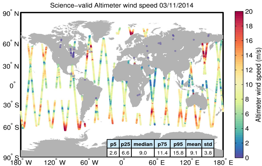
Figure 34. Geographical distribution of science-valid wind data over oceans and lakes for 03/11/2014. The statistical values shown in the table refer to the wind in m/s and are calculated over all measurements shown in the figure. Gray circles denote records that have been rejected based on the editing criteria described in Table 5.
