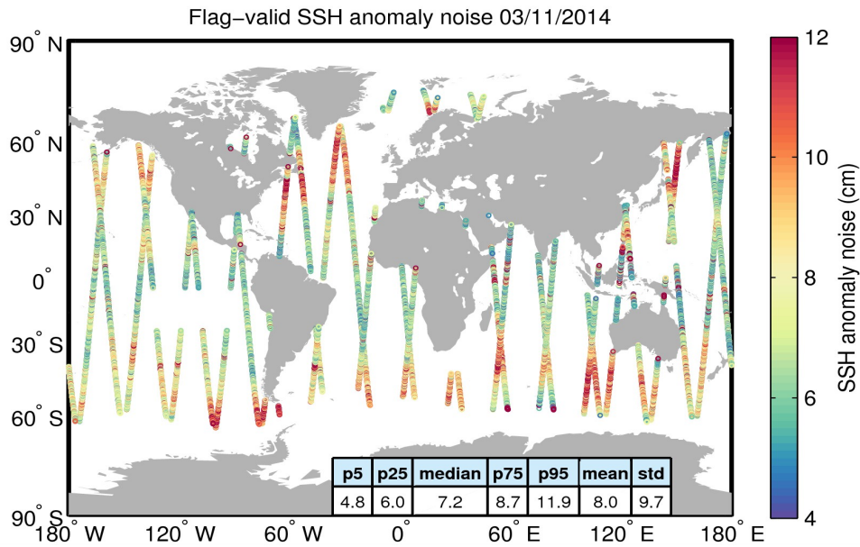
Figure 8. Geographical distribution of flag-valid 20-Hz SSH anomaly measurement noise over oceans and lakes for 03/11/2014. The statistical values shown in the table refer to the SSH anomaly noise and are calculated over all measurements shown in the figure.
