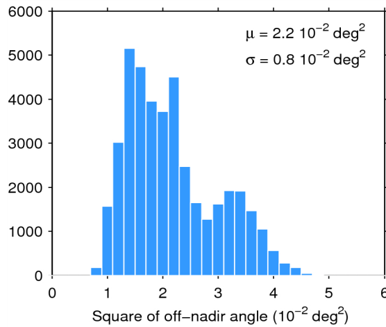
Figure 39. Histogram of flag-valid mispointing over oceans and lakes for 03/11/2014. The mean ( \mu ) and standard deviation ( \sigma ) are also shown. Note that values than 6 \cdot 10^{-2} \text{ deg}^2 are excluded from the histogram for the sake of readability but not from the computation of \mu and \sigma .
