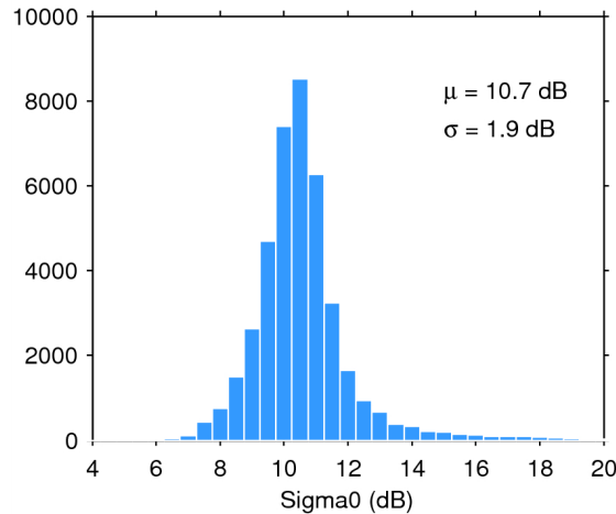
Figure 25. Histogram of flag-valid sigma0 over oceans and lakes for 03/11/2014. The mean ( \mu ) and standard deviation ( \sigma ) are also shown. Note that values outside [4 20] dB are excluded from the histogram for the sake of readability but not from the computation of \mu and \sigma .
