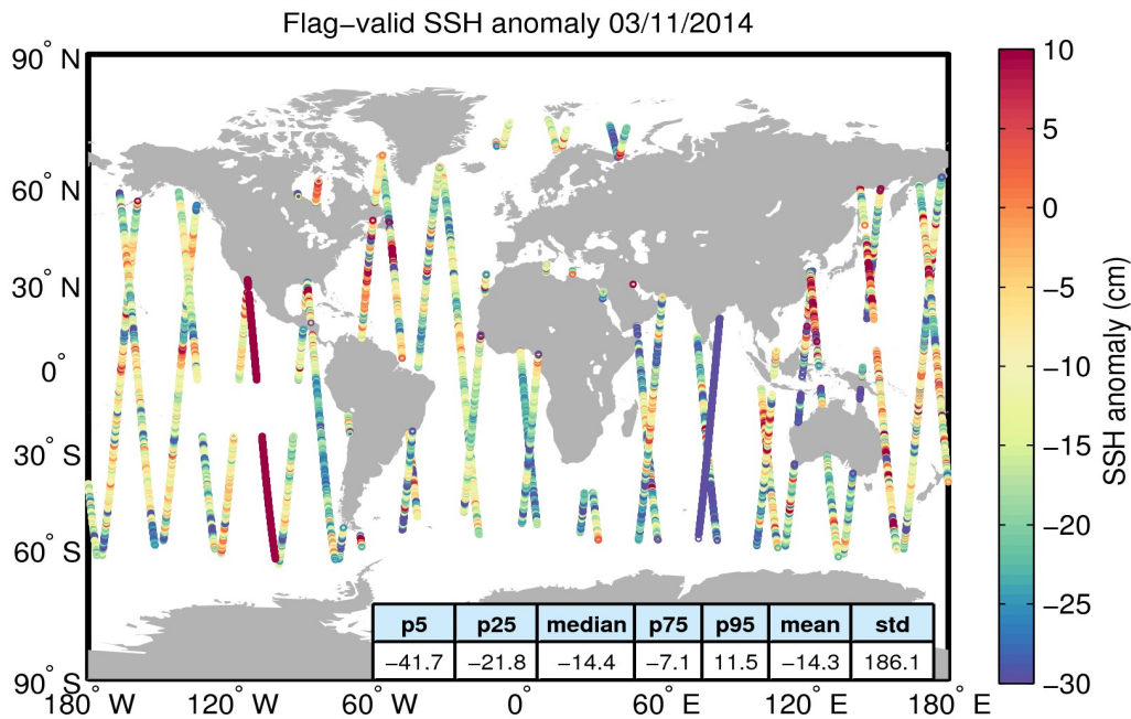
Figure 5. Geographical distribution of flag-valid 1-Hz SSH anomaly data over oceans and lakes for 03/11/2014. The statistical values shown in the table refer to the SSH anomaly in cm and are calculated over all measurements shown in the figure.
