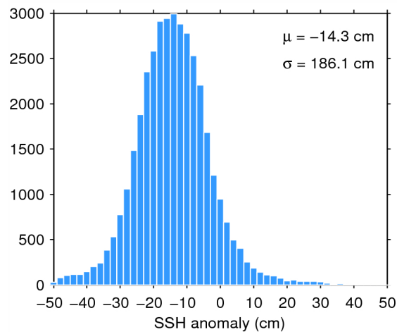
Figure 7. Histogram of flag-valid SSH anomaly over oceans and lakes for 03/11/2014. The mean ( \mu ) and standard deviation ( \sigma ) are also shown. Note that values outside [-50 50] cm are excluded from the histogram for the sake of readability but not from the computation of \mu and \sigma .
