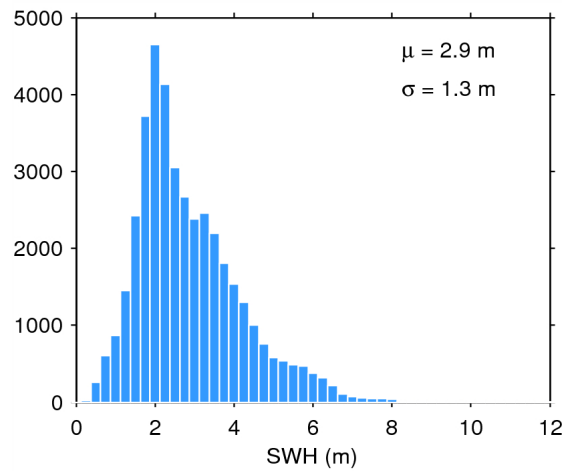
Figure 17. Histogram of flag-valid SWH over oceans and lakes for 03/11/2014. The mean ( \mu ) and standard deviation ( \sigma ) are also shown. Note that values larger than 12 m are excluded from the histogram for the sake of readability but not from the computation of \mu and \sigma .
