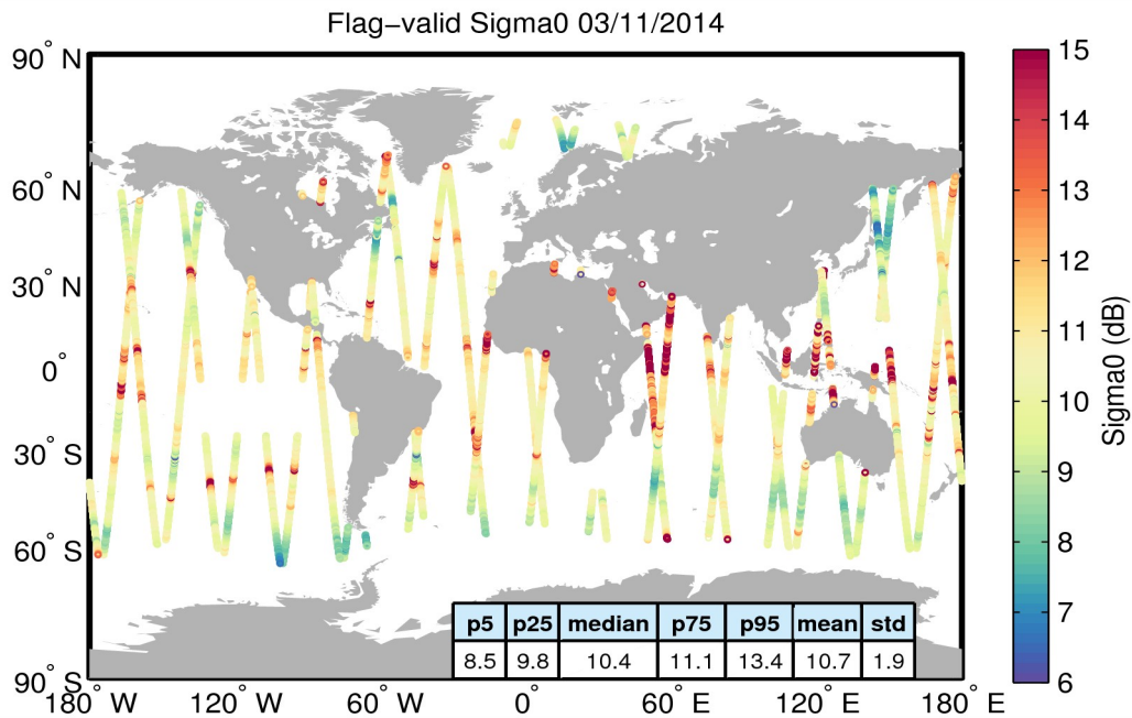
Figure 23. Geographical distribution of flag-valid sigma0 data over oceans and lakes for 03/11/2014. The statistical values shown in the table refer to the sigma0 in dB and are calculated over all measurements shown in the figure.
