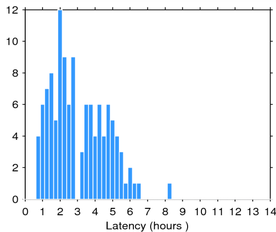
Figure 2. Histogram of the data latency for 03/11/2014. The y-axis denotes the number of files that are made available with a delay of x-hours with respect to the mean time of the records stored in the file.
