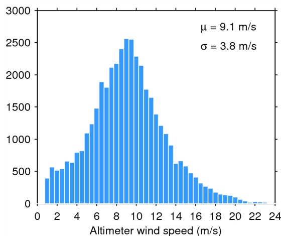
Figure 35. Histogram of science-valid wind over oceans and lakes for 03/11/2014. The mean ( \mu ) and standard deviation ( \sigma ) are also shown. Note that values larger than 24 m/s are excluded from the histogram for the sake of readability but not from the computation of \mu and \sigma .
