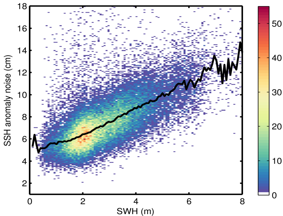
Figure 9. 2D histogram showing flag-valid SSH anomaly noise as a function of SWH for 03/11/2014. The black line denotes the median SSH anomaly as a function of SWH.
