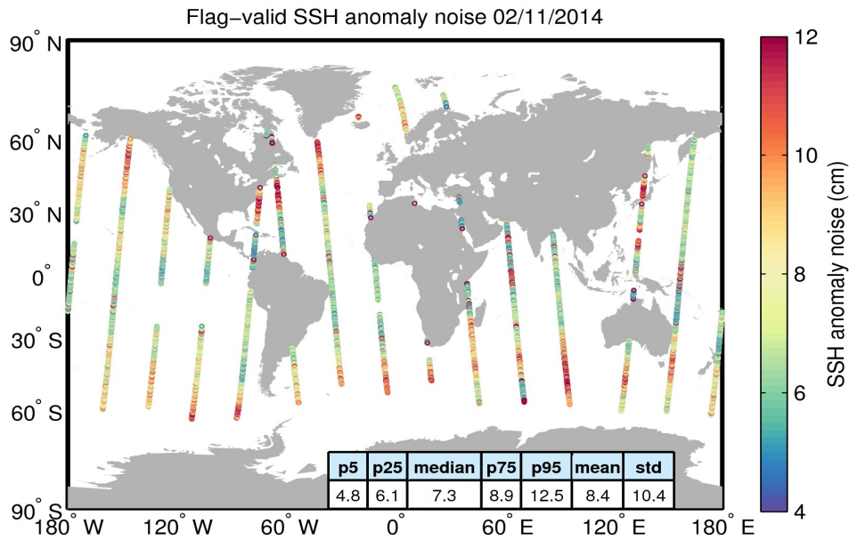
Figure 8. Geographical distribution of flag-valid 20-Hz SSH anomaly measurement noise over oceans and lakes for 02/11/2014. The statistical values shown in the table refer to the SSH anomaly noise and are calculated over all measurements shown in the figure.
