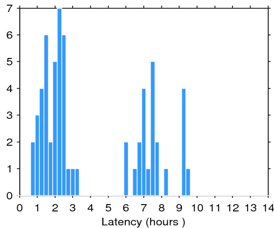
Figure 2. Histogram of the data latency for 02/11/2014. The y-axis denotes the number of files that are made available with a delay of x-hours with respect to the mean time of the records stored in the file.
