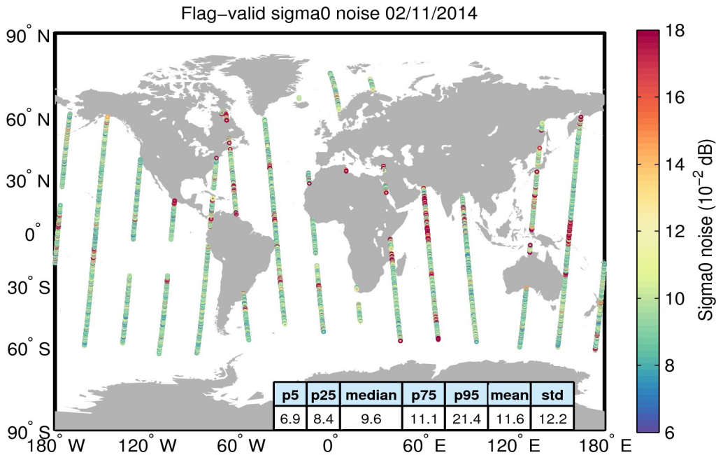
Figure 26. Geographical distribution of flag-valid 20-Hz sigma0 measurement noise over oceans and lakes for 02/11/2014. The statistical values shown in the table refer to the sigma0 noise and are calculated over all measurements shown in the figure.
