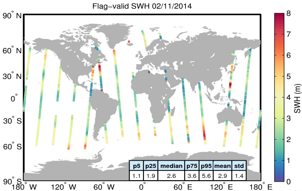
Figure 15. Geographical distribution of flag-valid SWH data over oceans and lakes for 02/11/2014. The statistical values shown in the figure refer to the SWH in m and are calculated over all measurements shown in the figure.
