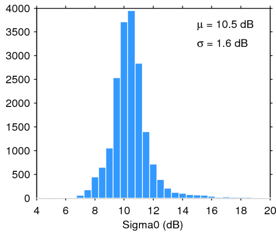
Figure 28. Histogram of science-valid sigma0 over oceans and lakes for 02/11/2014. The mean ( \mu ) and standard deviation ( \sigma ) are also shown. Note that values outside [4 20] dB are excluded from the histogram for the sake of readability but not from the computation of \mu and \sigma .
