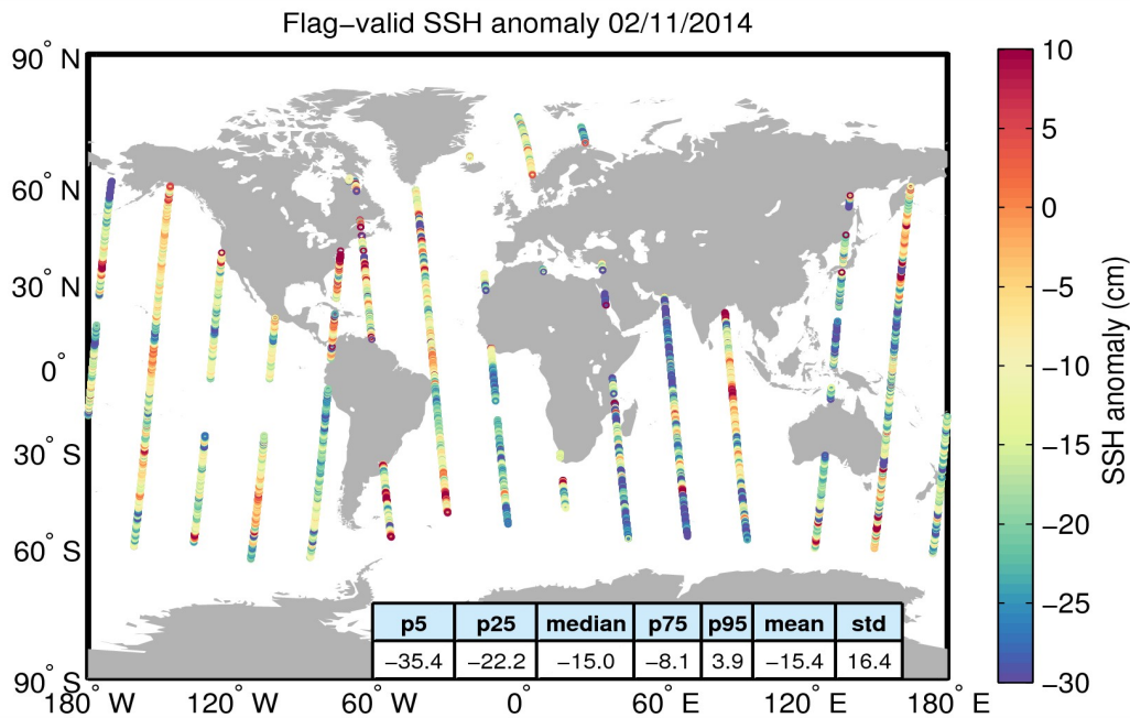
Figure 5. Geographical distribution of flag-valid 1-Hz SSH anomaly data over oceans and lakes for 02/11/2014. The statistical values shown in the table refer to the SSH anomaly in cm and are calculated over all measurements shown in the figure.
