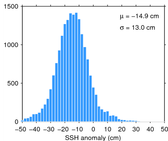
Figure 11. Histogram of science-valid SSH anomaly over oceans and lakes for 02/11/2014. The mean ( \mu ) and standard deviation ( \sigma ) are also shown. Note that values outside [-50 50] cm are excluded from the histogram for the sake of readability but not from the computation of \mu and \sigma .
