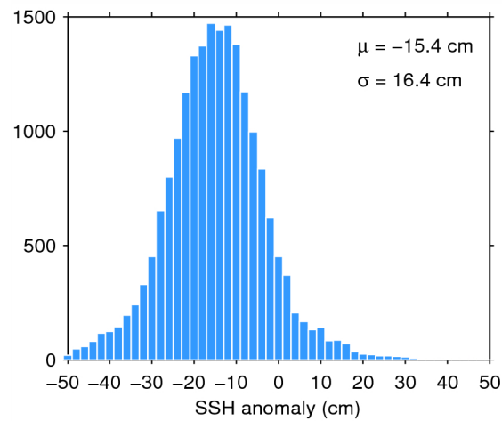
Figure 7. Histogram of flag-valid SSH anomaly over oceans and lakes for 02/11/2014. The mean ( \mu ) and standard deviation ( \sigma ) are also shown. Note that values outside [-50 50] cm are excluded from the histogram for the sake of readability but not from the computation of \mu and \sigma .
