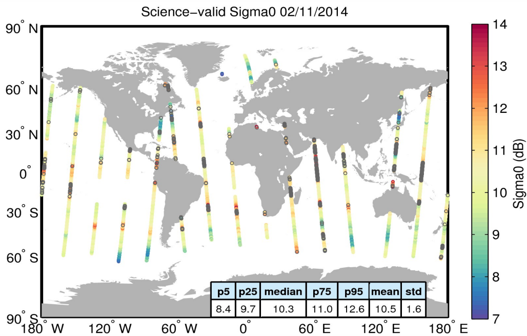
Figure 27. Geographical distribution of science-valid sigma0 data over oceans and lakes for 02/11/2014. The statistical values shown in the table refer to the sigma0 in dB and are calculated over all measurements shown in the figure. Gray circles denote records that have been rejected based on the editing criteria described in Table 4.
