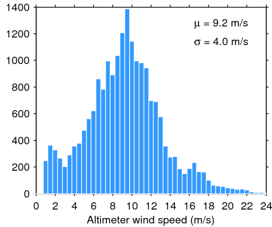
Figure 33. Histogram of flag-valid wind over oceans and lakes for 02/11/2014. The mean ( \mu ) and standard deviation ( \sigma ) are also shown. Note that values larger than 24 m/s are excluded from the histogram for the sake of readability but not from the computation of \mu and \sigma .
