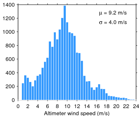
Figure 35. Histogram of science-valid wind over oceans and lakes for 02/11/2014. The mean ( \mu ) and standard deviation ( \sigma ) are also shown. Note that values larger than 24 m/s are excluded from the histogram for the sake of readability but not from the computation of \mu and \sigma .
