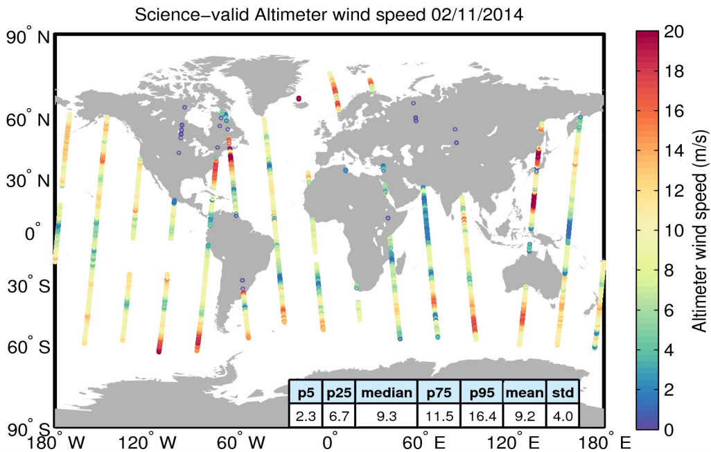
Figure 34. Geographical distribution of science-valid wind data over oceans and lakes for 02/11/2014. The statistical values shown in the table refer to the wind in m/s and are calculated over all measurements shown in the figure. Gray circles denote records that have been rejected based on the editing criteria described in Table 5.
