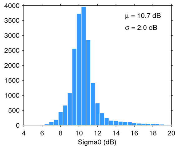
Figure 25. Histogram of flag-valid sigma0 over oceans and lakes for 02/11/2014. The mean ( \mu ) and standard deviation ( \sigma ) are also shown. Note that values outside [4 20] dB are excluded from the histogram for the sake of readability but not from the computation of \mu and \sigma .
