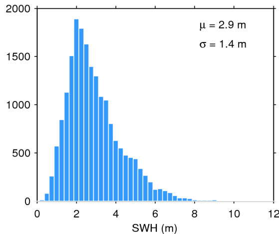
Figure 20. Histogram of science-valid SWH over oceans and lakes for 02/11/2014. The mean ( \mu ) and standard deviation ( \sigma ) are also shown. Note that values larger than 12 m are excluded from the histogram for the sake of readability but not from the computation of \mu and \sigma .
