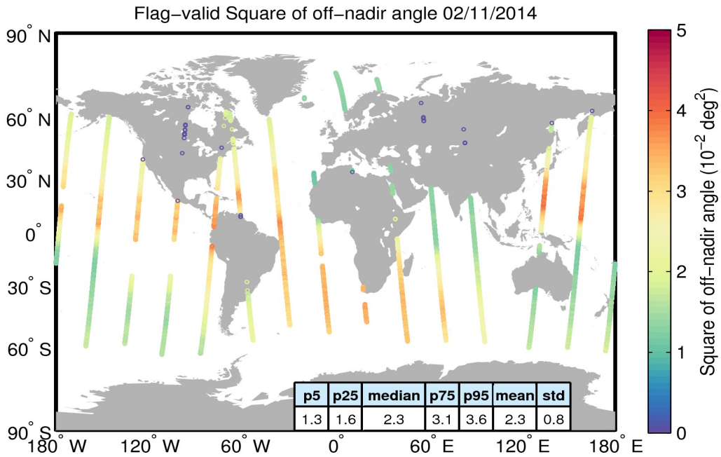
Figure 37. Geographical distribution of flag-valid mispointing data over oceans and lakes for 02/11/2014. The statistical values shown in the table refer to the mispointing in 10^{-2} \text{deg}^2 and are calculated over all measurements shown in the figure.
