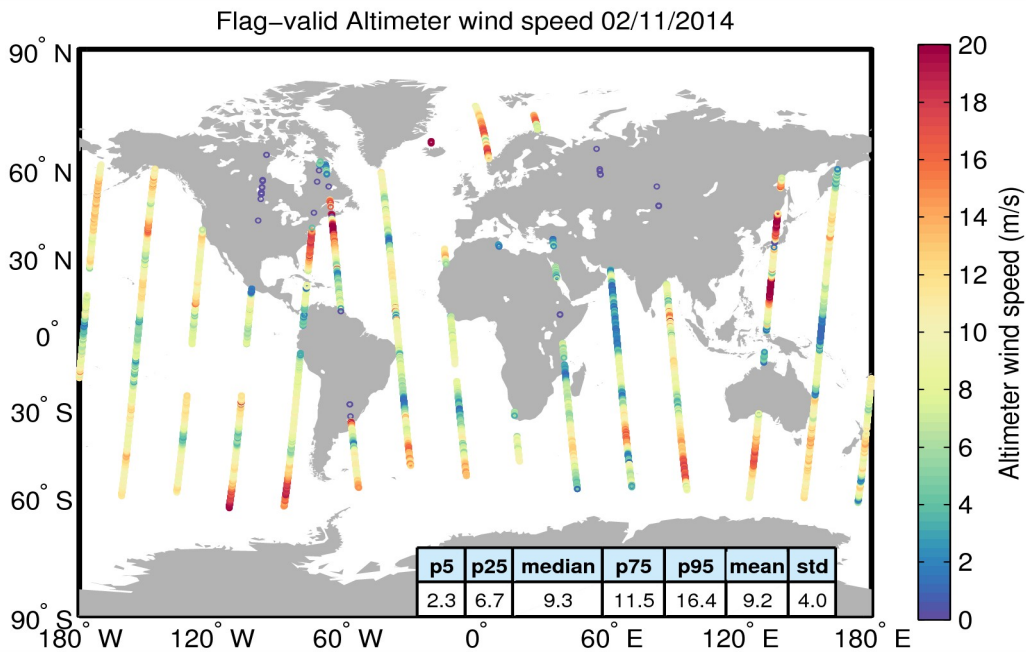
Figure 31. Geographical distribution of flag-valid wind data over oceans and lakes for 02/11/2014. The statistical values shown in the figure refer to the wind in m/s and are calculated over all measurements shown in the figure.
