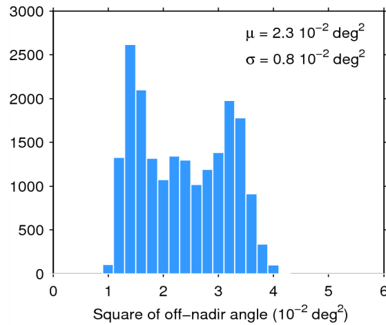
Figure 39. Histogram of flag-valid mispointing over oceans and lakes for 02/11/2014. The mean ( \mu ) and standard deviation ( \sigma ) are also shown. Note that values than 6 \cdot 10^{-2} \text{ deg}^2 are excluded from the histogram for the sake of readability but not from the computation of \mu and \sigma .
