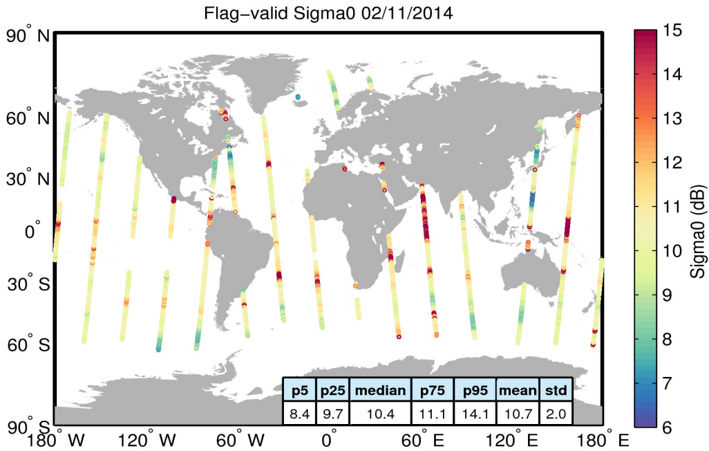
Figure 23. Geographical distribution of flag-valid sigma0 data over oceans and lakes for 02/11/2014. The statistical values shown in the table refer to the sigma0 in dB and are calculated over all measurements shown in the figure.
