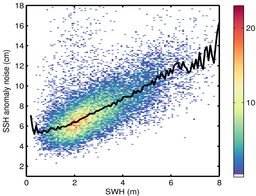
Figure 9. 2D histogram showing flag-valid SSH anomaly noise as a function of SWH for 02/11/2014. The black line denotes the median SSH anomaly as a function of SWH.
