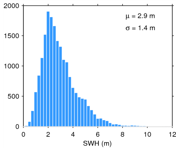
Figure 17. Histogram of flag-valid SWH over oceans and lakes for 02/11/2014. The mean ( \mu ) and standard deviation ( \sigma ) are also shown. Note that values larger than 12 m are excluded from the histogram for the sake of readability but not from the computation of \mu and \sigma .
